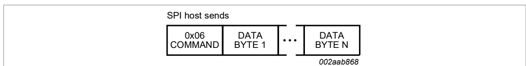
Figure 11. Read buffer
