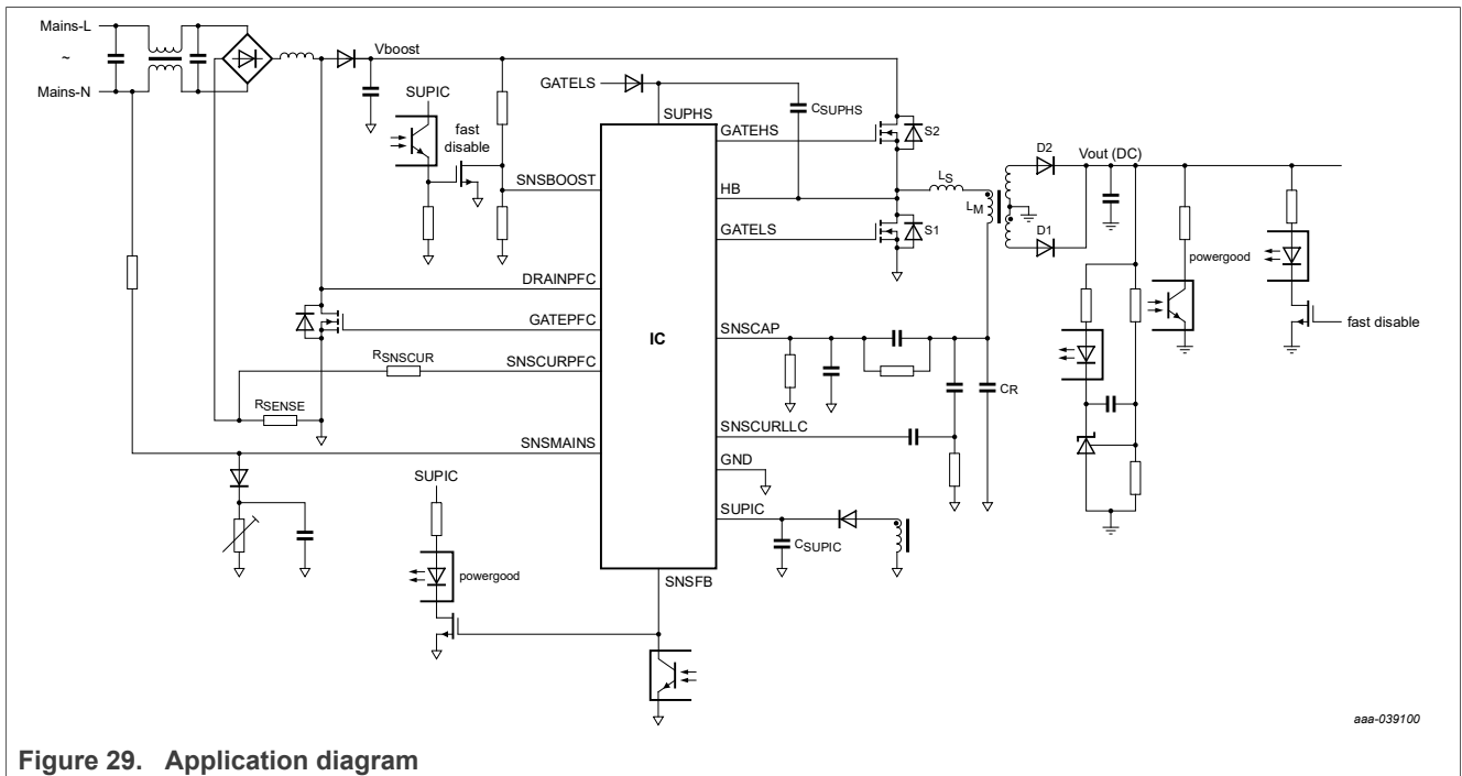
Figure 29. Application diagram
