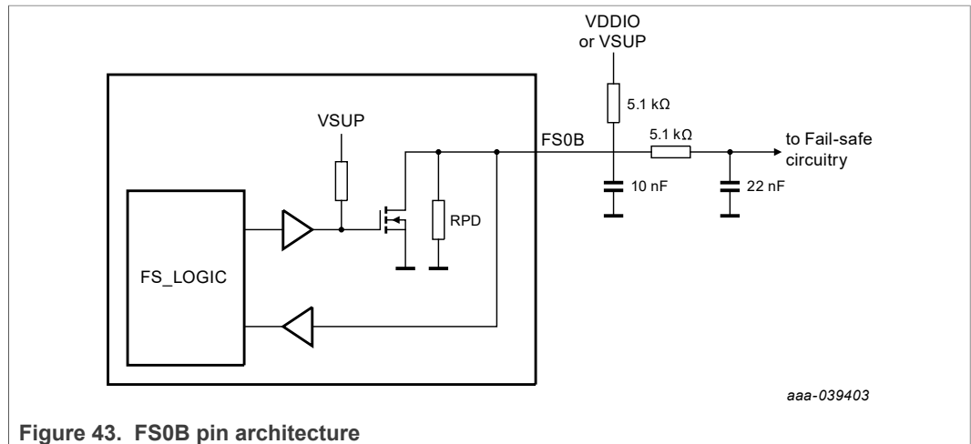
Figure 43. FS0B pin architecture
