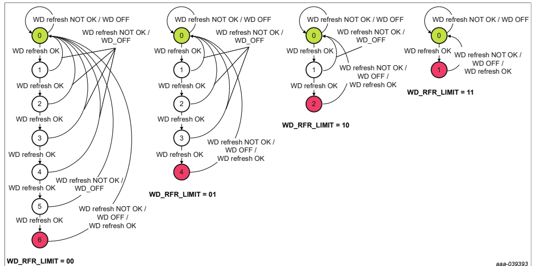
Figure 33. Watchdog refresh counter configurations
