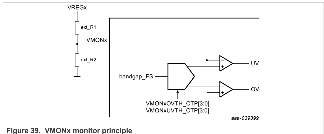
Figure 39. VMONx monitor principle
