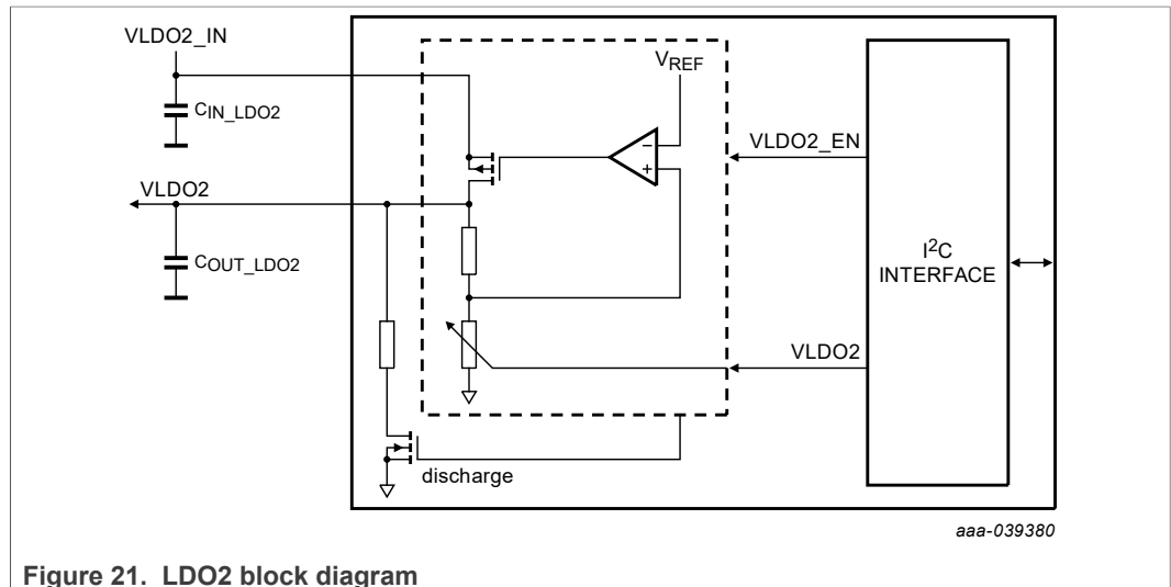
Figure 21. LDO2 block diagram
