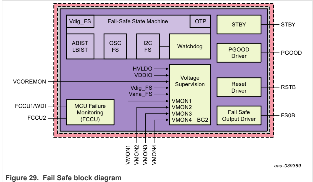
Figure 29. Fail Safe block diagram
