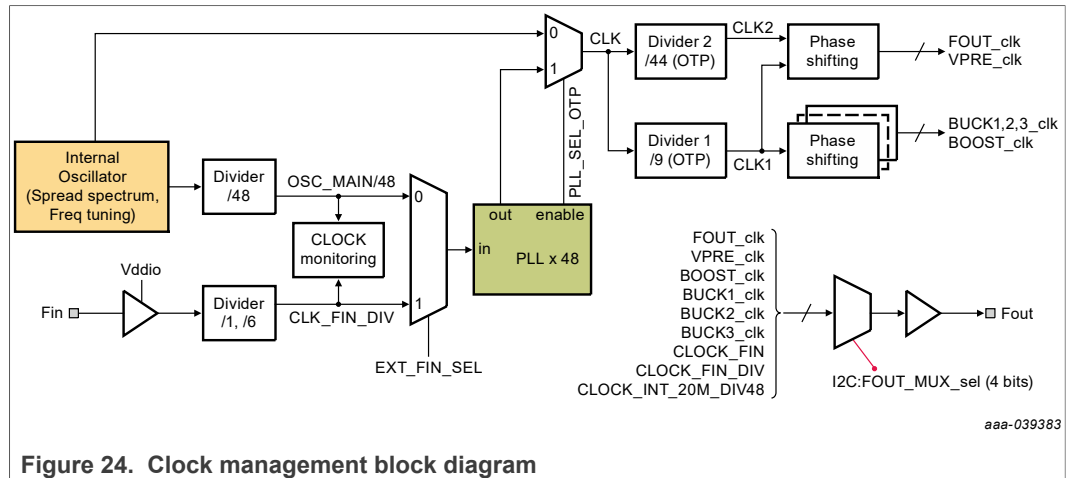
Figure 24. Clock management block diagram
