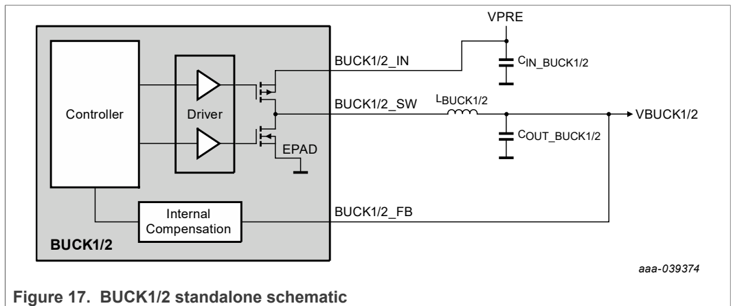
Figure 17. BUCK1/2 standalone schematic
