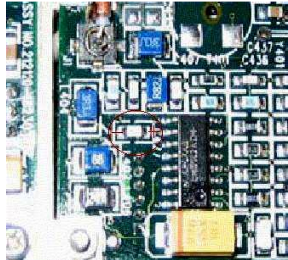
Capacitor to be modified on DDS board
