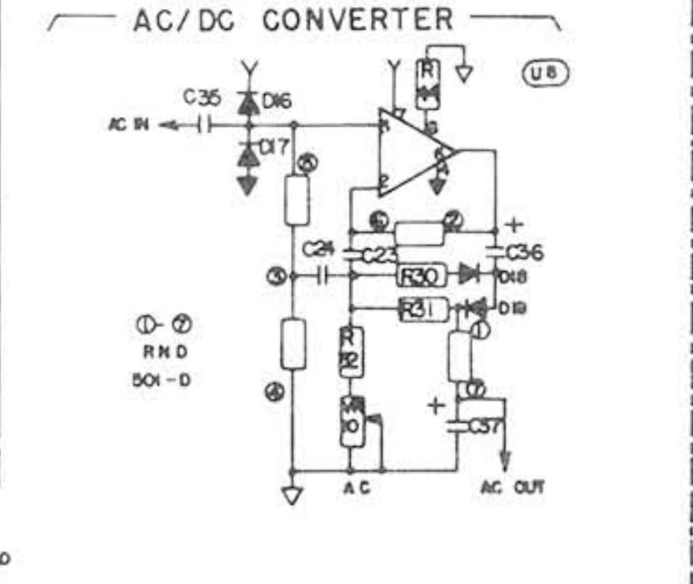
SUB PCB
