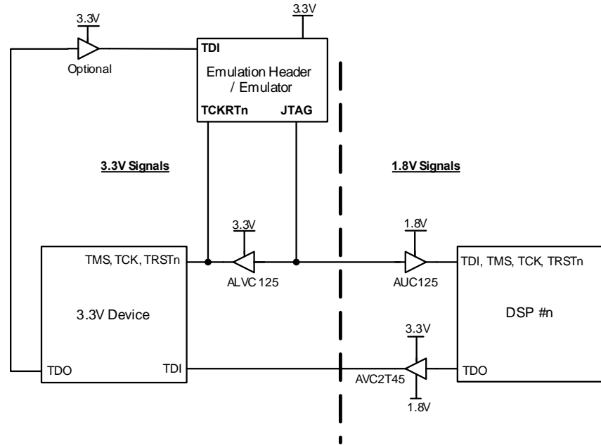
Figure 22 Emulation Voltage Translation with Buffers
