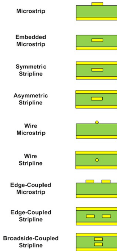
Figure 45 Transmission Line Geometries
