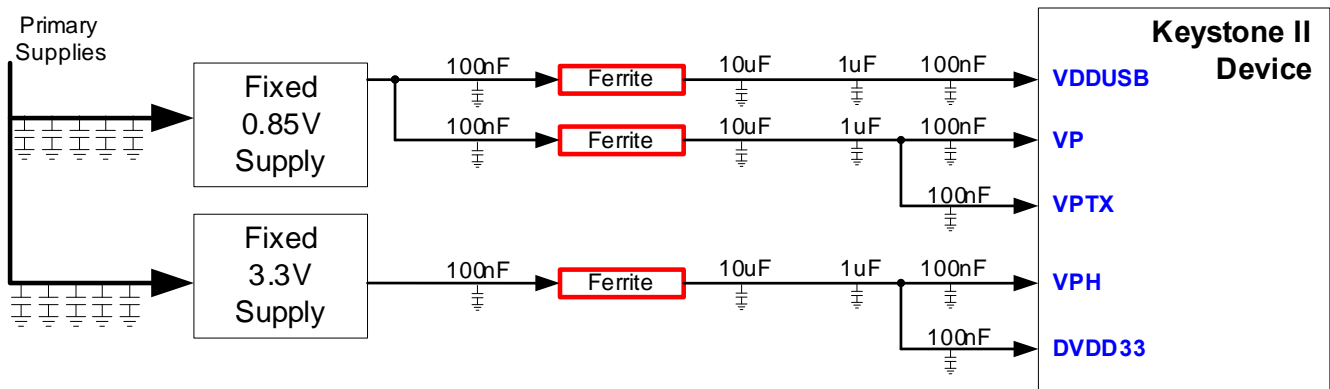
Figure 8 USB Power Supply Filters
