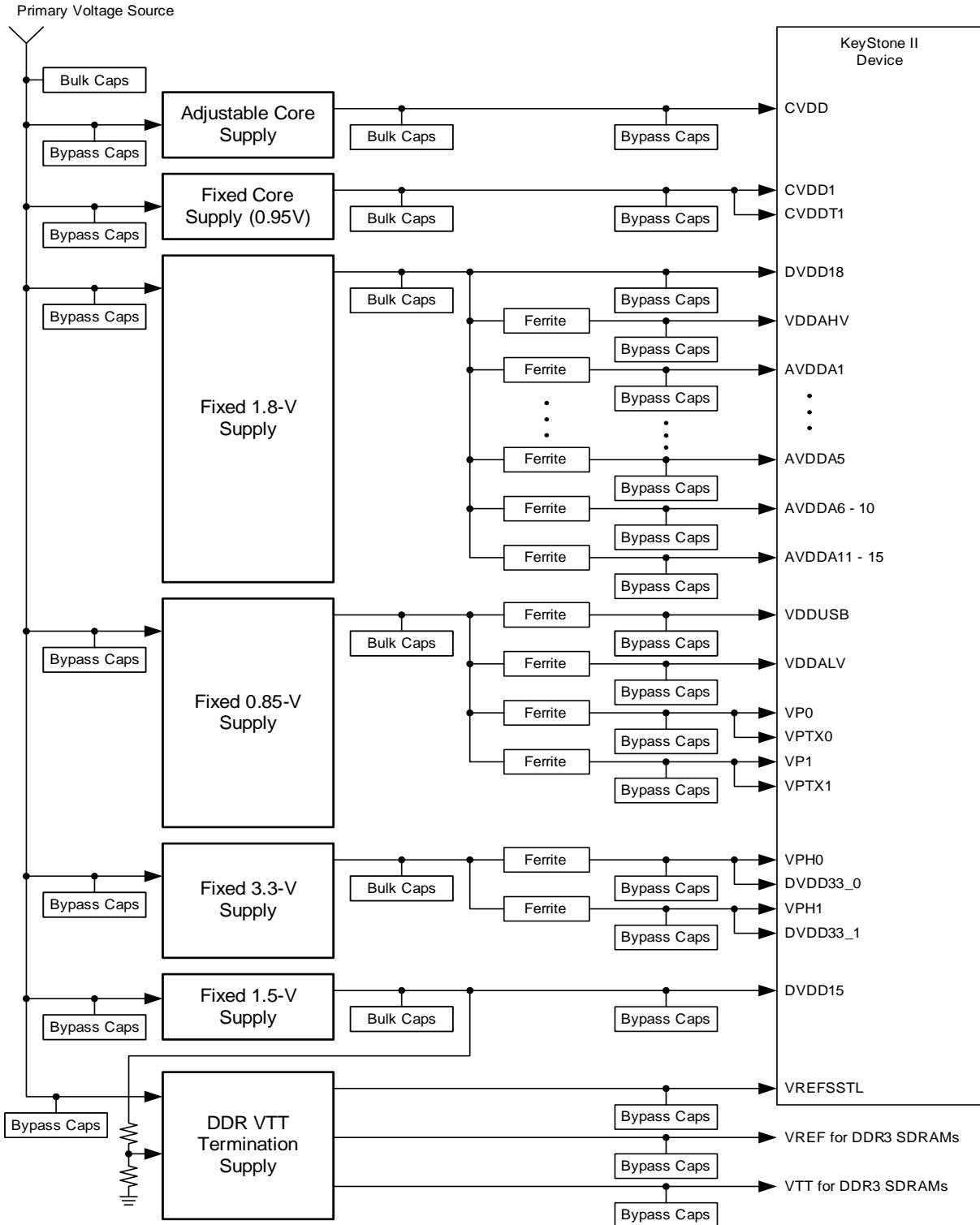
Figure 1 KeyStone II Power Supply Planes (Rails)
