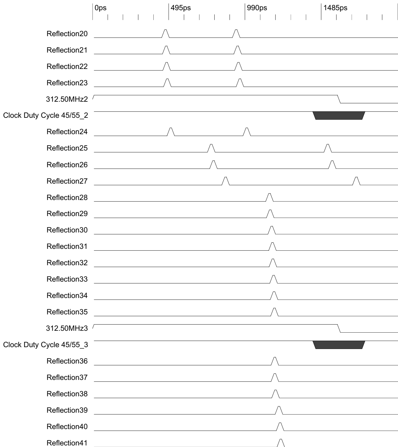
Figure 44 Reflections Timing Analysis
