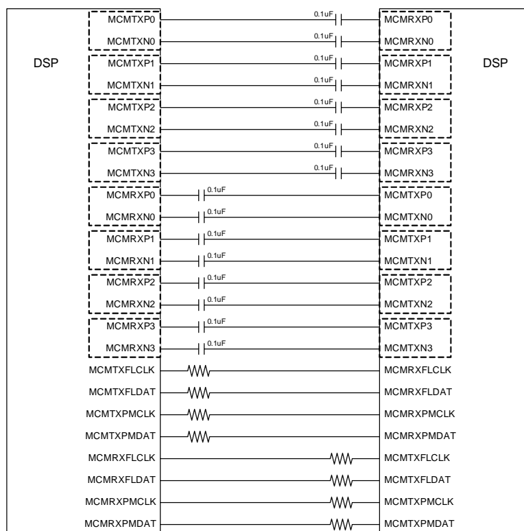
Figure 24 HyperLink Bus DSP-to-DSP Connection
