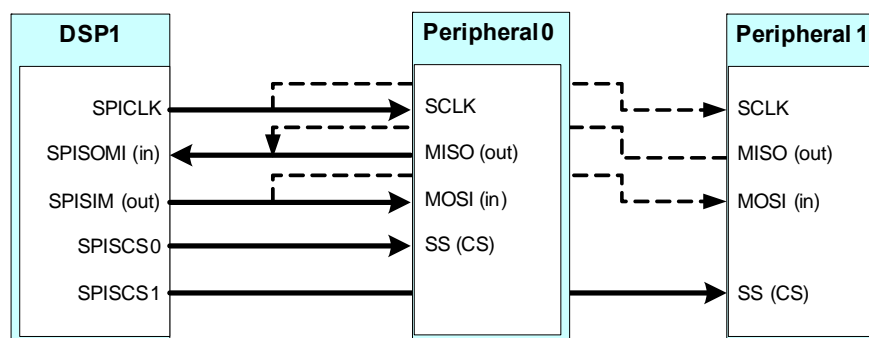
Figure 29 SPI Connections
