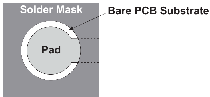
Figure 34 Non-Solder-Mask Defined (NSMD) PCB Land
