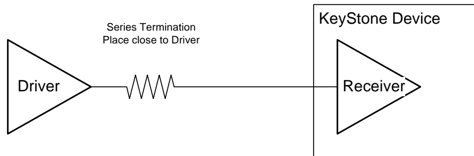
Figure 33 Basic Series Termination
