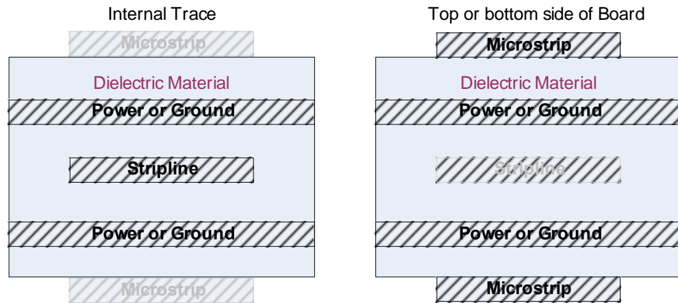
Figure 36 Stripline and Microstrip Topologies
