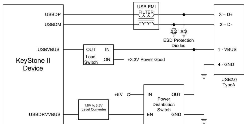
Figure 30 USB2.0 Host Connection
