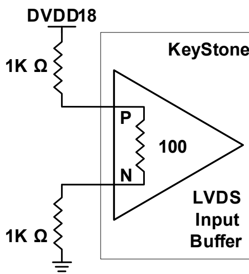
Figure 16 Unused LVDS Clock Input Connection
