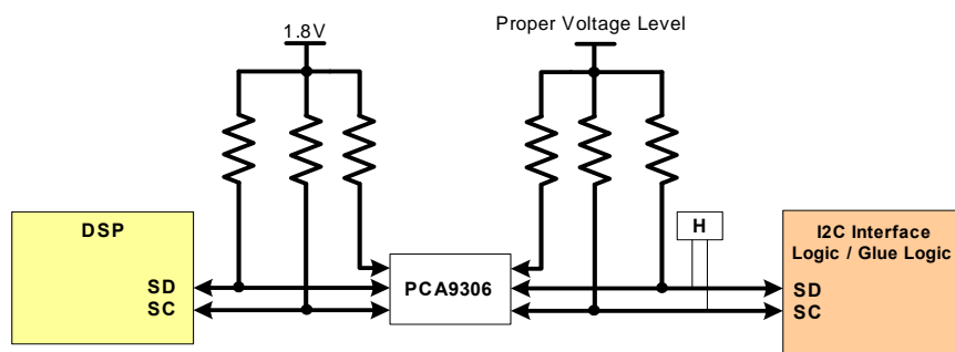
Figure 25 I 2 C Voltage Level Translation
