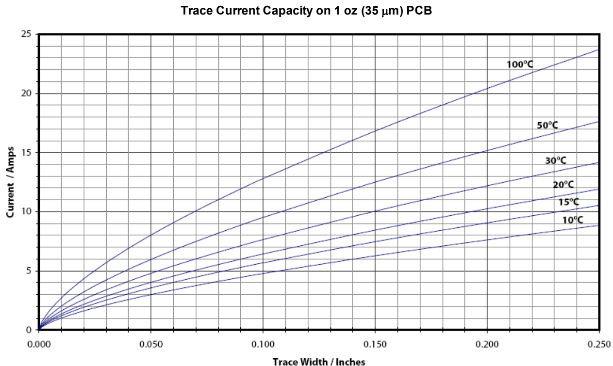
Figure 37 Trace Width to Current Specifications
