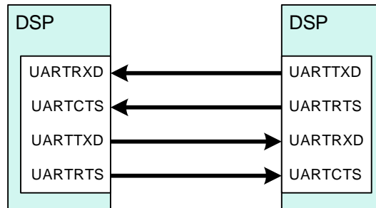
Figure 28 UART Connections with Autoflow Support
