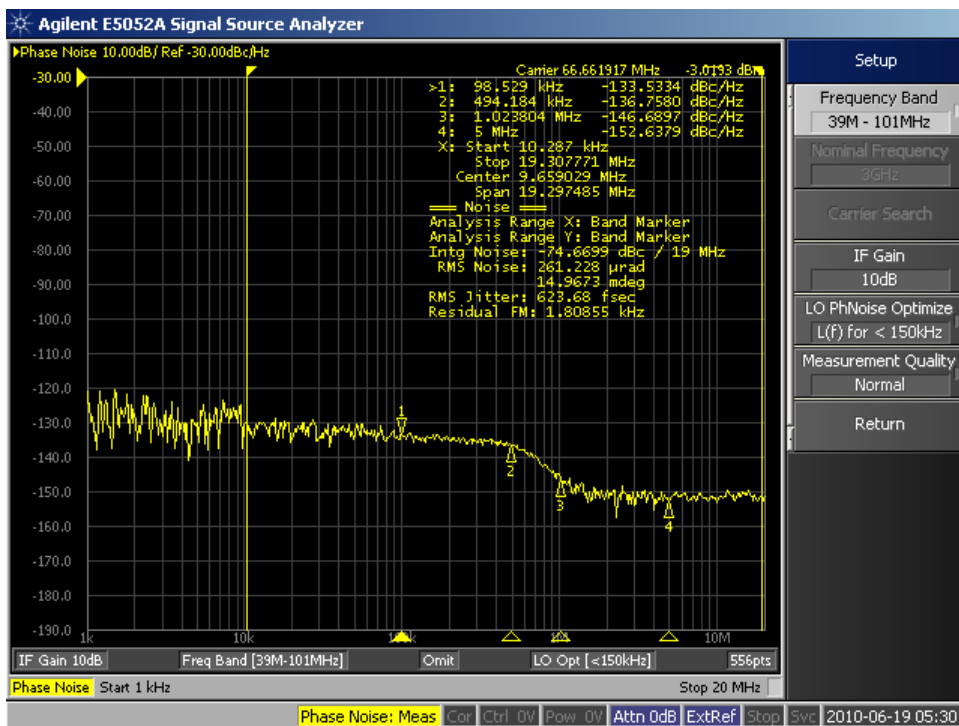
Figure 39 Phase Noise Plot - CECE62002/5 @ 66.667 MHz
