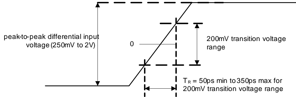
Figure 12 System Clock Rise Time
