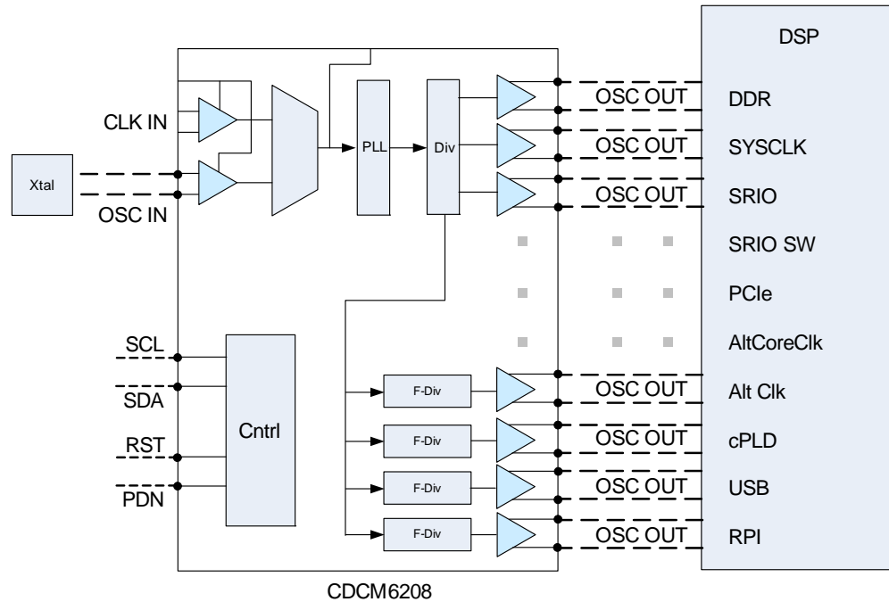
Figure 17 Clock Fan Out - for Single Device
