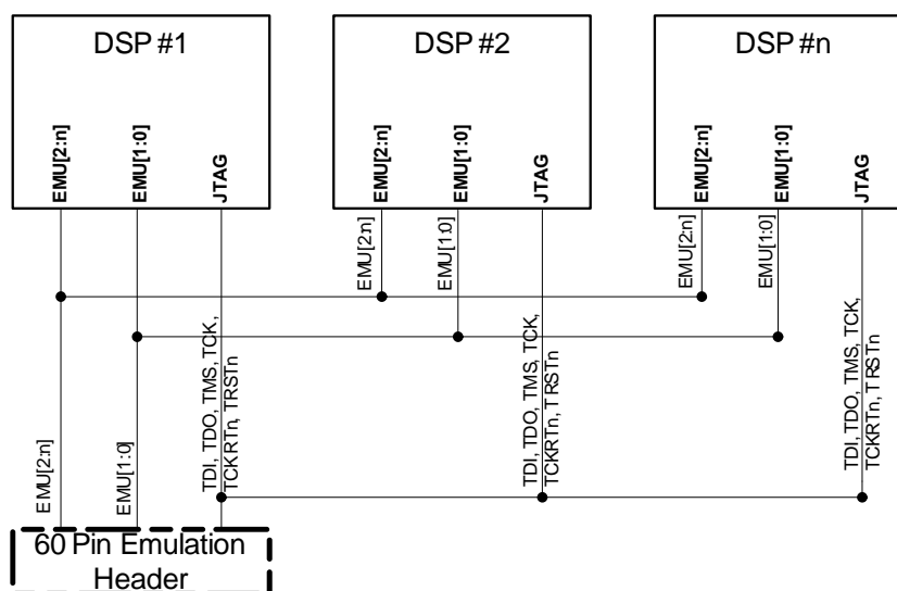
Figure 21 Emulator with Trace Solution #2
