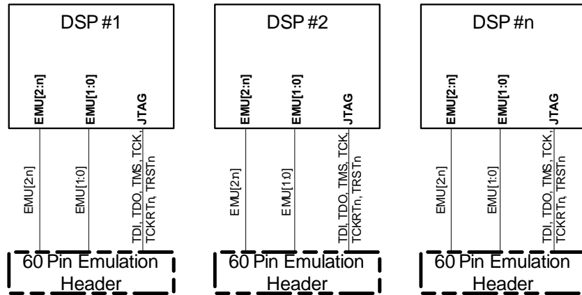
Figure 20 Emulator with Trace Solution #1
