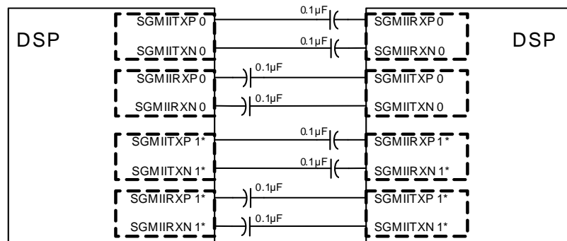
Figure 26 SGMII MAC to MAC Connection
