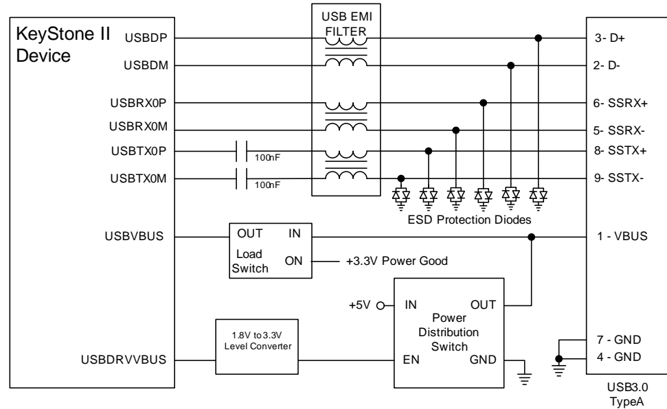
Figure 31 USB3.0 Host Connection
