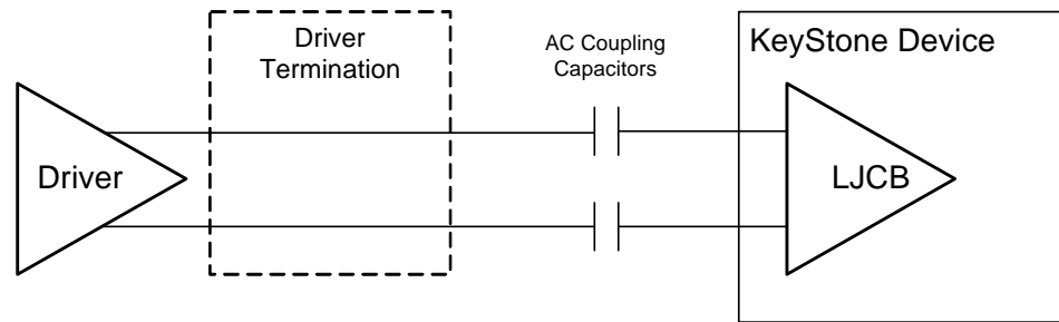
Figure 32 LJCB Clock Inputs
