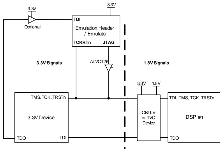
Figure 23 Emulator Voltage Translation with Switches
