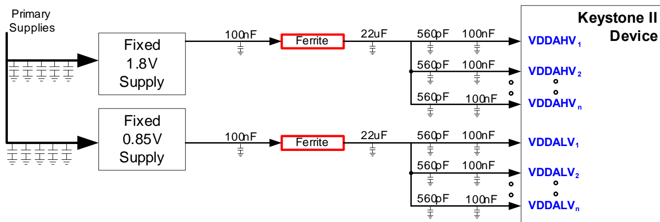
Figure 7 VDDAHV & VDDALV Power Supply Filters
