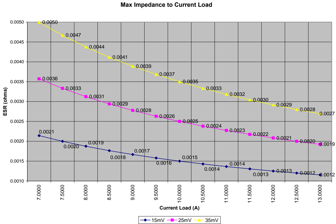
Figure 11 ESR Plot for Delta Current to Tolerance #3
