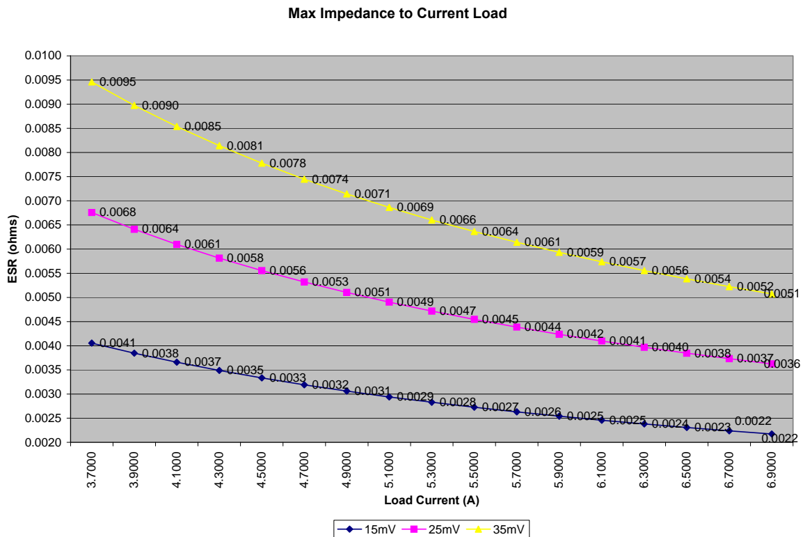
Figure 10 ESR Plot for Delta Current to Tolerance #2
