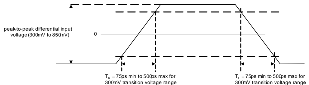
Figure 14 USB Clock Rise Time
