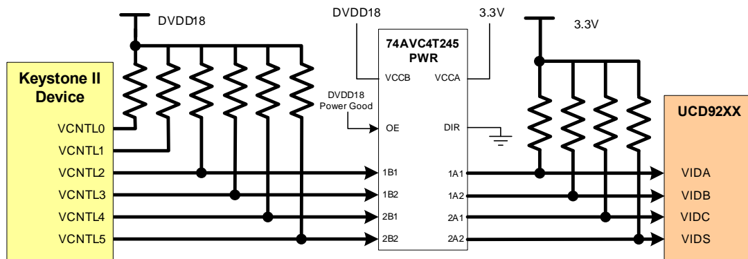
Figure 4 VCNTL Level Translation
