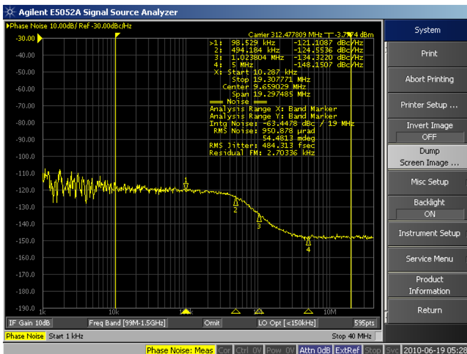
Figure 43 Phase Noise Plot - CECE62002/5 @ 312.50 MHz
