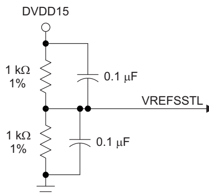
Figure 5 DDR3 VREFSSTL Voltage Divider
