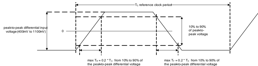
Figure 13 SerDes/CML Clock Rise Time
