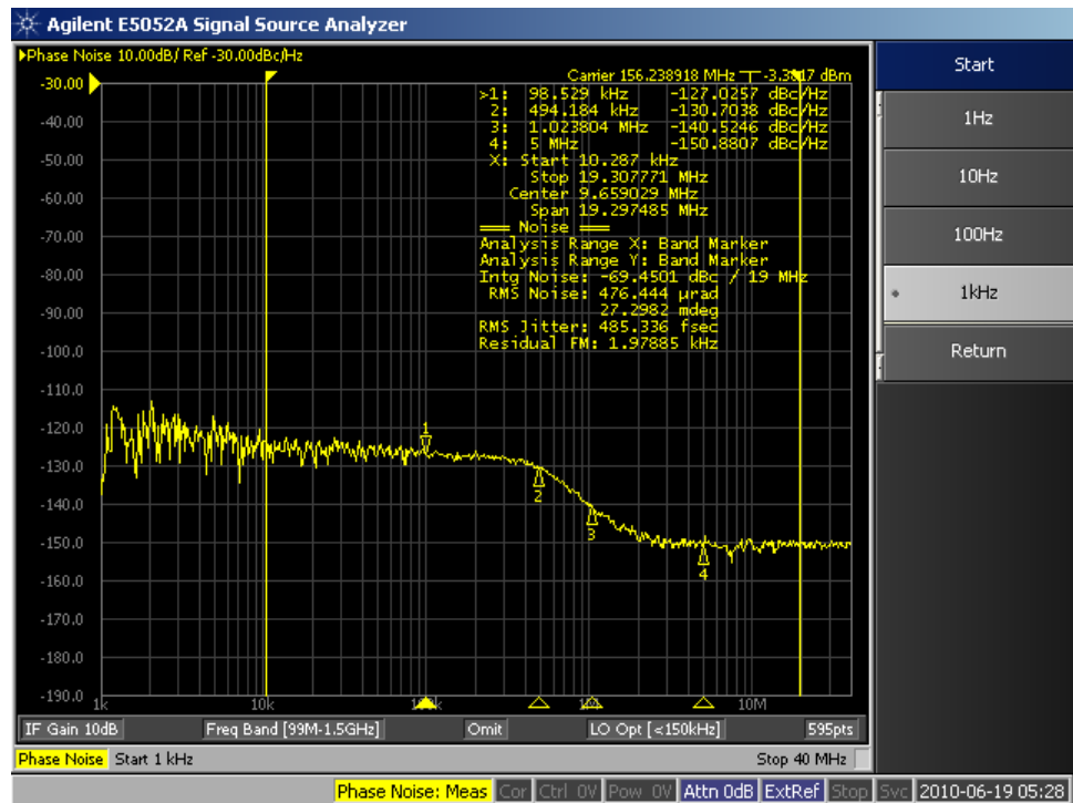
Figure 42 Phase Noise Plot - CECE62002/5 @ 156.25 MHz
