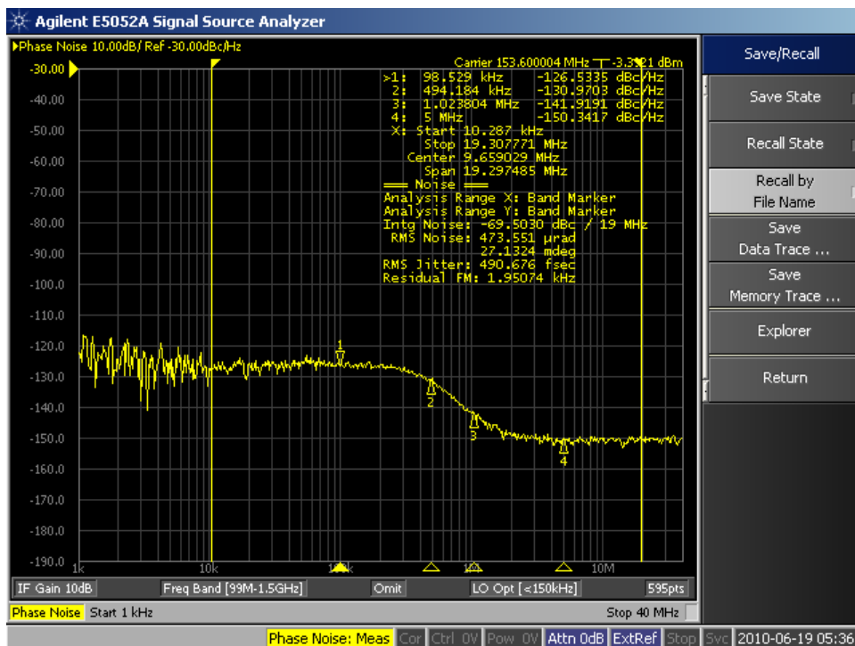
Figure 41 Phase Noise Plot - CECE62002/5 @ 153.60 MHz
