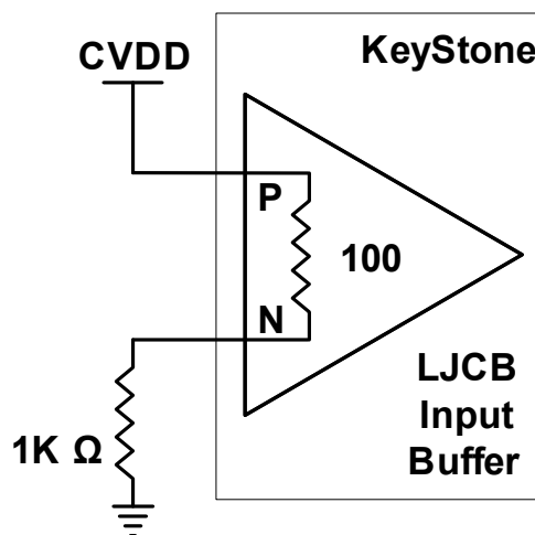
Figure 15 Unused LJCBS Clock Input Connection
