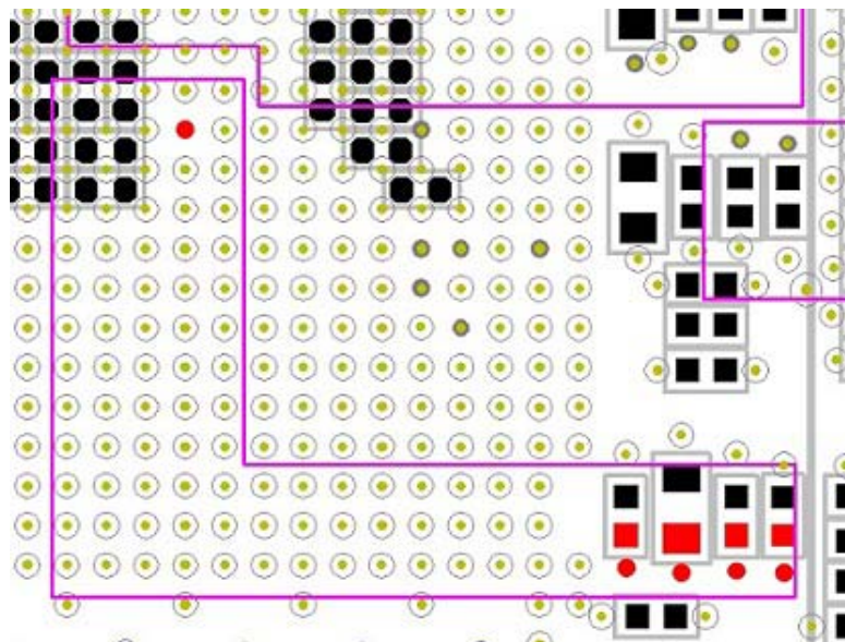
Figure 35 Filtered Voltage Plane
