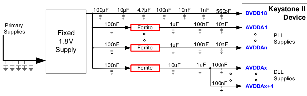
Figure 6 AVDDAx Power Supply Filter
