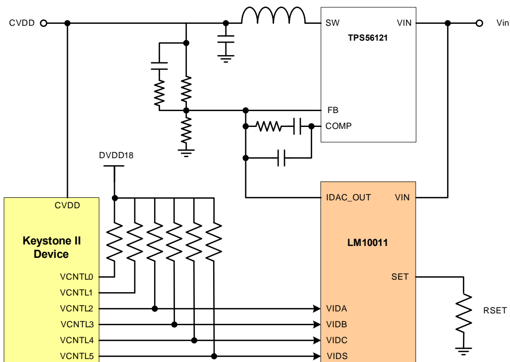
Figure 2 LM10011/TPS56121 CVDD Supply Block Diagram
