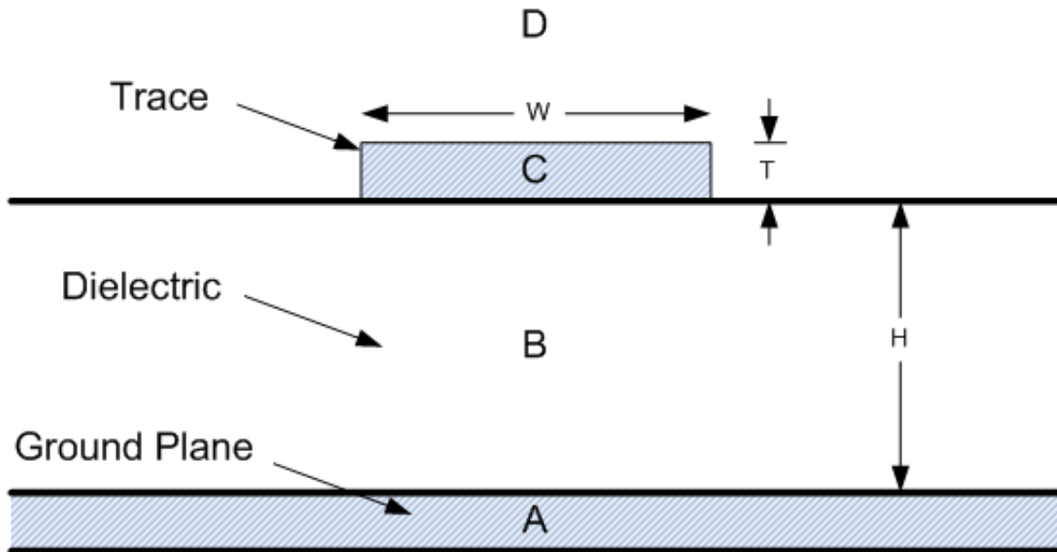
Figure 47 Microstrip Transmission Line Construction
