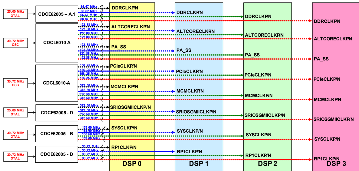
Figure 18 Clock Fan Out - Multiple DSPs
