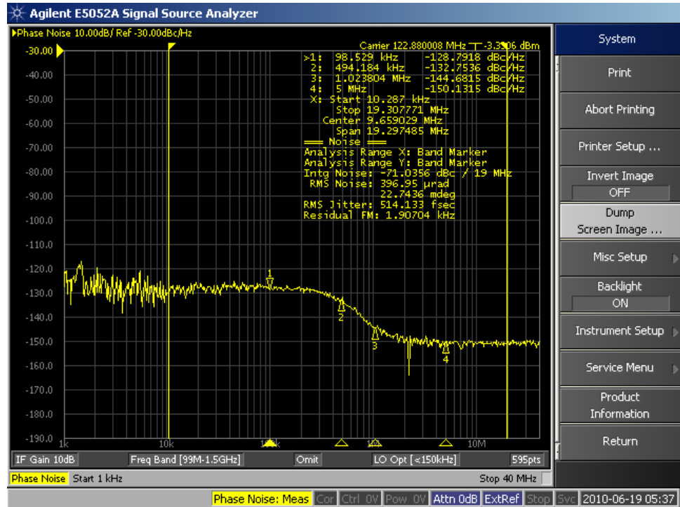
Figure 40 Phase Noise Plot - CECE62002/5 @ 122.88 MHz
