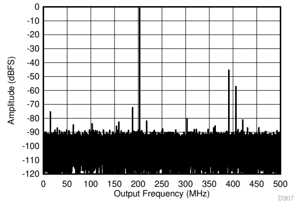
Figure 7-14. Single Tone FFT at 1797 MHz and -1 dBFS
