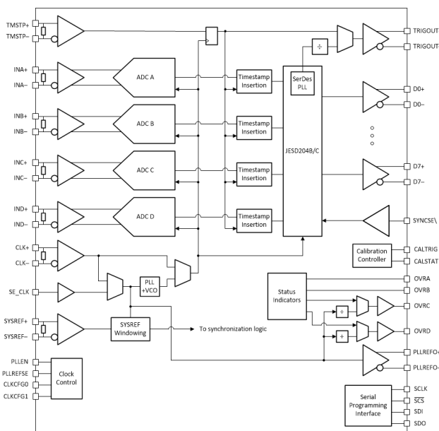
Quad Channel Block Diagram
