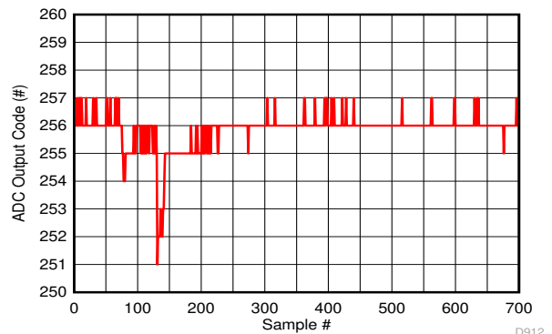
Figure 7-126. Background Calibration Core Transition (midscale voltage)
