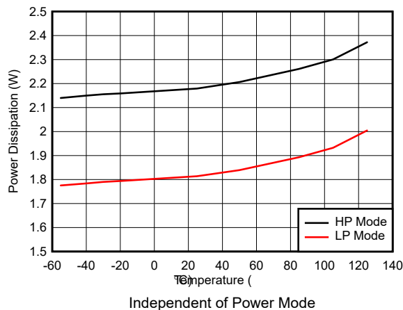
Figure 7-113. Quad Channel, Power Dissipation vs Temperature
