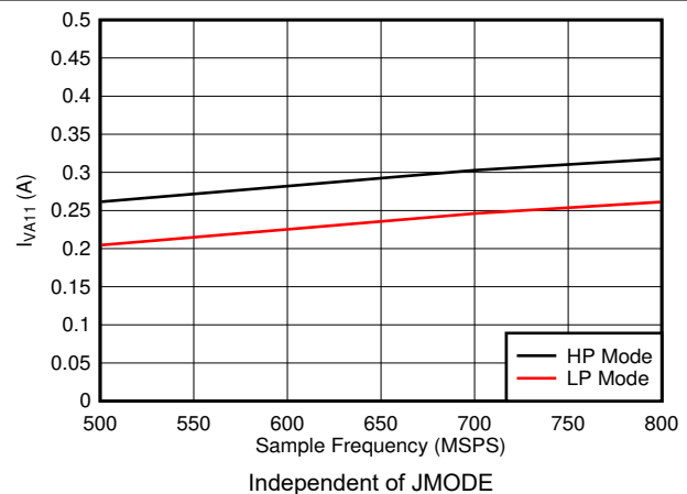
Figure 7-96. Single Channel, I_{VA11} vs F_S
