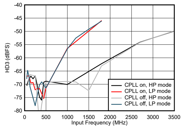
Figure 7-70. HD3 vs Input Frequency and CPLL and Power Mode
