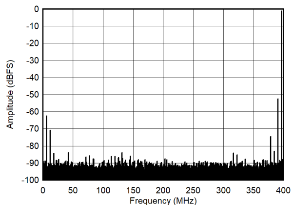
Figure 7-12. Single Tone FFT at 1197MHz and -1dBFS
