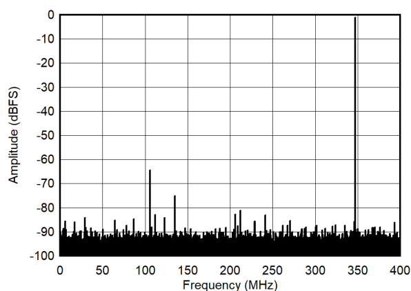
Figure 7-4. Single Tone FFT at 347 MHz and -1dBFS
