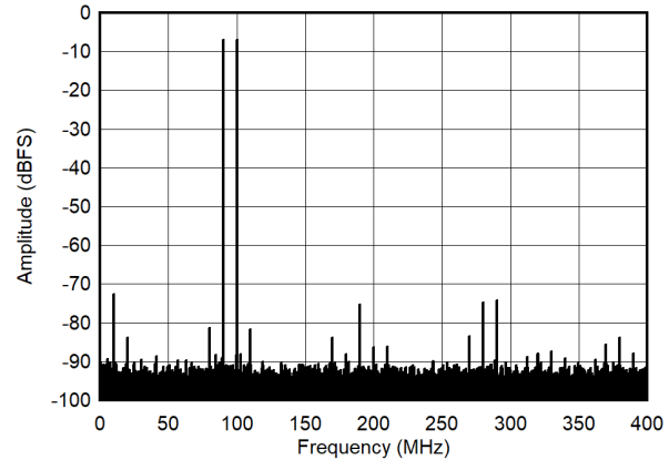
Figure 7-56. Dual Tone FFT at 95 MHz (LP Mode)
