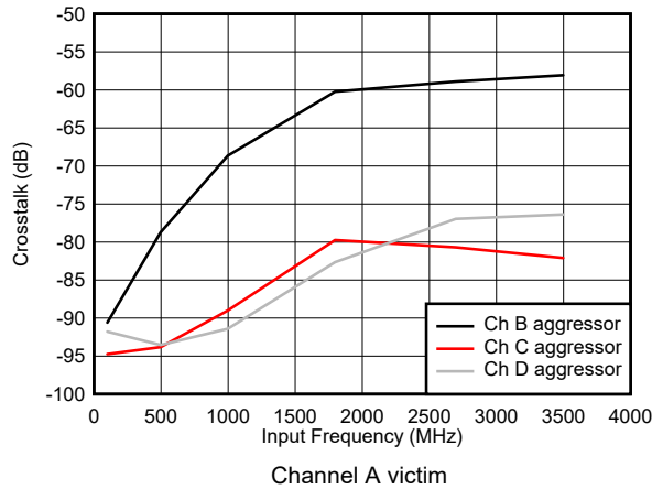
Figure 7-61. Crosstalk vs Input Frequency
