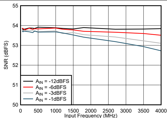
Figure 7-15. SNR vs Input Frequency
