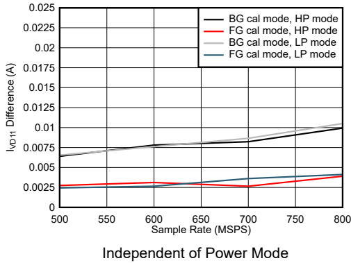
Figure 7-111. Dual Channel, I_{VD11} Change with Calibration Mode
