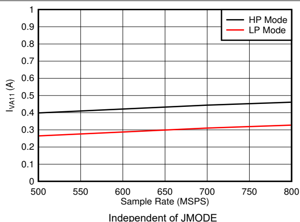
Figure 7-76. Quad Channel, I_{VA11} vs F_S
