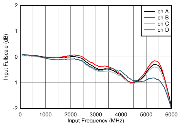
Figure 7-3. Input Fullscale vs Input Frequency
