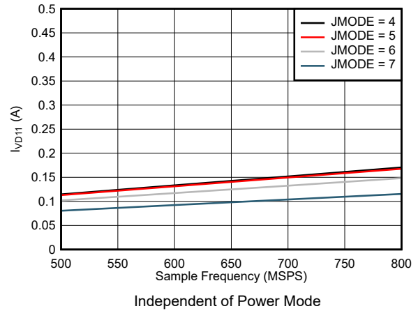
Figure 7-98. Single Channel, I_{VD11} vs F_S for JMODES 4 - 7
