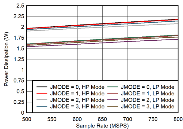
Figure 7-71. Quad Channel, Power Dissipation vs F_S for JMODES 0 - 3
