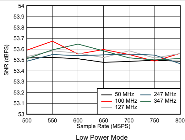
Figure 7-25. SNR vs Sample Rate
