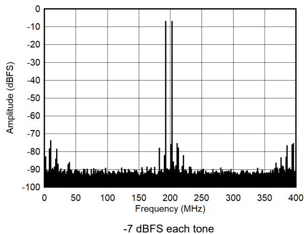
Figure 7-52. Dual Tone FFT at 998 MHz
