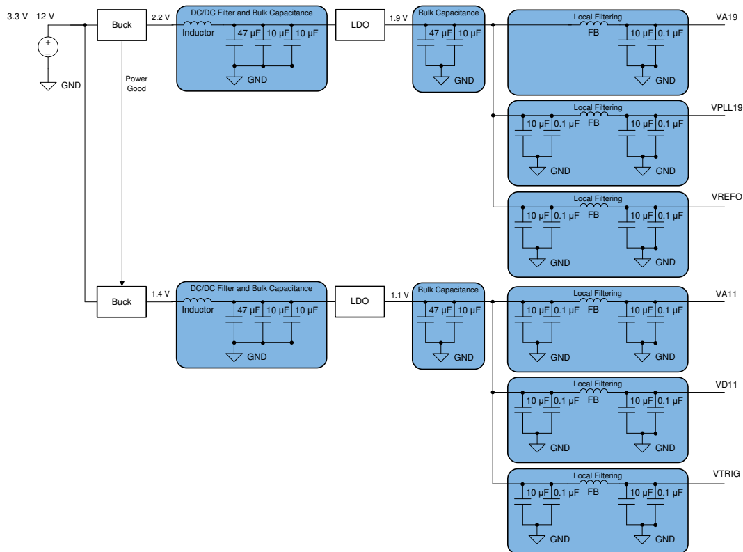
Figure 10-1. LDO Linear Regulator Approach Example
