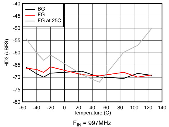
Figure 7-38. HD3 vs Temperature
