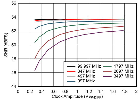
Figure 7-32. SNR vs Clock Amplitude
