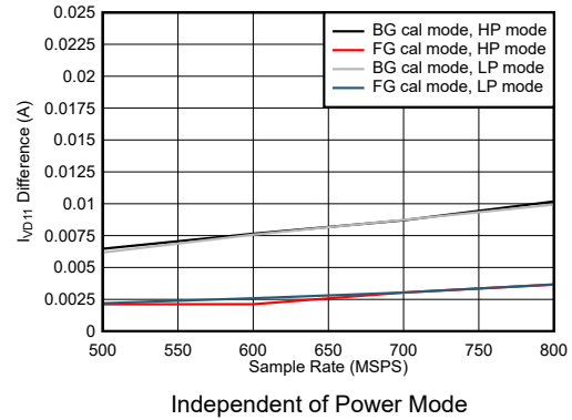
Figure 7-112. Single Channel, I_{VD11} Change with Calibration Mode
