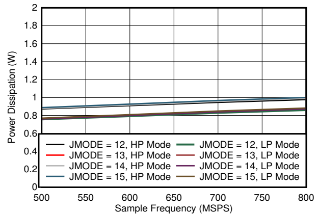
Figure 7-94. Single Channel, Power Dissipation vs F_S for JMODES 12 - 15
