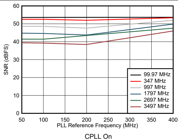
Figure 7-63. SNR vs Reference Clock Frequency
