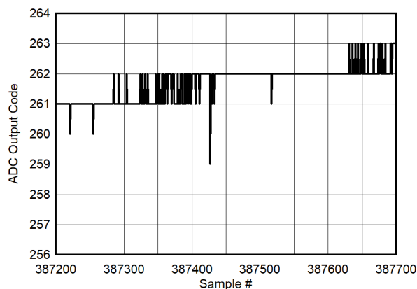
Figure 7-118. Background Core Transition (AC Signal Zoomed)
