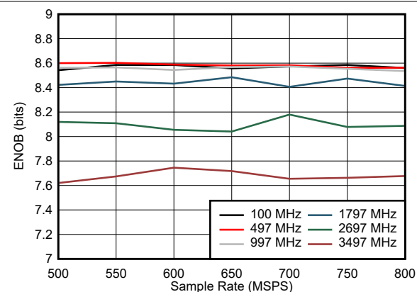
Figure 7-23. ENOB vs Sample Rate
