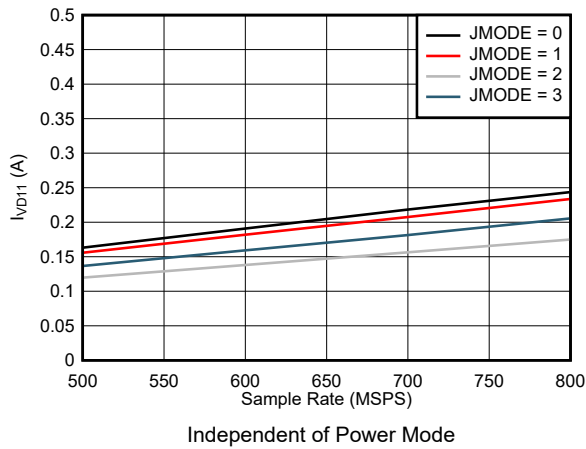
Figure 7-87. Dual Channel, I_{VD11} vs F_S for JMODES 0 - 3
