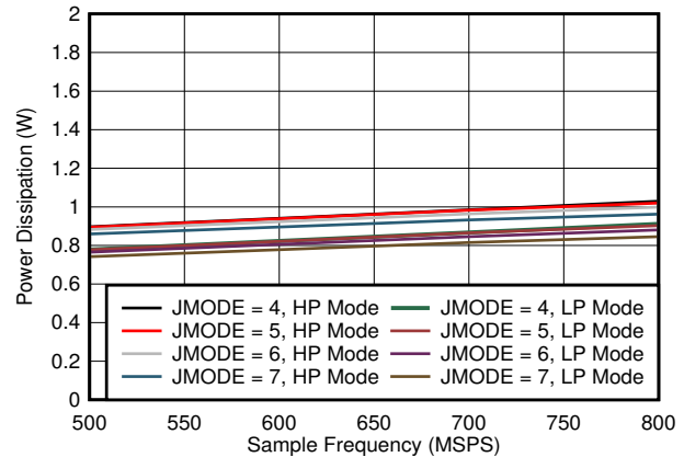
Figure 7-92. Single Channel, Power Dissipation vs F_S for JMODES 4 - 7
