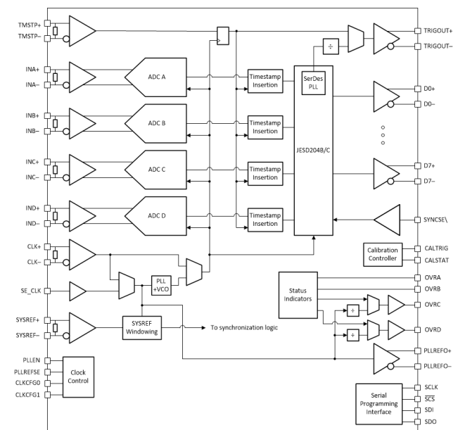
Quad Channel Block Diagram
