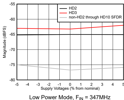
Figure 7-49. HD2, HD3 and Worst non-HD2/3 Spur vs Supply Voltage
