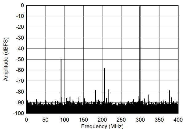
Figure 7-9. Single Tone FFT at 3497 MHz and -1dBFS
