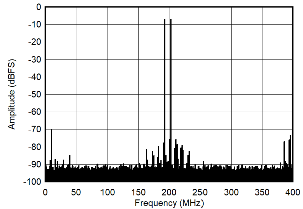
Figure 7-58. Dual Tone FFT at 998 MHz (LP Mode)
