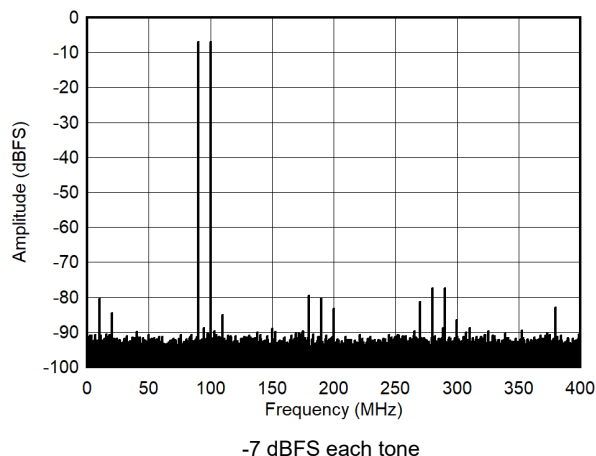
Figure 7-50. Dual Tone FFT at 95 MHz
