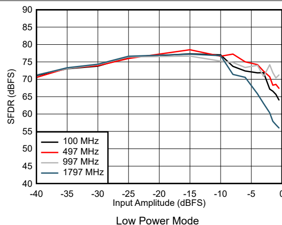
Figure 7-30. SFDR vs Input Amplitude
