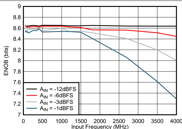
Figure 7-17. ENOB vs Input Frequency
