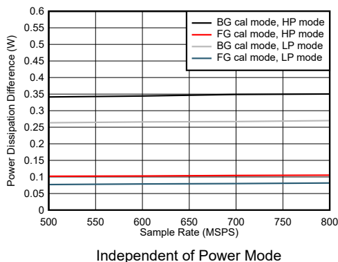
Figure 7-101. Quad Channel, Power Dissipation Change with Calibration Mode
