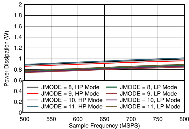
Figure 7-93. Single Channel, Power Dissipation vs F_S for JMODES 8 - 11
