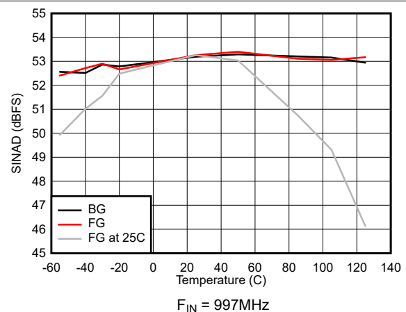
Figure 7-36. SINAD vs Temperature
