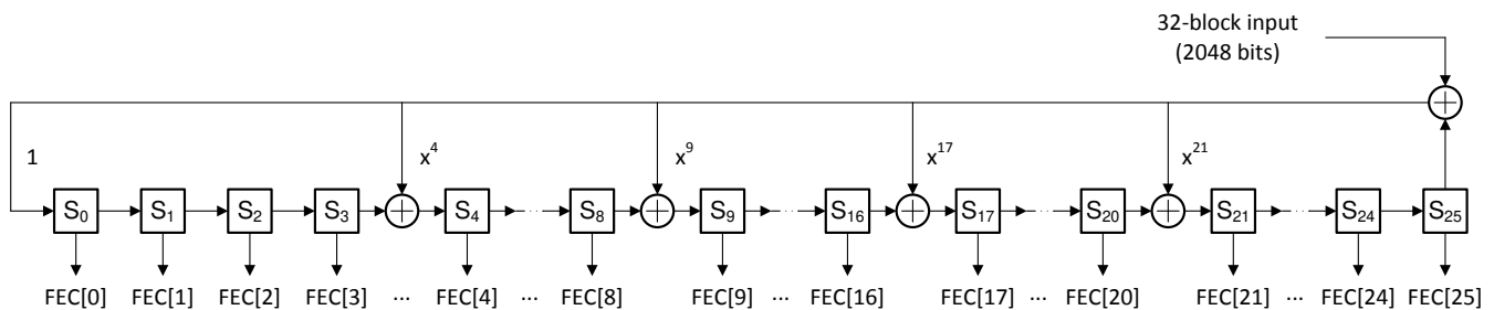
Figure 8-10. FEC Parity Bit Generator
