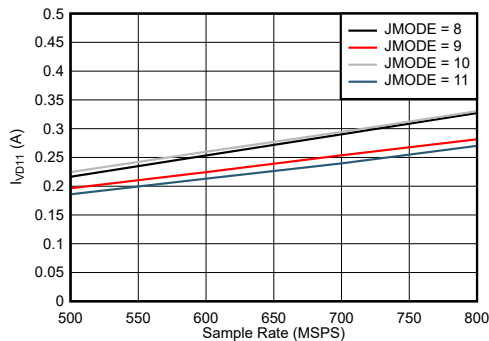
Figure 7-79. Quad Channel, I_{VD11} vs F_S for JMODES 8 - 11
