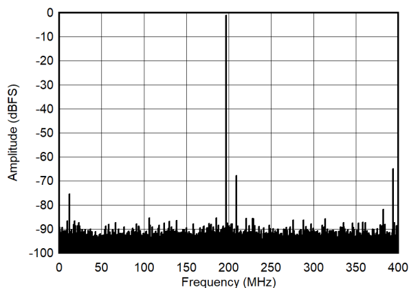
Figure 7-5. Single Tone FFT at 997 MHz and -1dBFS
