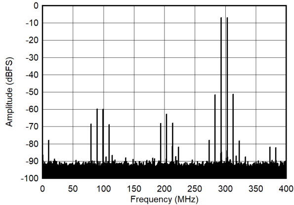
Figure 7-55. Dual Tone FFT at 2698 MHz
