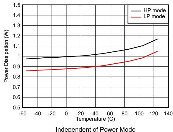
Figure 7-115. Single Channel, Power Dissipation vs Temperature
