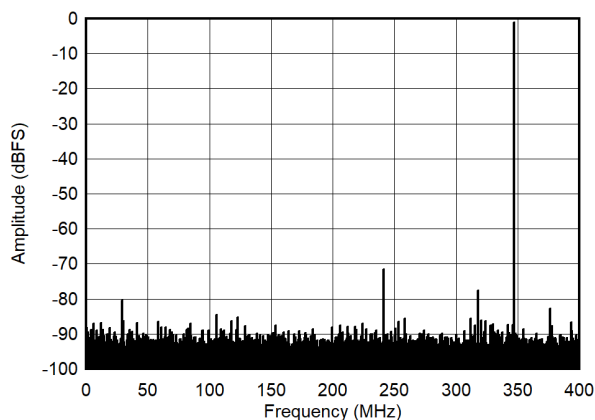
Figure 7-11. Single Tone FFT at 347MHz and -1dBFS
