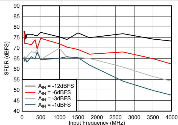
Figure 7-14. SFDR vs Input Frequency
