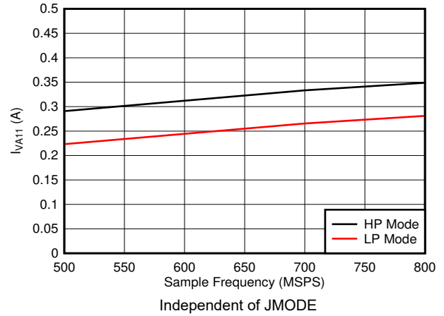
Figure 7-86. Dual Channel, I_{VA11} vs F_S
