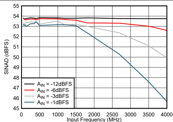
Figure 7-16. SINAD vs Input Frequency
