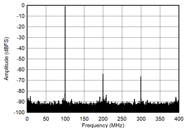
Figure 7-10. Single Tone FFT at 100MHz and -1dBFS
