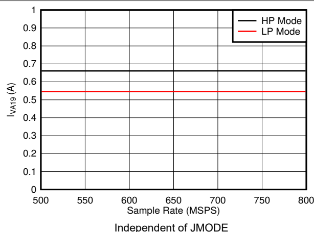
Figure 7-75. Quad Channel, I_{VA19} vs F_S
