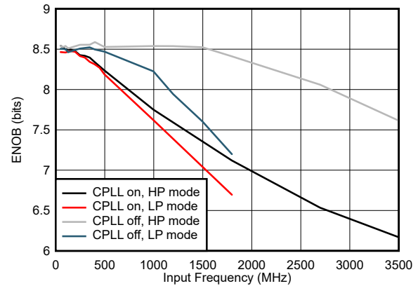
Figure 7-68. ENOB vs Input Frequency and CPLL and Power Mode
