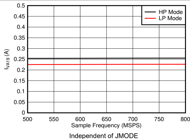
Figure 7-95. Single Channel, I_{VA19} vs F_S
