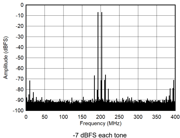
Figure 7-53. Dual Tone FFT at 1798 MHz
