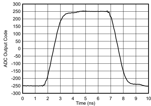
Figure 9-2. Measured Pulse using Sub-Sampling Technique for Equivalent 25.6 GSPS Measurement
