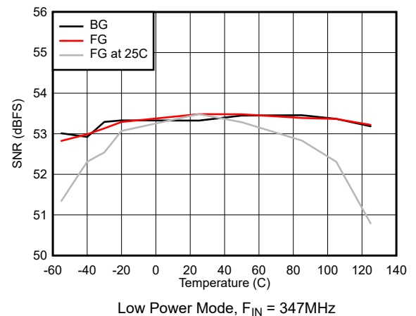
Figure 7-40. SNR vs Temperature
