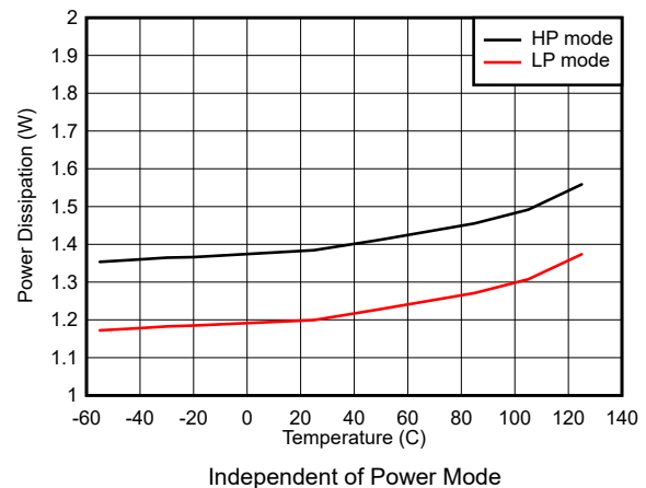
Figure 7-114. Dual Channel, Power Dissipation vs Temperature
