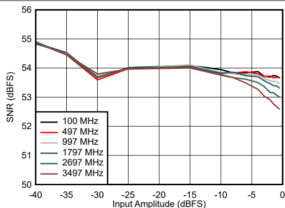
Figure 7-29. SNR vs Input Amplitude
