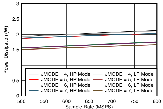
Figure 7-72. Quad Channel, Power Dissipation vs F_S for JMODES 4 - 7
