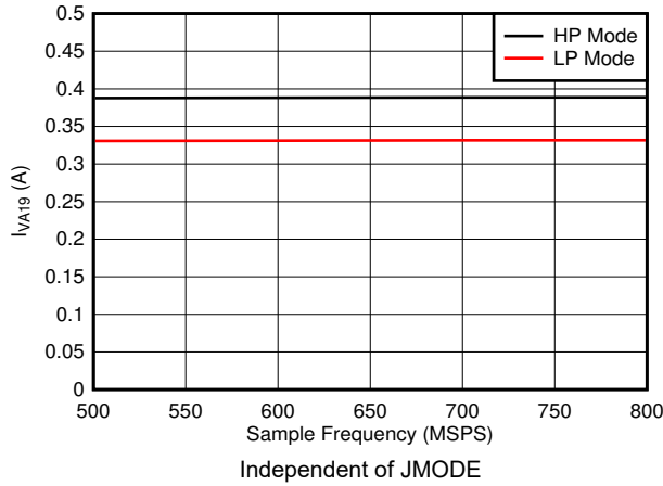
Figure 7-85. Dual Channel, I_{VA19} vs F_S
