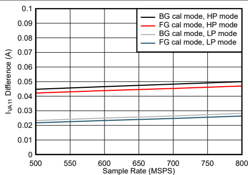
Figure 7-107. Quad Channel, I_{VA11} Change with Calibration Mode
