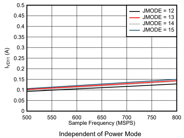
Figure 7-100. Single Channel, I_{VD11} vs F_S for JMODES 12 - 15
