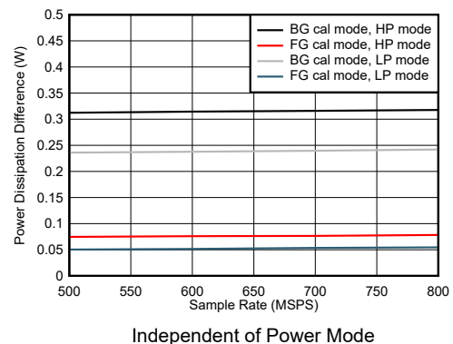
Figure 7-102. Dual Channel, Power Dissipation Change with Calibration Mode
