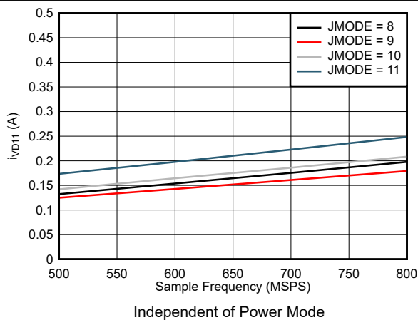
Figure 7-89. Dual Channel, I_{VD11} vs F_S for JMODES 8 - 11
