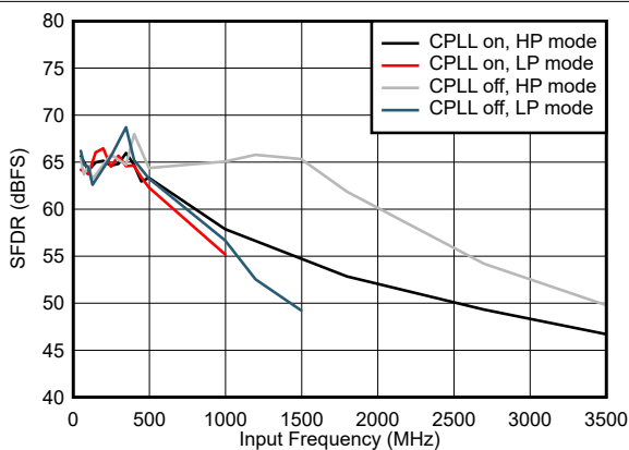
Figure 7-65. SFDR vs Input Frequency and CPLL and Power Mode
