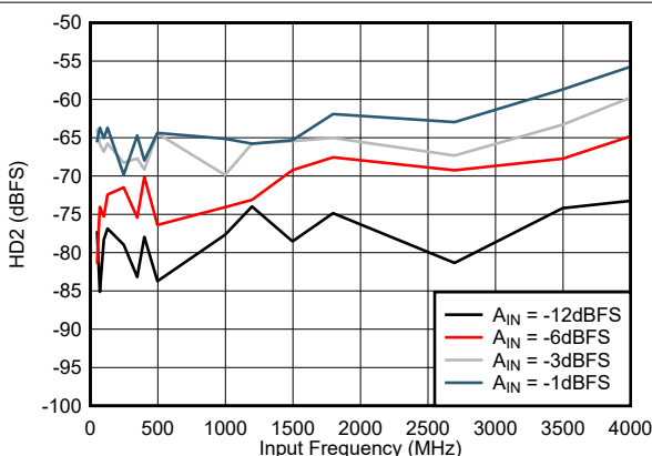
Figure 7-18. HD2 vs Input Frequency
