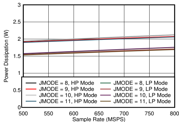
Figure 7-73. Quad Channel, Power Dissipation vs F_S for JMODES 8 - 11
