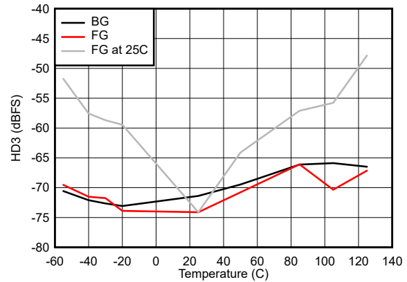
Figure 7-44. HD3 vs Temperature
