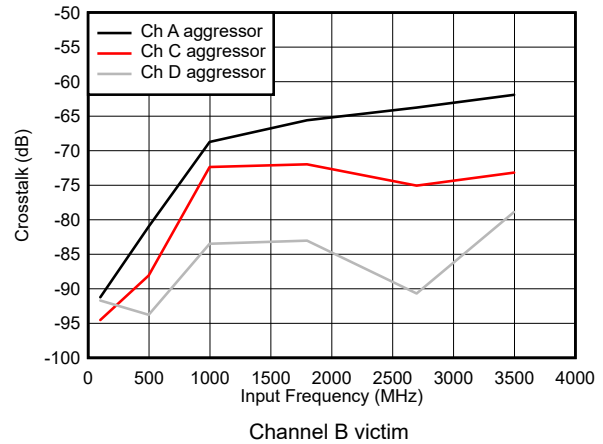
Figure 7-62. Crosstalk vs Input Frequency
