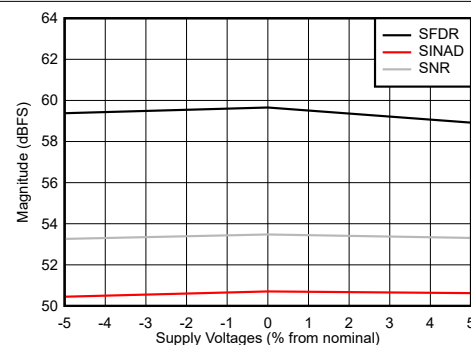
Figure 7-48. SNR, SFDR and SINAD vs Supply Voltage
