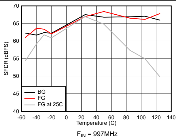
Figure 7-35. SFDR vs Temperature
