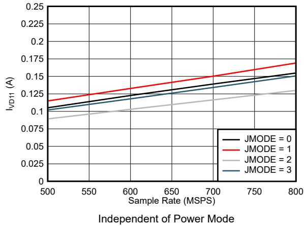
Figure 7-97. Single Channel, I_{VD11} vs F_S for JMODES 0 - 3
