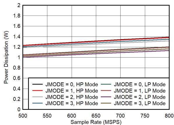
Figure 7-81. Dual Channel, Power Dissipation vs F_S for JMODES 0 - 3
