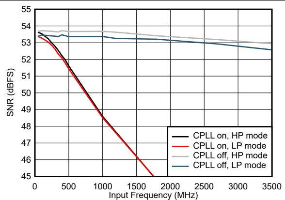
Figure 7-66. SNR vs Input Frequency and CPLL and Power Mode
