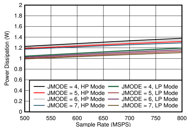
Figure 7-82. Dual Channel, Power Dissipation vs F_S for JMODES 4 - 7
