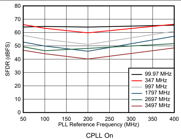
Figure 7-64. SFDR vs Reference Clock Frequency
