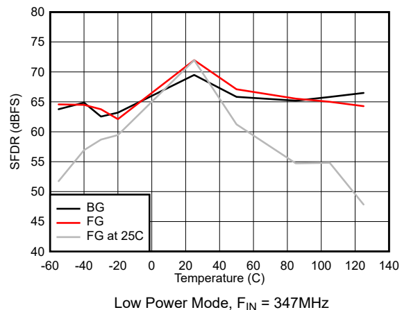
Figure 7-41. SFDR vs Temperature
