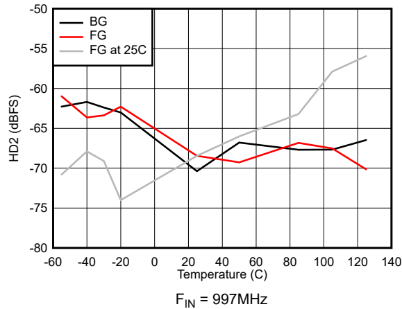
Figure 7-37. HD2 vs Temperature
