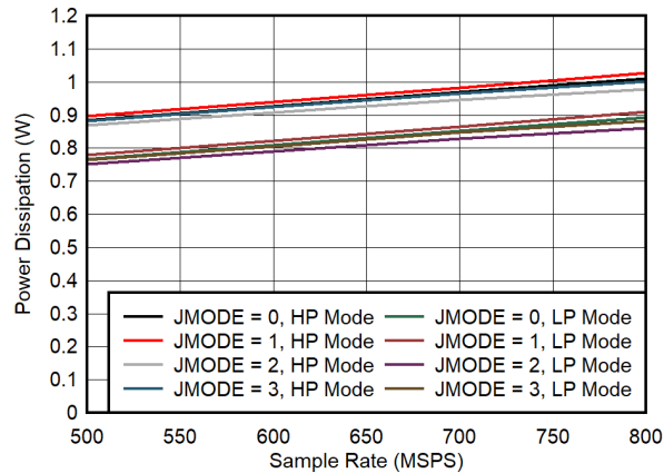
Figure 7-91. Single Channel, Power Dissipation vs F_S for JMODES 0 - 3
