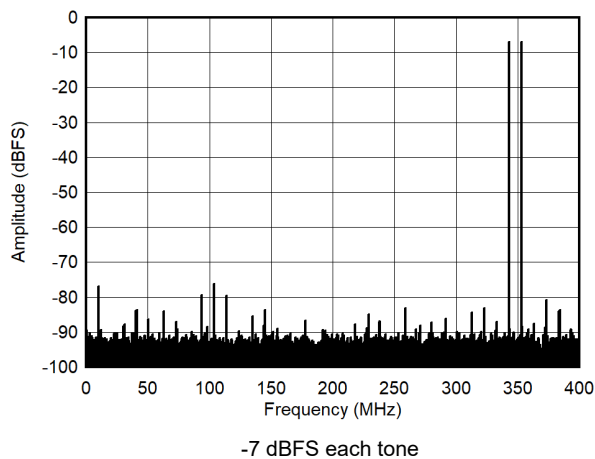
Figure 7-51. Dual Tone FFT at 348 MHz
