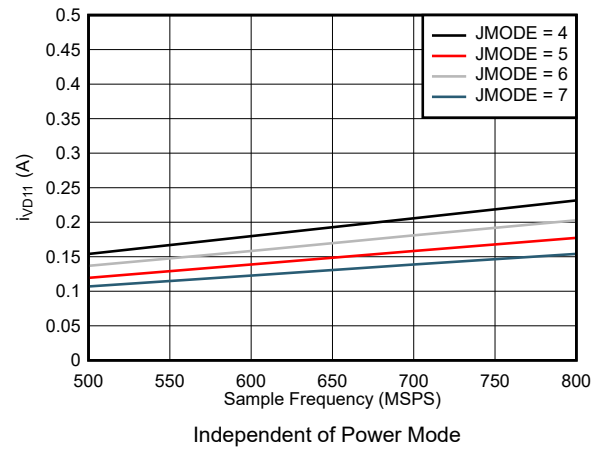
Figure 7-88. Dual Channel, I_{VD11} vs F_S for JMODES 4 - 7
