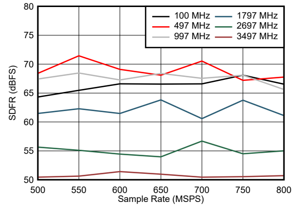
Figure 7-20. SFDR vs Sample Rate
