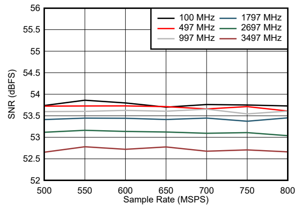
Figure 7-21. SNR vs Sample Rate
