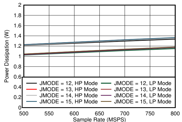
Figure 7-84. Dual Channel, Power Dissipation vs F_S for JMODES 12 - 15
