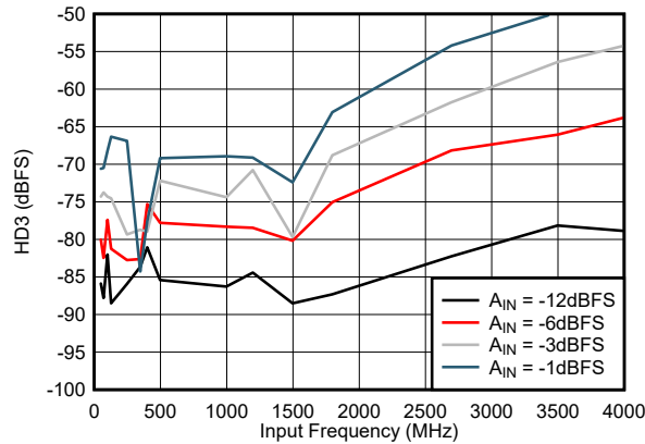
Figure 7-19. HD3 vs Input Frequency
