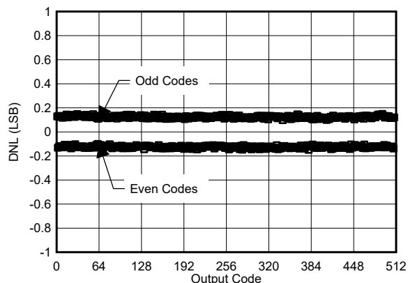
Figure 7-1. DNL vs Code
