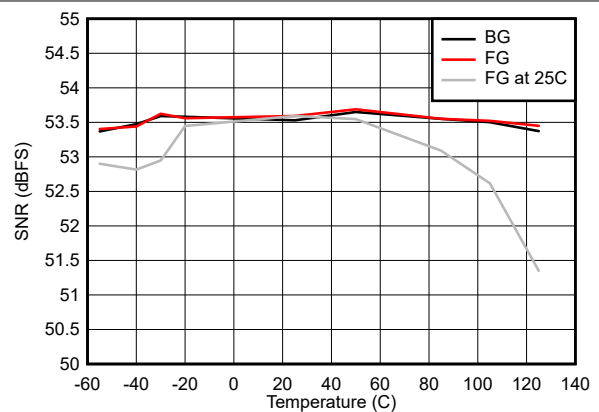
Figure 7-34. SNR vs Temperature
