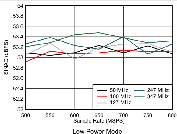
Figure 7-26. SINAD vs Sample Rate
