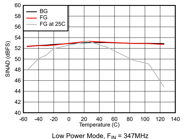
Figure 7-42. SINAD vs Temperature
