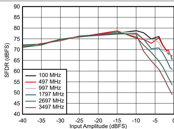
Figure 7-28. SFDR vs Input Amplitude
