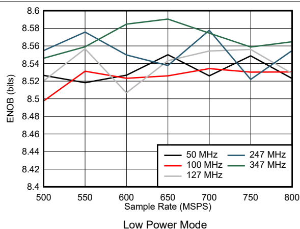
Figure 7-27. ENOB vs Sample Rate
