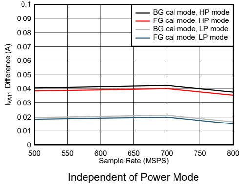
Figure 7-109. Single Channel, I_{VA11} Change with Calibration Mode
