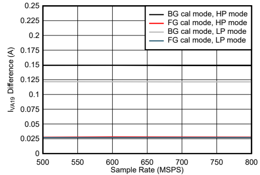
Figure 7-104. Quad Channel, I_{VA19} Change with Calibration Mode
