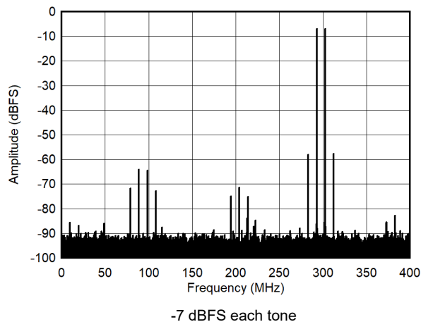
Figure 7-54. Dual Tone FFT at 2698 MHz
