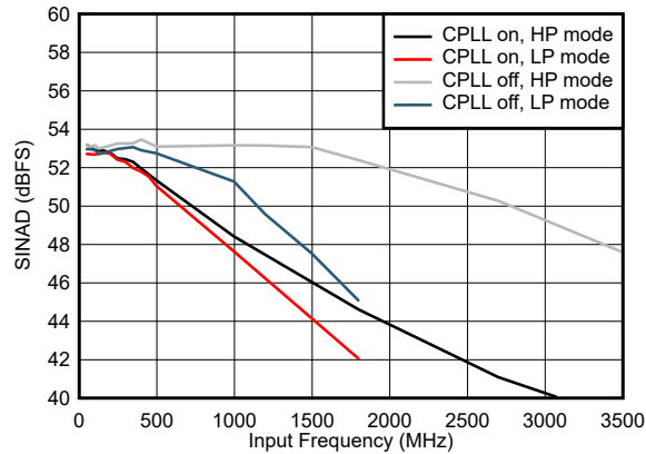
Figure 7-67. SINAD vs Input Frequency and CPLL and Power Mode
