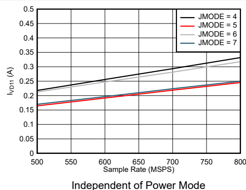
Figure 7-78. Quad Channel, I_{VD11} vs F_S for JMODES 4 - 7
