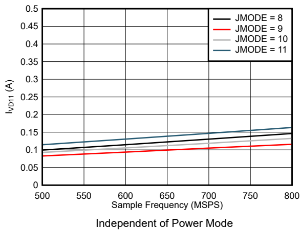
Figure 7-99. Single Channel, I_{VD11} vs F_S for JMODES 8 - 11
