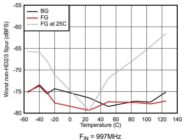
Figure 7-39. Worst non-HD2/3 Spur vs Temperature
