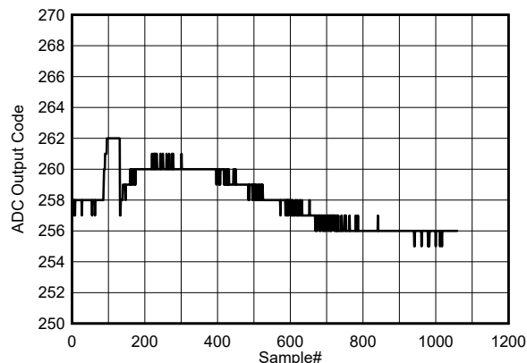
Figure 7-116. Background Core Transition (DC midscale input)
