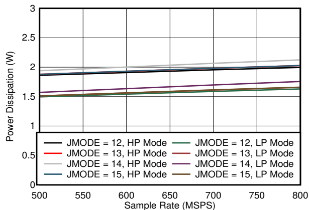
Figure 7-74. Quad Channel, Power Dissipation vs F_S for JMODES 12 - 15
