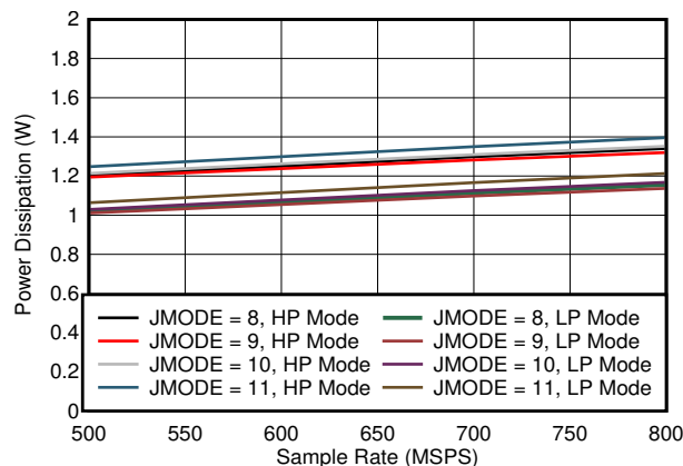
Figure 7-83. Dual Channel, Power Dissipation vs F_S for JMODES 8 - 11
