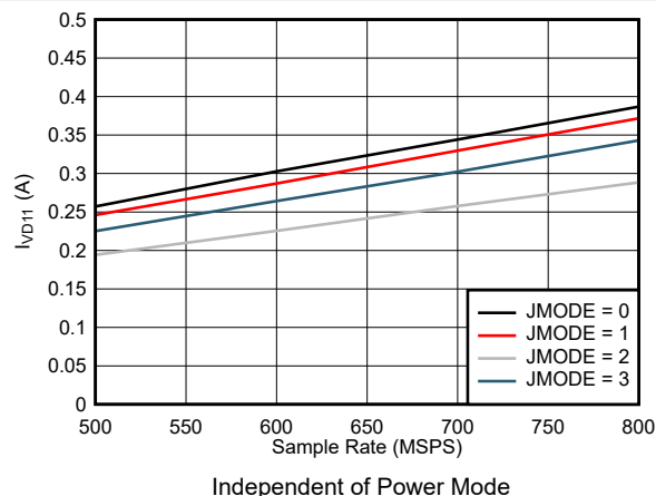
Figure 7-77. Quad Channel, I_{VD11} vs F_S for JMODES 0 - 3
