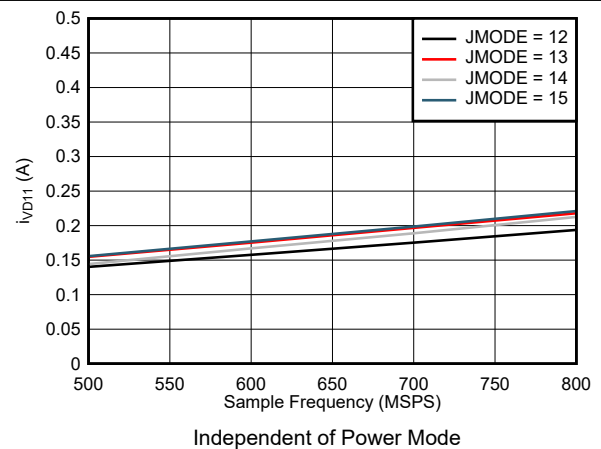
Figure 7-90. Dual Channel, I_{VD11} vs F_S for JMODES 12 - 15
