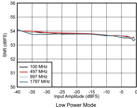
Figure 7-31. SNR vs Input Amplitude
