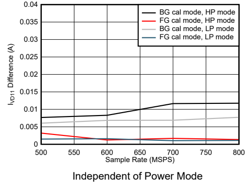
Figure 7-110. Quad Channel, I_{VD11} Change with Calibration Mode
