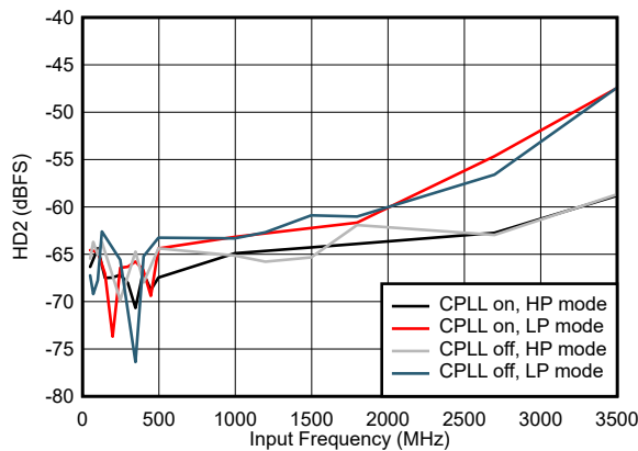
Figure 7-69. HD2 vs Input Frequency and CPLL and Power Mode
