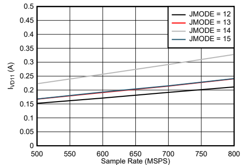
Figure 7-80. Quad Channel, I_{VD11} vs F_S for JMODES 12 - 15
