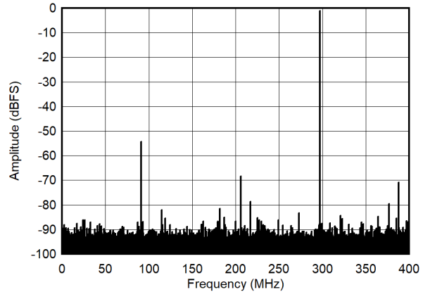
Figure 7-8. Single Tone FFT at 2697 MHz and -1dBFS
