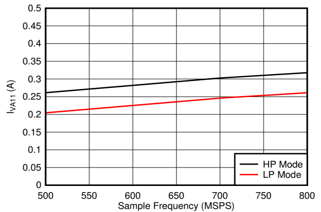
Figure 7-96. Single Channel, I_{VA11} vs F_S
