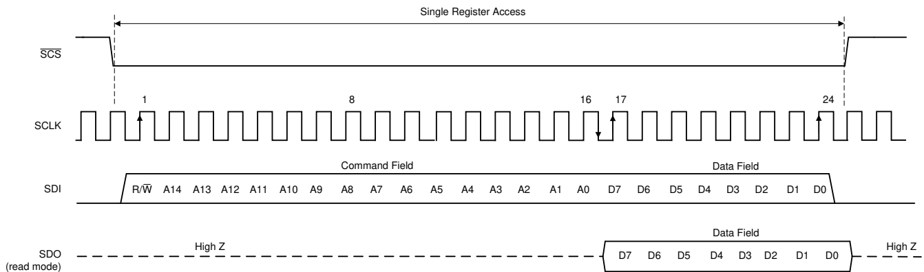
Figure 8-18. Serial Interface Protocol: Single Read/Write
