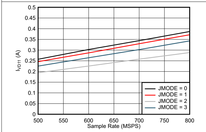
Figure 7-77. Quad Channel, I_{VD11} vs F_S for JMODES 0 - 3 Independent of Power Mode
