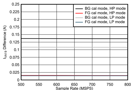
Figure 7-104. Quad Channel, I_{VA19} Change with Calibration Mode
