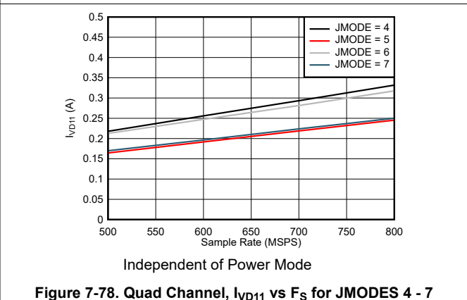
Figure 7-78. Quad Channel, I_{VD11} vs F_S for JMODES 4 - 7 Independent of Power Mode
