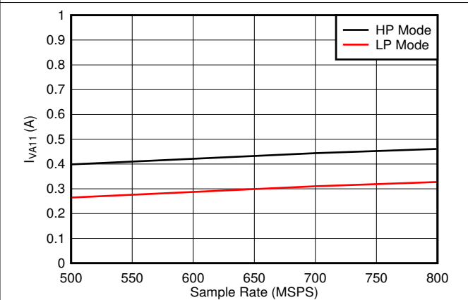
Figure 7-76. Quad Channel, I_{VA11} vs F_S Independent of JMODE
