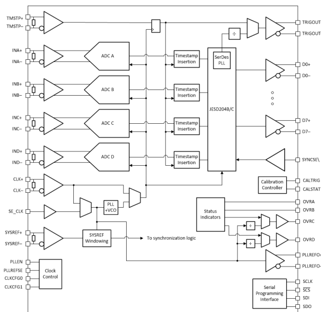
Quad Channel Block Diagram
