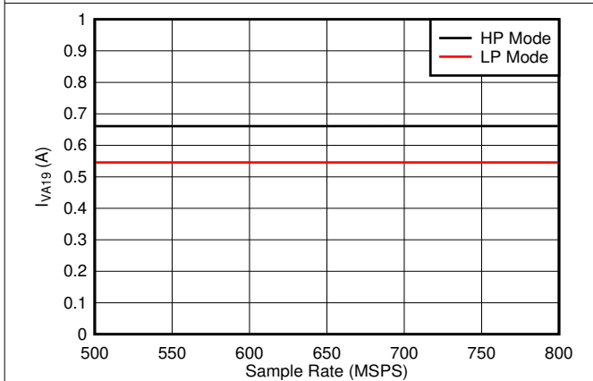
Figure 7-75. Quad Channel, I_{VA19} vs F_S Independent of JMODE
