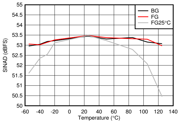
Low Power Mode, F_{IN} = 347 \text{ MHz} , FG25°C means calibration at 25°C and held across temperature
