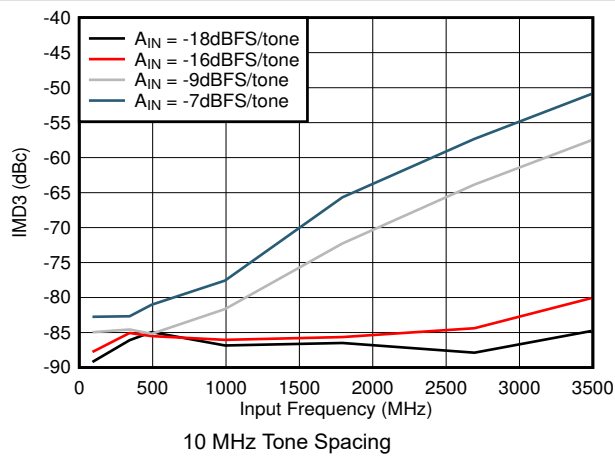
Figure 7-57. IMD3 vs Input Frequency
