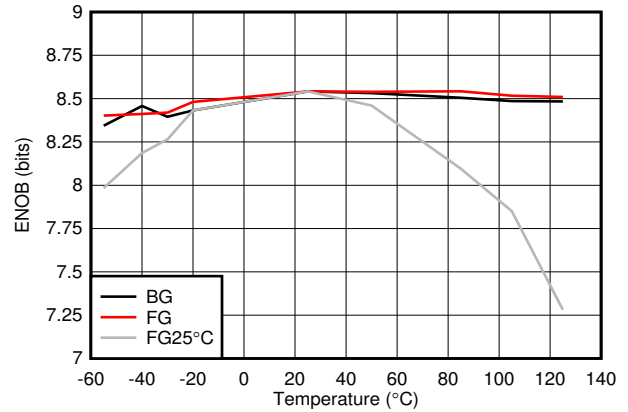
F_{IN} = 997 \text{ MHz} , FG25°C means calibration at 25°C and held across temperature
