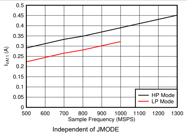
Figure 7-96. Dual Channel, I_{VA11} vs FS
