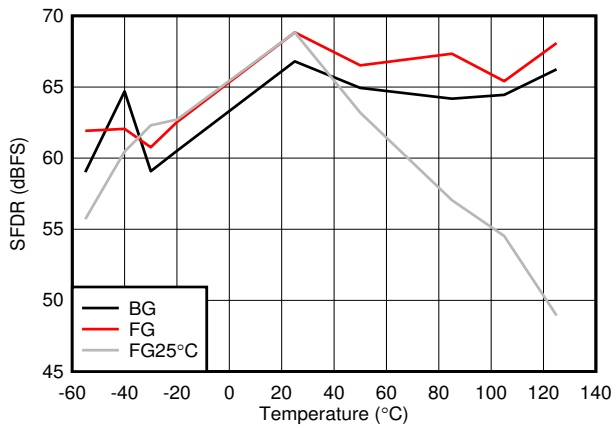
F_{IN} = 997 \text{ MHz} , FG25°C means calibration at 25°C and held across temperature
