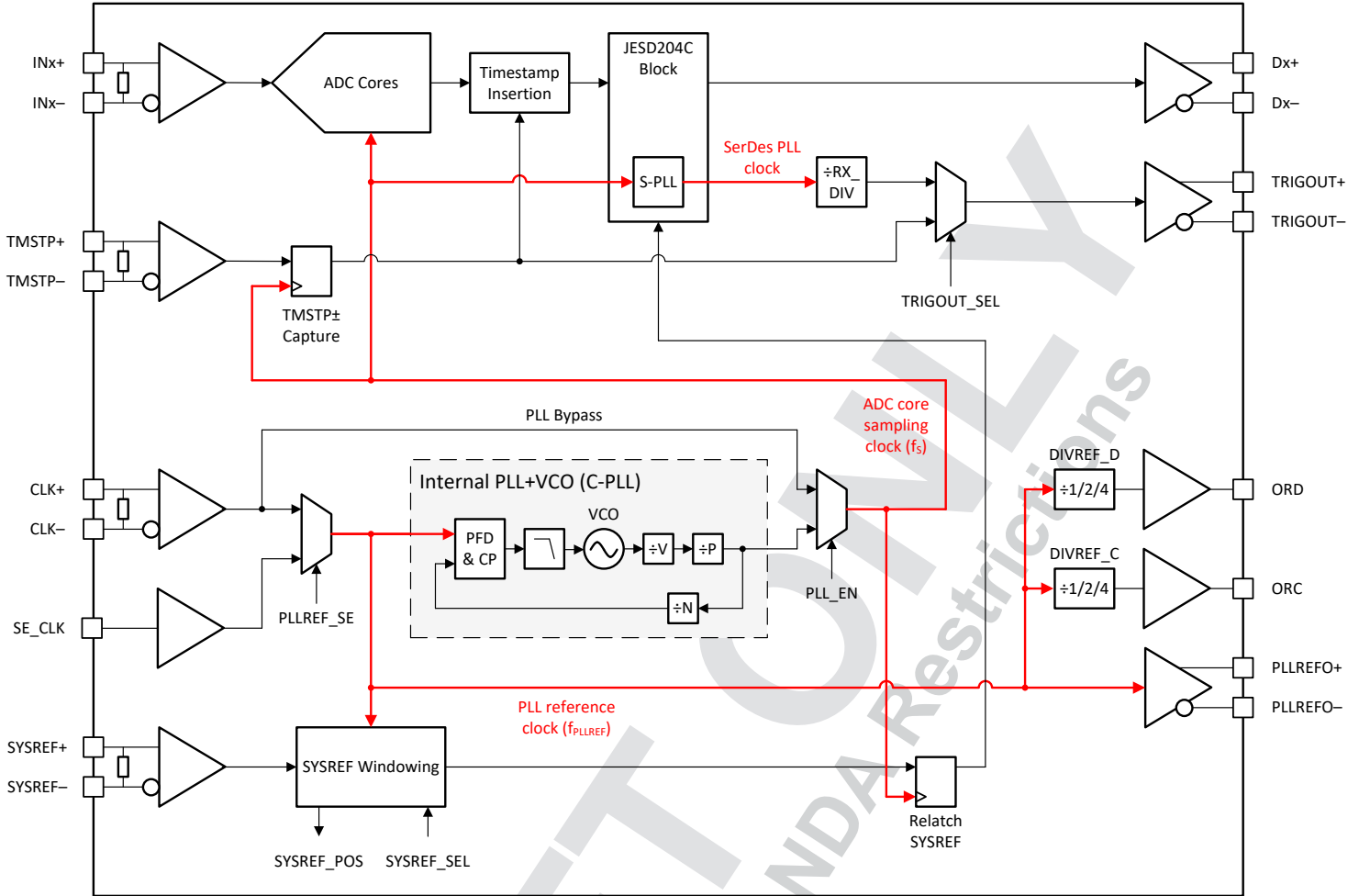
Figure 9-5. Clocking Subsystem
