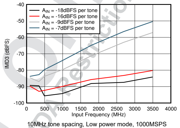
Figure 8-76. IMD3 vs F_{IN}
