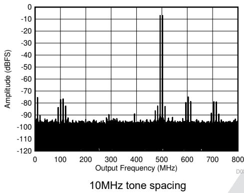
Figure 8-69. Two Tone FFT at 498MHz
