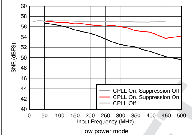
Figure 8-45. SNR vs F_{IN} and C-PLL modes
