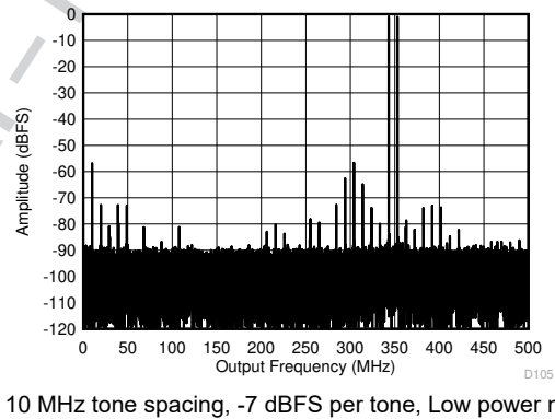
Figure 8-72. Two Tone FFT at 348 MHz
