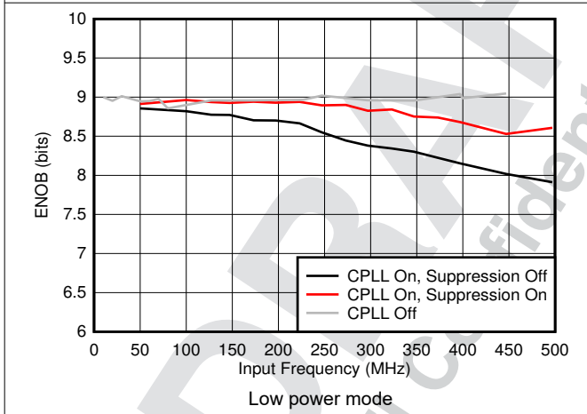
Figure 8-47. ENOB vs F_{IN} and C-PLL modes
