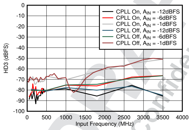
Figure 8-53. HD3 vs A_{IN} and C-PLL
