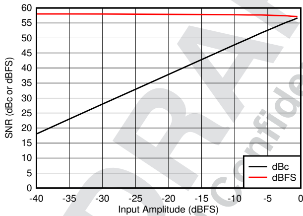
Figure 8-33. SNR vs A_{IN}
