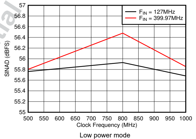
Figure 8-30. SINAD vs Sample Rate
