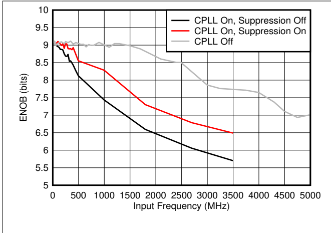
Figure 8-43. ENOB vs F_{IN} and C-PLL modes
