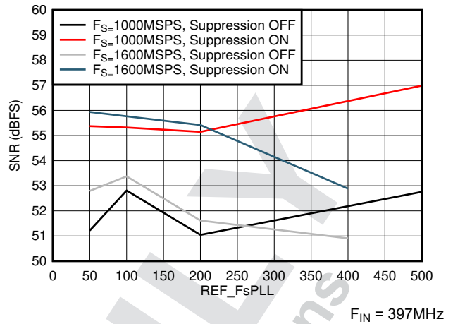
Figure 8-38. SNR vs F REF and Suppression
