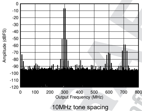
Figure 8-71. Two Tone FFT at 3498MHz
