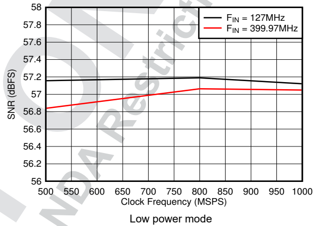
Figure 8-28. SNR vs Sample Rate
