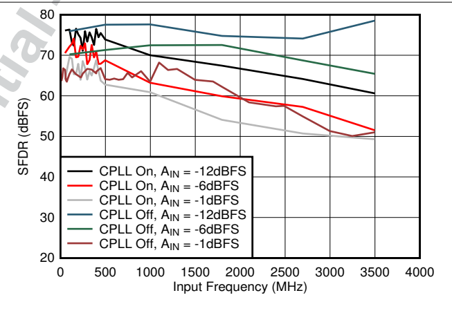
Figure 8-48. SFDR vs A_{IN} and C-PLL
