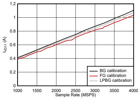
Figure 7-118. DES Mode: I_{VD11} vs Sample Rate JMODE = 1
