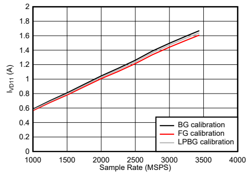
Figure 7-119. DES Mode: I_{VD11} vs Sample Rate JMODE = 21
