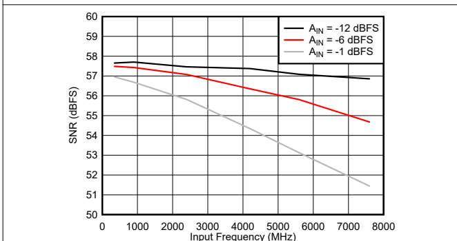
Figure 7-77. DES Mode: SNR vs Input Frequency
