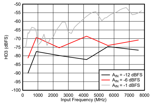
Figure 7-86. Dual Channel Mode: HD3 vs Input Frequency
