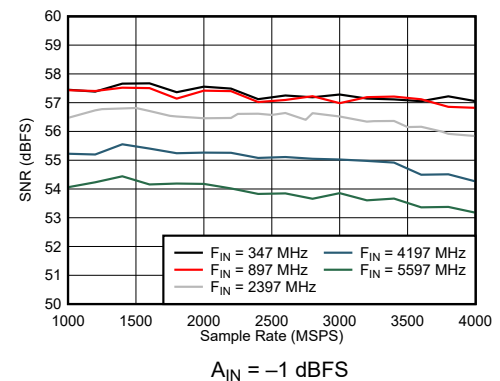
Figure 7-42. Dual Channel Mode: SNR vs Sample Rate and Input Frequency
