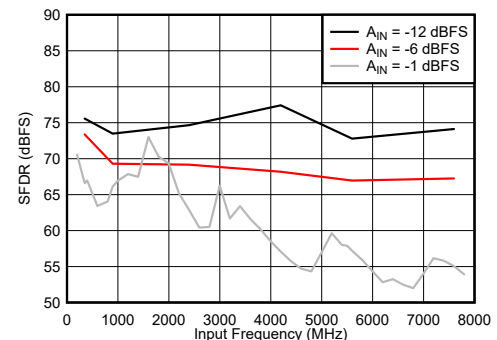
Figure 7-84. Dual Channel Mode: SFDR vs Input Frequency
