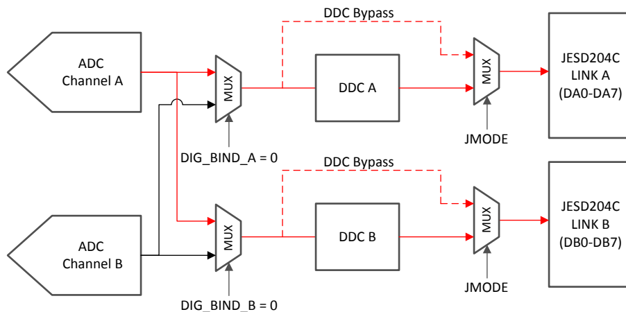
Figure 8-24. Dual DDC Mode or Redundant Data Mode for Channel A
