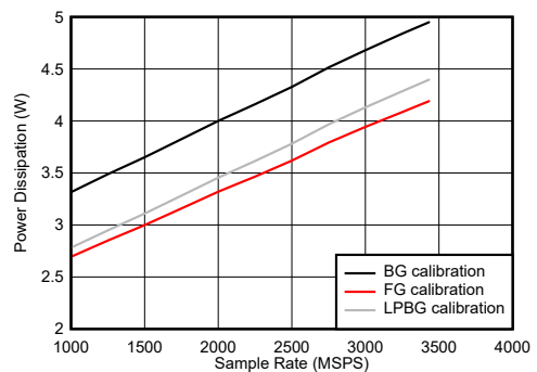
Figure 7-123. DES Mode: Power Dissipation vs Sample Rate JMODE = 21
