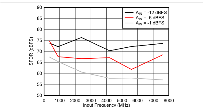
Figure 7-78. DES Mode: SFDR vs Input Frequency
