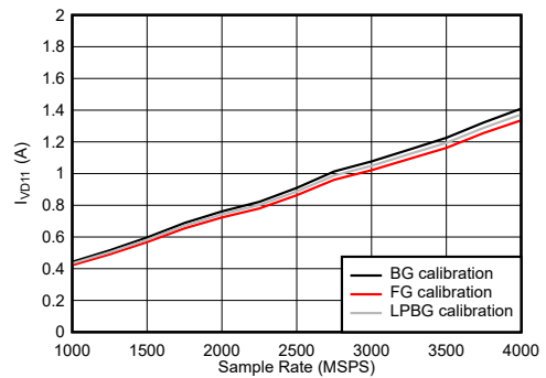
Figure 7-121. DES Mode: I_{VD11} vs Sample Rate JMODE = 61
