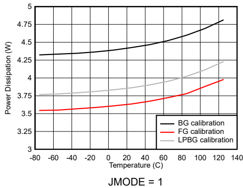
Figure 7-136. DES Mode: Power Dissipation vs Temperature
