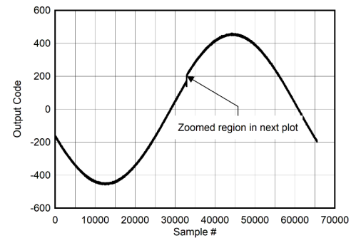
Figure 7-139. Background Calibration Core Transition (AC Signal)
