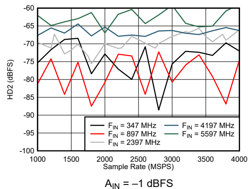
Figure 7-48. Dual Channel Mode: HD2 vs Sample Rate and Input Frequency
