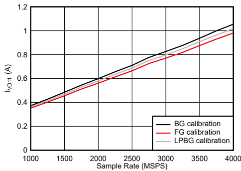
Figure 7-120. DES Mode: I_{VD11} vs Sample Rate JMODE = 30
