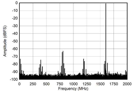
Figure 7-20. Dual Channel Mode: Single Tone FFT at 2397 MHz
