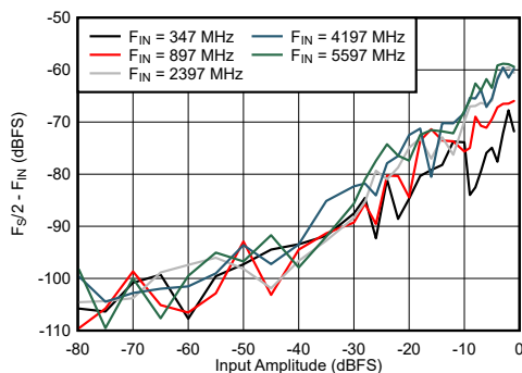
Figure 7-63. DES Mode: F_{S/2} - F_{\text{IN}} vs Input Amplitude and Frequency
