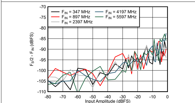
Figure 7-75. Dual Channel Mode: F_S/2 - F_{IN} vs Input Amplitude and Frequency
