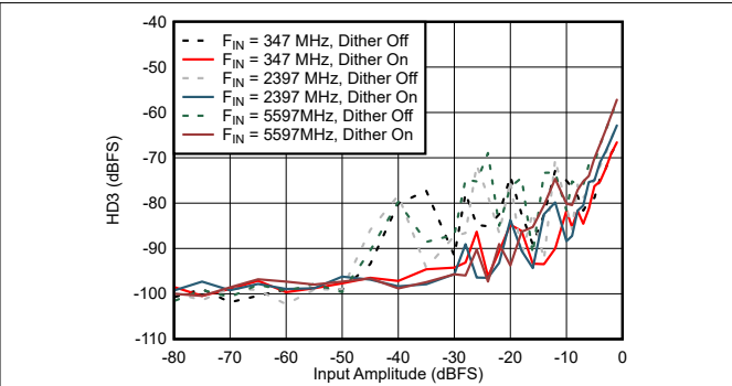
Figure 7-74. Dual Channel Mode: HD3 vs Input Amplitude and Dither
