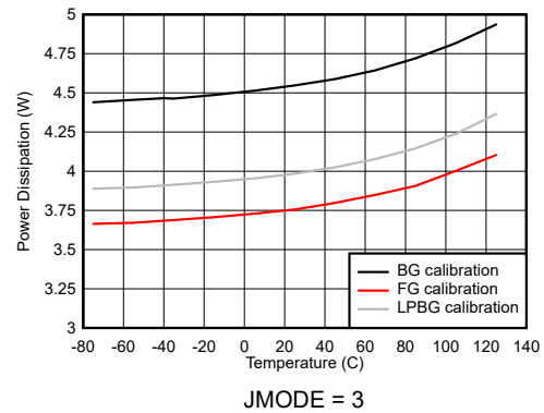
Figure 7-137. Dual Channel Mode: Power Dissipation vs Temperature
