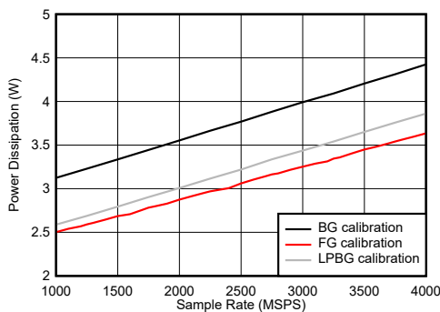
Figure 7-122. DES Mode: Power Dissipation vs Sample Rate JMODE = 1
