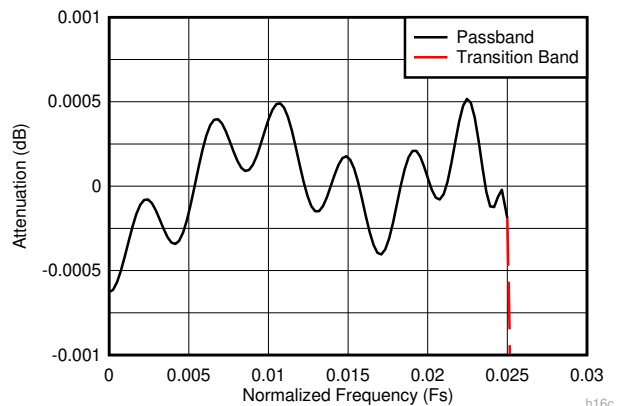
Figure 8-16. Decimate-by-16 Composite Zoomed Pass-Band Response
