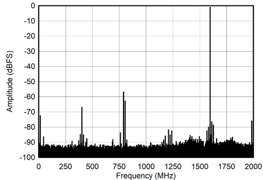
Figure 7-22. Dual Channel Mode: Single Tone FFT at 5597 MHz
