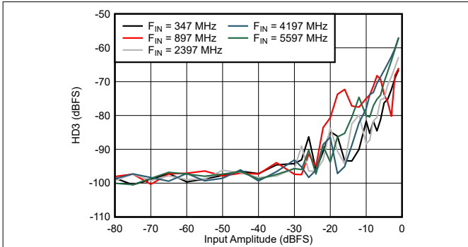
Figure 7-73. Dual Channel Mode: HD3 vs Input Amplitude and Frequency
