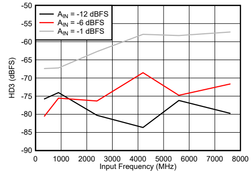
Figure 7-80. DES Mode: HD3 vs Input Frequency
