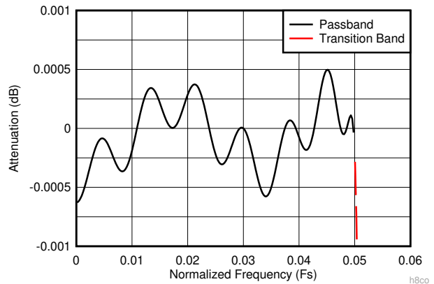
Figure 8-14. Decimate-by-8 Composite Zoomed Pass-Band Response
