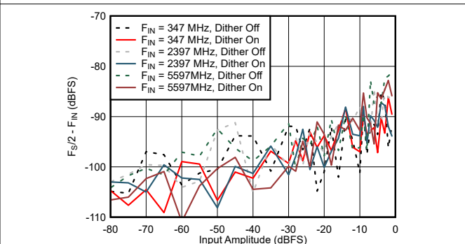
Figure 7-76. Dual Channel Mode: F_S/2 - F_{IN} vs Input Amplitude and Dither
