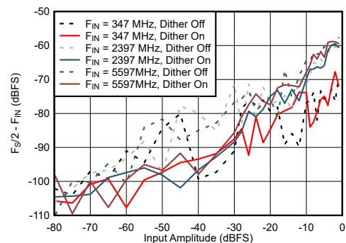
Figure 7-64. DES Mode: F_{S/2} - F_{\text{IN}} vs Input Amplitude and Dither
