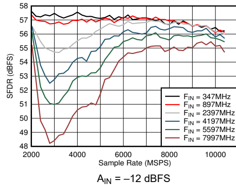
Figure 6-34. DES Mode: SFDR vs Sample Rate and Input Frequency A_{IN} = -12\text{ dBFS}
