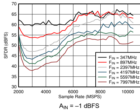
Figure 6-32. DES Mode: SFDR vs Sample Rate and Input Frequency A_{IN} = -1\text{ dBFS}
