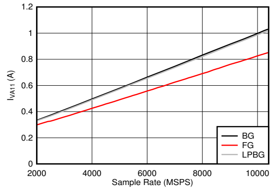
Figure 6-122. DES Mode: I_{VA11} vs Sample Rate
