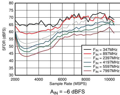
Figure 6-33. DES Mode: SFDR vs Sample Rate and Input Frequency A_{IN} = -6\text{ dBFS}
