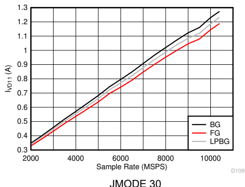
Figure 6-125. DES Mode: I_{VD11} vs Sample Rate
