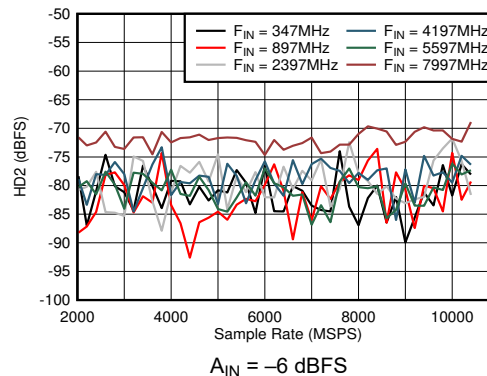
Figure 6-36. DES Mode: HD2 vs Sample Rate and Input Frequency A_{IN} = -6\text{ dBFS}
