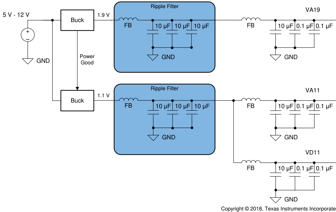
Figure 8-4. Switcher-Only Approach Example
