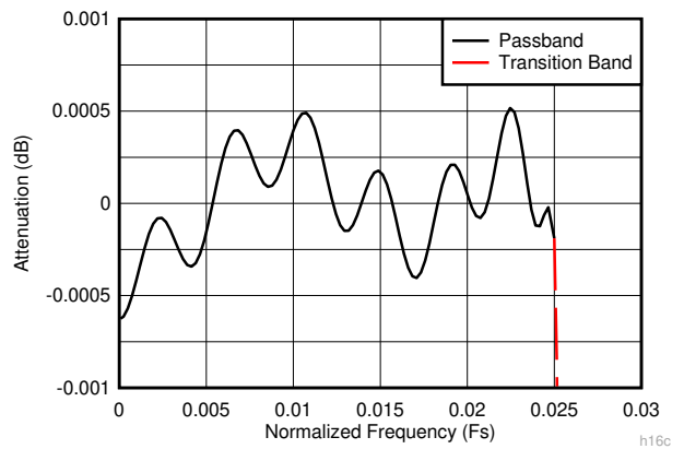
Figure 7-16. Decimate-by-16 Composite Zoomed Pass-Band Response h16c
