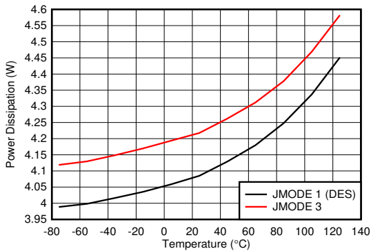
Figure 6-141. Power Dissipation vs Temperature
