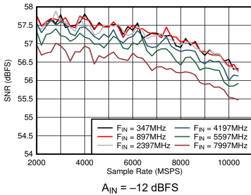
Figure 6-31. DES Mode: SNR vs Sample Rate and Input Frequency A_{IN} = -12\text{ dBFS}
