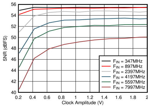
Figure 6-81. DES Mode: SNR vs Clock Amplitude
