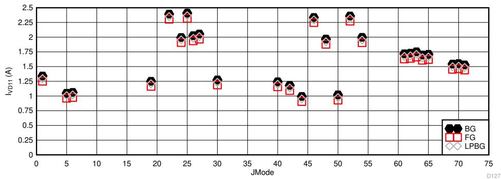
Figure 6-110. DES Mode: I_{VA11} vs JMODE at 10.4GSPS
