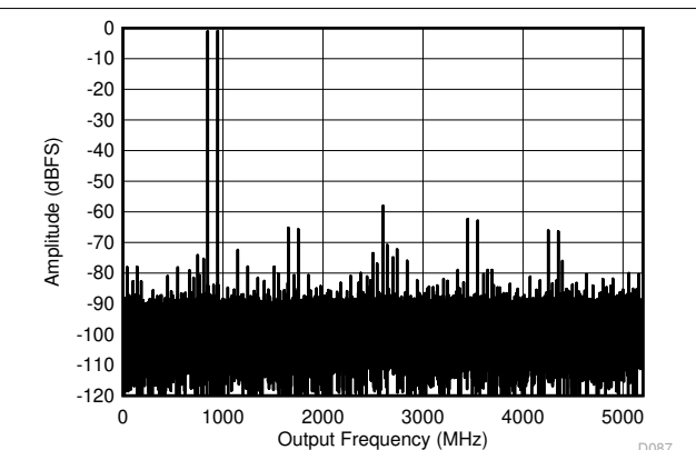
Figure 6-12. DES Mode: Two Tone FFT at 897 MHz
