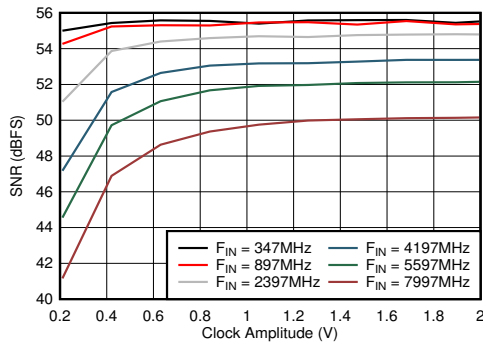
Figure 6-83. Dual Channel Mode: SNR vs Clock Amplitude
