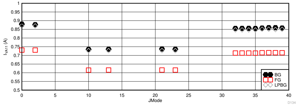
Figure 6-118. Other Modes with Lower Maximum F_S : I_{VA11} vs JMODE
