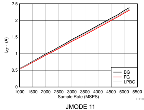
Figure 6-134. Dual Channel Mode: I_{VD11} vs Sample Rate
