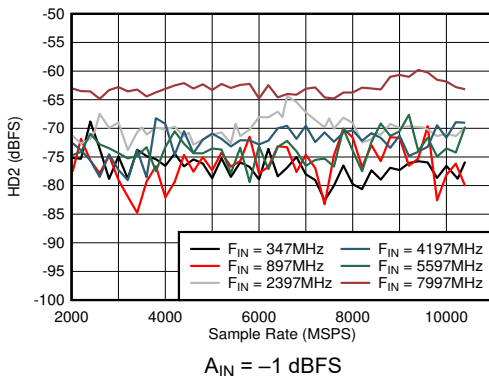
Figure 6-35. DES Mode: HD2 vs Sample Rate and Input Frequency A_{IN} = -1\text{ dBFS}
