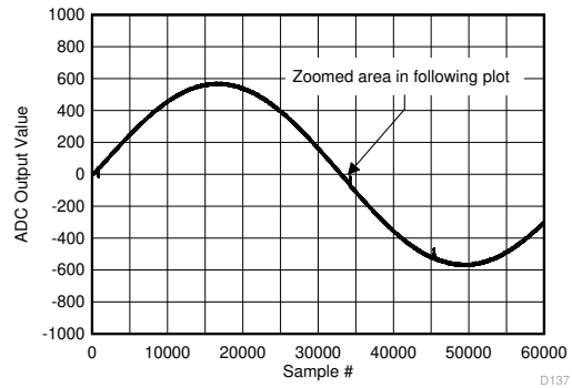
Figure 6-142. Background Calibration Core Transition (AC Signal)
