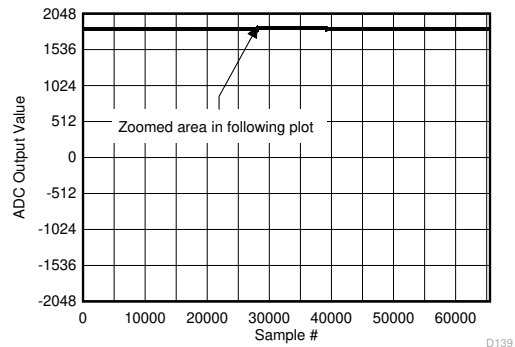
Figure 6-144. Background Calibration Core Transition (DC Signal)
