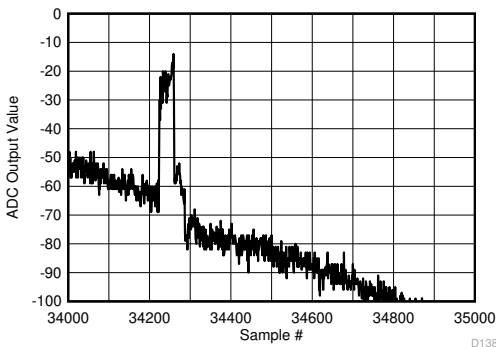
Figure 6-143. Background Calibration Core Transition (AC Signal - zoomed)
