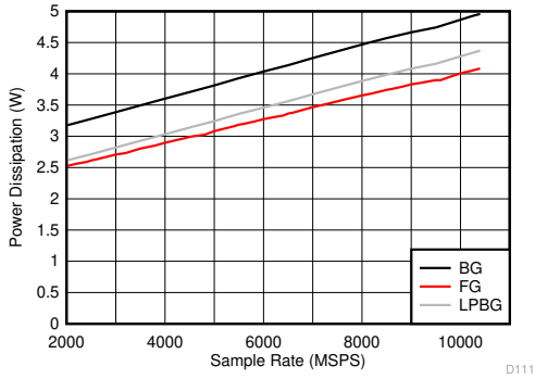
Figure 6-127. DES Mode: Power Dissipation vs Sample Rate
