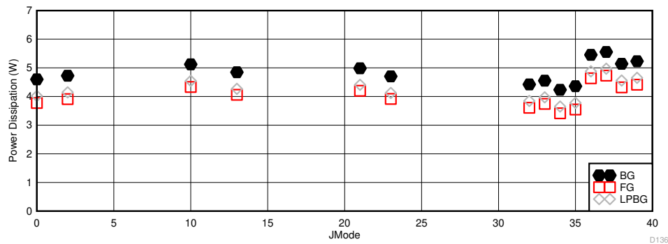
Figure 6-119. Other Modes with Lower Maximum F_S : I_{VD11} vs JMODE
