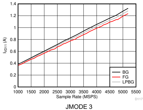
Figure 6-133. Dual Channel Mode: I_{VD11} vs Sample Rate
