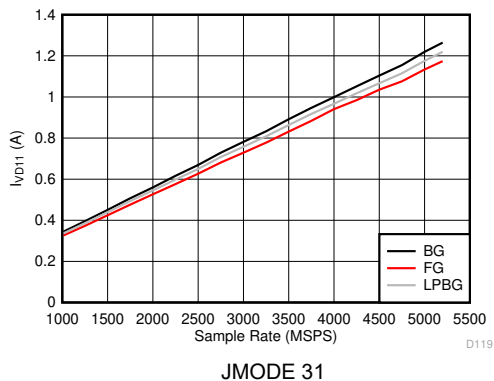
Figure 6-135. Dual Channel Mode: I_{VD11} vs Sample Rate
