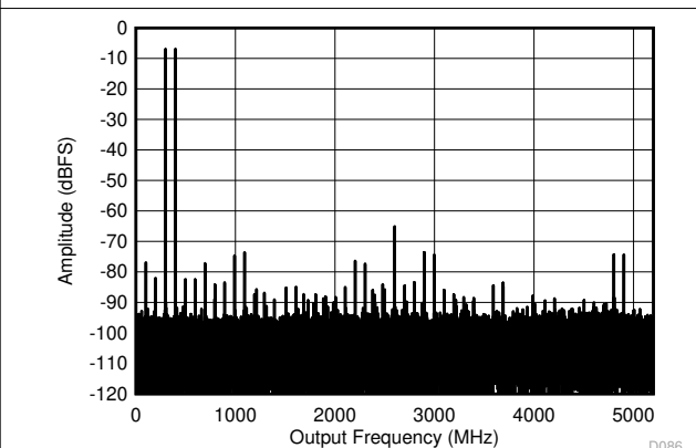
Figure 6-11. DES Mode: Two Tone FFT at 347 MHz
