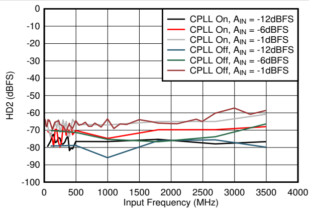
Figure 7-52. HD2 vs A_{IN} and C-PLL
