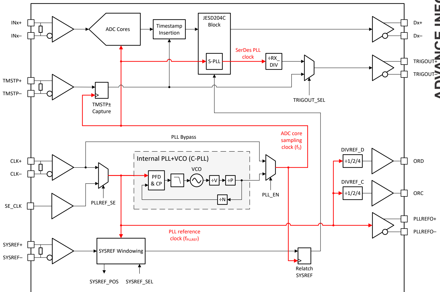
Figure 8-3. Clocking Subsystem
