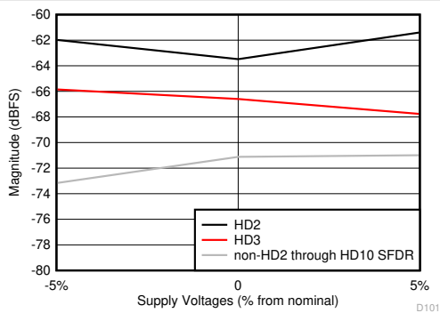
All supplies changed together, high power mode Figure 7-61. HD2, HD3 and Worst non-HD Spur vs Supply Voltage
