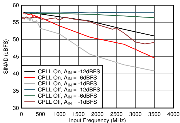
Figure 7-50. SINAD vs A_{IN} and C-PLL
