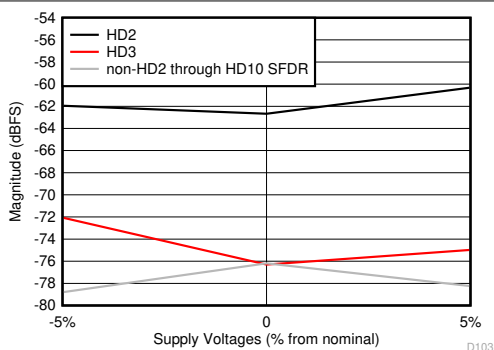
All supplies changed together, low power mode, F_S = 1000 MSPS Figure 7-63. HD2, HD3 and Worst non-HD Spur vs Supply Voltage
