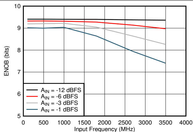
Figure 7-20. ENOB vs Input Frequency
