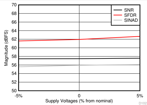
All supplies changed together, low power mode, F_S = 1000 MSPS Figure 7-62. SNR, SFDR and SINAD vs Supply Voltages
