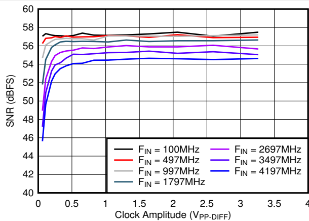
Figure 7-37. SNR vs A_{CLK}
