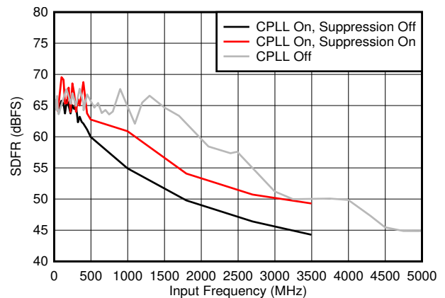
Figure 7-40. SFDR vs F_{IN} and C-PLL modes
