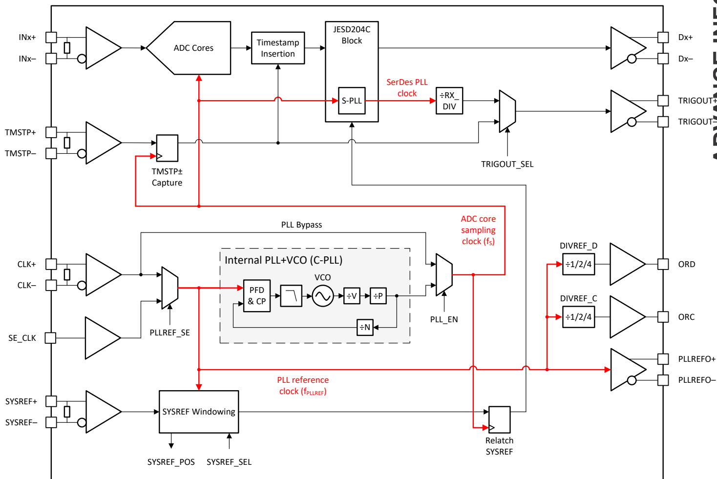
Figure 8-3. Clocking Subsystem
