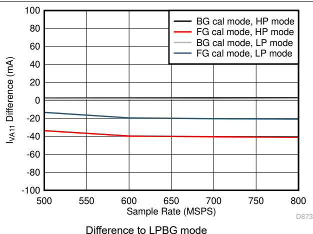
Figure 7-113. Single Channel, I_{VA11} vs F_S over Modes
