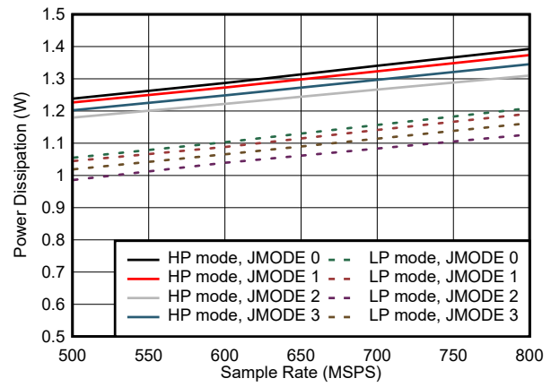
Figure 7-88. Dual Channel, Power Dissipation vs F_S for JMODES 0 - 3
