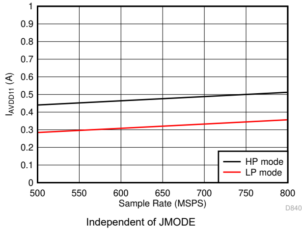
Figure 7-79. Quad Channel, I_{AVD11} vs F_S
