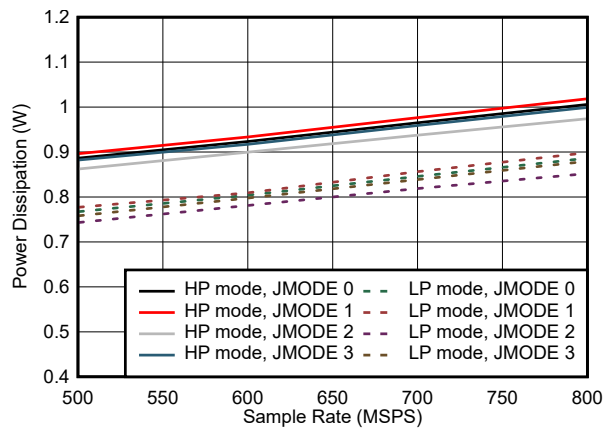
Figure 7-101. Dual Channel, Power Dissipation vs F_S for JMODES 0 - 3
