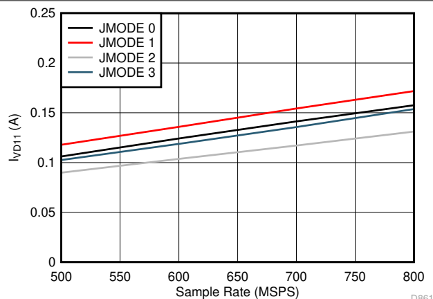
Figure 7-107. Single Channel, I_{VD11} vs F_S for JMODES 0 - 3
