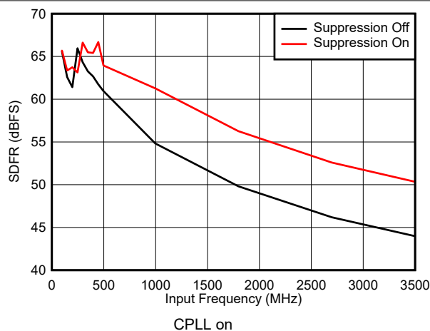
Figure 7-35. SFDR vs Input Frequency and Suppression
