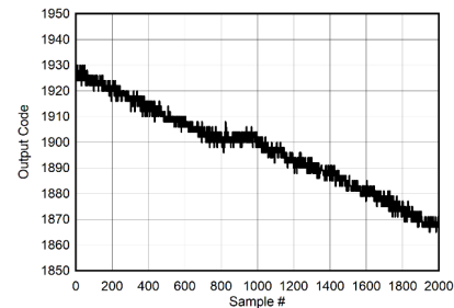
Figure 7-116. Background Calibration Core Transition (voltage offset)
