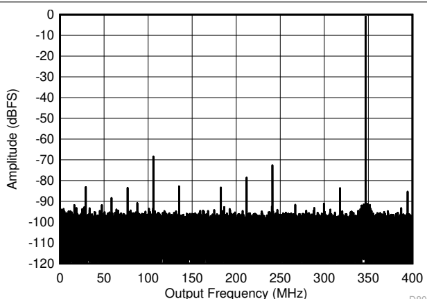
Figure 7-6. Single Tone FFT at 347 MHz and -1dBFS
