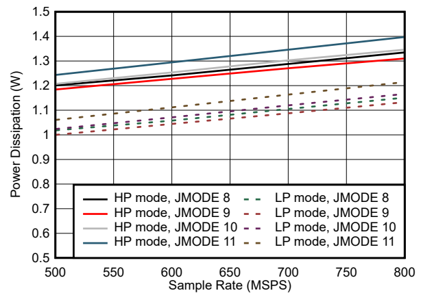
Figure 7-90. Dual Channel, Power Dissipation vs F_S for JMODES 8 - 11
