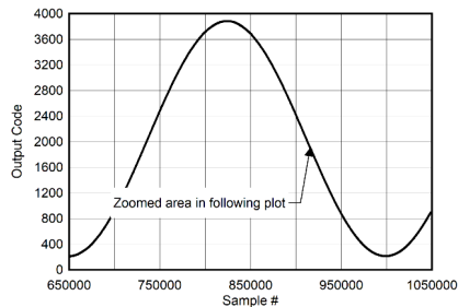
Figure 7-115. Background Calibration Core Transition (midscale)
