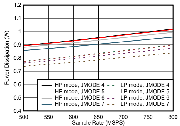
Figure 7-102. Single Channel, Power Dissipation vs F_S for JMODES 4 - 7
