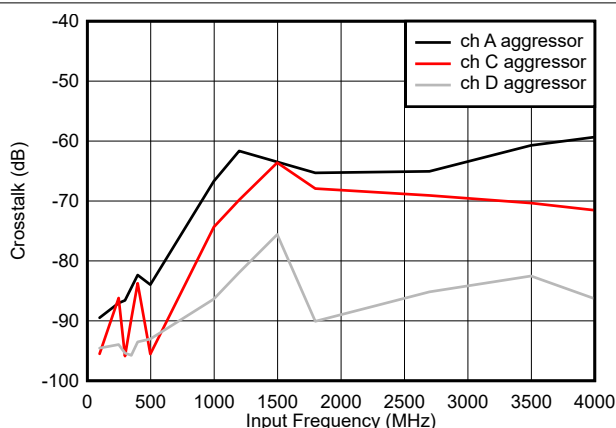
Figure 7-5. Crosstalk vs Input Frequency, Channel B victim
