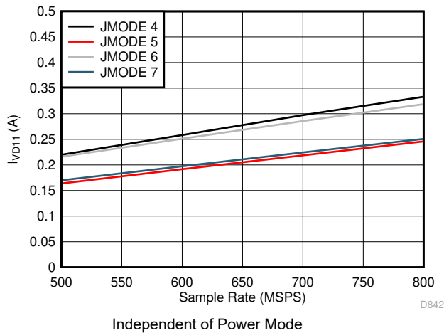
Figure 7-81. Quad Channel, I_{VD11} vs F_S for JMODES 4 - 7
