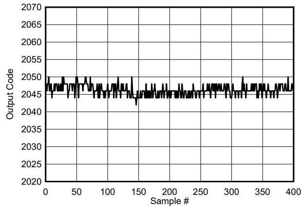
Figure 7-115. Background Calibration Core Transition (midscale)
