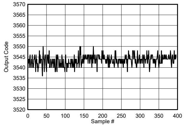
Figure 7-116. Background Calibration Core Transition (voltage offset)
