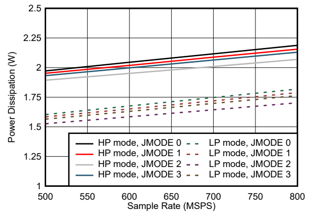
Figure 7-74. Quad Channel, Power Dissipation vs F_S for JMODES 0 - 3
