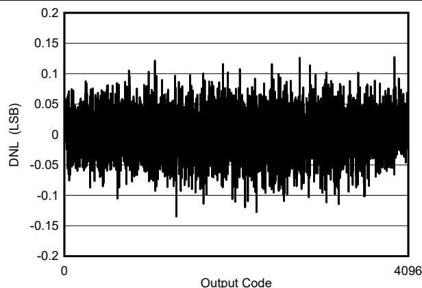
Figure 7-1. DNL vs Code
