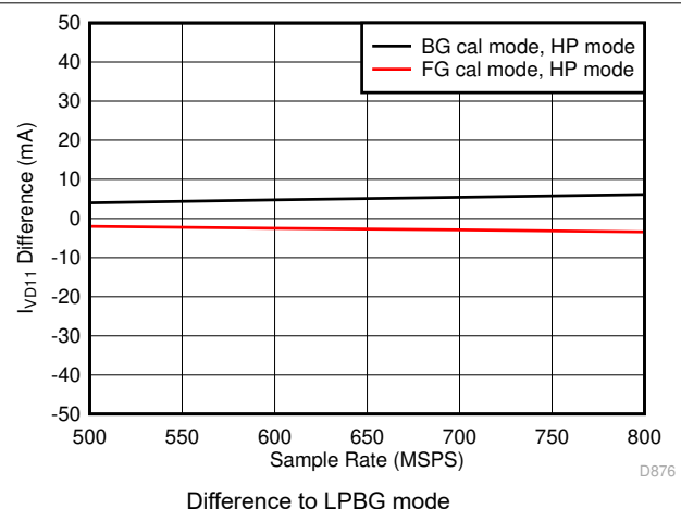
Figure 7-114. Single Channel, I_{VD11} vs F_S over Modes
