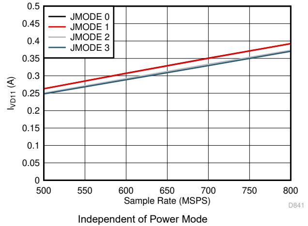
Figure 7-80. Quad Channel, I_{VD11} vs F_S for JMODES 0 - 3
