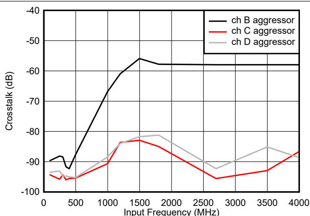
Figure 7-4. Crosstalk vs Input Frequency, Channel A victim
