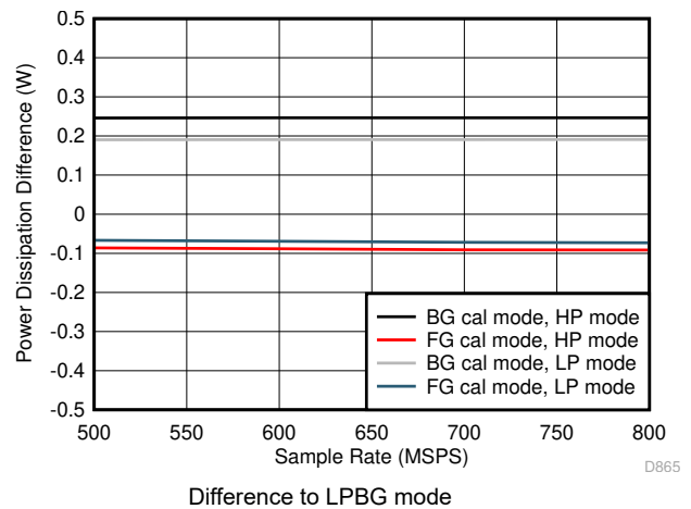
Figure 7-84. Quad Channel, Power Dissipation vs F_S over Modes
