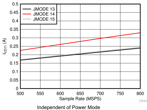
Figure 7-83. Quad Channel, I_{VD11} vs F_S for JMODES 13-15
