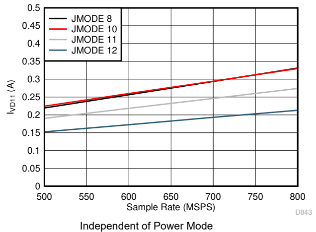
Figure 7-82. Quad Channel, I_{VD11} vs F_S for JMODES 8-12
