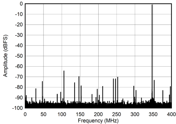
Figure 7-19. Single Tone FFT at 347 MHz and -1dBFS
