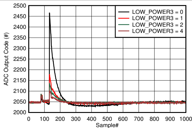
Figure 8-12. Background Calibration Core Transition In Low Power Mode
