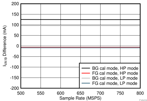
Figure 7-99. Dual Channel, I_{VA19} vs F_S over Modes
