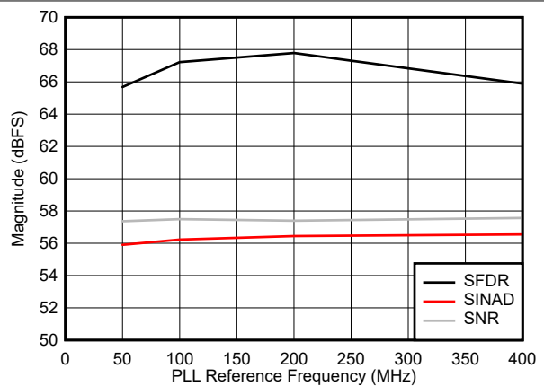
Figure 7-42. SNR, SFDR and SINAD vs Reference Frequency with PLL on
