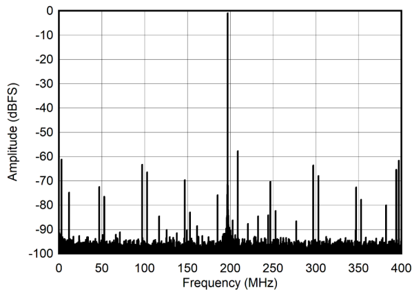
Figure 7-21. Single Tone FFT at 997 MHz and -1dBFS
