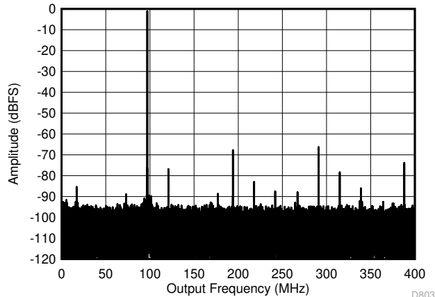
Figure 7-7. Single Tone FFT at 897 MHz and -1dBFS
