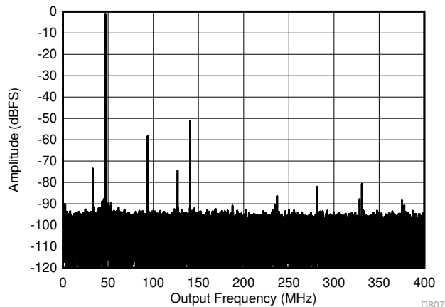
Figure 7-9. Single Tone FFT at 3247 MHz and -1dBFS
