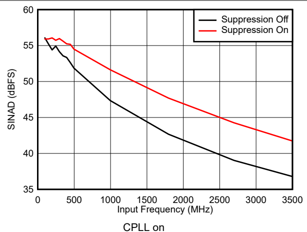
Figure 7-36. SINAD vs Input Frequency and Suppression
