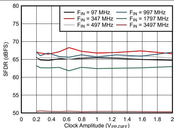
Figure 7-41. SFDR vs Clock Amplitude
