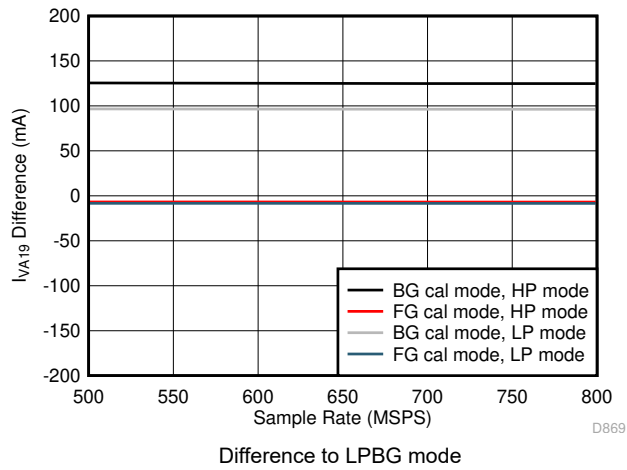
Figure 7-99. Dual Channel, I_{VA19} vs F_S over Modes
