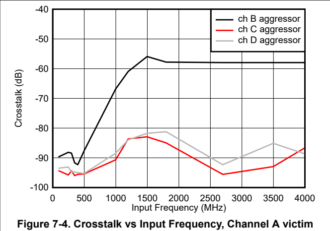
Figure 7-4. Crosstalk vs Input Frequency, Channel A victim
