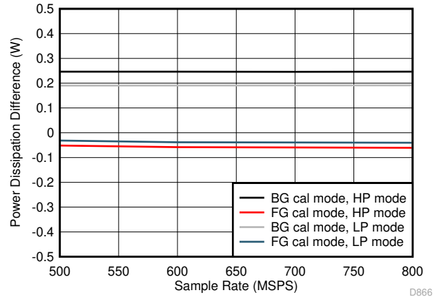
Figure 7-98. Dual Channel, Power Dissipation vs F_S over Modes
