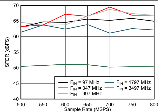
Figure 7-29. SFDR vs Sample Rate
