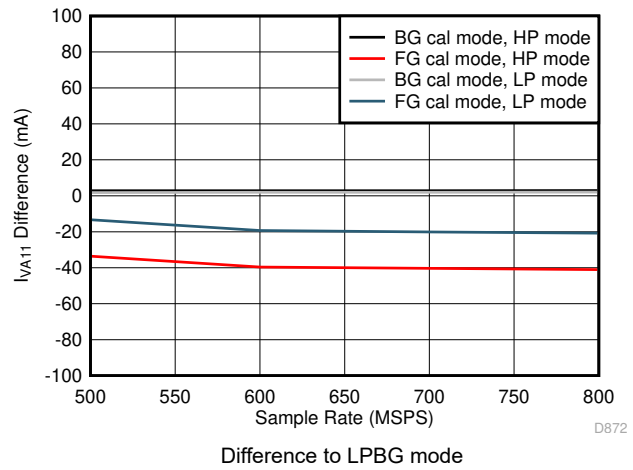
Figure 7-100. Dual Channel, I_{VA11} vs F_S over Modes
