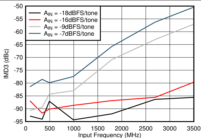
Figure 7-72. IMD3 vs Input Frequency
