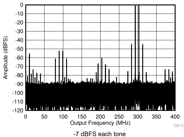
Figure 7-68. Two Tone FFT at 3498 MHz
