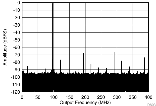
Figure 7-7. Single Tone FFT at 897 MHz and -1dBFS
