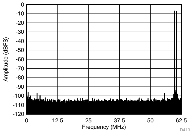
f_S = 125\text{ MSPS} , \text{IMD} = 96.2\text{ dBFS} , f_{IN1} = 185\text{ MHz} , f_{IN2} = 190\text{ MHz}
