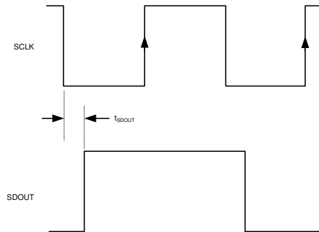
Figure 8-57. SDOUT Timing
