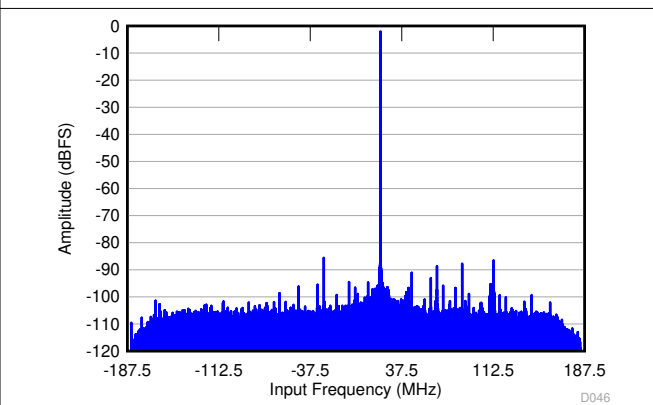
f_{IN} = 1.78 GHz, A_{IN} = -2 dBFS, f_S = 2949.12 MSPS, SNR = 62.6 dBFS, SFDR (includes IL) = 86 dBc
