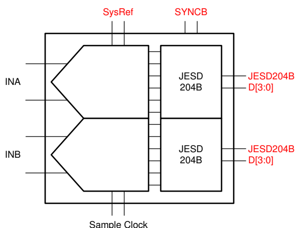
Figure 8-53. JESD Signal Overview
