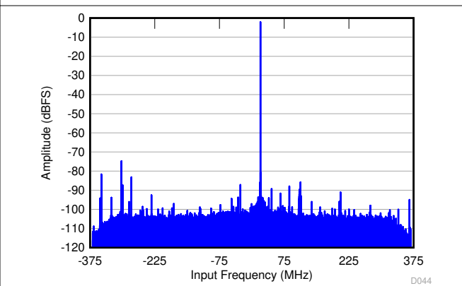
f_{IN} = 1.78 GHz, A_{IN} = -2 dBFS, f_S = 2949.12 MSPS, SNR = 60.6 dBFS, SFDR (includes IL) = 75 dBc
