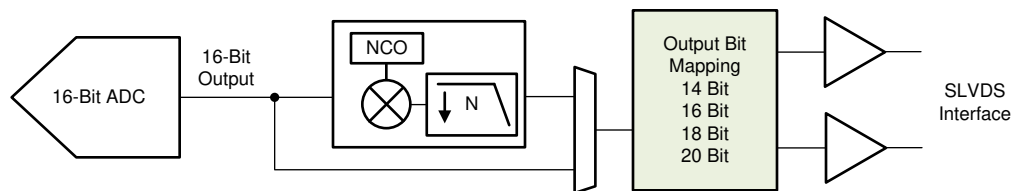
Figure 8-39. Interface output bit mapper
