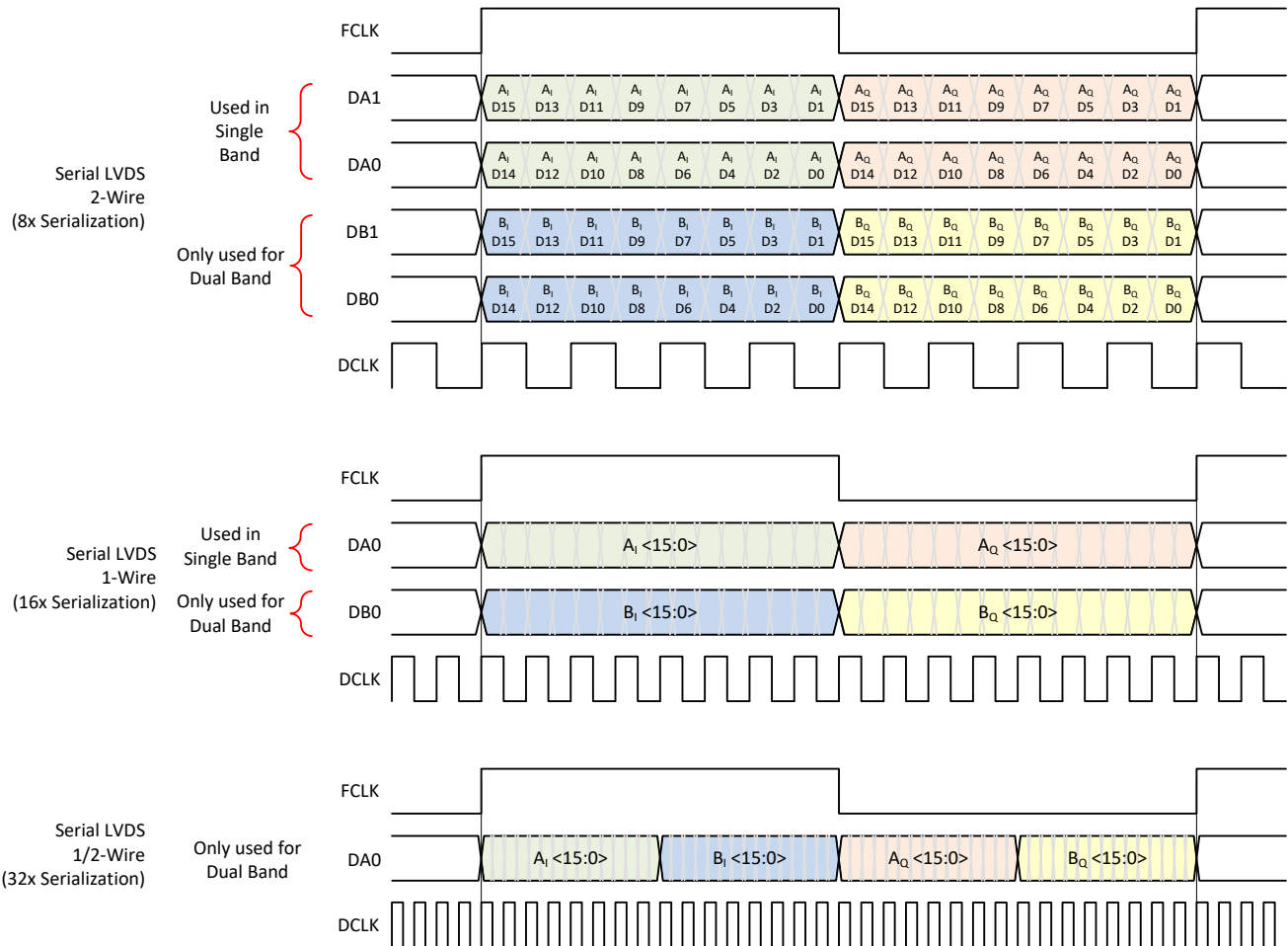
Figure 8-37. Output Data Format in Complex Decimation
