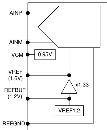
Figure 8-15. Different voltage reference options for ADC356x
