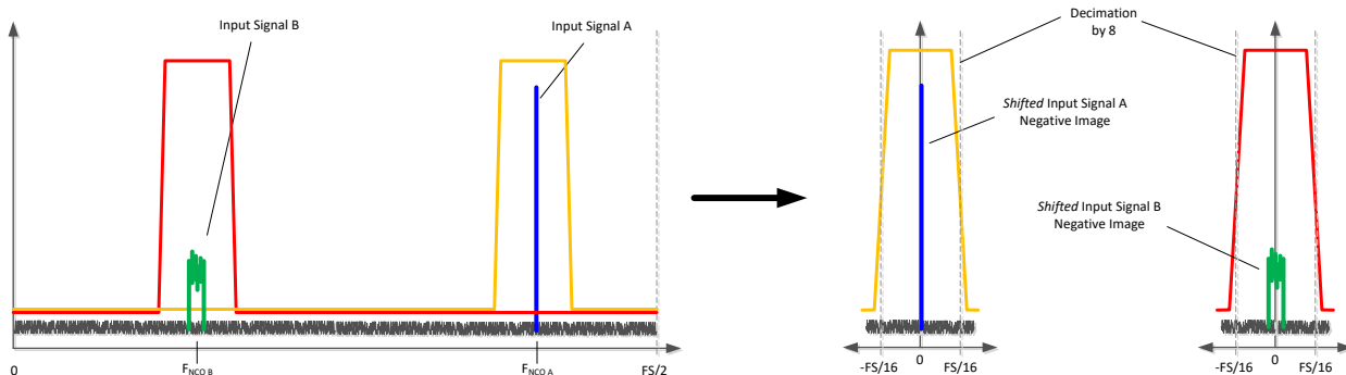
Figure 8-21. Complex Decimation (by 8) with dual band illustration
