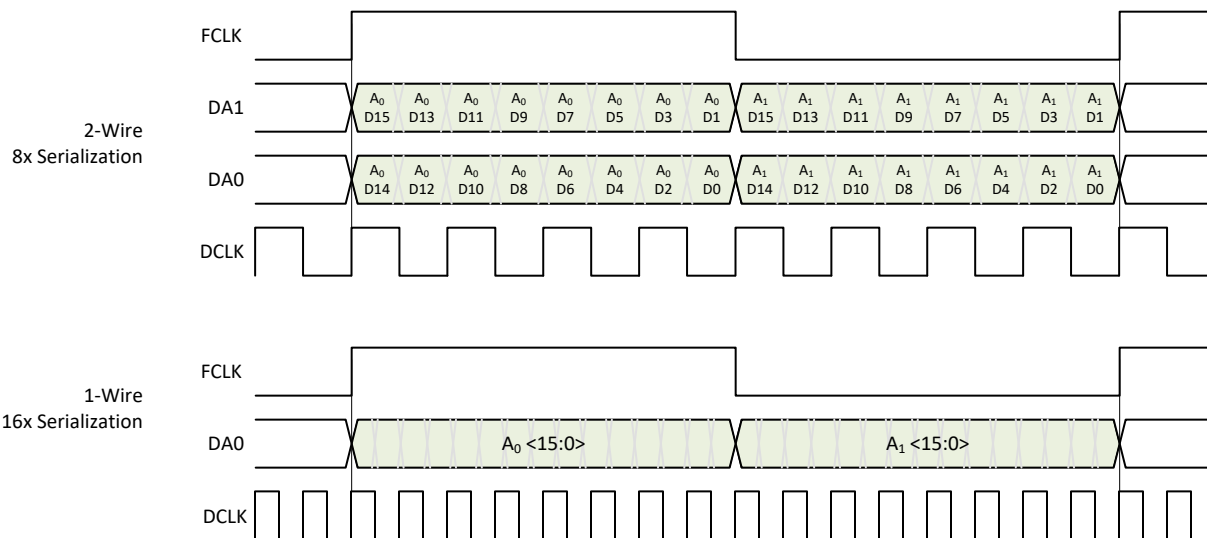
Figure 8-38. Output Data Format in Real Decimation
