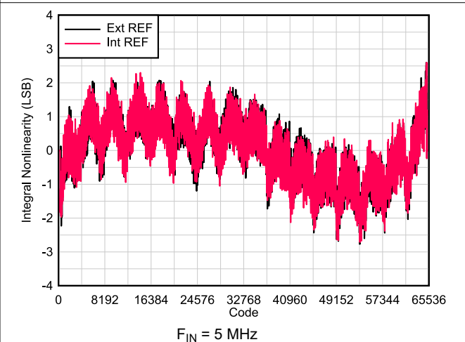
Figure 6-20. INL vs Code
