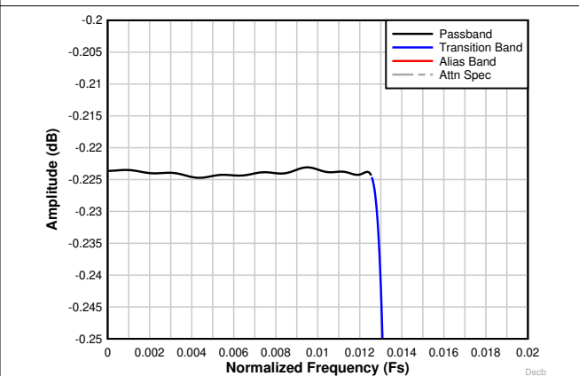
Figure 8-35. Decimation by 32 complex passband ripple response
