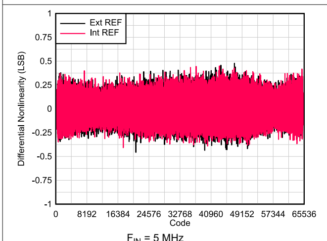
Figure 6-21. DNL vs Code
