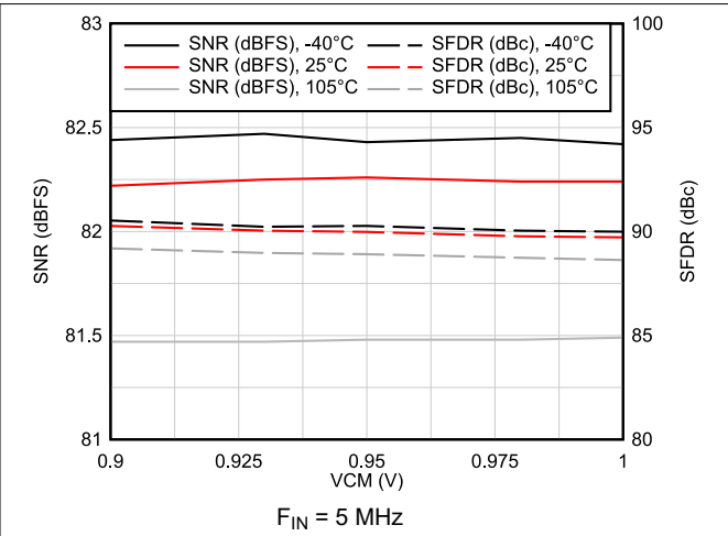
Figure 6-18. AC Performance vs VCM vs Temperature
