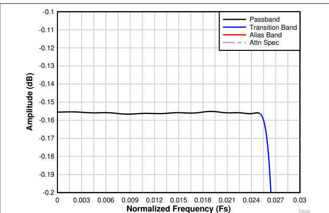
Figure 8-33. Decimation by 16 complex passband ripple response
