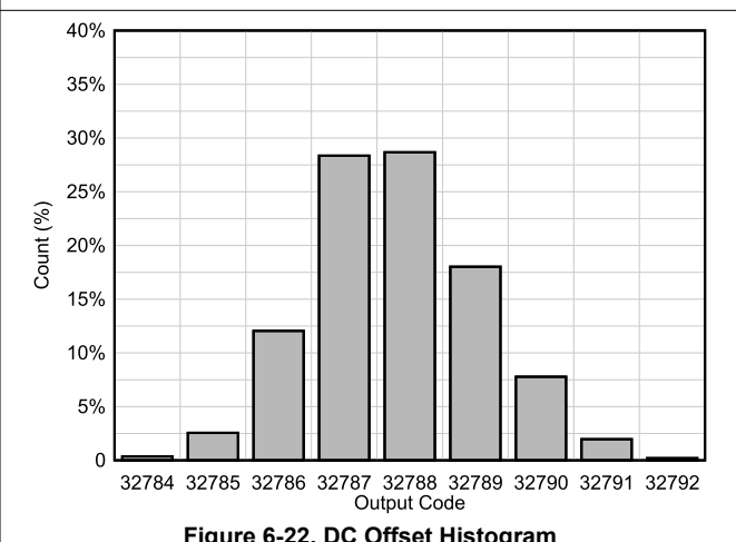
Figure 6-22. DC Offset Histogram
