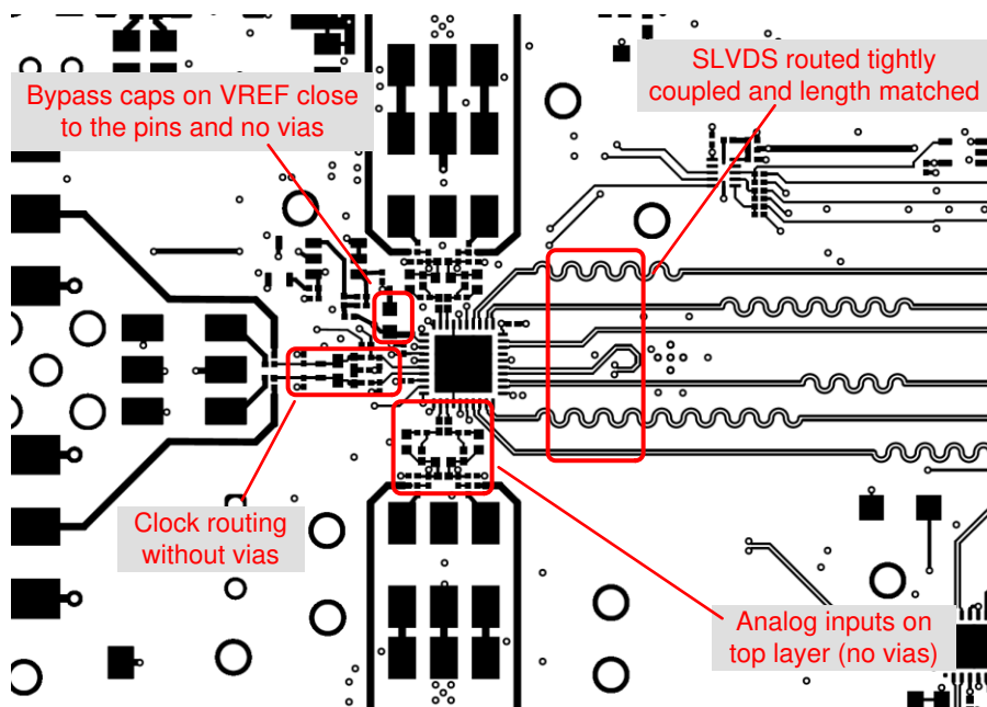
Figure 11-1. Layout example: top layer of ADC356x/368x EVM
