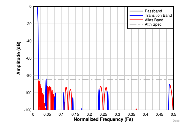
Figure 8-34. Decimation by 32 complex frequency response
