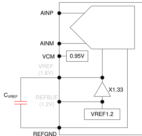
Figure 8-16. Internal reference
