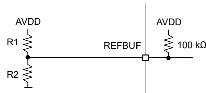
Figure 8-41. Configuration of external voltage on REFBUF pin
