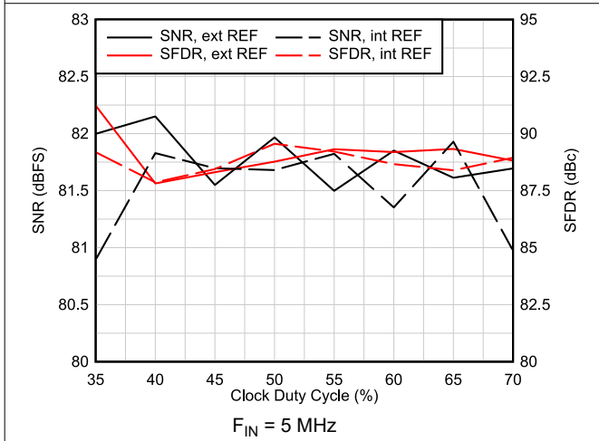
Figure 6-19. AC Performance vs Clock Duty Cycle
