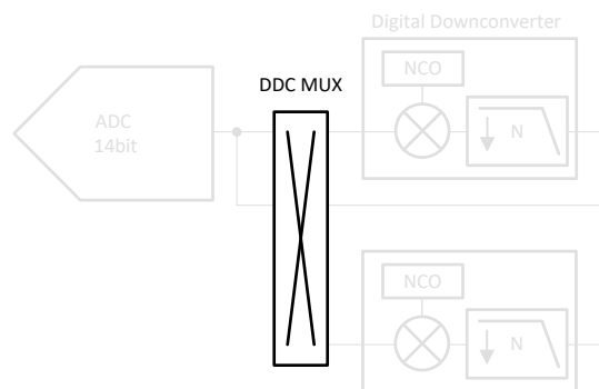
Figure 8-20. DDC MUX
