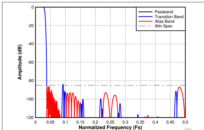
Figure 8-32. Decimation by 16 complex frequency response
