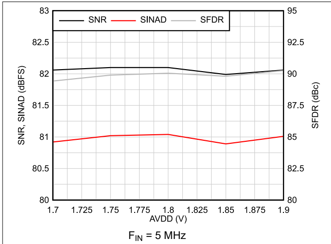
Figure 6-17. AC Performance vs AVDD
