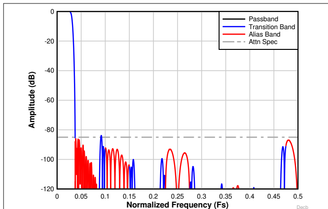
Figure 8-31. Decimation by 16 complex frequency response
