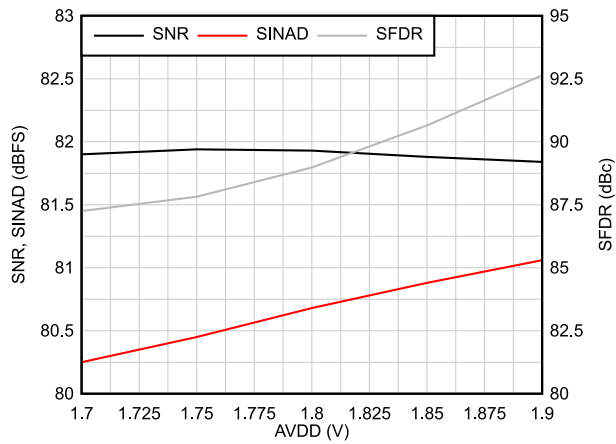
Figure 6-17. AC Performance vs AVDD
