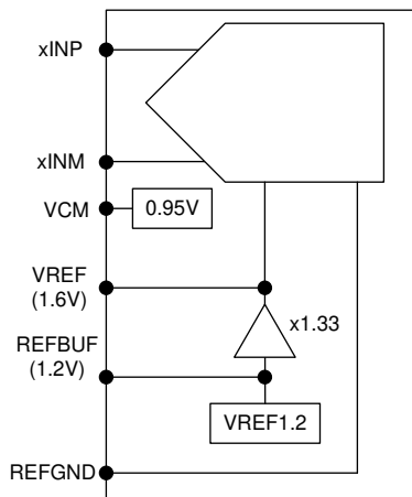
Figure 8-15. Different voltage reference options for ADC366x
