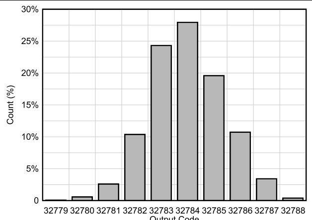
Figure 6-22. DC Offset Histogram
