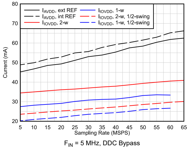
Figure 6-23. Current vs Sampling Rate
