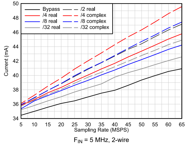
Figure 6-24. Current vs Decimation
