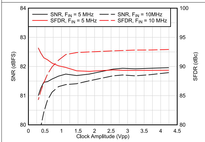
Figure 6-15. AC Performance vs Clock Amplitude
