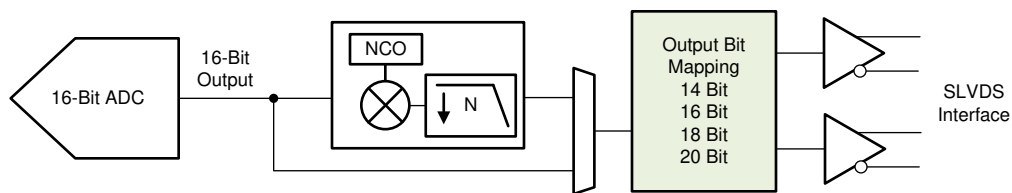
Figure 8-38. Interface output bit mapper
