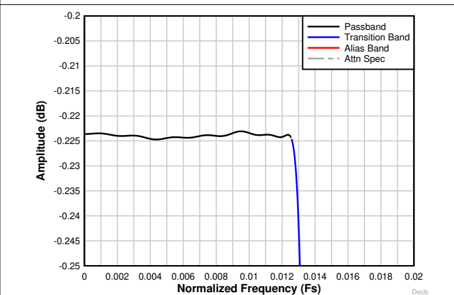
Figure 8-34. Decimation by 32 complex passband ripple response
