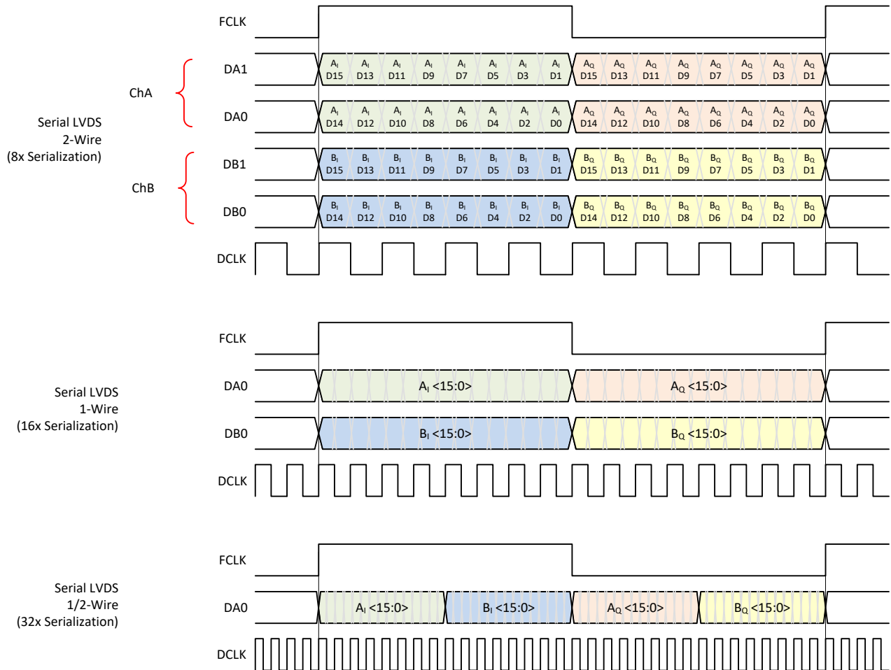
Figure 8-36. Output Data Format in Complex Decimation
