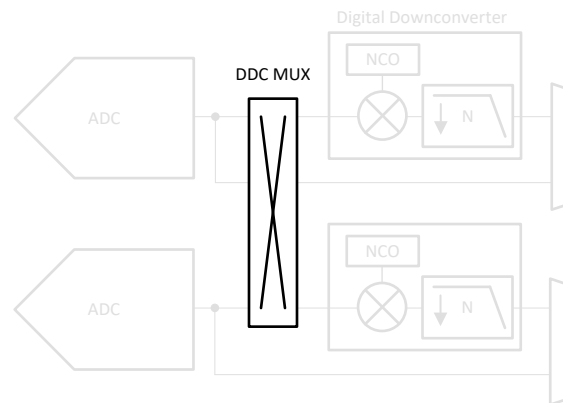
Figure 8-20. DDC MUX
