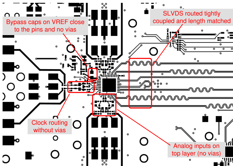
Figure 11-1. Layout example: top layer of ADC366x/368x EVM
