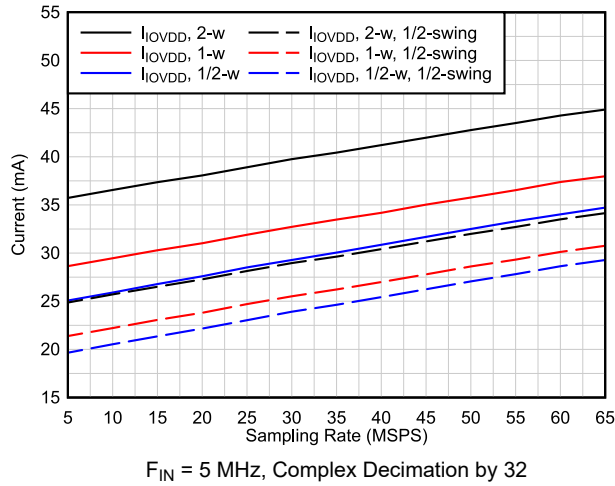
Figure 6-25. Current vs Output Interface
