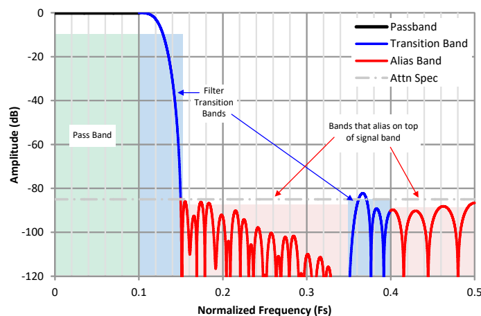
Figure 8-24. Interpretation of the Decimation Filter Plots
