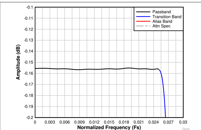
Figure 8-32. Decimation by 16 complex passband ripple response
