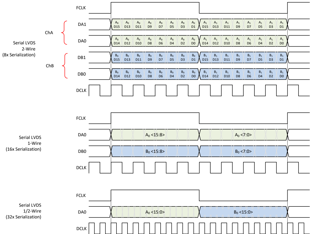
Figure 8-37. Output Data Format in Real Decimation
