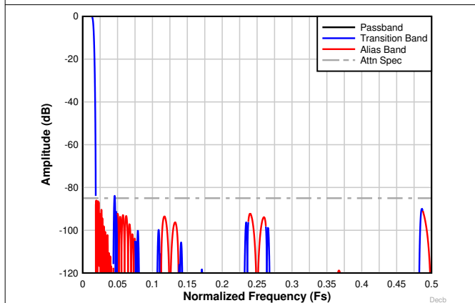
Figure 8-33. Decimation by 32 complex frequency response
