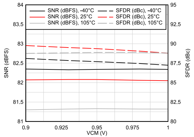
Figure 6-18. AC Performance vs VCM vs Temperature
