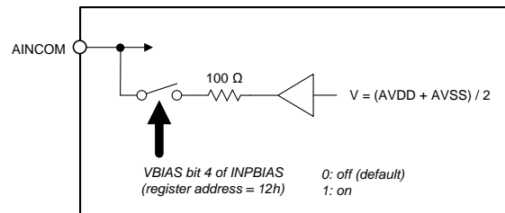
Figure 17. Level-Shift Voltage Diagram
