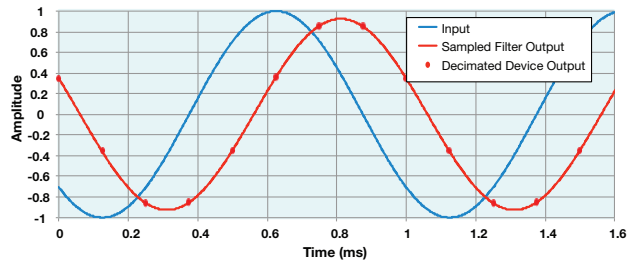
Figure 4: Analog input (blue), sampled digital filter output (red), and decimated device output (red dots).
