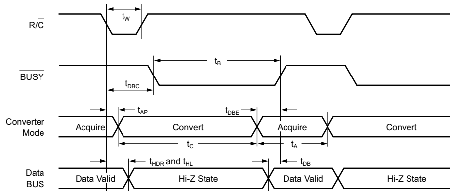
Figure 13. Convert Mode: R/C Pulse LOW — Outputs Enabled After Conversion
