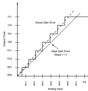
Figure 3. Positive Gain Error
