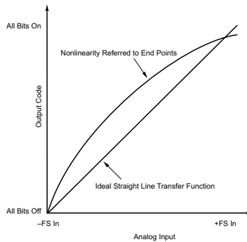
Figure 5. Integral Nonlinearity Referred to Inputs
