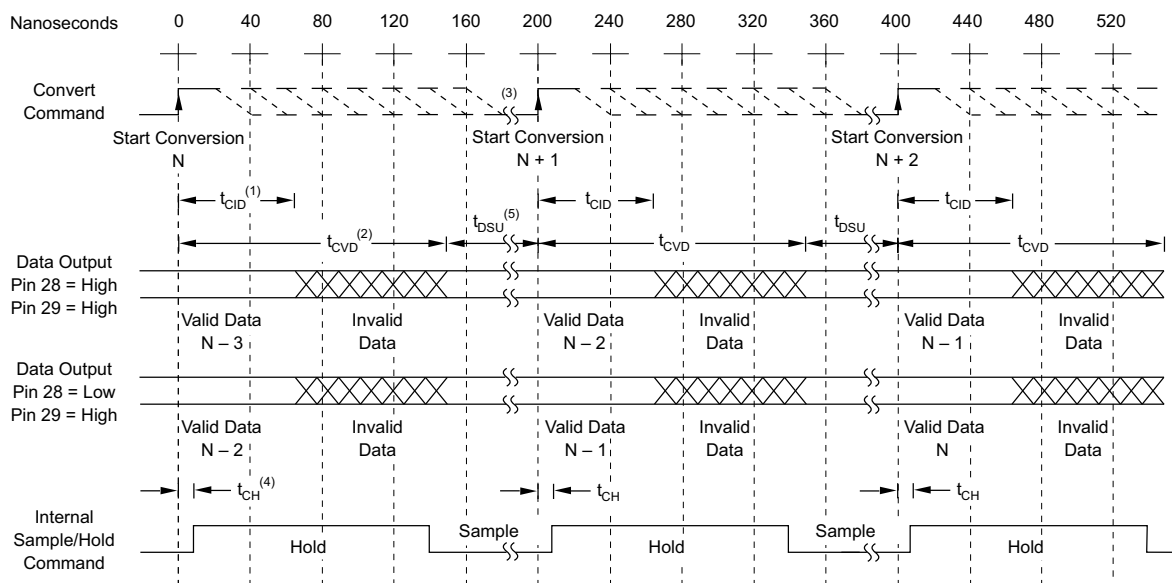
Figure 14. Basic Conversion Timing
