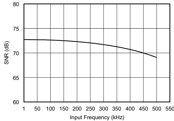
Figure 8. SNR vs Input Frequency for ADS602
