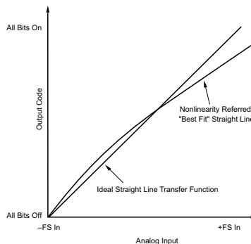
Figure 6. Integral Nonlinearity Referred to Best-Fit Straight Line
