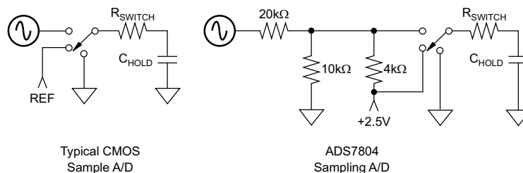
Figure 10. Comparison of Input Structures
