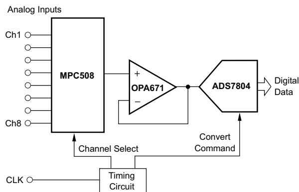
Figure 9. Traditional Analog Multiplexing System
