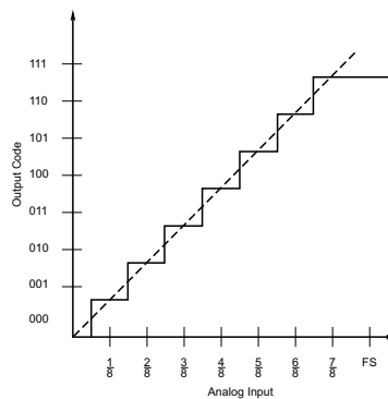
Figure 1. Ideal 3-Bit A/D Converter Transfer Function
