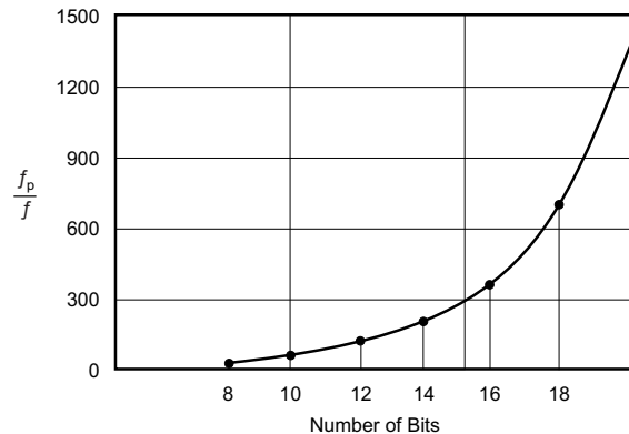
Figure 11. Ratio of First Pole to Input Frequency Required to Maintain 0.25 LSB Accuracy
