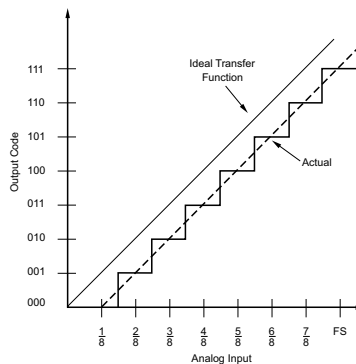
Figure 2. Offset Error of +1LSB
