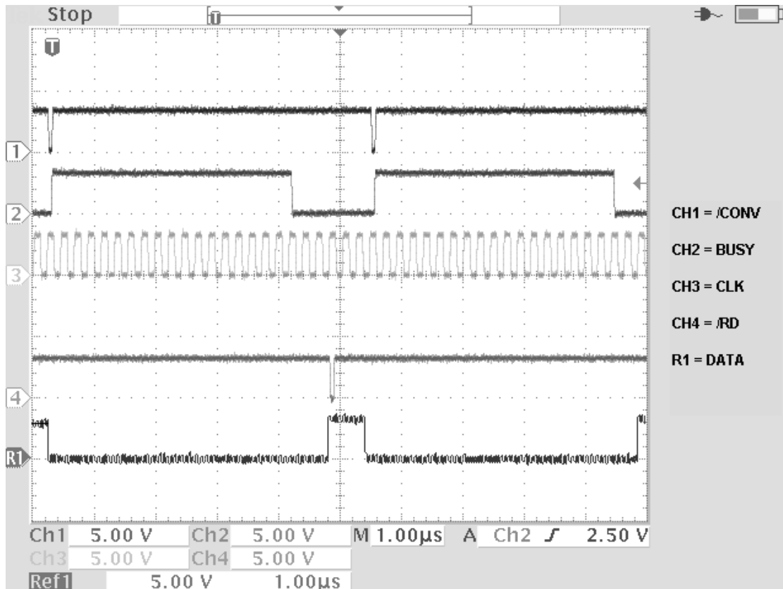
Figure 2. ADS8342 Waveforms
