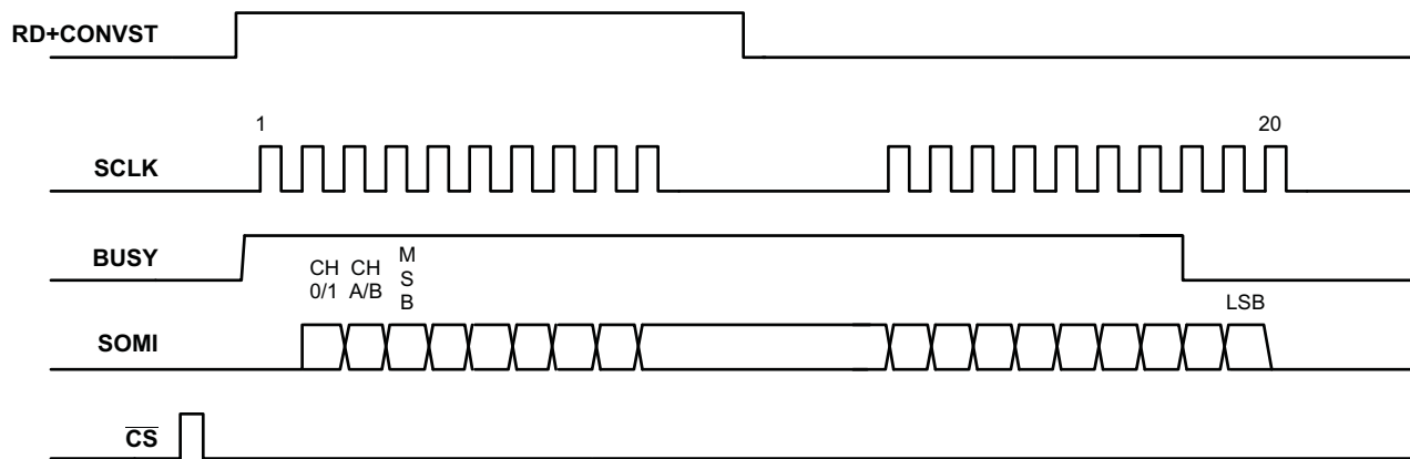
Figure 3. Timing of a Single Conversion
