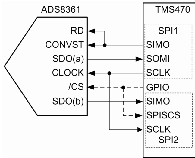
Figure 2. Hardware Interface – Modes I and III
