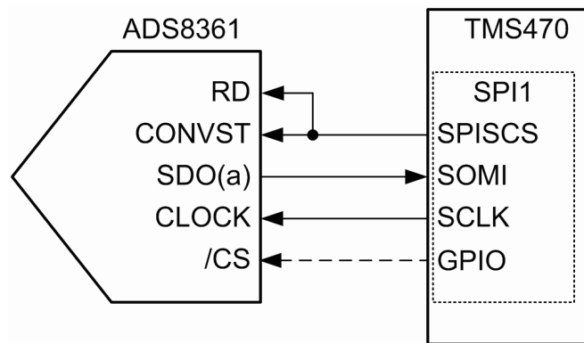
Figure 1. Hardware Interface – Modes II and IV
