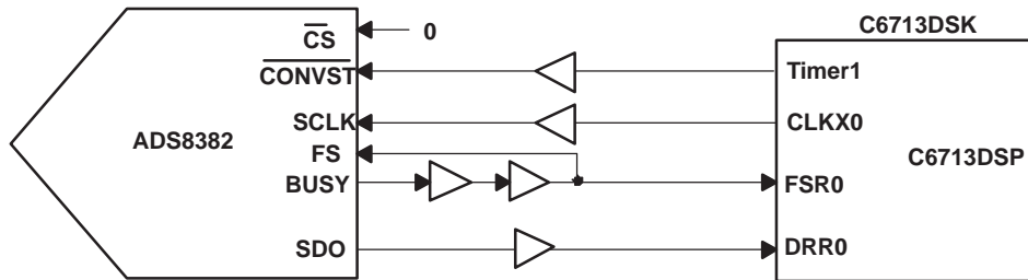
Figure 1. Hardware Connection
