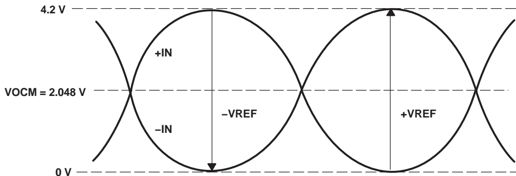
Figure 3. Analog Input Signal Range
