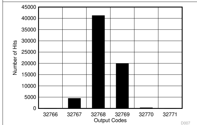
Figure 6-13. DC Histogram for Mid-Scale Inputs ( \pm 12.288\text{ V} )
