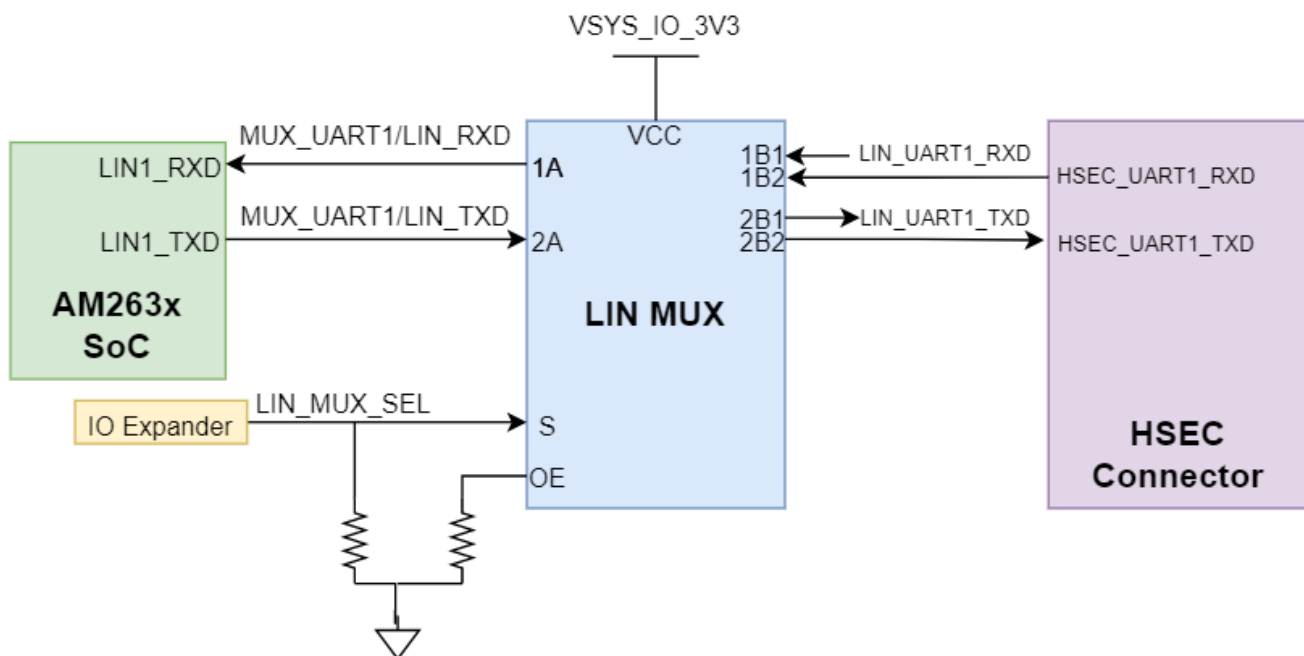
Figure 4-18. UART 1:2 MUX to HSEC
