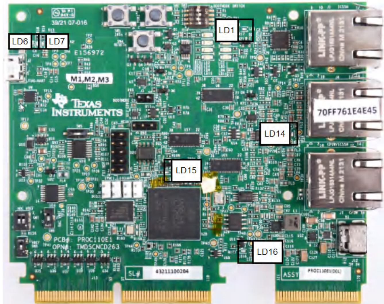
Figure 3-2. Power Status LEDs
