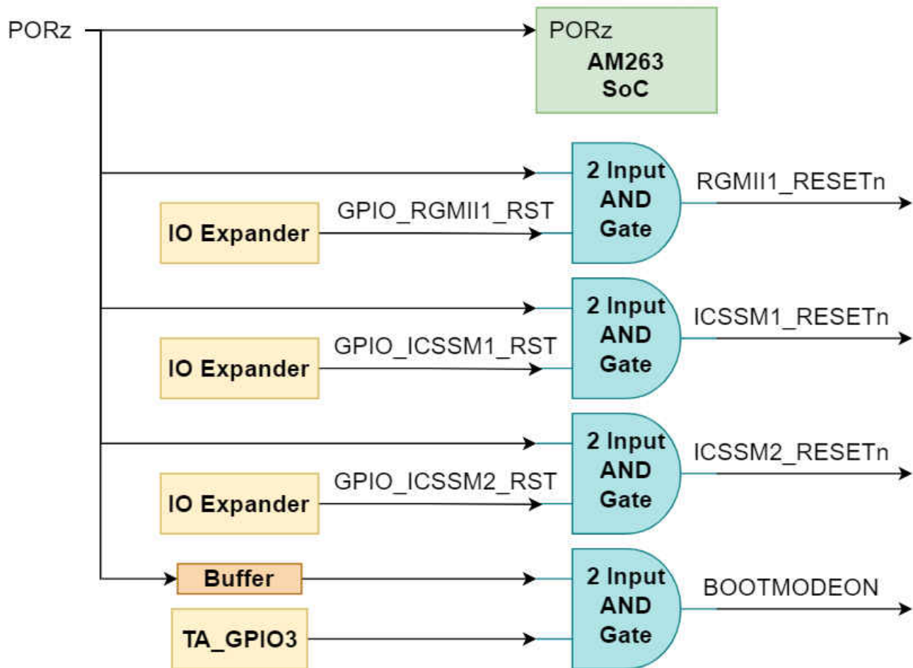
Figure 4-3. PORz Reset Signal Tree
