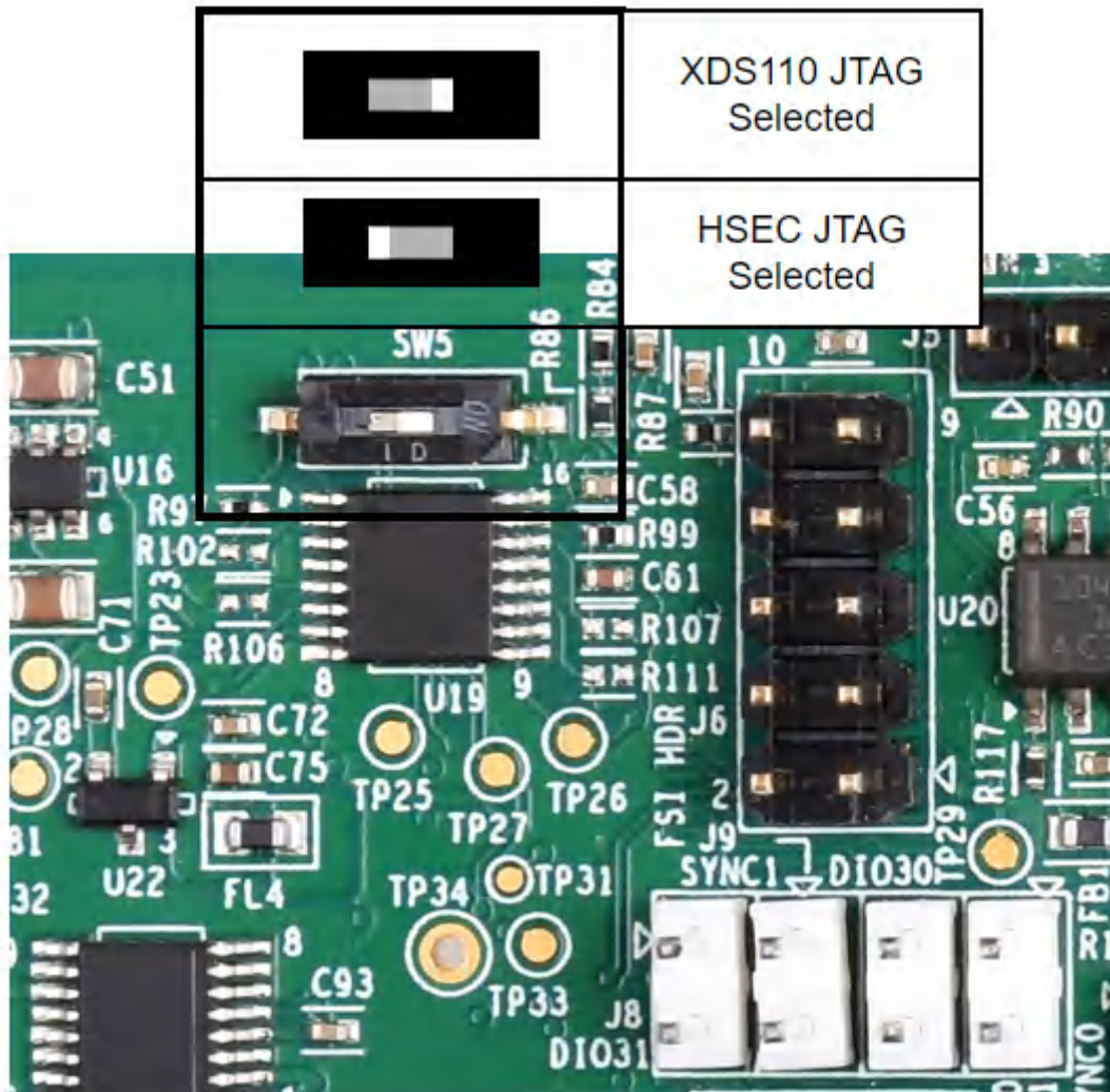
Figure 3-7. JTAG Path Switch Position
