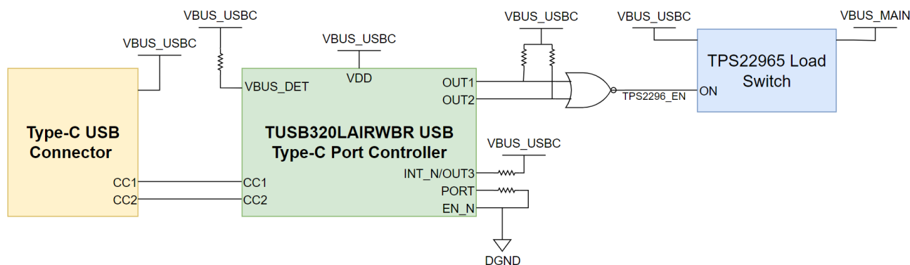
Figure 3-1. Type-C CC Configuration
