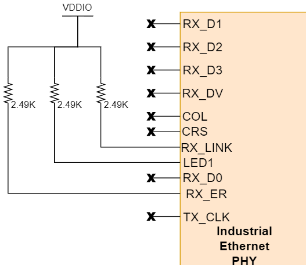
Figure 4-13. PRU1 ICSSM Industrial Ethernet PHY Strapping Resistors
