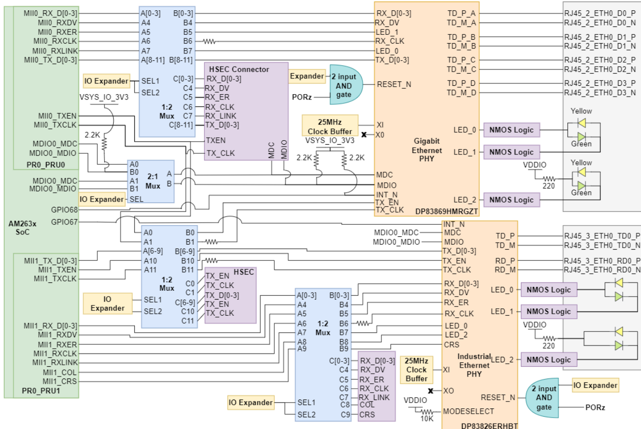
Figure 4-11. ICSSM Overview
