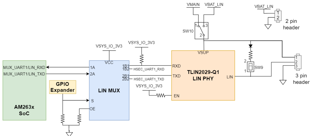
Figure 4-24. LIN PHY
