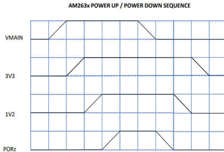
Figure 3-4. Power Sequence Diagram
