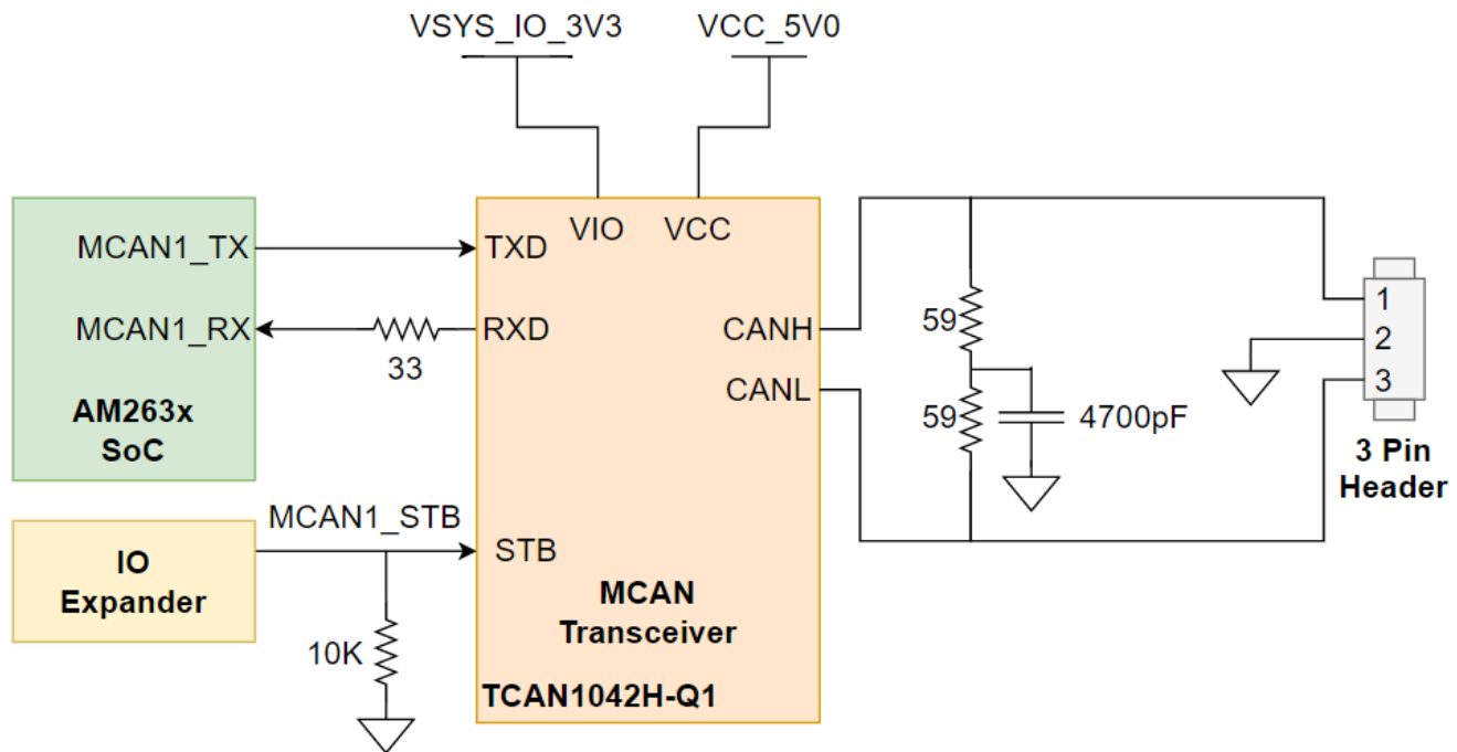
Figure 4-19. MCAN Transceiver
