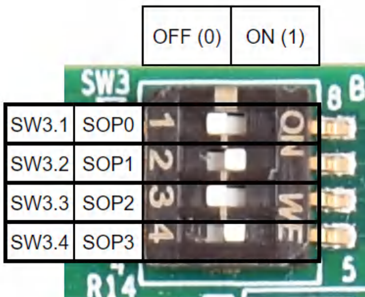
Figure 3-6. SW3 Switch Positions
