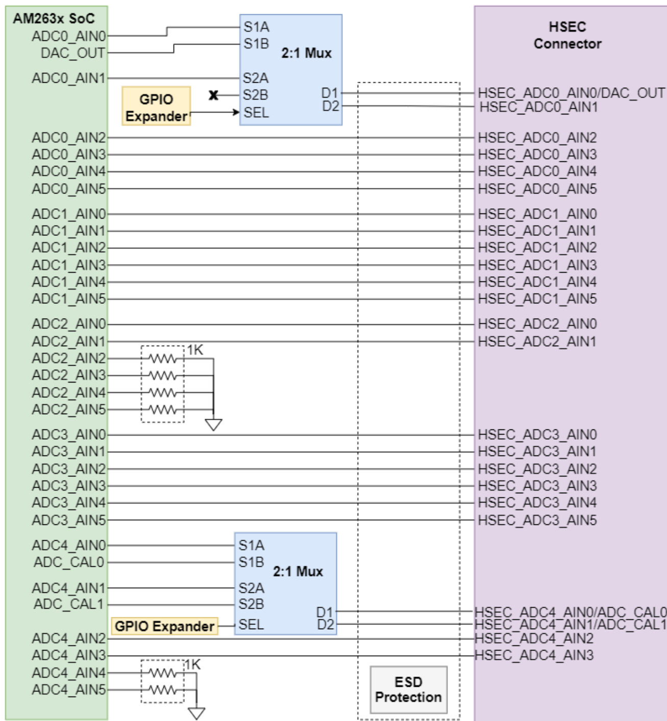
Figure 4-26. ADC HSEC Connections
