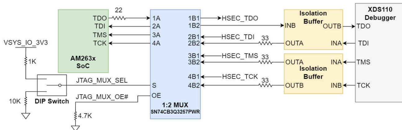
Figure 4-21. JTAG
