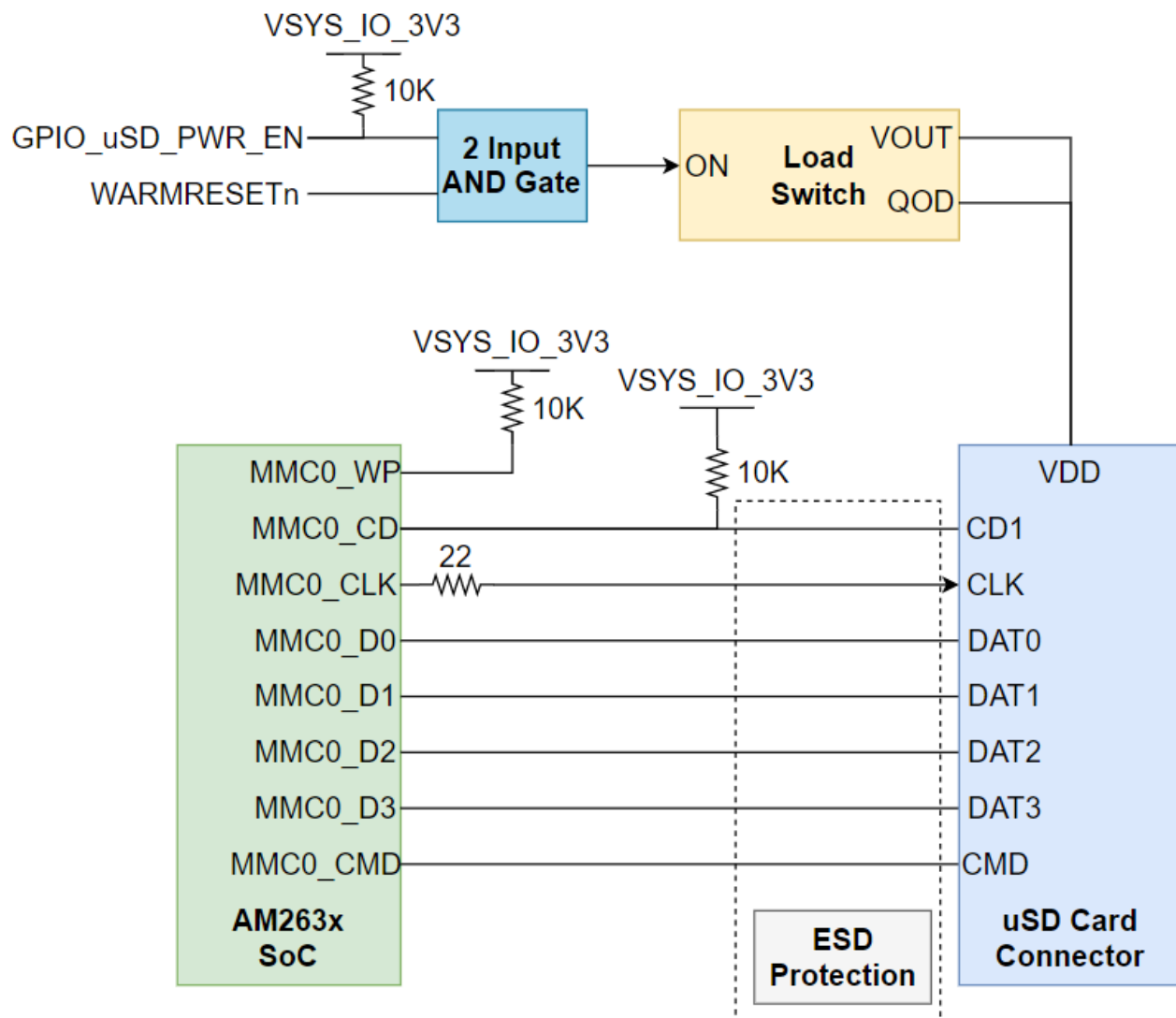
Figure 4-25. Micro-SD Connector Interface
