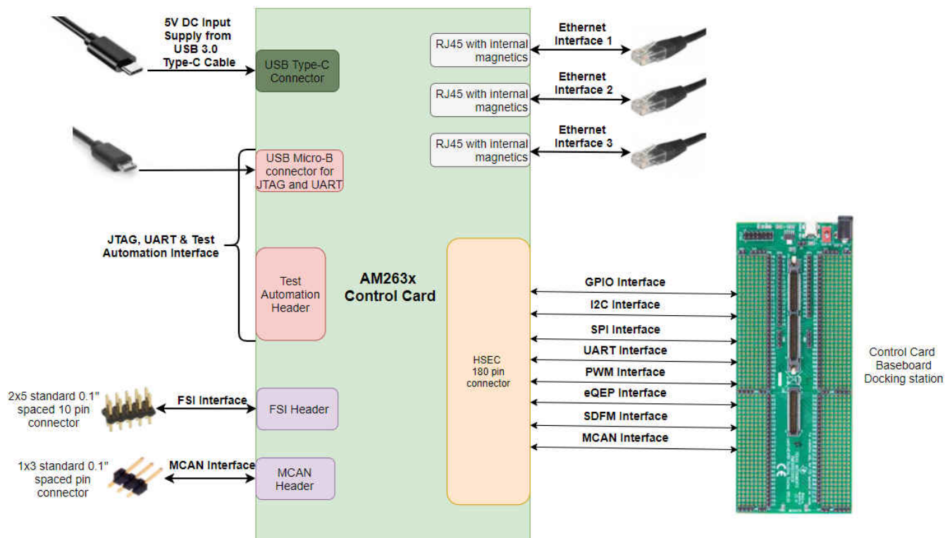
Figure 2-1. System Architecture
