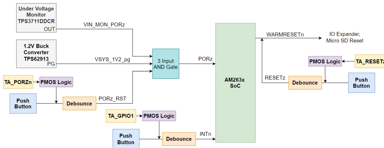
Figure 4-2. Reset Architecture
