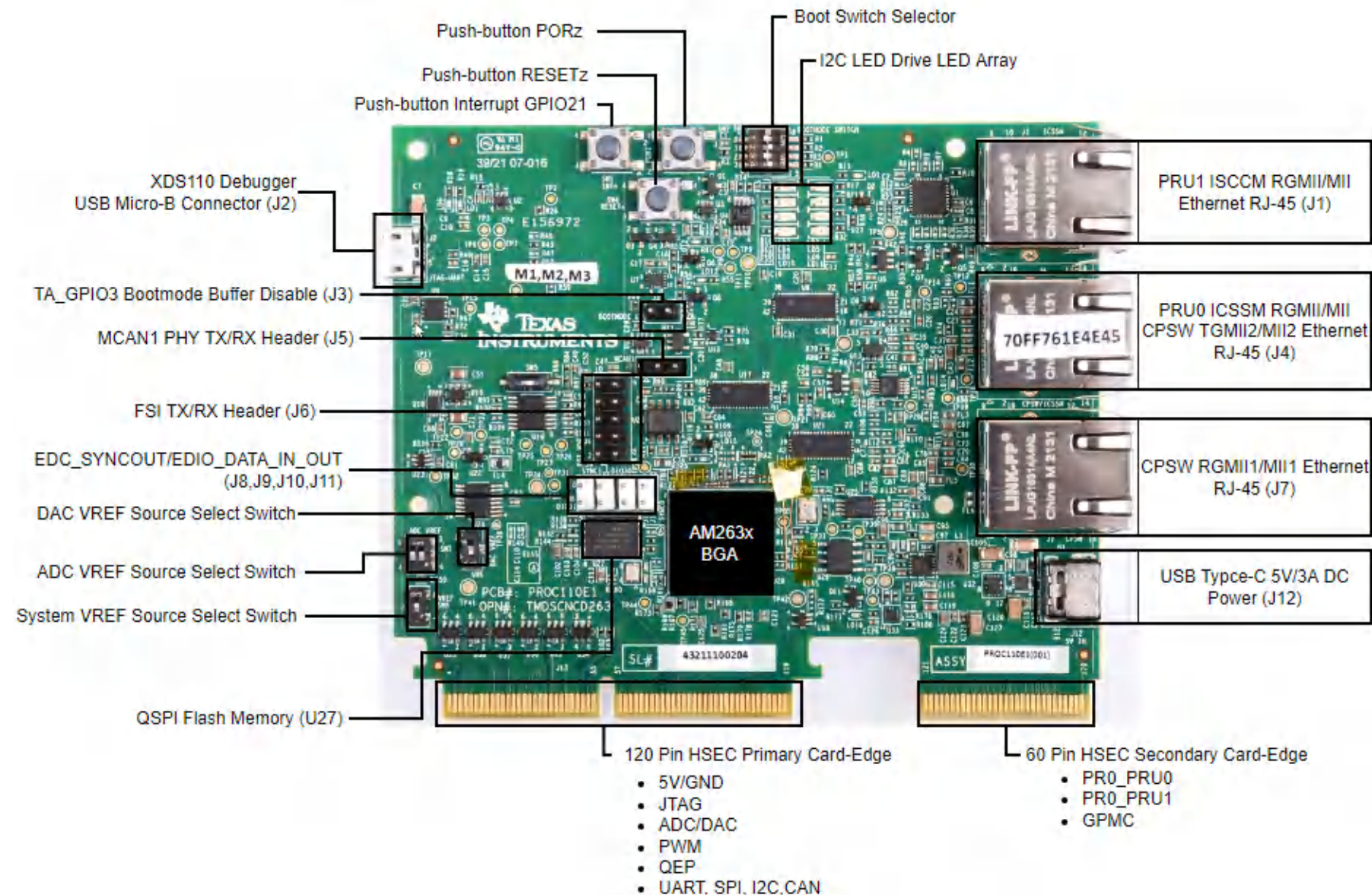
Figure 2-2. Component Identification
