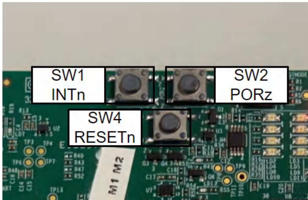
Figure 3-5. Push Buttons
