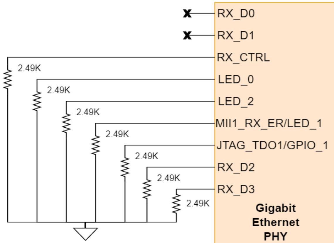
Figure 4-10. RGMII1 Gigabit Ethernet PHY Strapping Resistors
