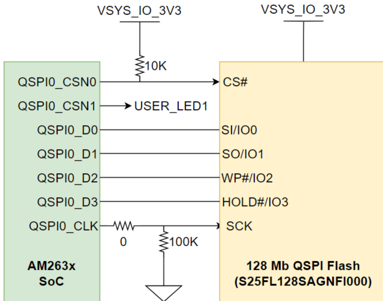
Figure 4-7. QSPI Interface
