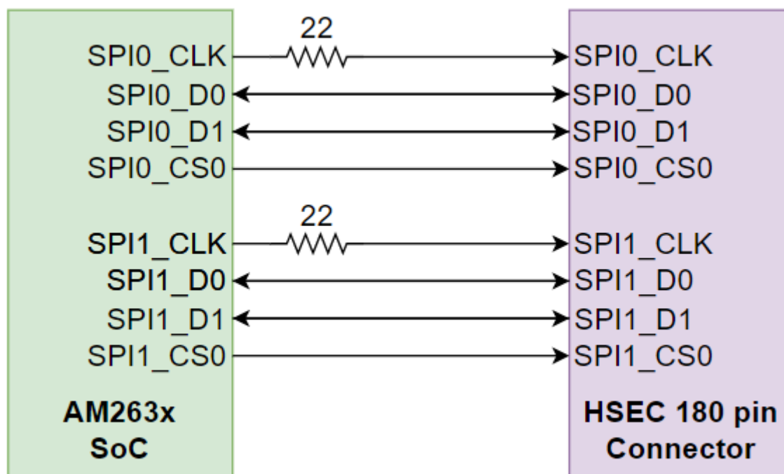
Figure 4-16. SPI
