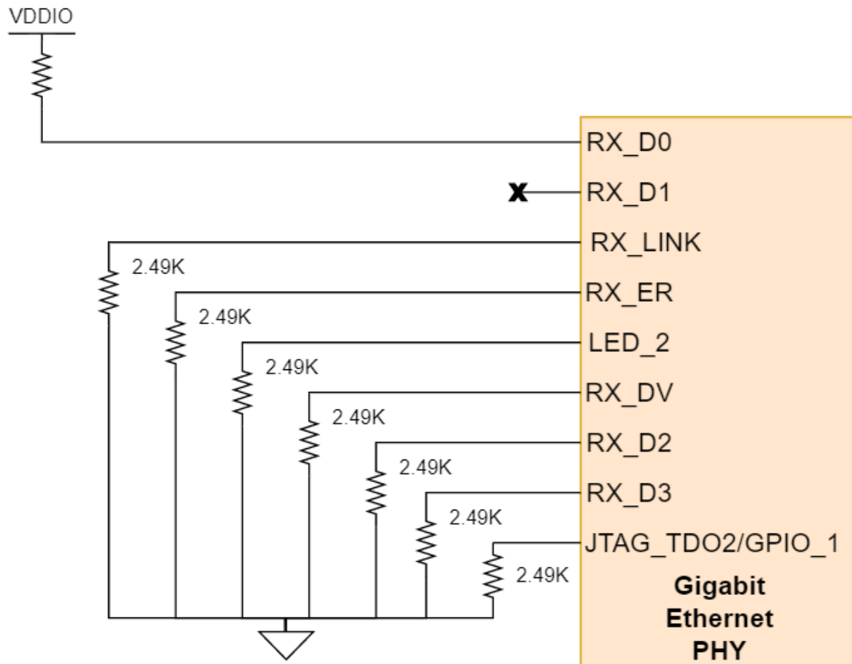
Figure 4-12. PRU0 ICSSM Gigabit Ethernet PHY Strapping Resistors
