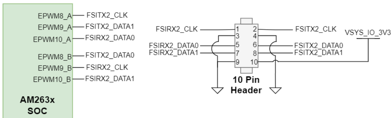
Figure 4-20. FSI Header
