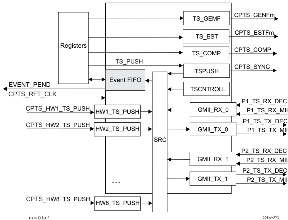
Figure 13-106. CPTS Block Diagram
