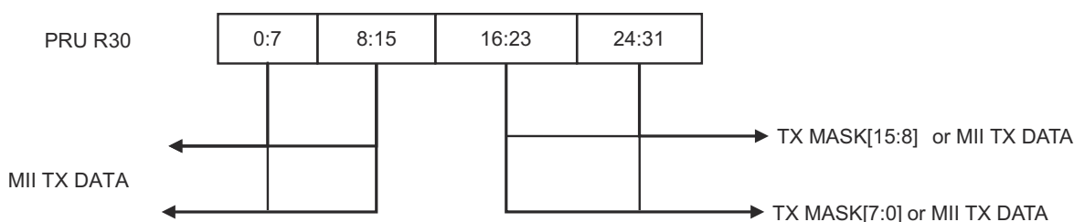
Figure 7-72. PRU to TX MII Interface
