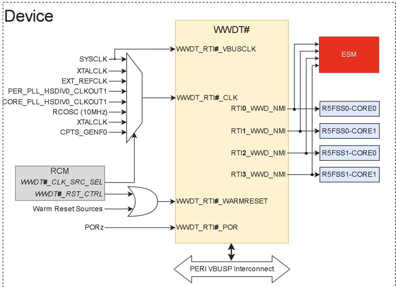
Figure 4-22. WWDT Integration
