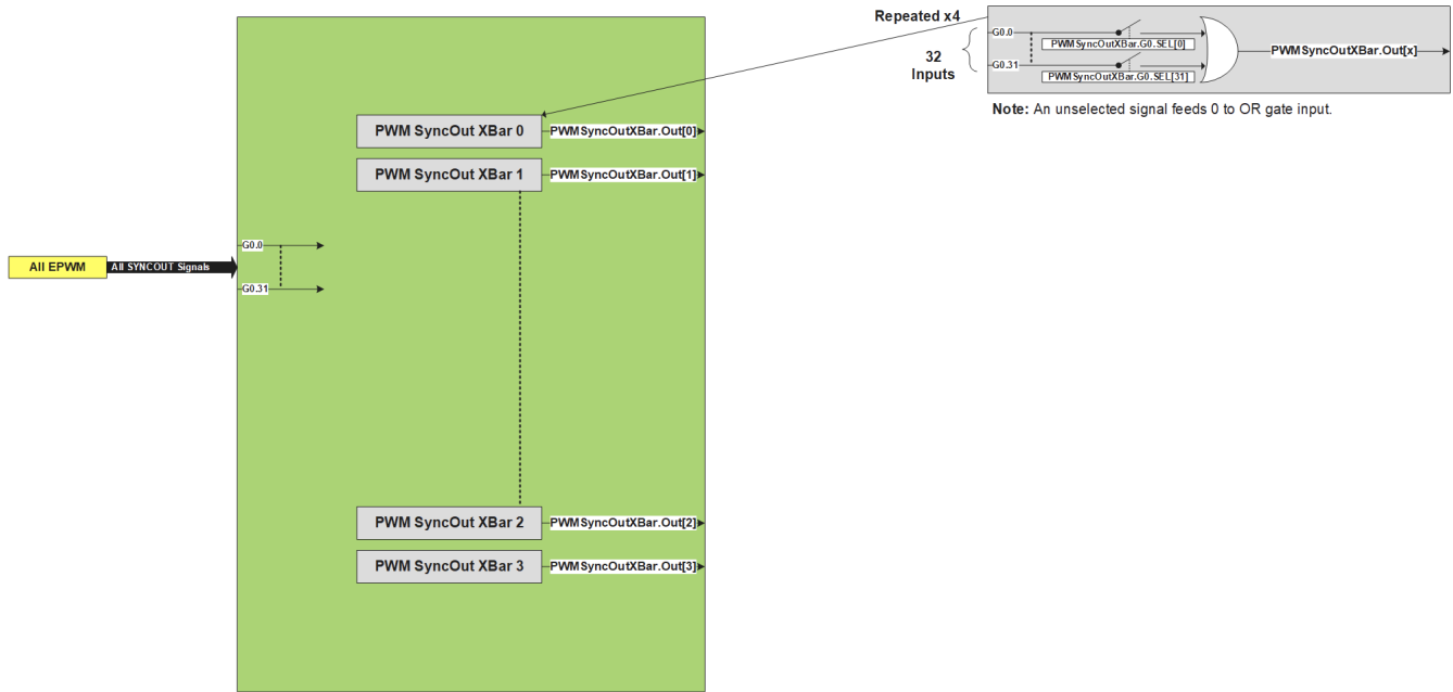
Figure 7-263. pwmsyncout x-bar
