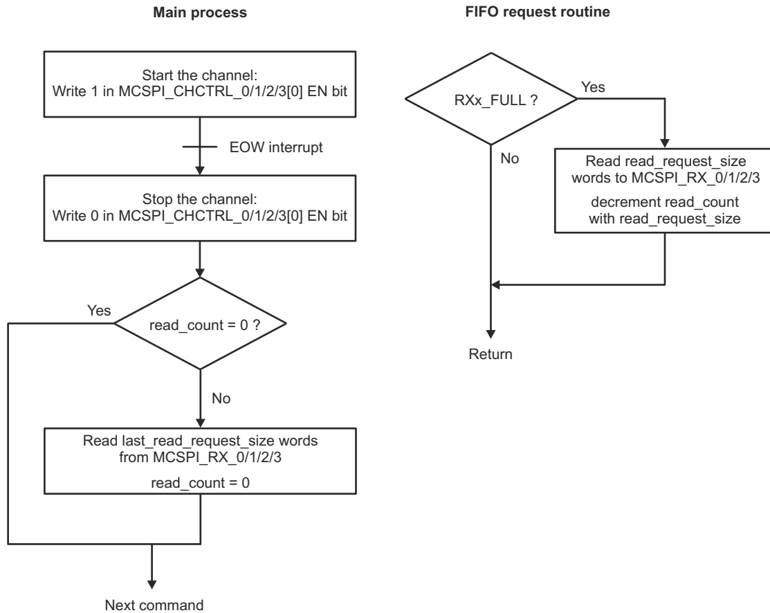
Figure 13-54. FIFO Mode Receive-Only With Word Count (Controller)
