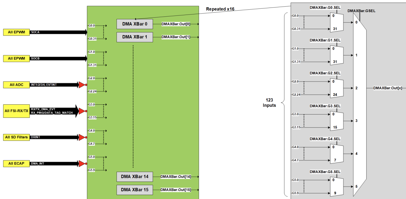
Figure 7-262. DMAXBAR Block Diagram
