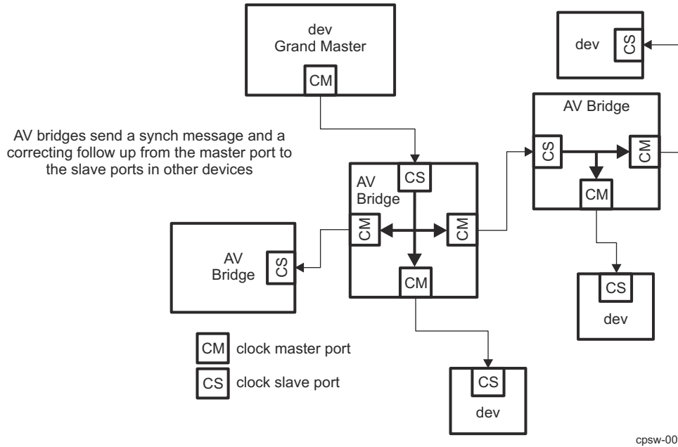
Figure 13-102. AVB Network & PTP Clock Entities
