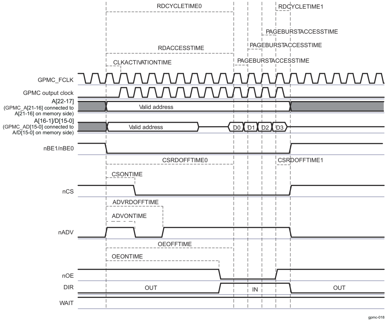
Figure 13-145. Synchronous Multiple (Burst) Read (GPMCFCLKDIVIDER = 0)
