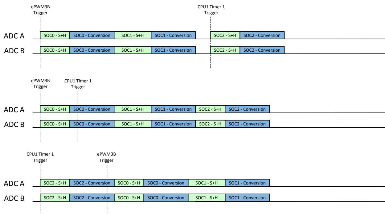
Figure 7-99. Example: Synchronous Operation with Multiple Trigger Sources
