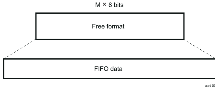
Figure 13-63. SIR FF Mode
