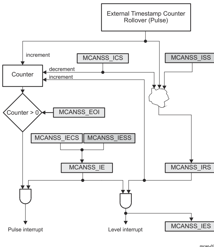
Figure 13-230. External Timestamp Counter Interrupt
