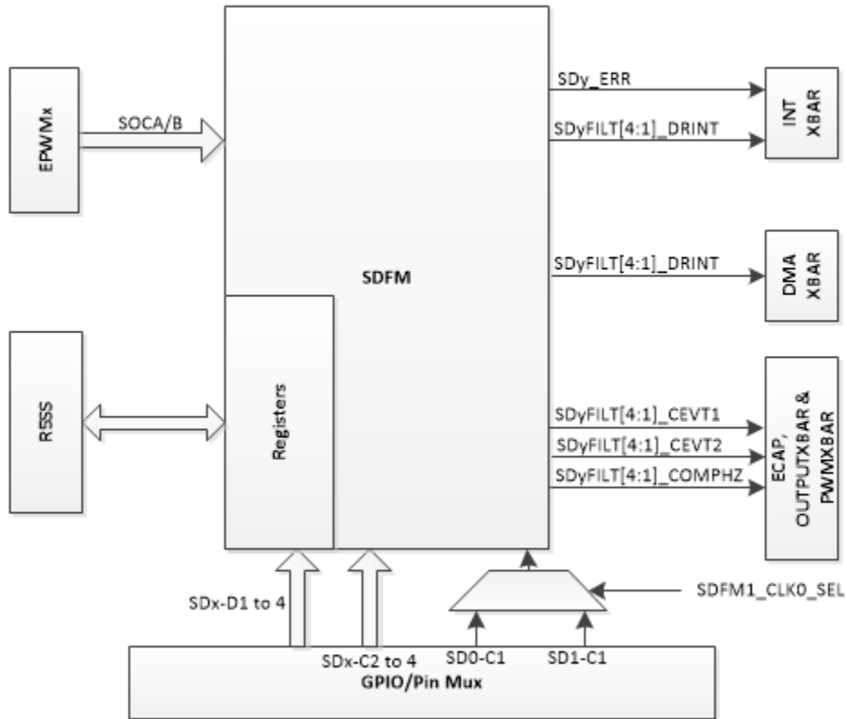
Figure 7-247. SDFM Integration Diagram (Simple)
