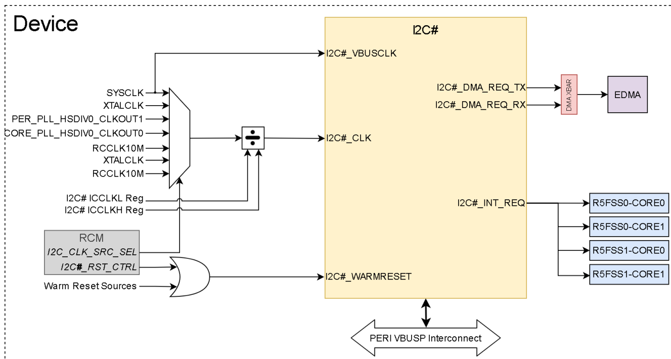
Figure 13-18. I2C Integration
