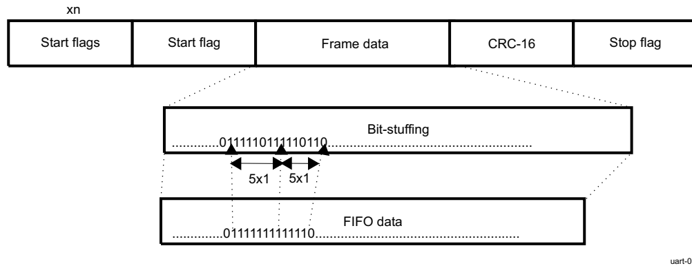
Figure 13-64. MIR Transmit Frame Format
