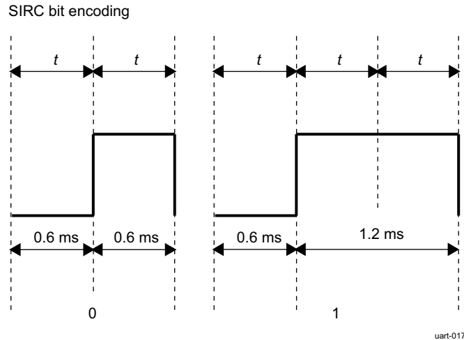
Figure 13-72. UART SIRC Bit Encoding
