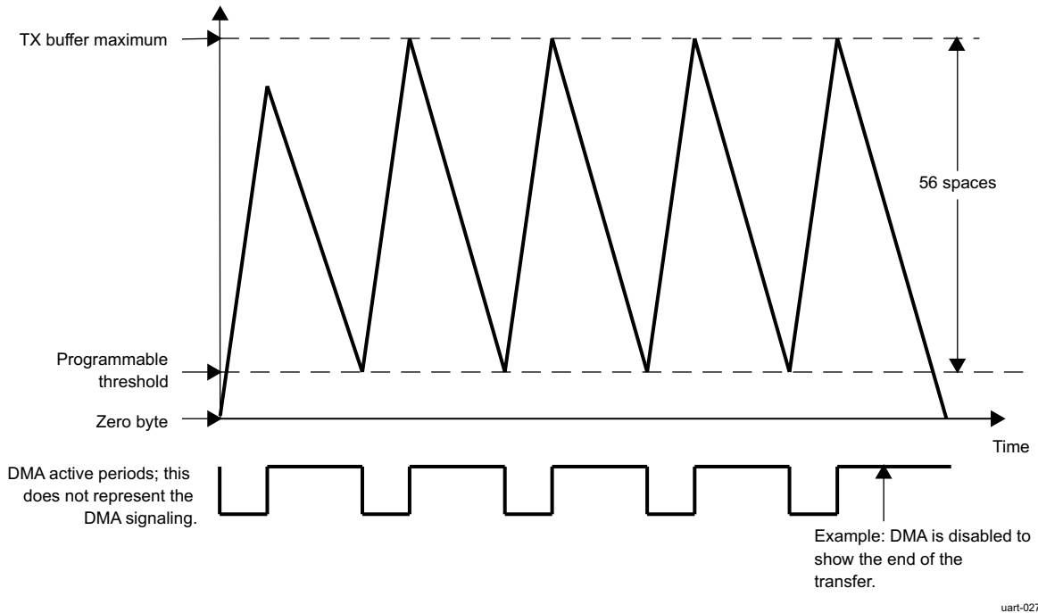
Figure 13-82. UART Transmit FIFO DMA Request Generation (56 Spaces)
