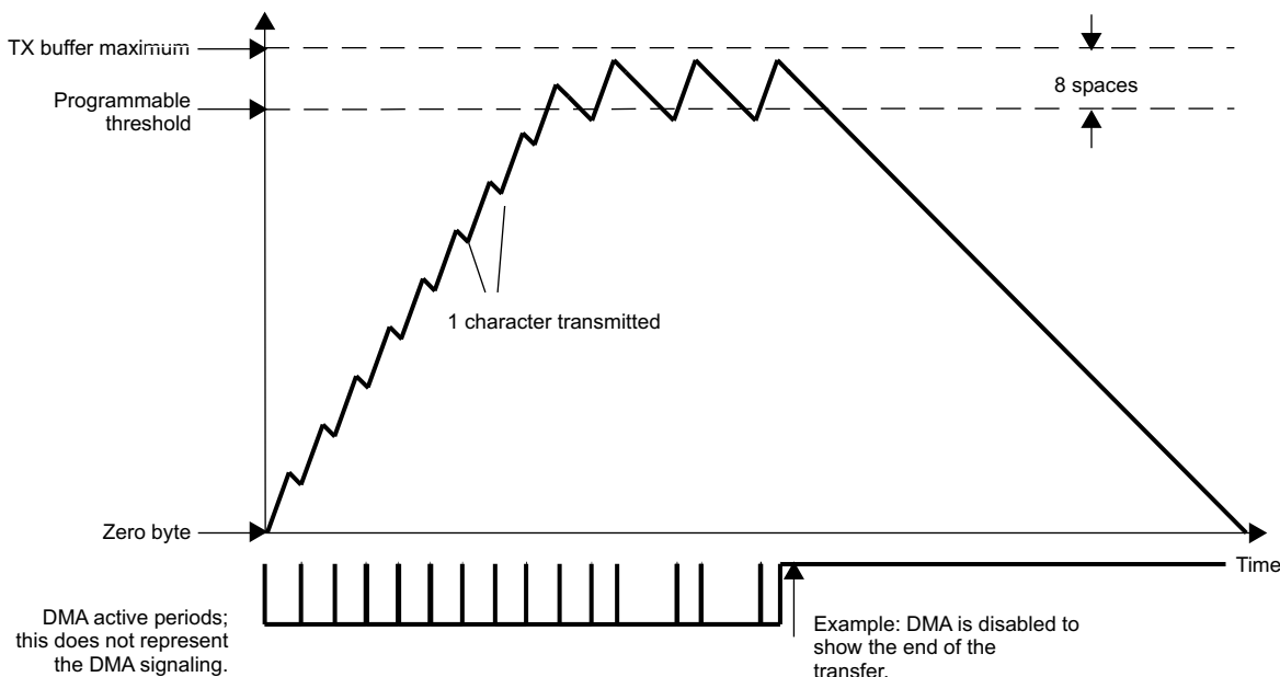
Figure 13-83. UART Transmit FIFO DMA Request Generation (8 Spaces)
