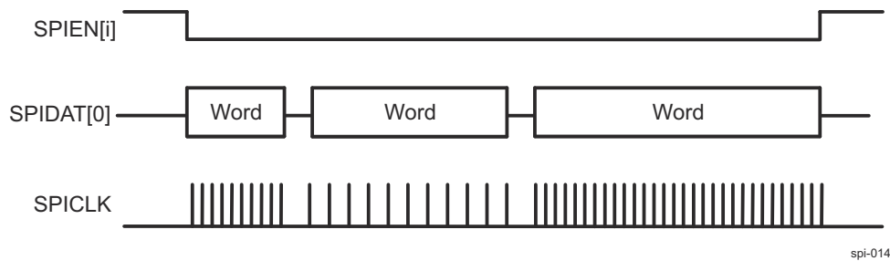
Figure 13-39. Continuous Transfers With SPIEN[i] Maintained Active (Single-Data-Pin Interface Mode)
