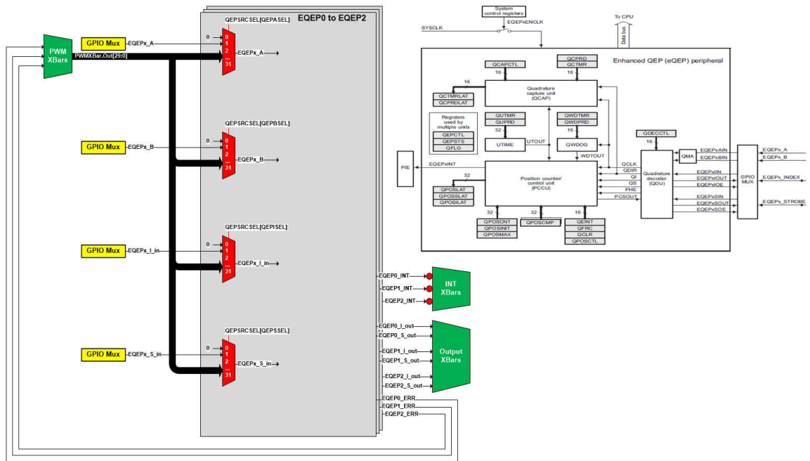
Figure 7-212. EQEP Integration Diagram
