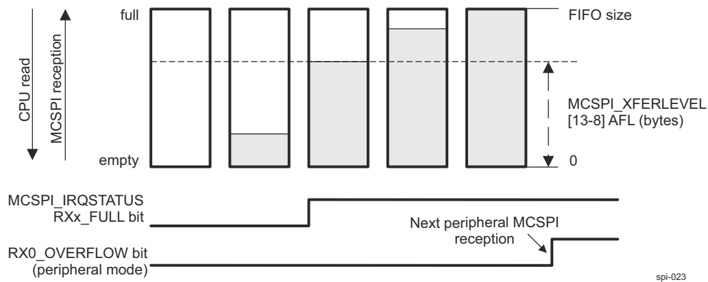
Figure 13-48. Buffer Almost Full Level (AFL)
