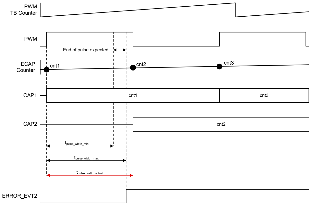
Figure 7-202. ECAP Signal Monitoring Unit Pulse Width Error Example
