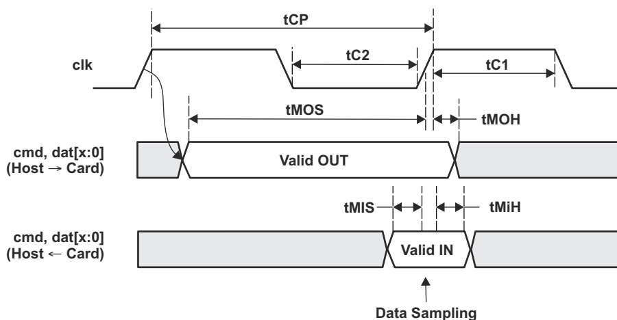
Figure 13-208. Output Driven on Rising Edge
