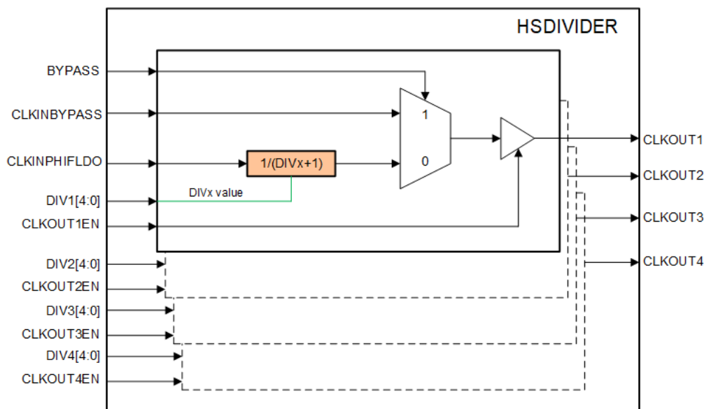
Figure 6-21. HSDIVIDER Architecture
