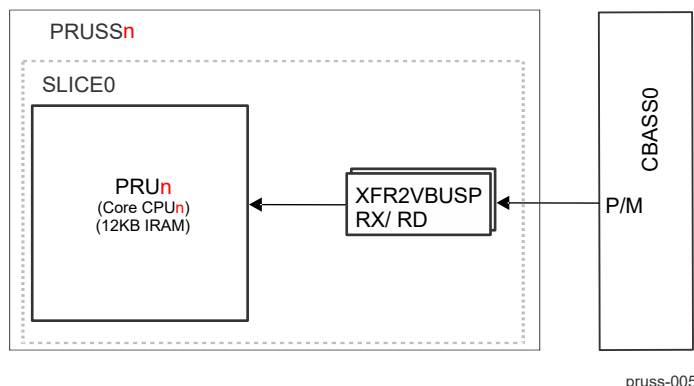
Figure 7-42. XFR2VBUS Hardware Accelerator
