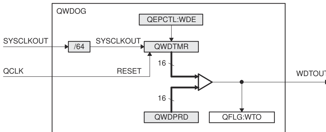
Figure 7-228. eQEP Watchdog Timer
