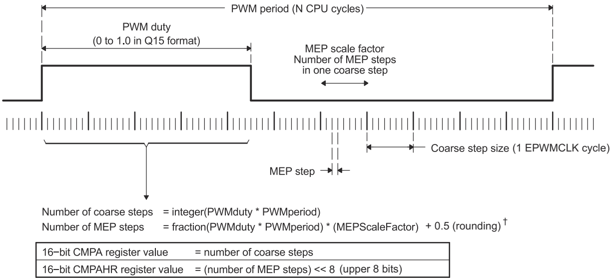
Figure 7-179. Operating Logic Using MEP
