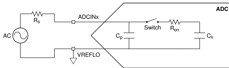
Figure 7-88. Single-Ended Input Model
