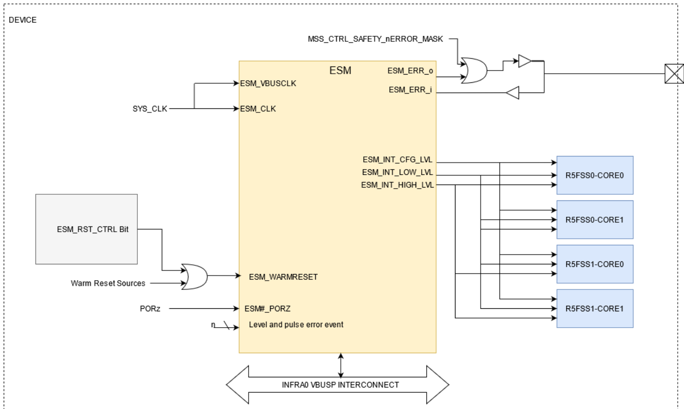
Figure 13-289. ESM Integration Diagram
