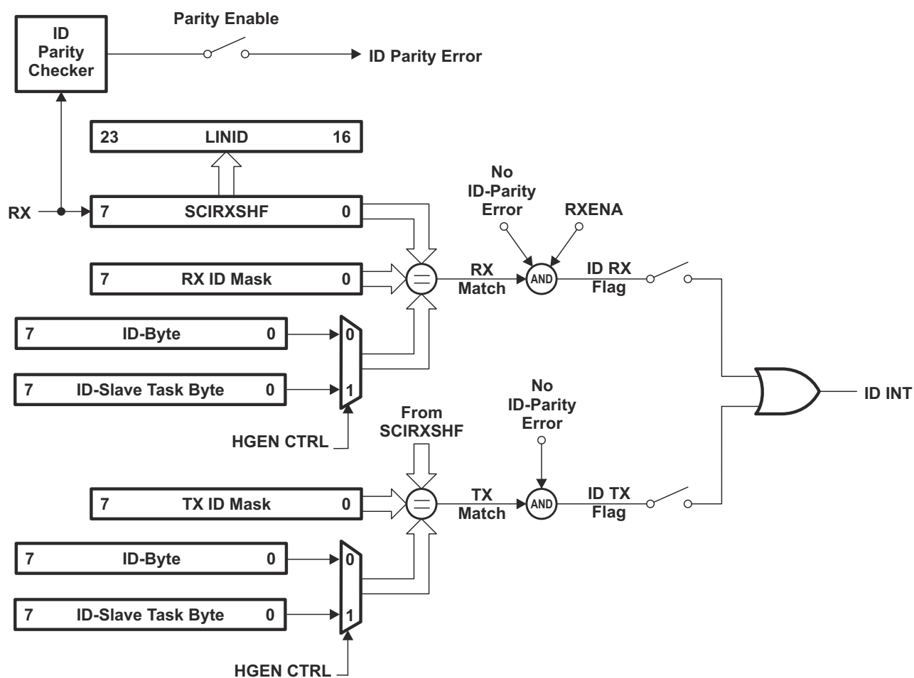
Figure 13-266. ID Reception, Filtering and Validation
