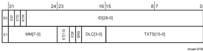
Figure 13-239. Tx Buffer Element Structure
