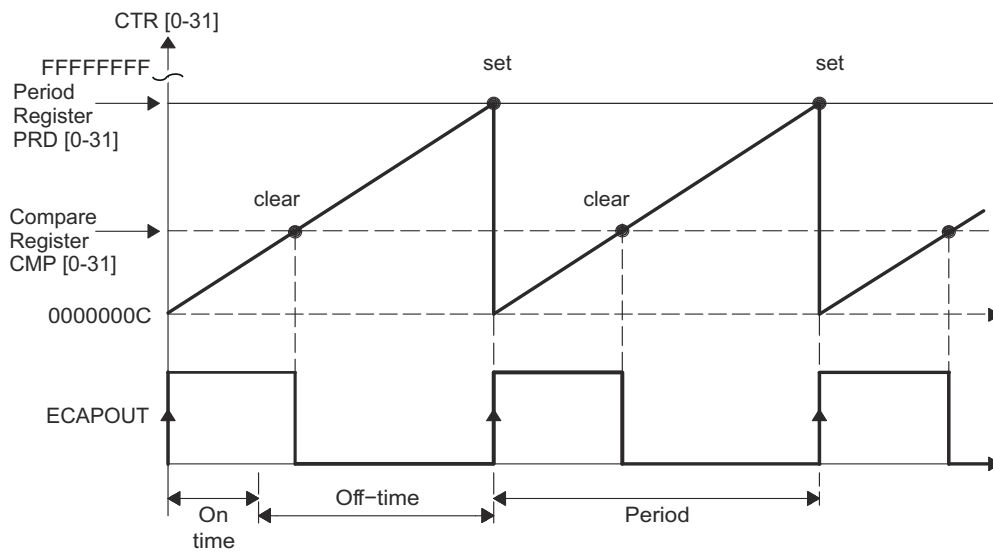
Figure 7-192. Counter Compare and PRD Effects on the eCAP Output in APWM Mode
