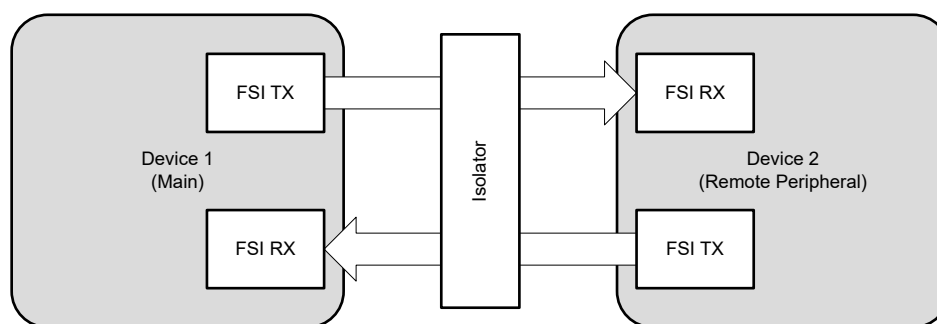
Figure 7-243. Point to Point Connection
