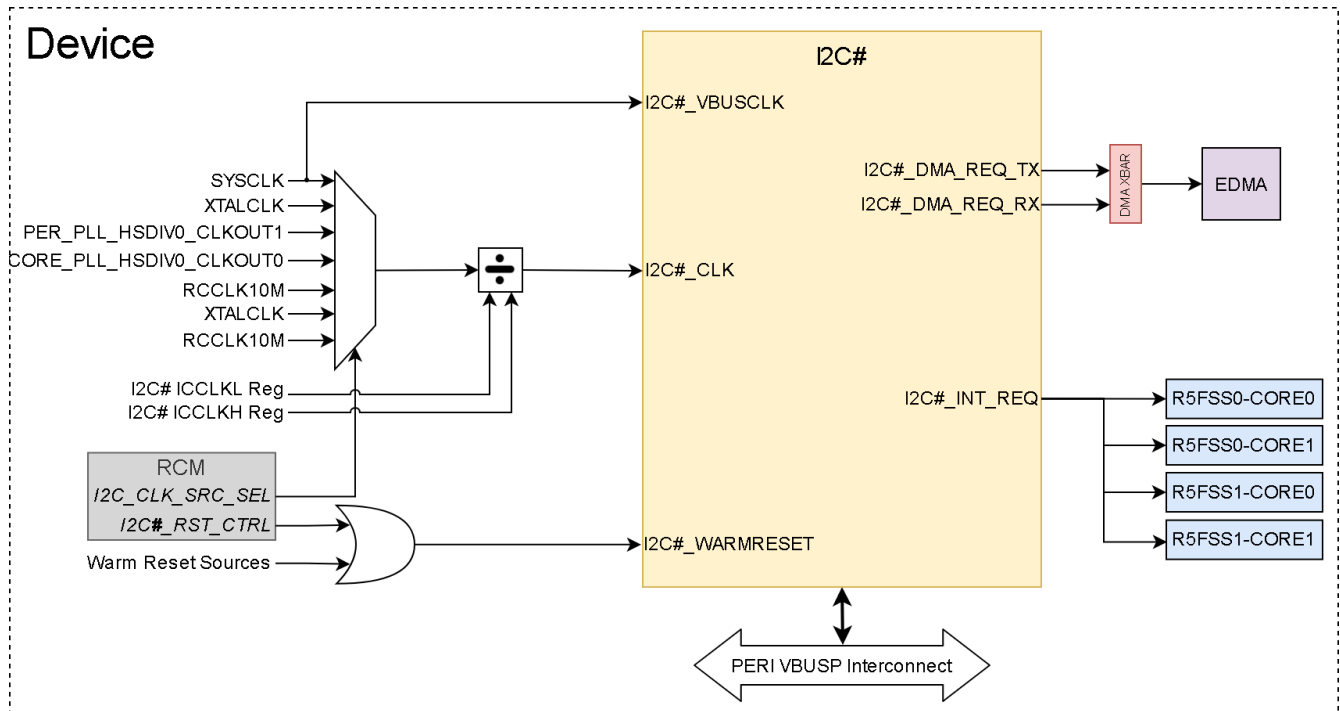
Figure 4-13. I2C Integration
