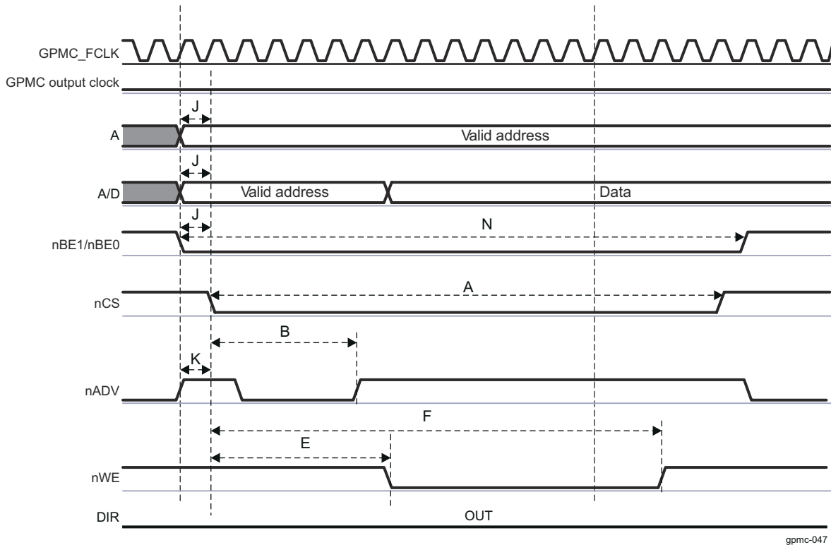
Figure 13-176. Asynchronous NOR Single Write Simplified Example
