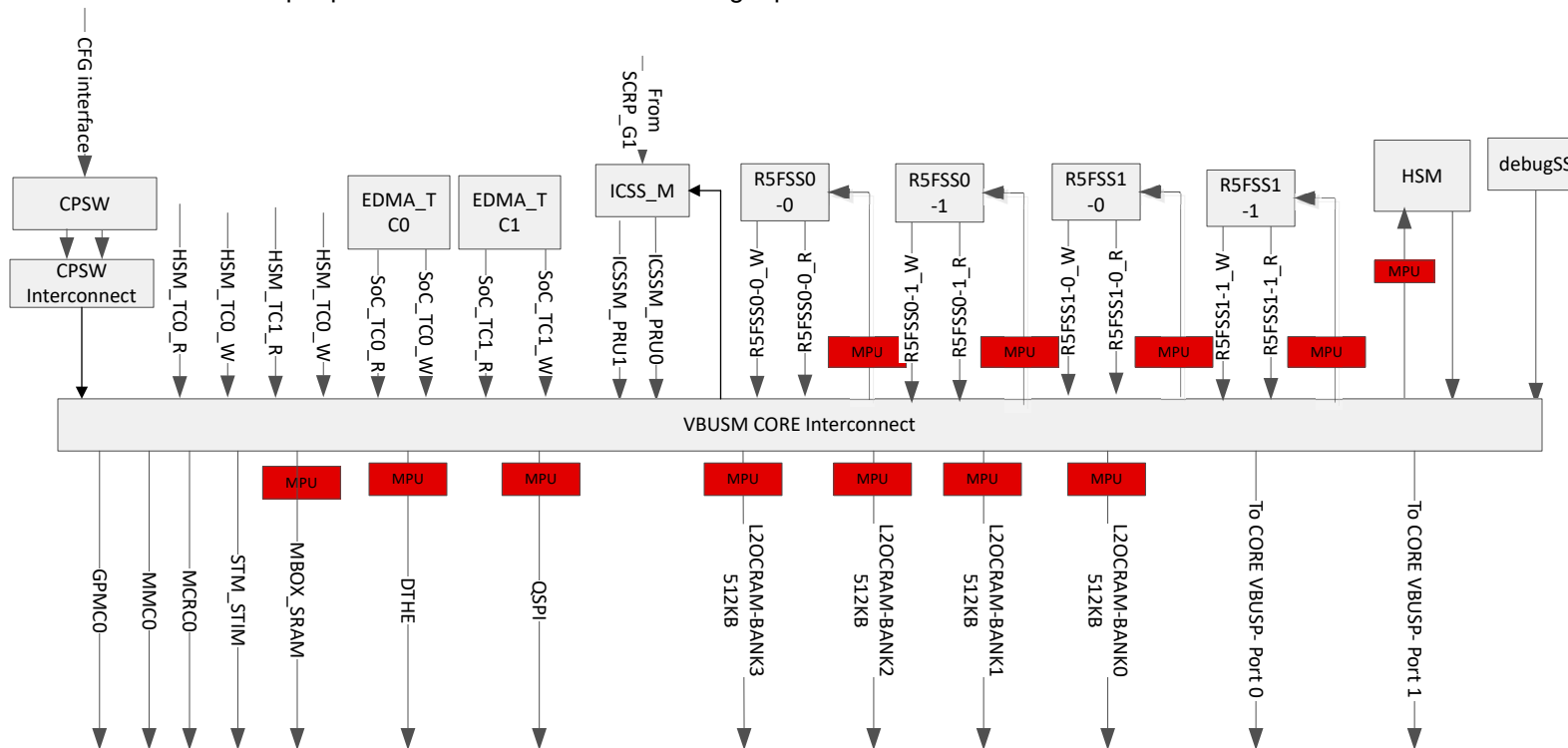
Figure 3-1. Core Interconnect Diagram
