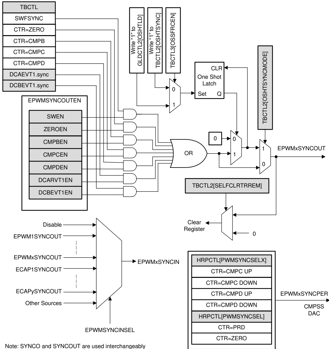
Figure 7-117. Time-Base Counter Synchronization Scheme
