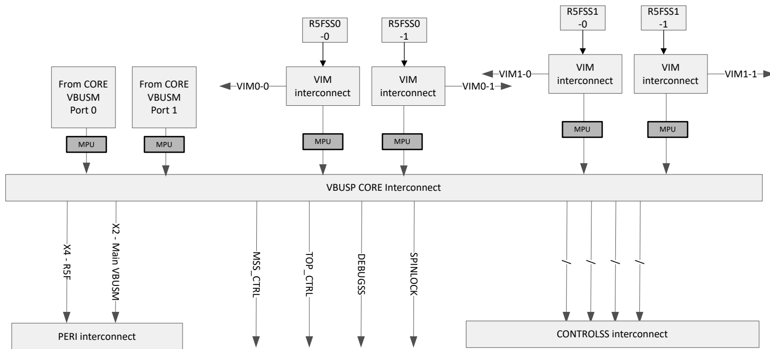
Figure 3-2. CORE VBUSP Interconnect Diagram
