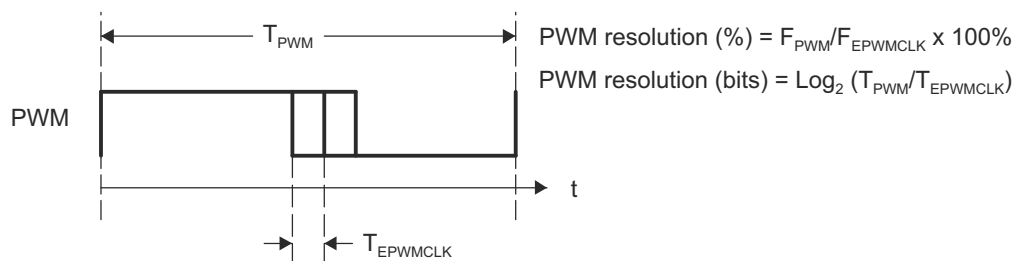
Figure 7-178. Resolution Calculations for Conventionally Generated PWM
