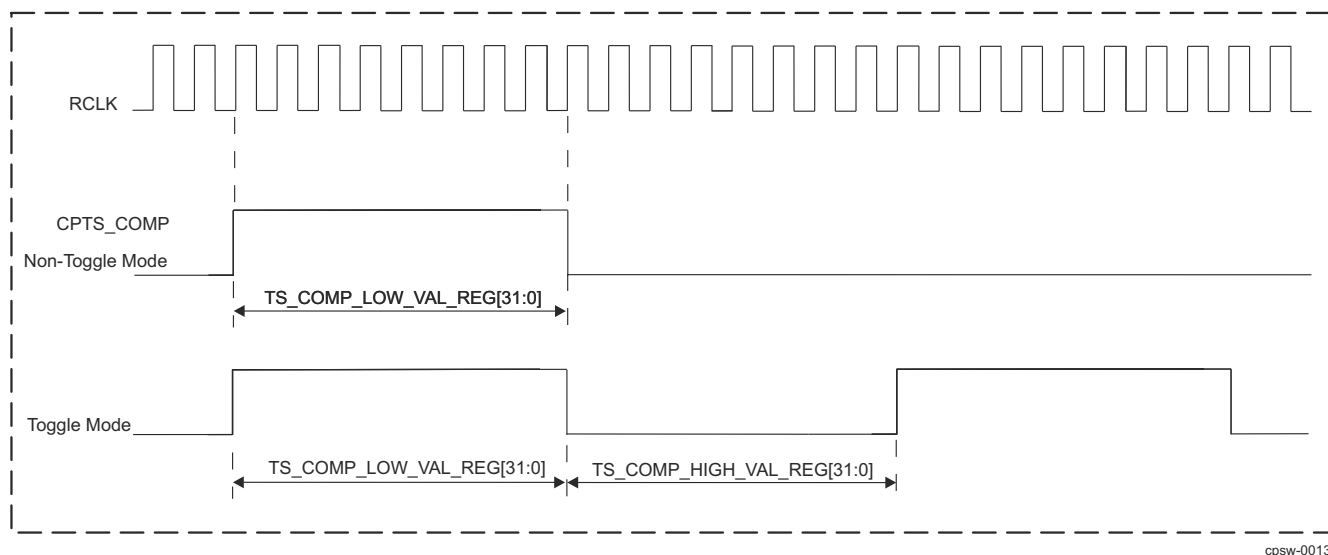
Figure 13-107. CPTS_COMP Output in Toggle and Non-Toggle Mode
