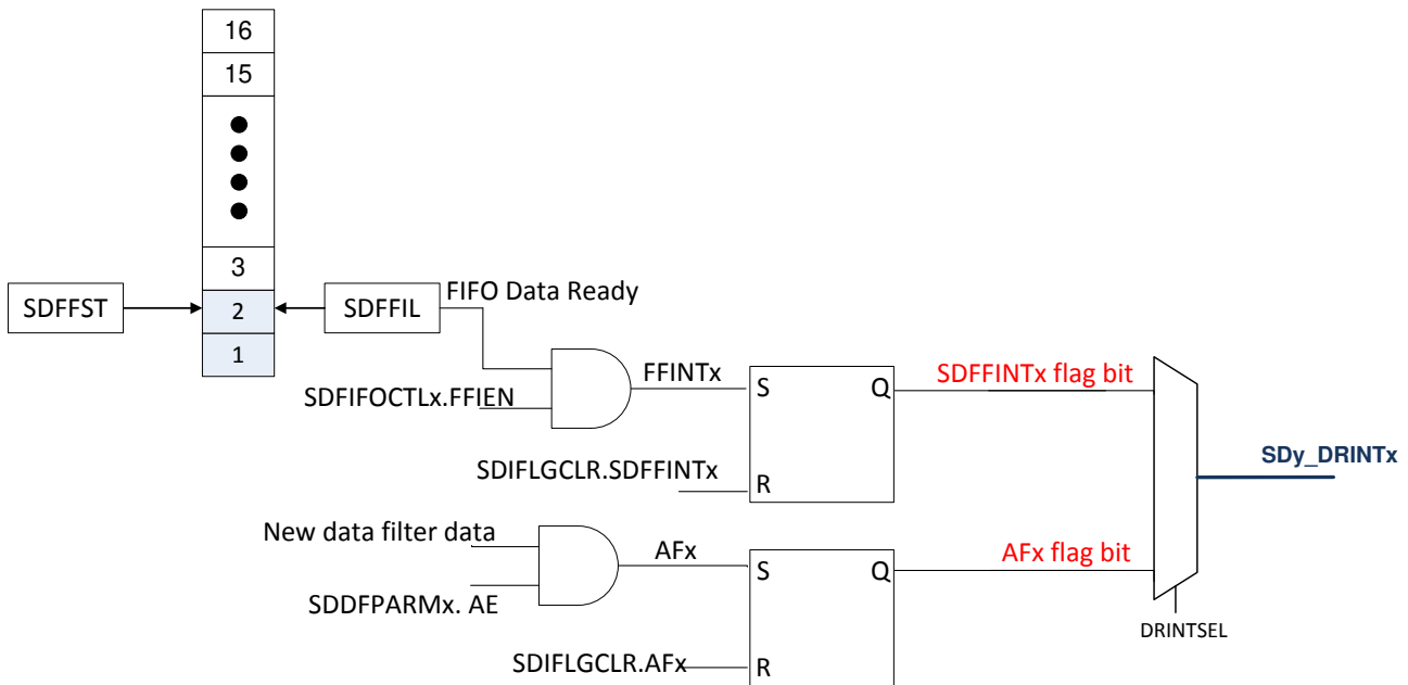
Figure 7-259. SDFM Data Ready (SDy_DRINTx) Interrupt
