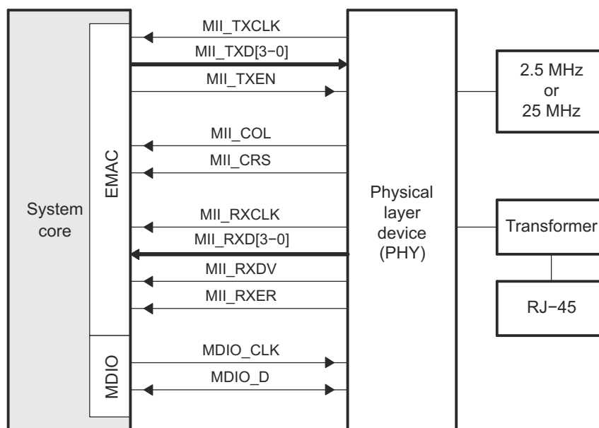
Figure 13-93. Ethernet Configuration—MII Connections
