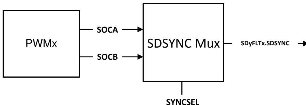
Figure 7-255. SDSYNC Event
