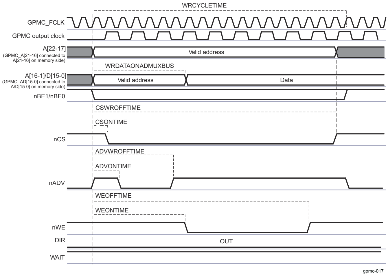
Figure 13-147. Synchronous Single Write on an Address/Data-Multiplexed Device
