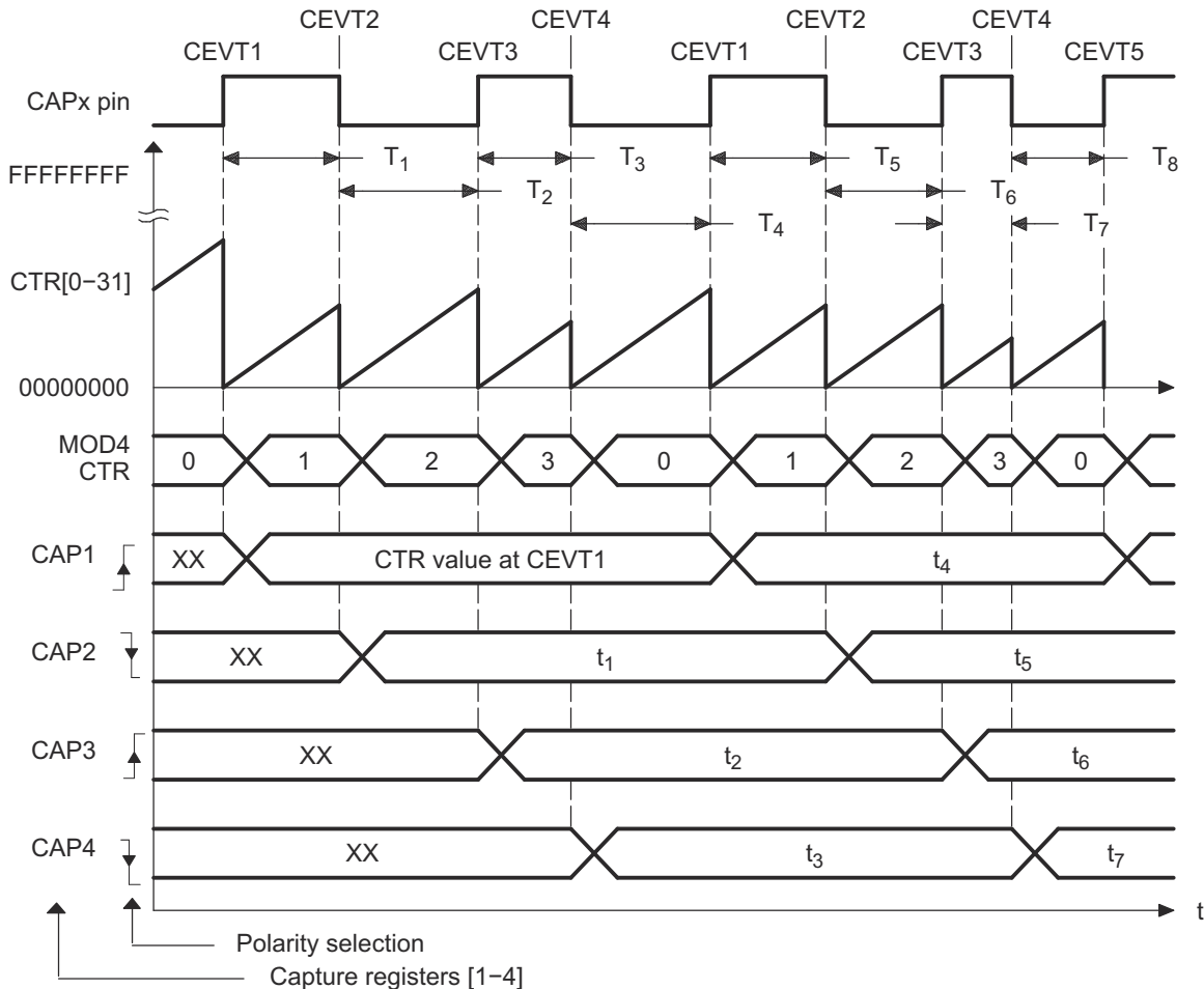
Figure 7-207. Capture Sequence for Delta Mode Time-stamp With Rising and Falling Edge Detect
