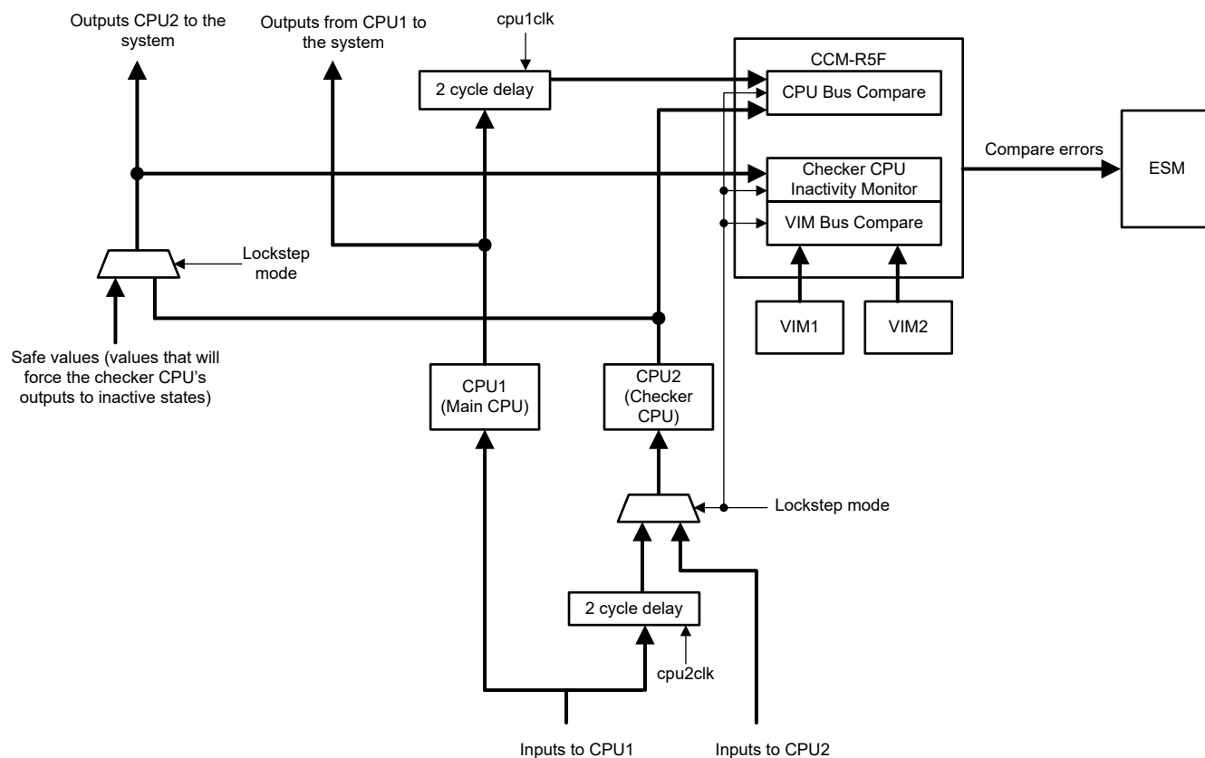
Figure 7-6. Block Diagram
