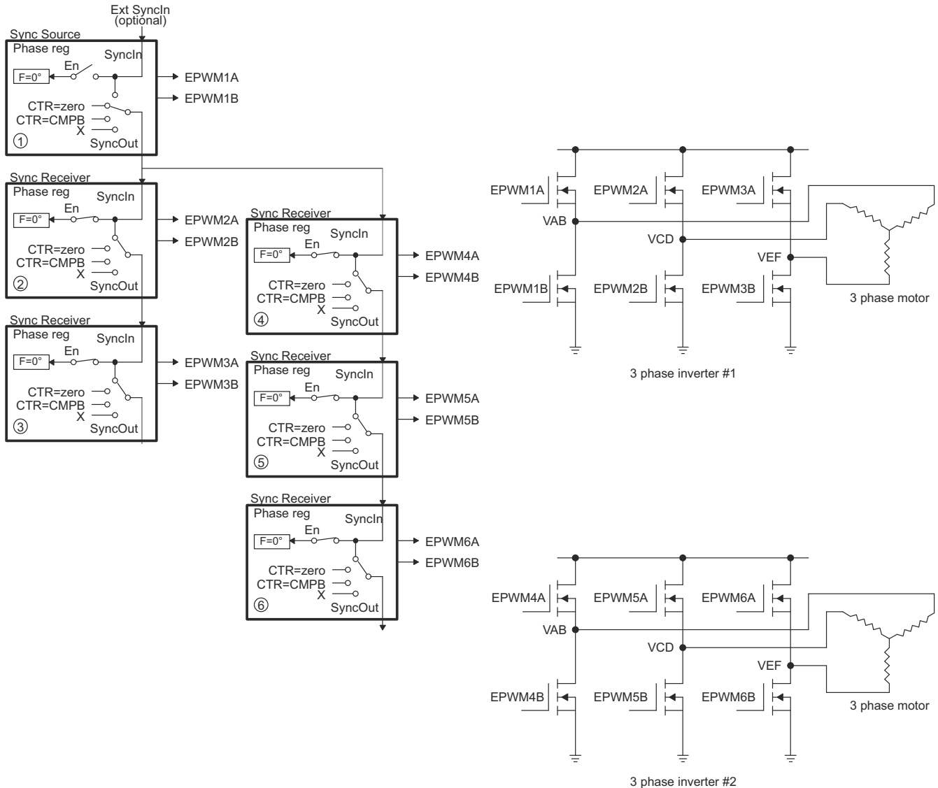
Figure 7-165. Control of Dual 3-Phase Inverter Stages as Is Commonly Used in Motor Control
