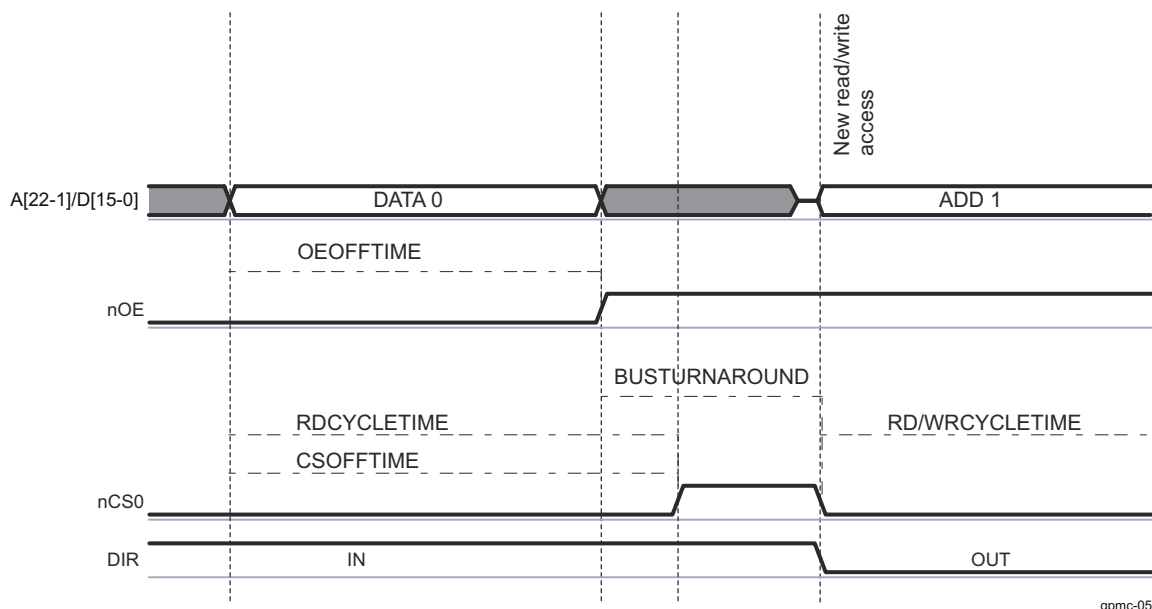
Figure 13-137. Read-to-Read/Write for a Address-Data or AAD-Multiplexed Device, on Same Chip-Select, With Bus Turnaround
