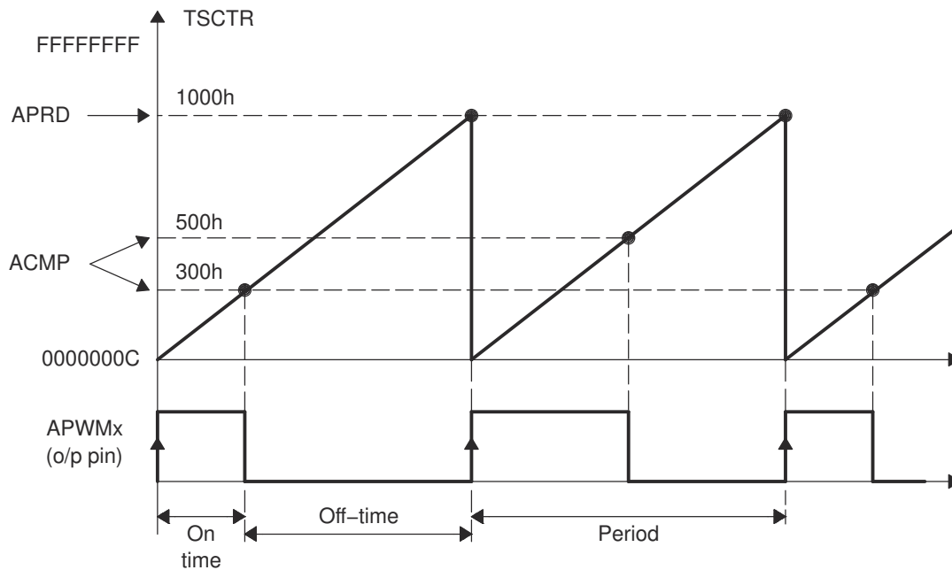
Figure 7-200. PWM Waveform Details Of APWM Mode Operation
