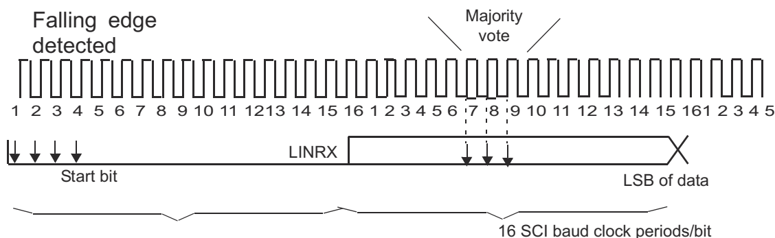
Figure 13-247. Asynchronous Communication Bit Timing
