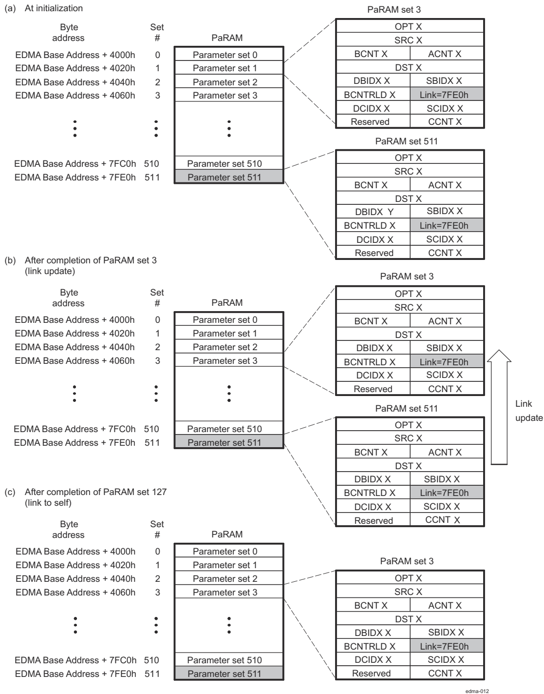
Figure 11-10. Link-to-Self Transfer
