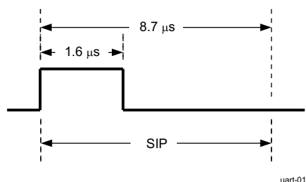
Figure 13-66. SIP
