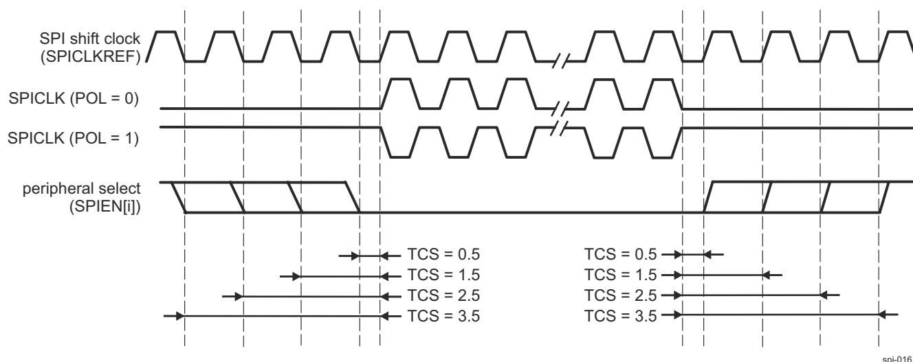
Figure 13-41. CS SPIEN Timing Controls
