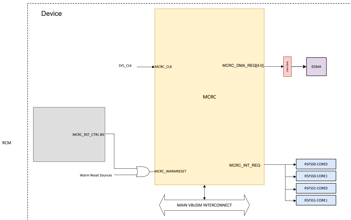
Figure 4-26. MCRC Integration
