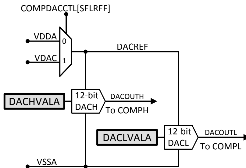
Figure 7-107. Reference DAC Block Diagram
