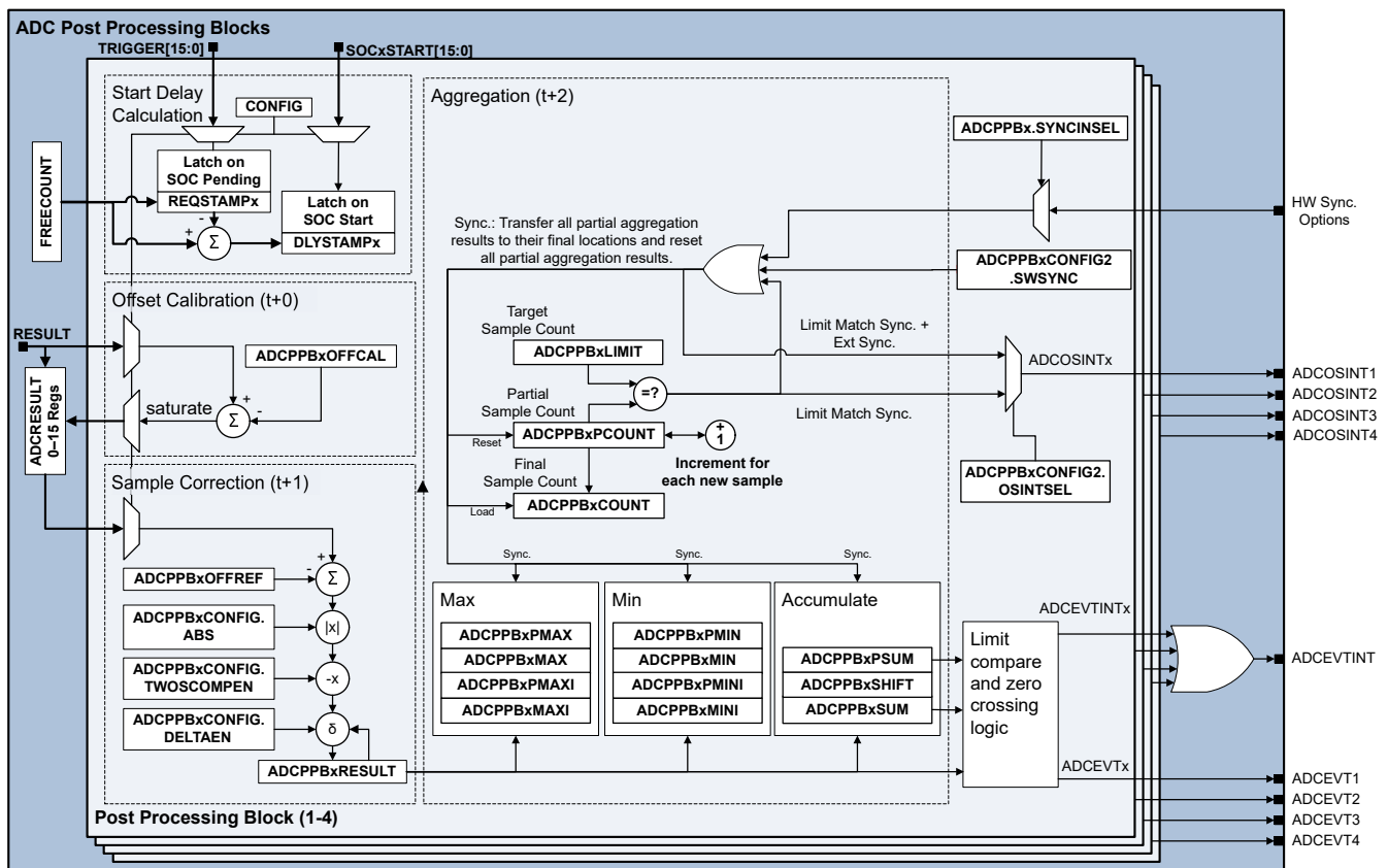
Figure 7-94. ADC PPB Block Diagram
