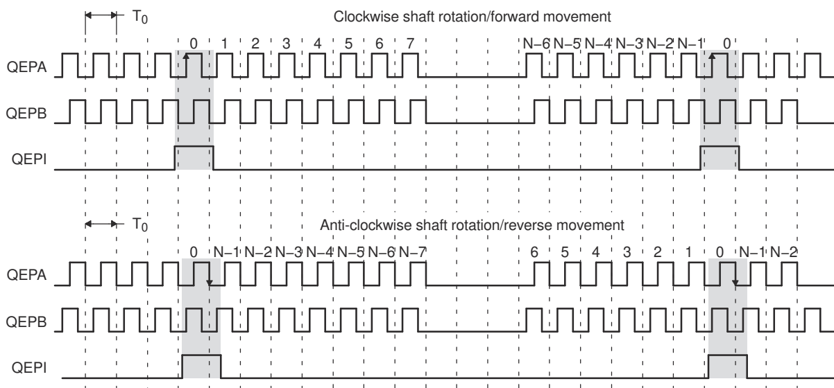
Figure 7-210. QEP Encoder Output Signal for Forward/Reverse Movement
