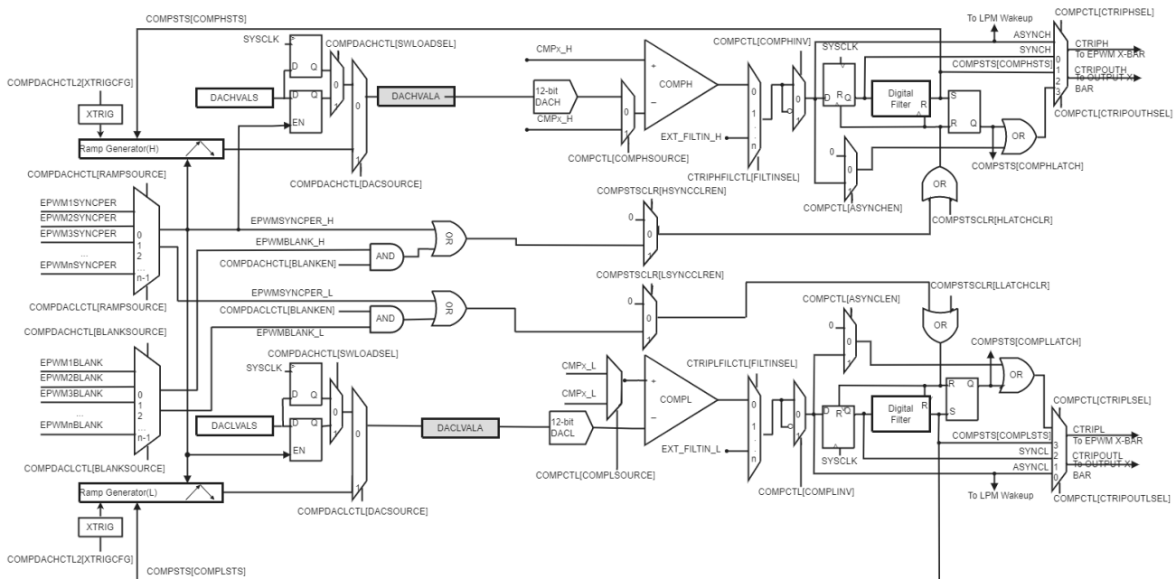
Figure 7-105. CMPSSB Module Block Diagram
