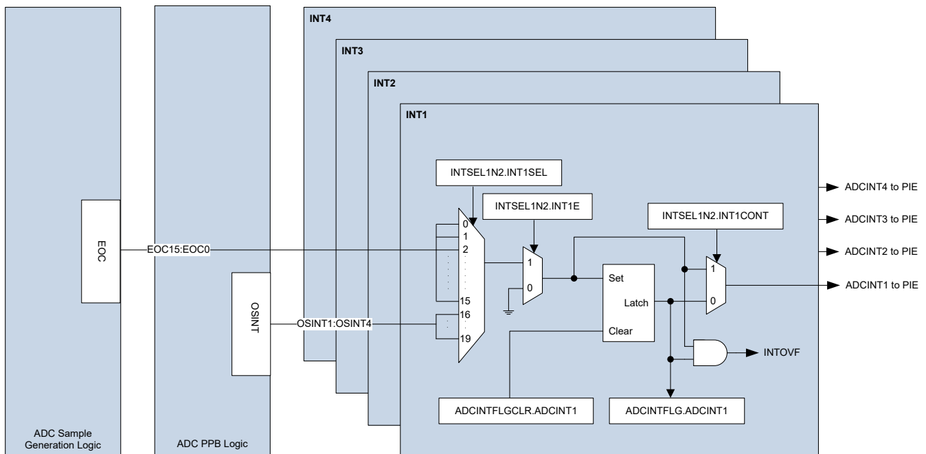
Figure 7-93. ADC EOC Interrupts
