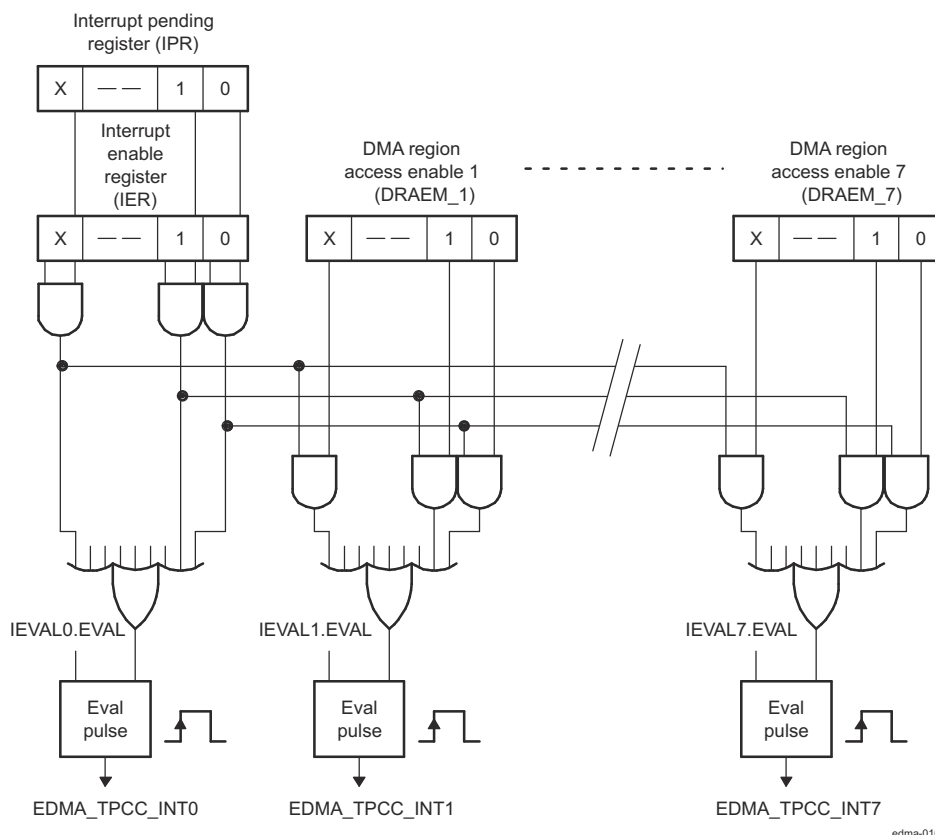
Figure 11-14. Interrupt Diagram
