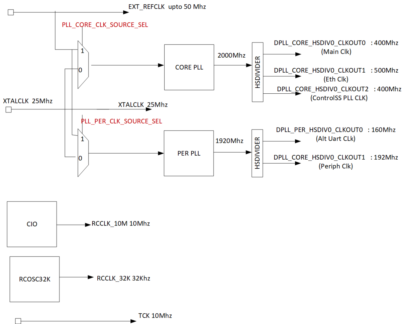
Figure 6-18. Root Clocks
