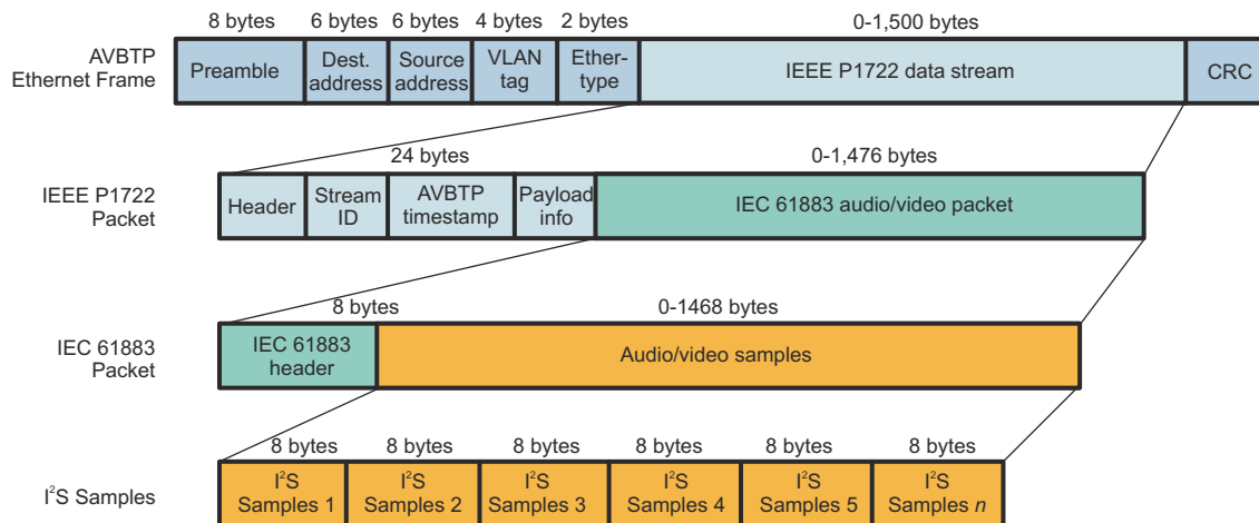
Figure 13-103. IEEE 1722 Packets
