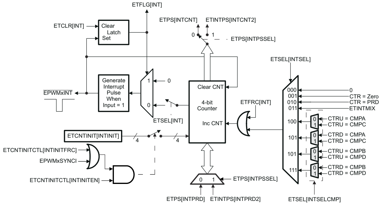
Figure 7-153. Event-Trigger Interrupt Generator
