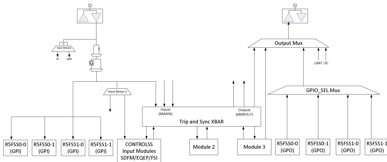
Figure 4-12. GPIO Mux Diagram
