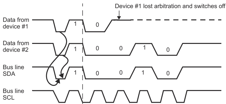
Figure 13-16. Arbitration Procedure Between Two Master Transmitters
