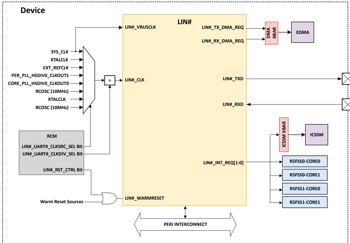
Figure 4-20. LIN Integration
