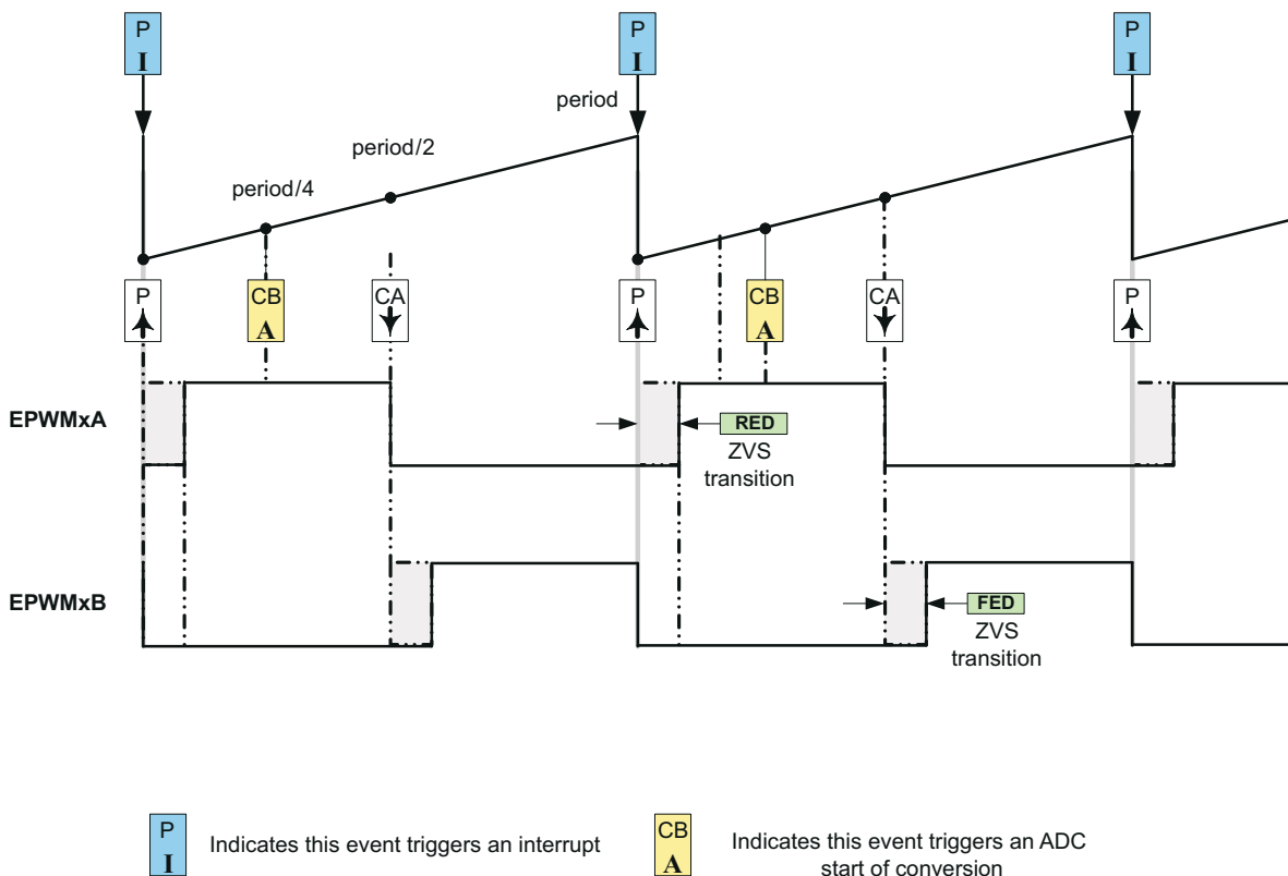
Figure 7-176. H-Bridge LLC Resonant Converter PWM Waveforms
