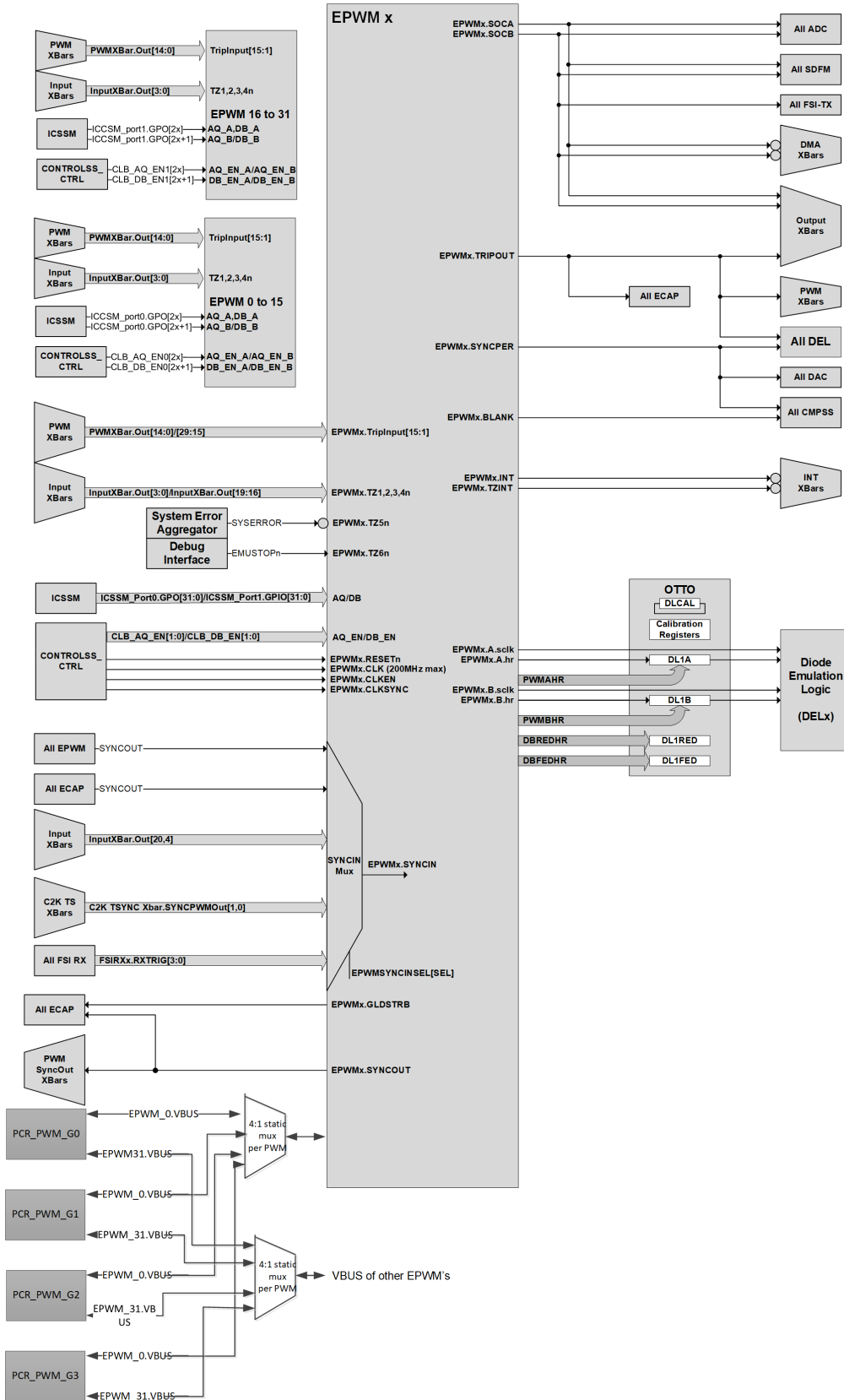
Figure 7-114. EPWM Integration Diagram
