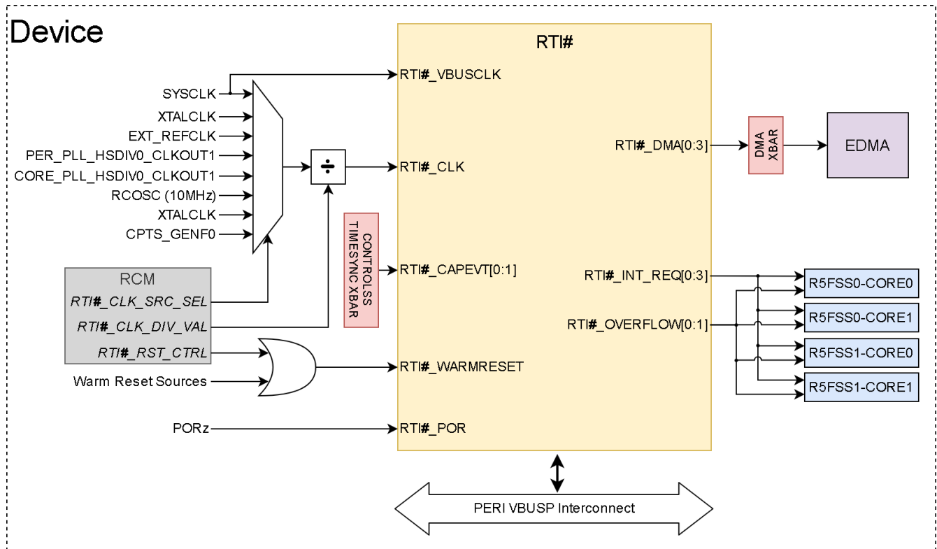
Figure 4-21. RTI Integration
