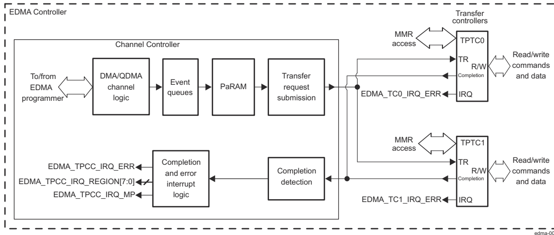
Figure 11-2. EDMA Controller Block Diagram
