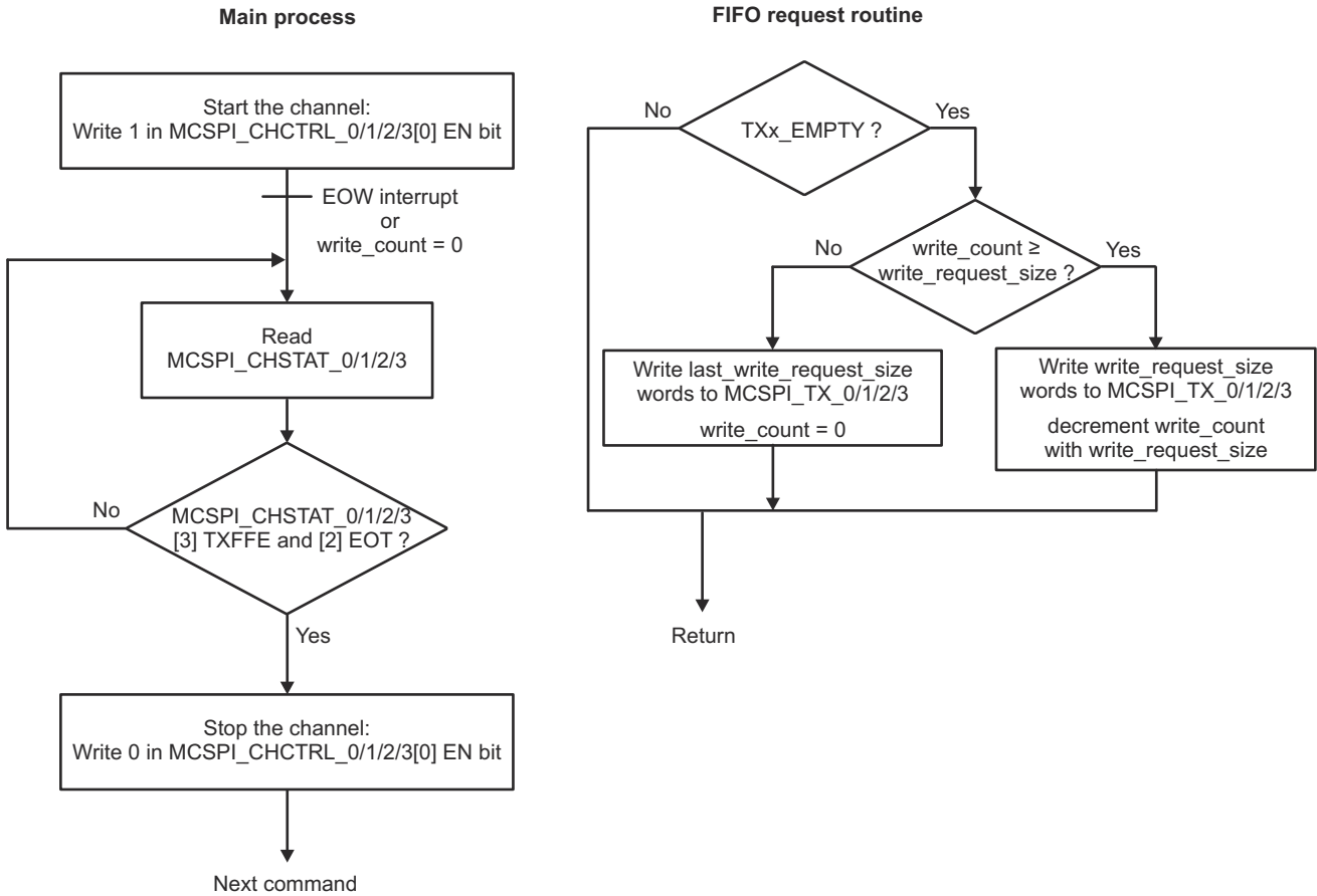
Figure 13-53. FIFO Mode Transmit-Only (Controller)
