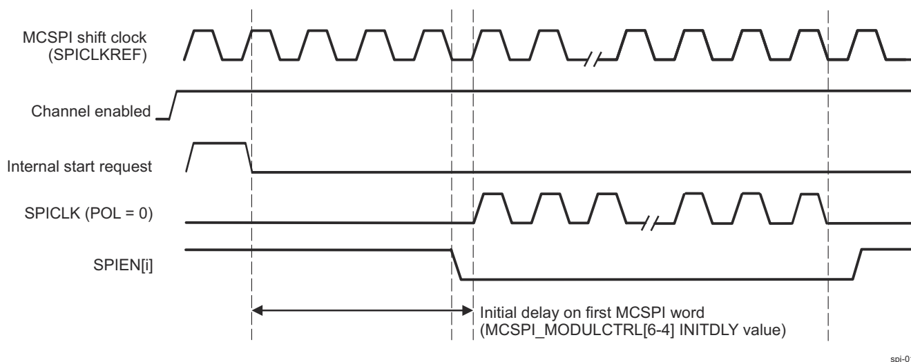
Figure 13-50. Controller Single Channel Initial Delay
