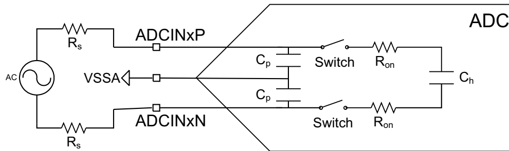
Figure 7-89. Differential Input Model
