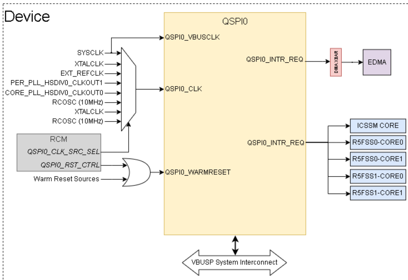
Figure 13-217. QSPI Integration Diagram
