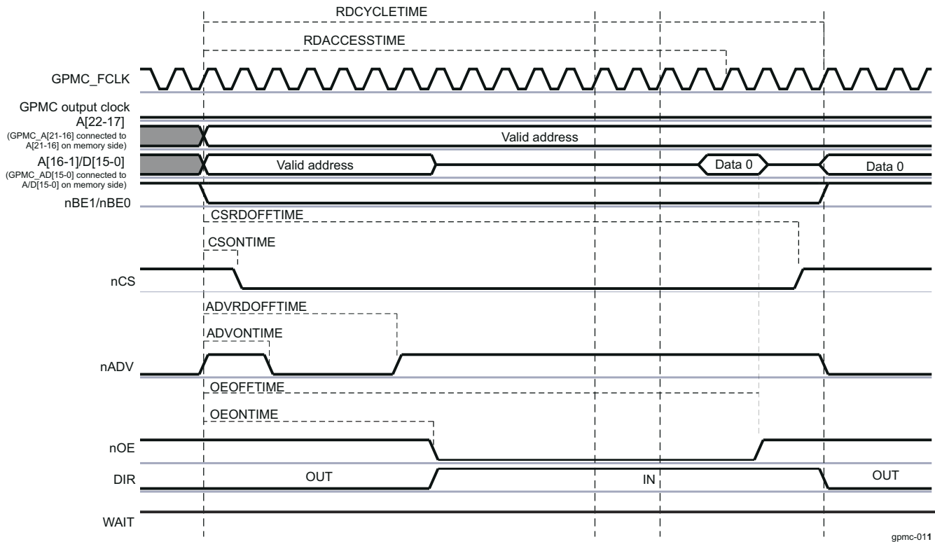
Figure 13-138. Asynchronous Single Read on an Address/Data-Multiplexed Device
