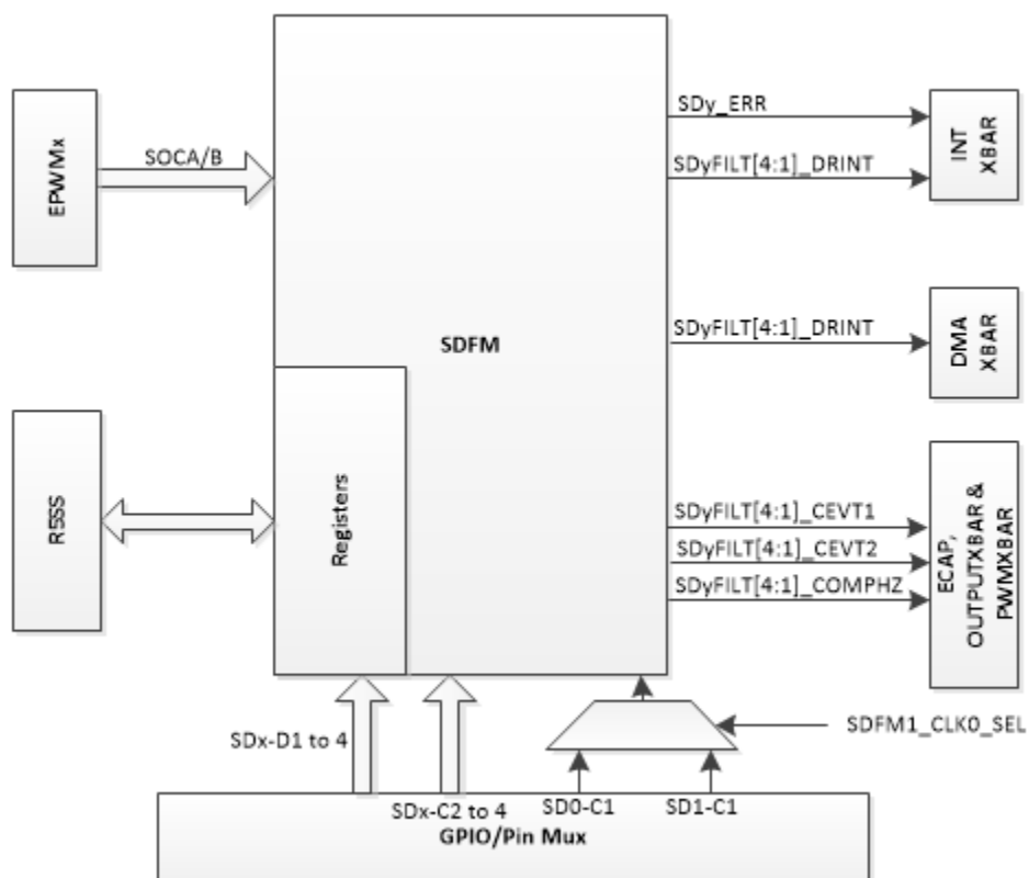
Figure 7-244. Sigma Delta Filter Module (SDFM) CPU Interface
