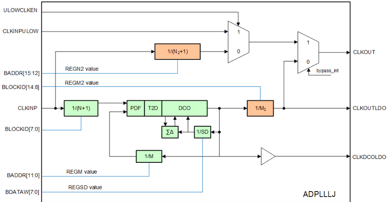
Figure 6-20. ADPLLJ Architecture
