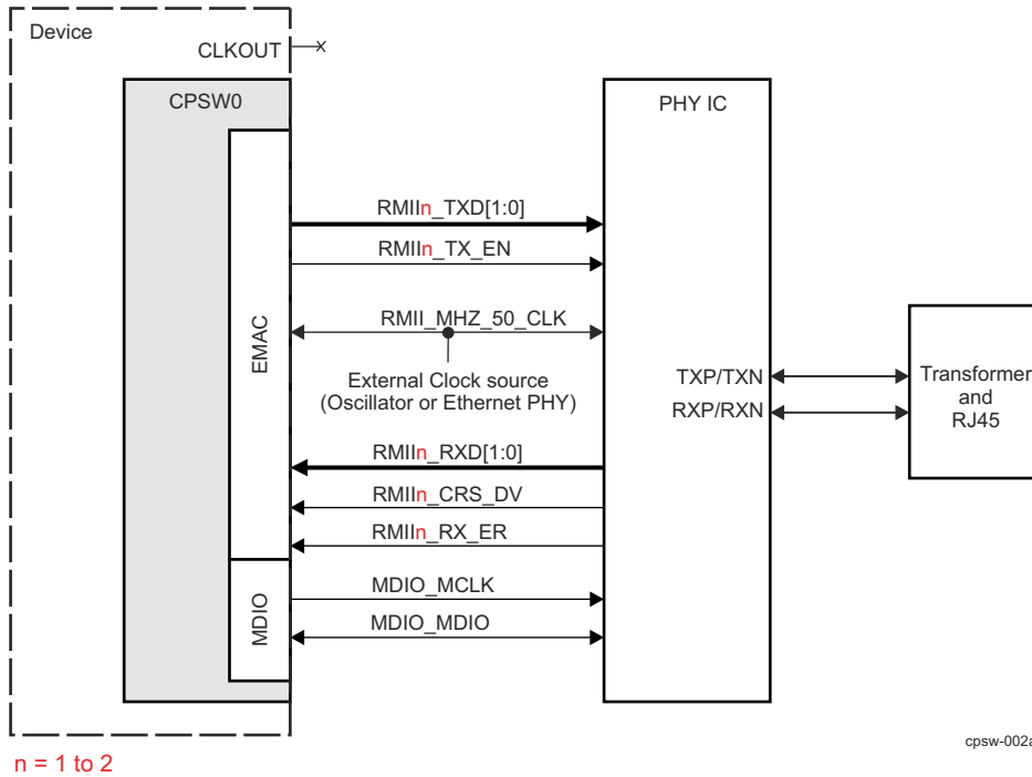
Figure 13-95. RMIi Interface Typical Application (External Clock Source)
