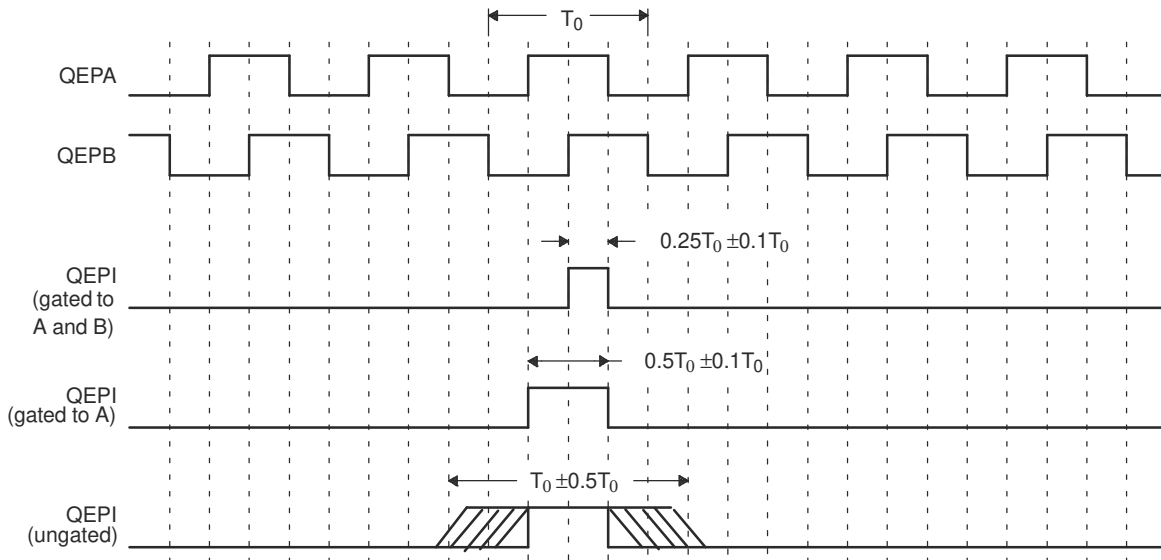
Figure 7-211. Index Pulse Example
