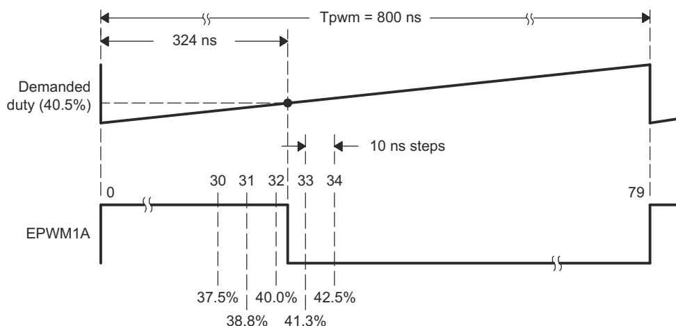
Figure 7-181. Required PWM Waveform for a Requested Duty = 40.5%
