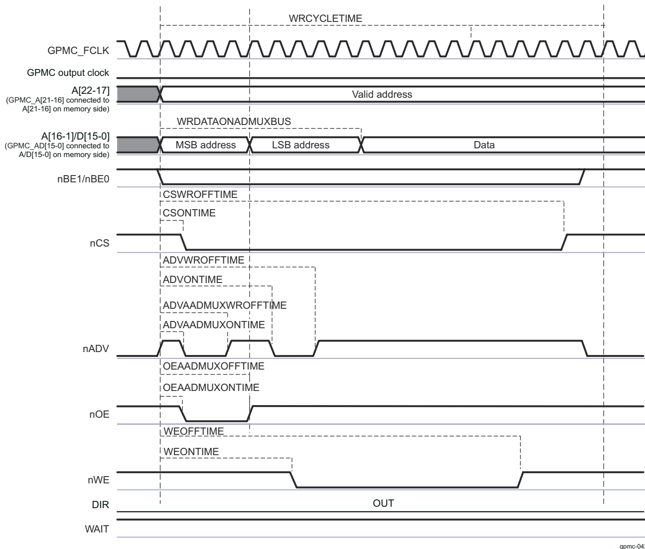
Figure 13-142. Asynchronous Single Write on an AAD-Multiplexed Device
