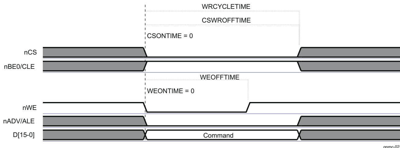
Figure 13-153. NAND Command Latch Cycle
