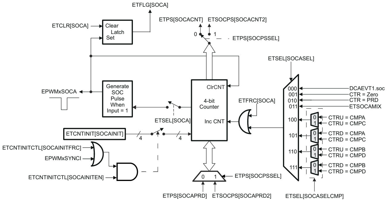
Figure 7-154. Event-Trigger SOCA Pulse Generator
