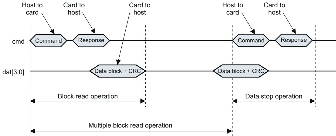
Figure 13-186. Multiple Block Read Operation (MMC Cards Only)
