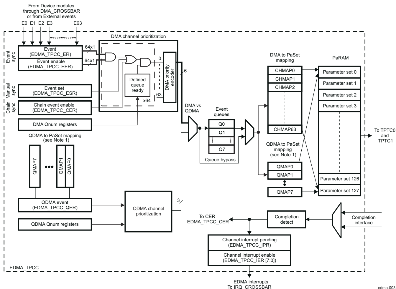
Figure 11-3. EDMA Channel Controller Block Diagram
