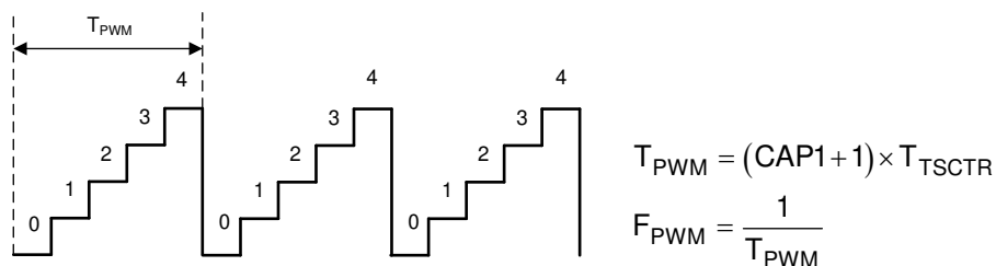
Figure 7-201. Time-Base Frequency and Period Calculation
