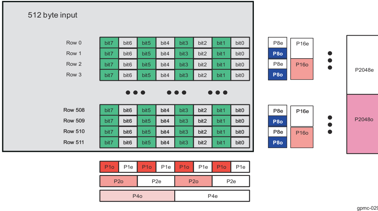
Figure 13-160. ECC Computation for a 512-Byte Data Stream (Read or Write)
