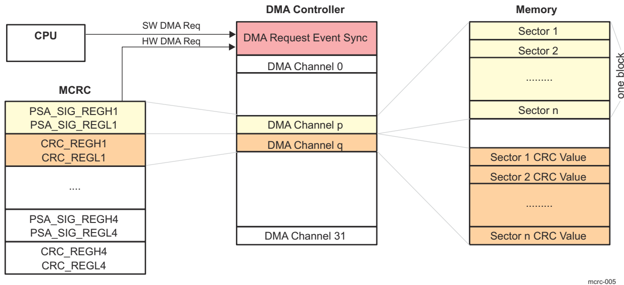
Figure 13-301. AUTO Mode With Software CPU Trigger
