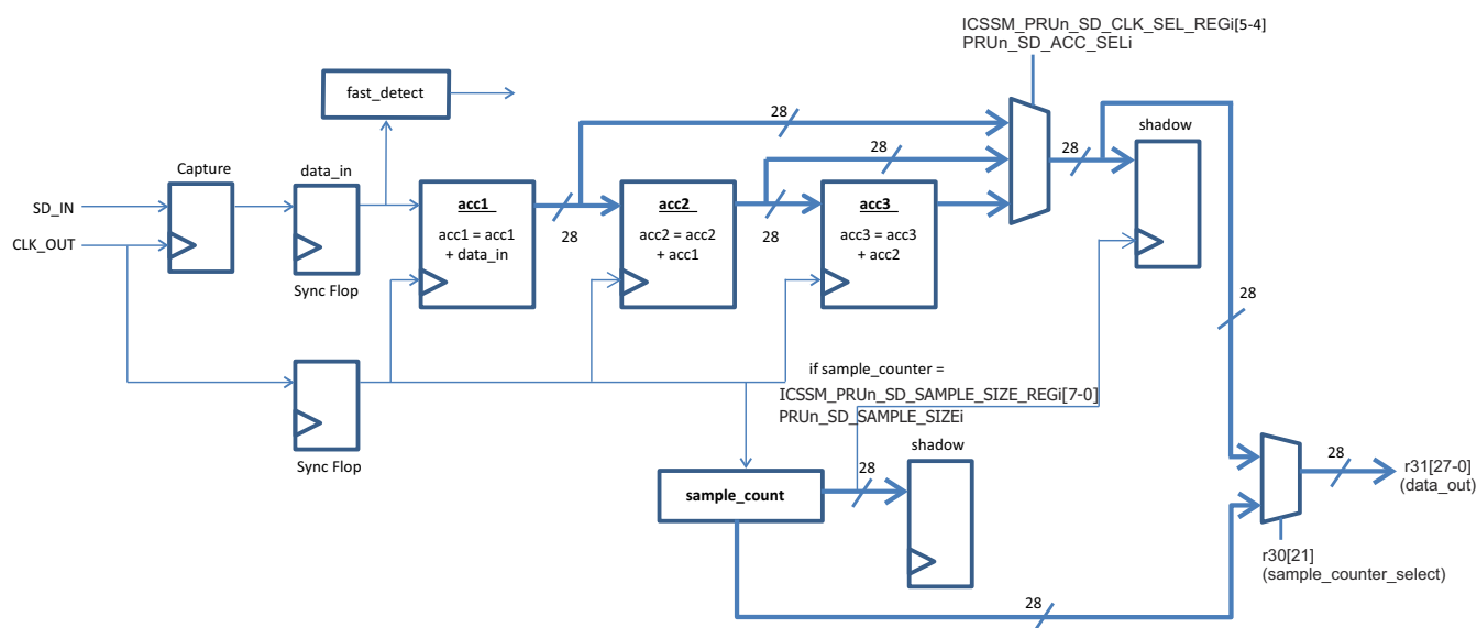
Figure 7-31. Sigma Delta Hardware Integrators Block Diagram (snoop = 1)
