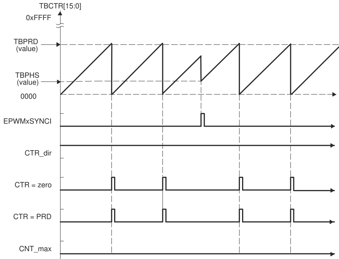
Figure 7-119. Time-Base Up-Count Mode Waveforms
