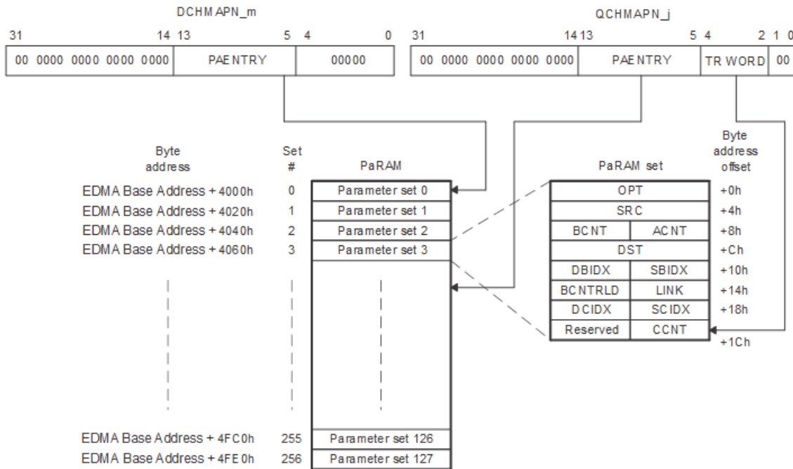
Figure 11-8. PaRAM Set
