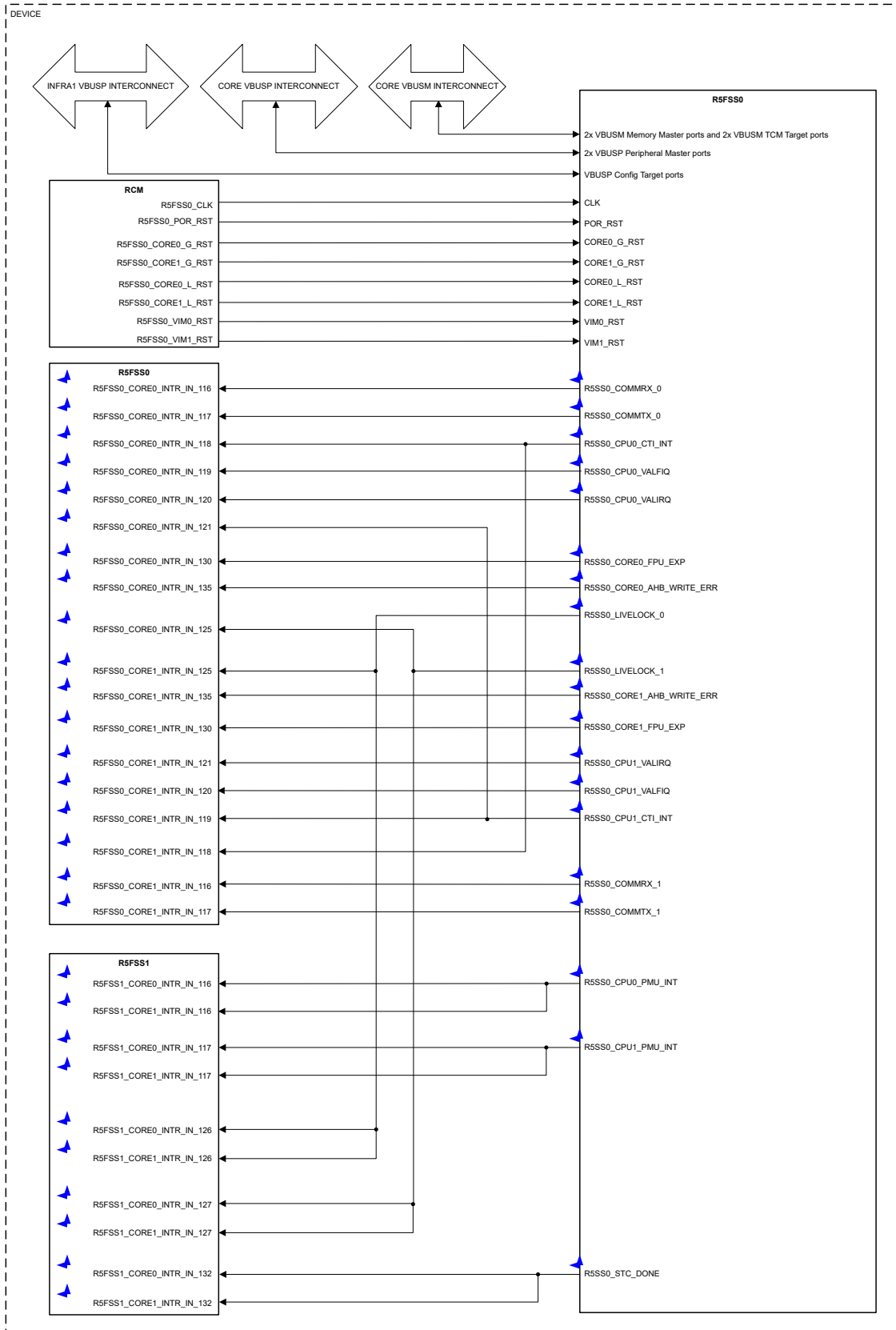
Figure 7-1. R5FSS0 Integration Diagram
