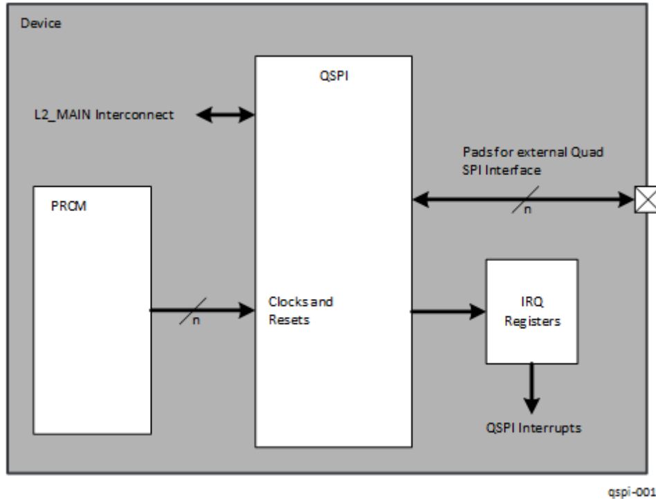
Figure 13-215. QSPI Overview
