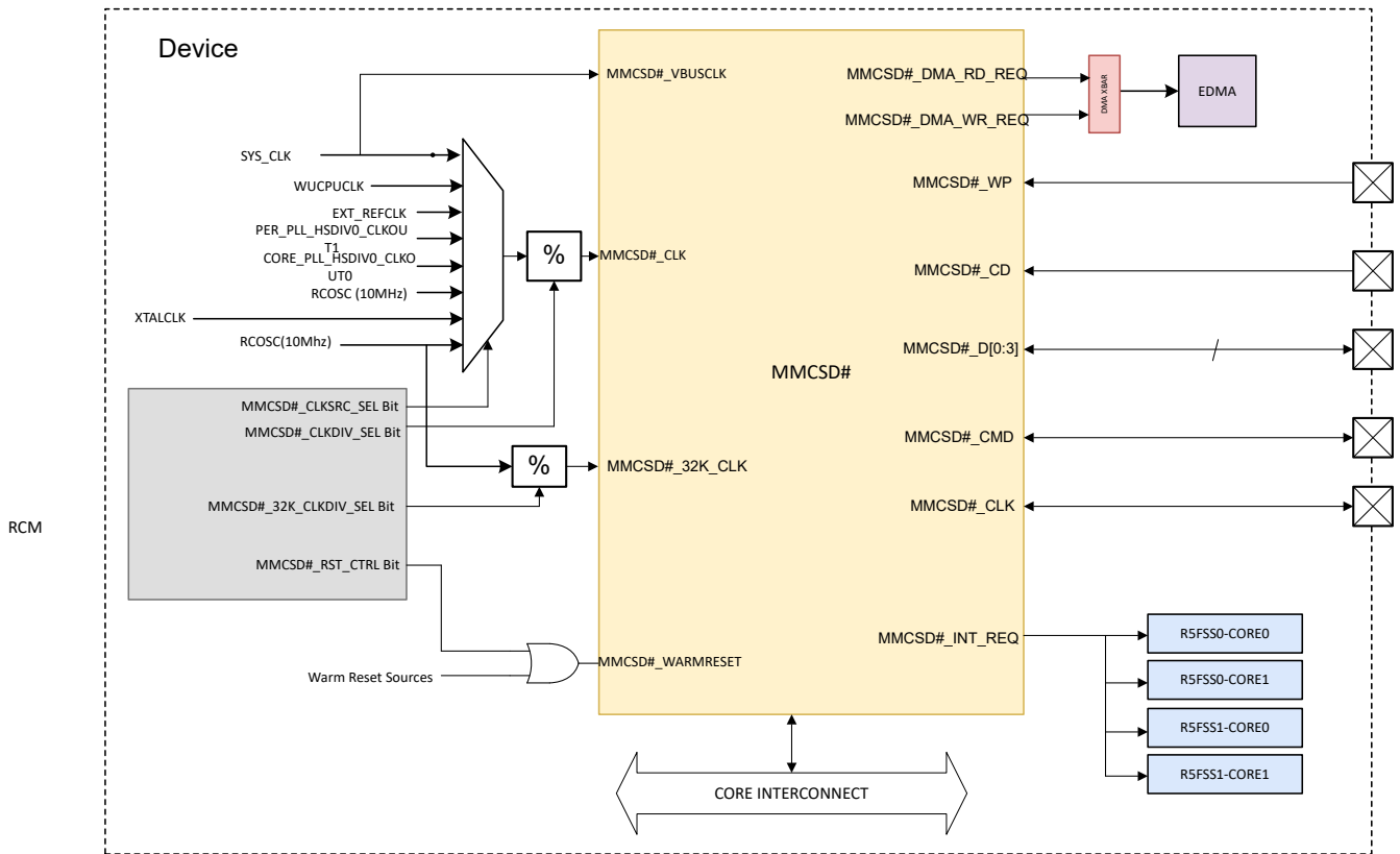
Figure 4-17. MMCSD Integration
