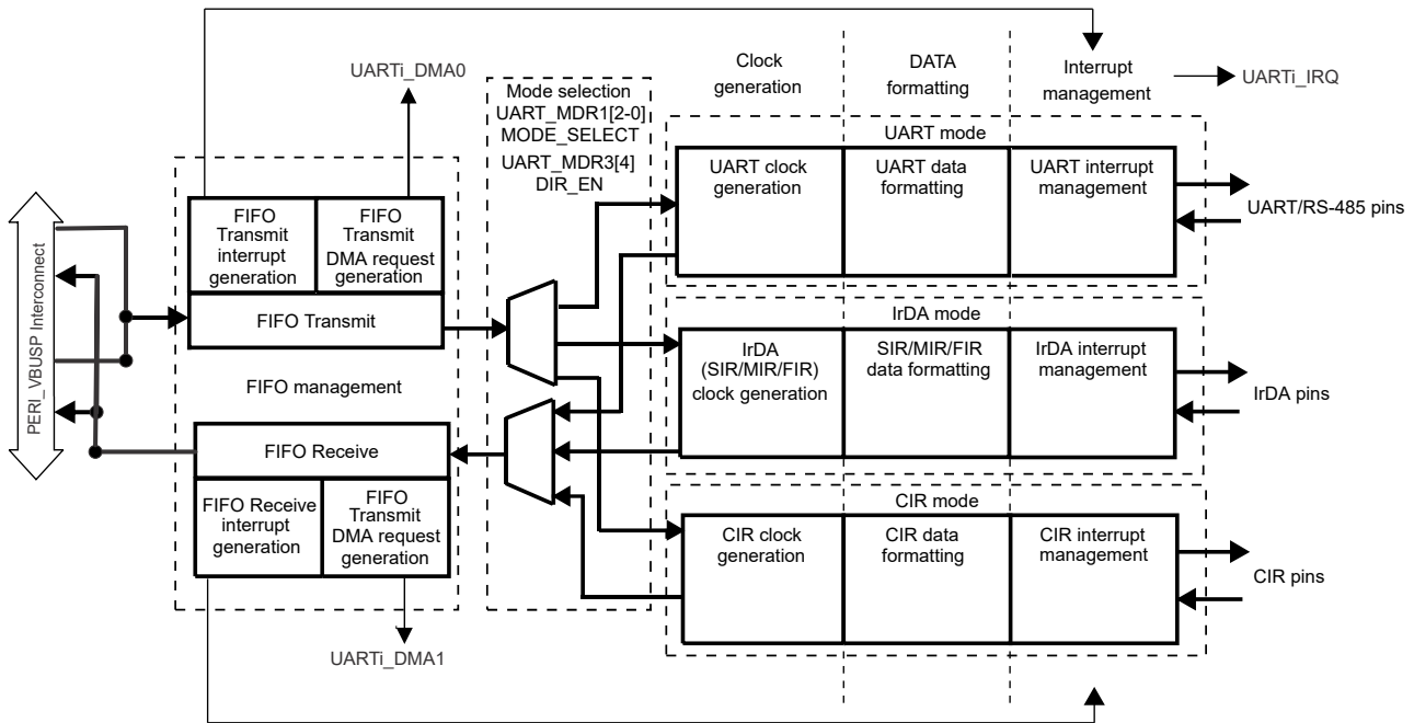
Figure 13-77. UART Functional Block Diagram
