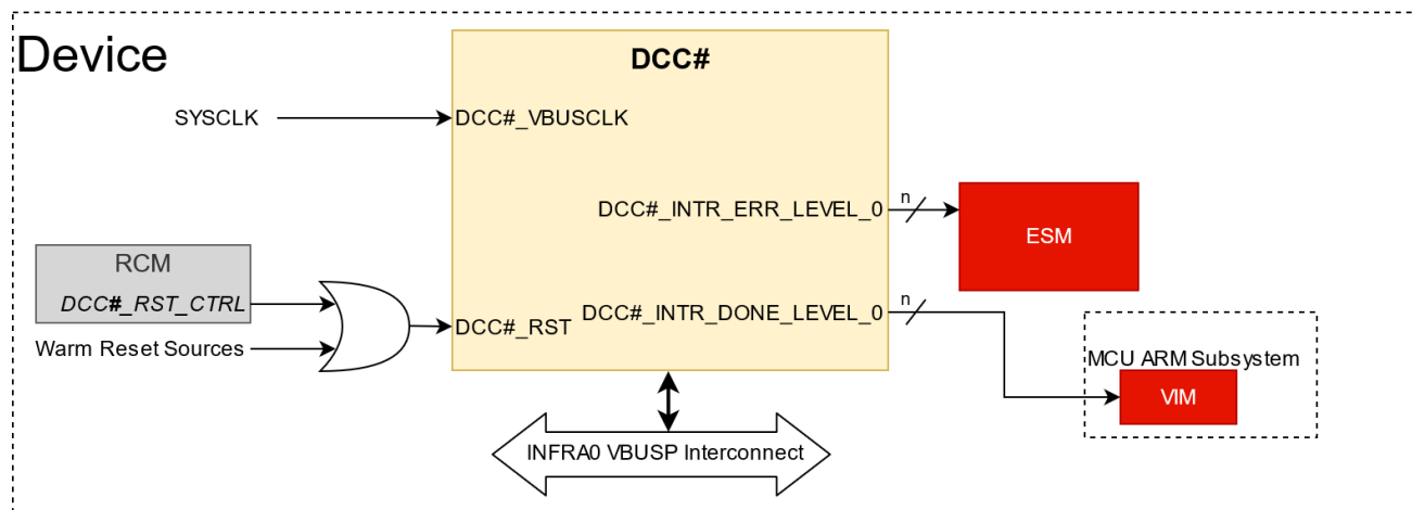
Figure 13-279. DCC Integration Diagram
