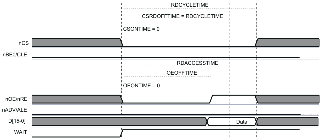
Figure 13-155. NAND Data Read Cycle
