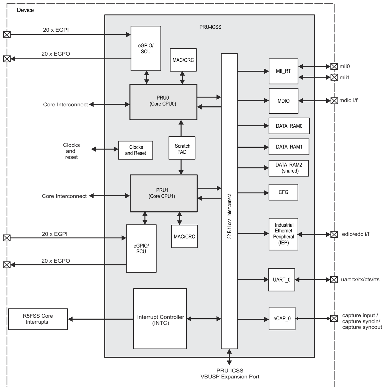
Figure 7-15. PRU-ICSS Overview
