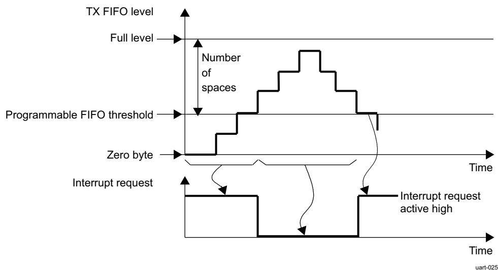
Figure 13-80. UART TX FIFO Interrupt Request Generation
