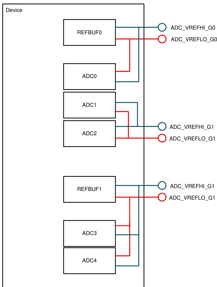
Figure 7-86. ADC Reference Connectivity Diagram
