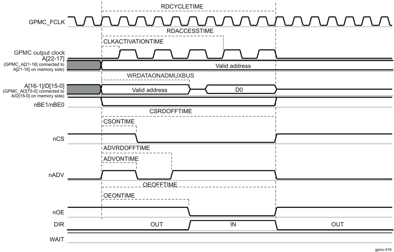
Figure 13-144. Synchronous Single Read (GPMCFCLKDIVIDER = 1)
