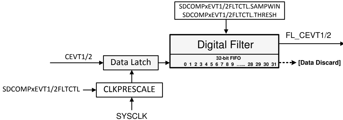
Figure 7-257. Digital Filter
