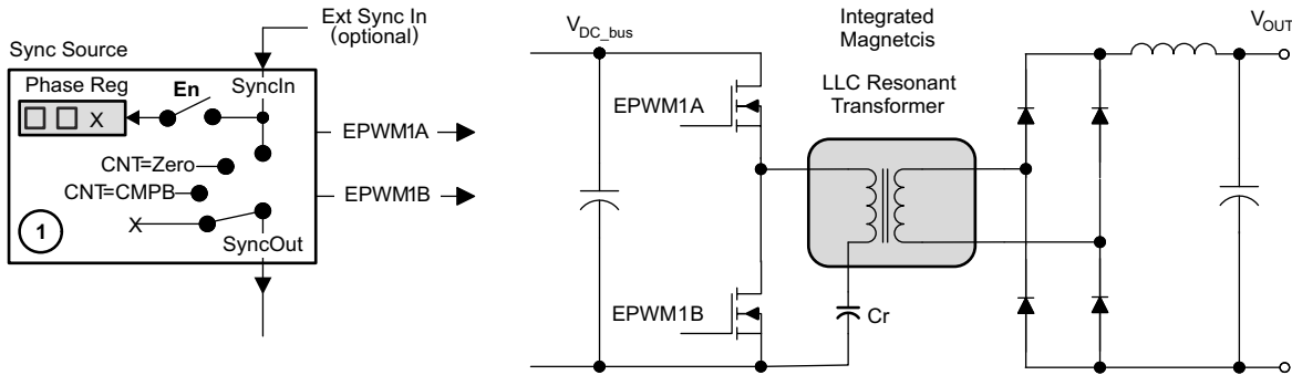
Figure 7-175. Control of Two Resonant Converter Stages
