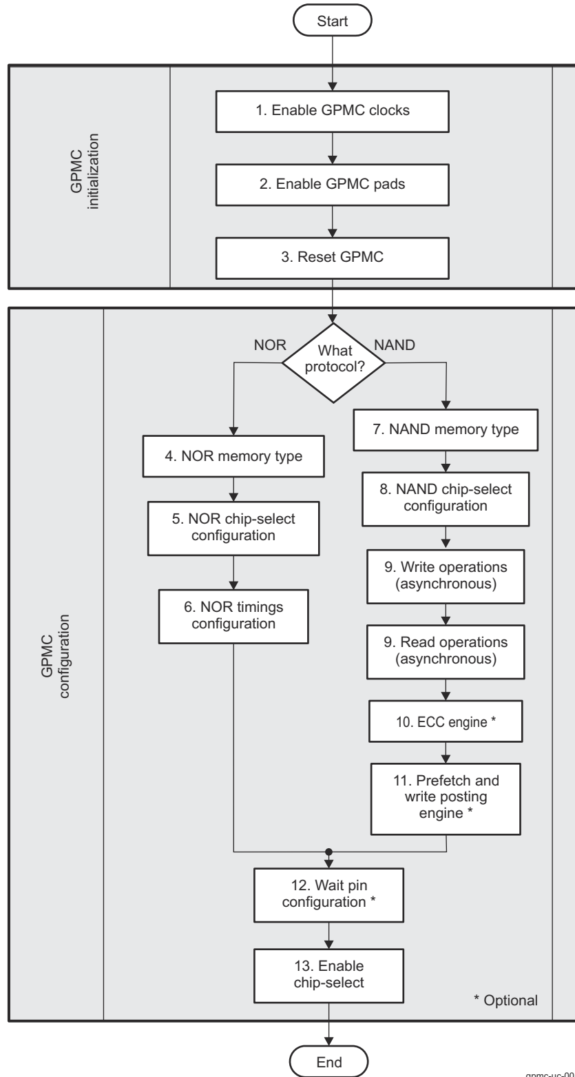
Figure 13-172. Programming Model Top-Level Diagram
