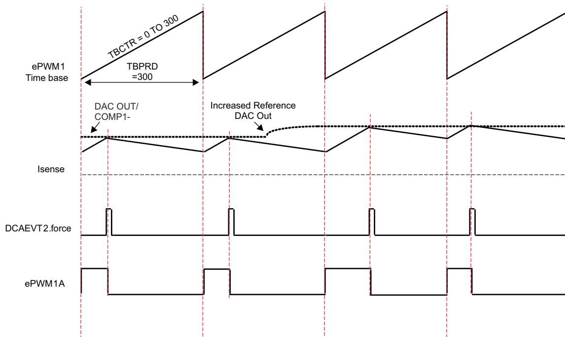
Figure 7-174. Peak Current Mode Control Waveforms for Control of Buck Converter
