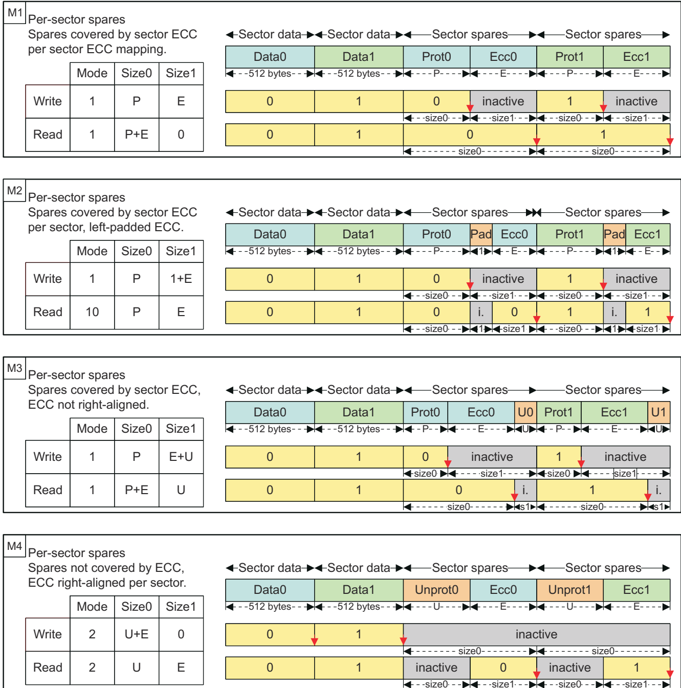
Figure 13-164. NAND Page Mapping and ECC: Per-Sector Schemes
