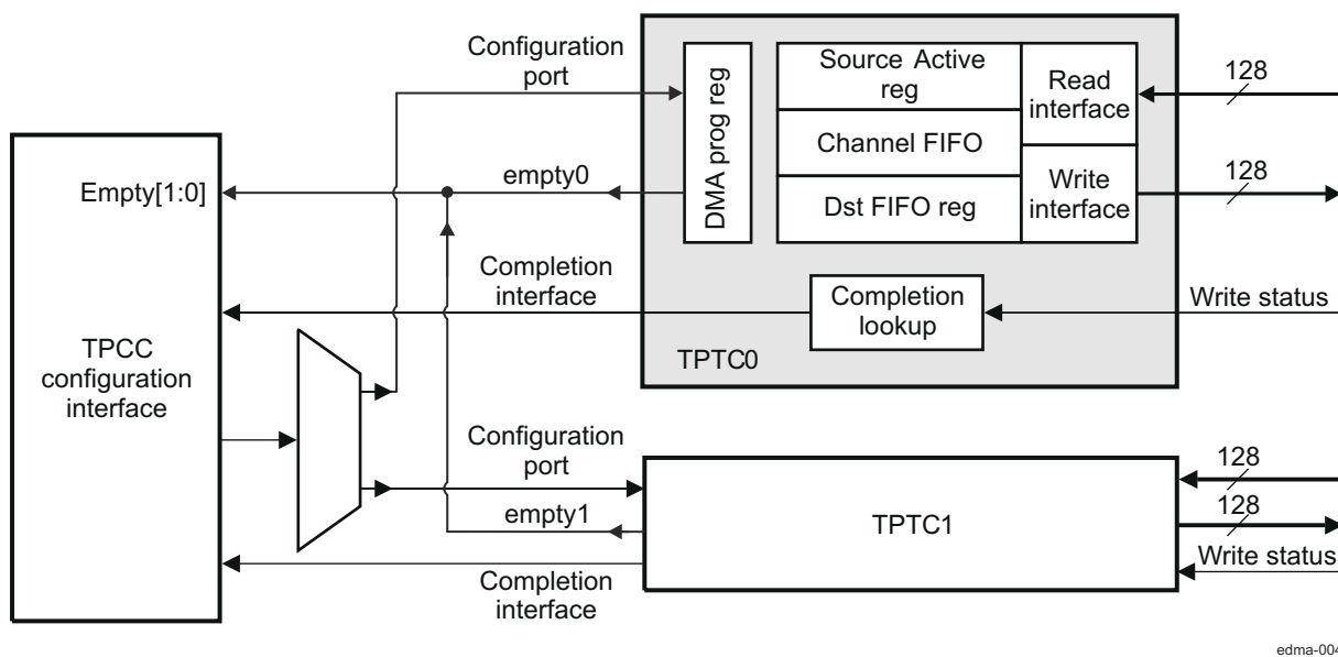
Figure 11-4. TPTC Block Diagram
