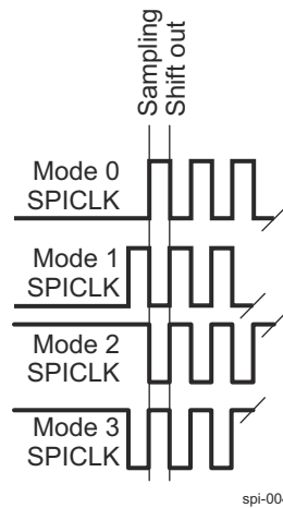
Figure 13-29. Phase and Polarity Combinations
