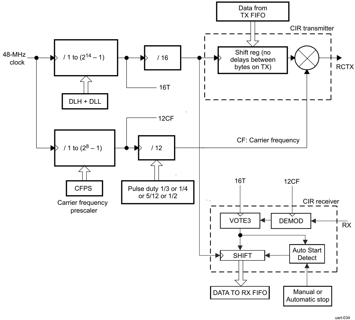
Figure 13-91. CIR Mode Block Components
