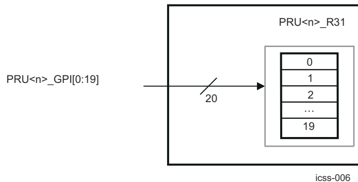
Figure 7-24. PRU R31 (EGPI) Direct Input Mode Block Diagram
