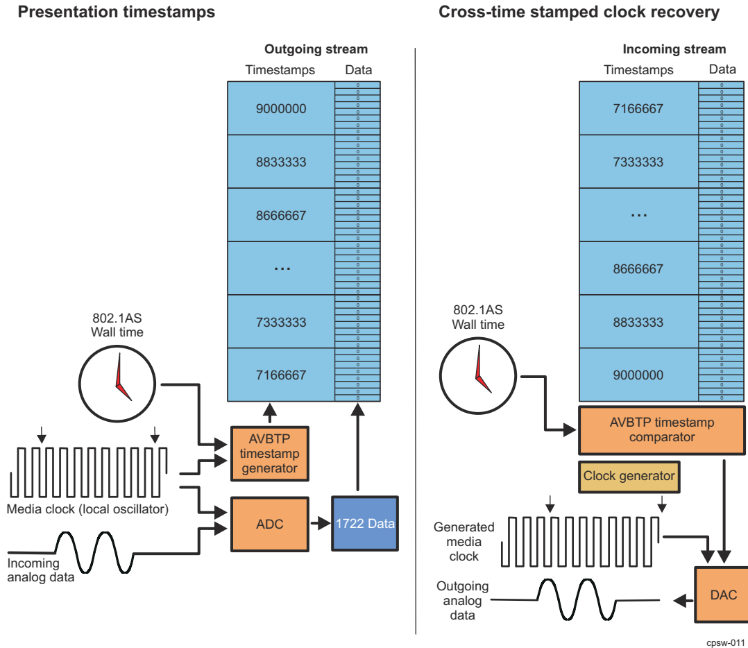
Figure 13-104. Cross Time Stamping and Presentation Timestamps
