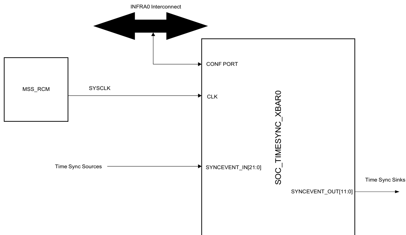
Figure 4-9. SOC_TIMESYNC_XBAR0 Integration
