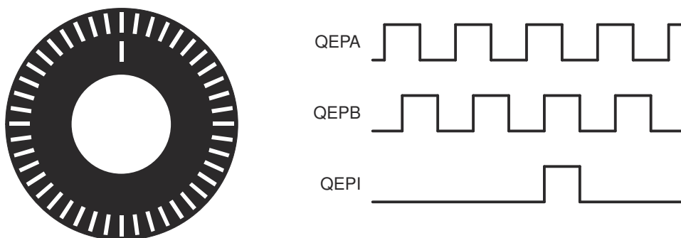
Figure 7-209. Optical Encoder Disk
