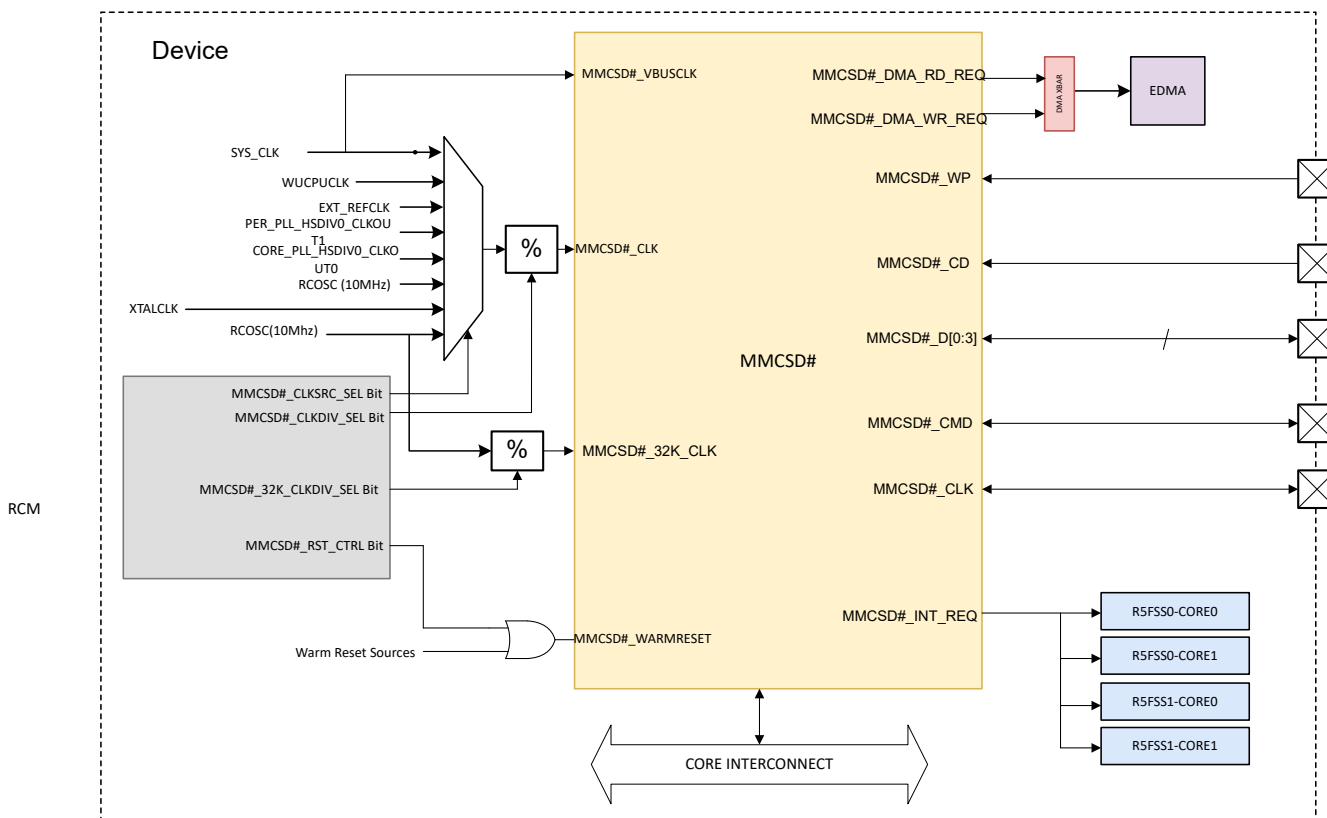
Figure 13-181. MMCSD Integration
