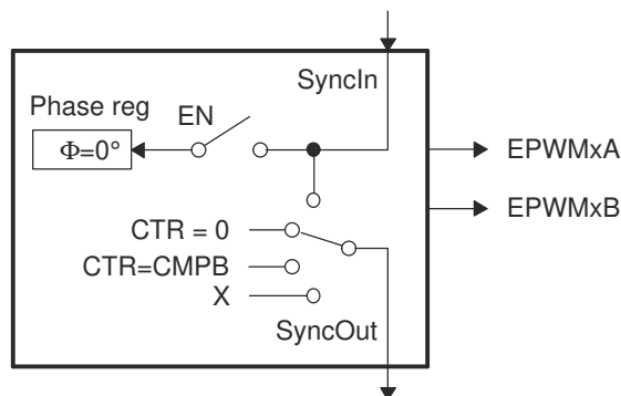
Figure 7-157. Simplified ePWM Module
