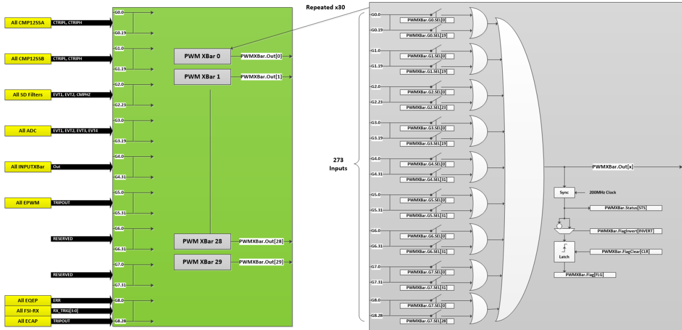
Figure 7-261. PWMXBAR
