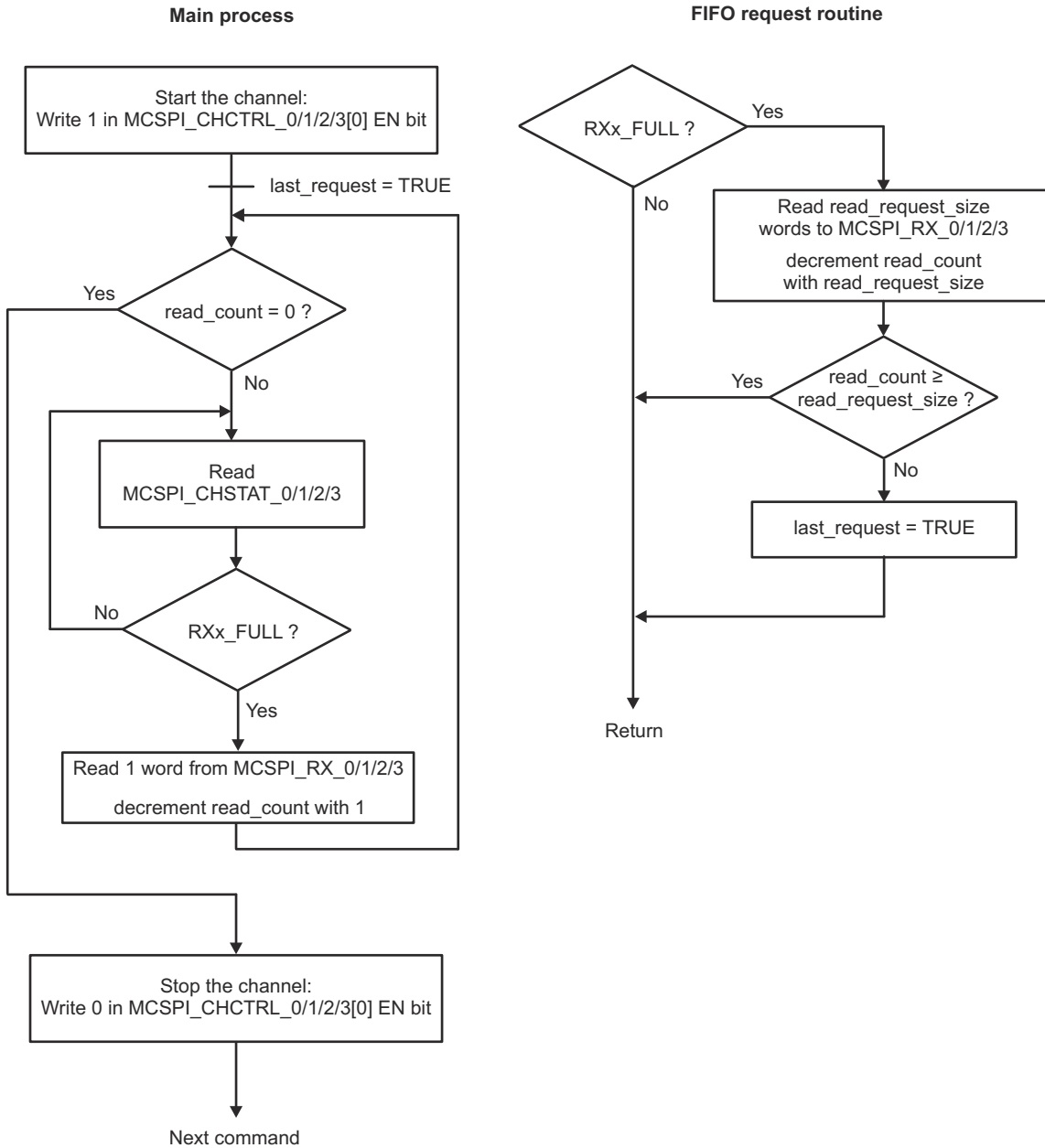
Figure 13-55. FIFO Mode Receive-Only Without Word Count (Controller)
