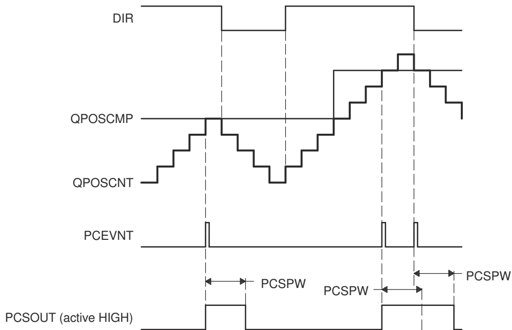
Figure 7-224. eQEP Position-compare Sync Output Pulse Stretcher
