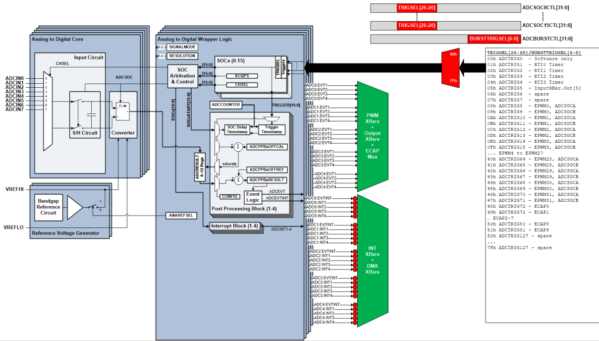
Figure 4-1. ADC Integration Diagram
