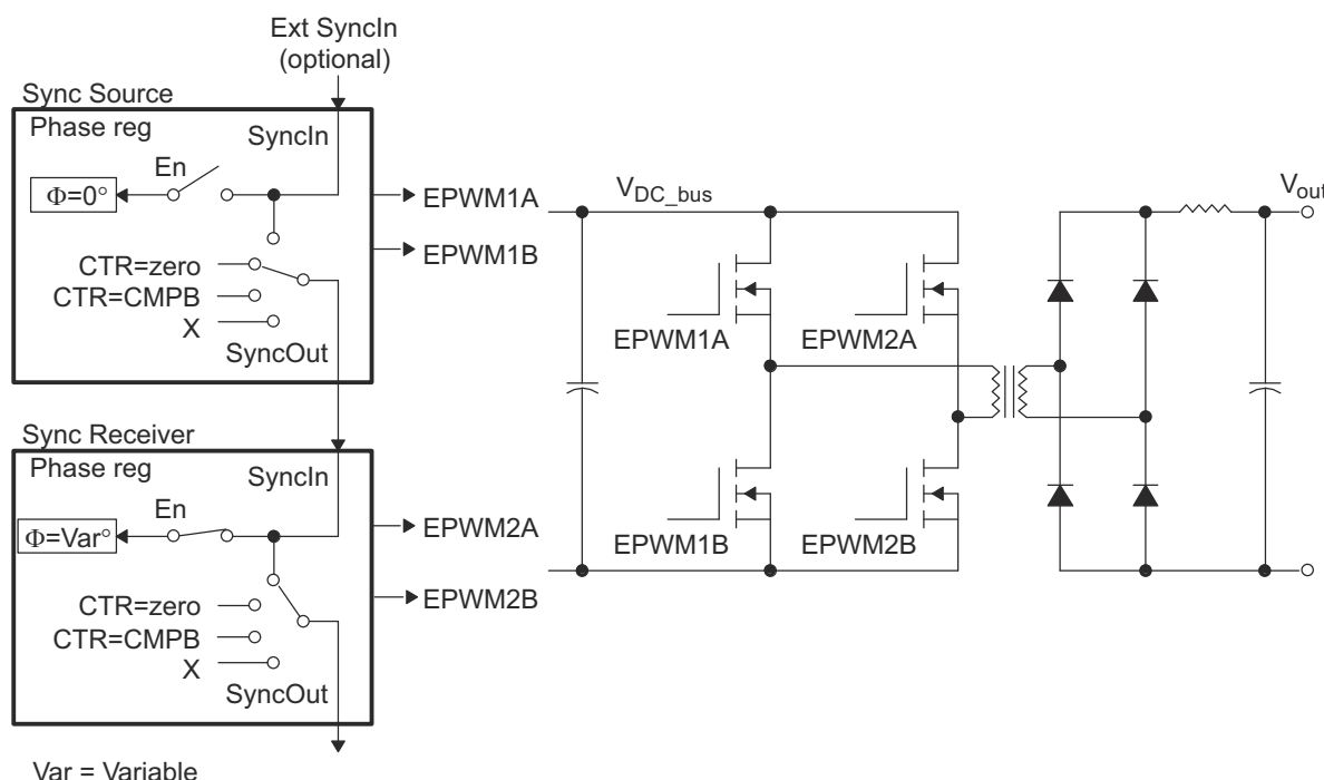
Figure 7-171. Control of Full-H Bridge Stage ( F_{PWM2} = F_{PWM1} )
