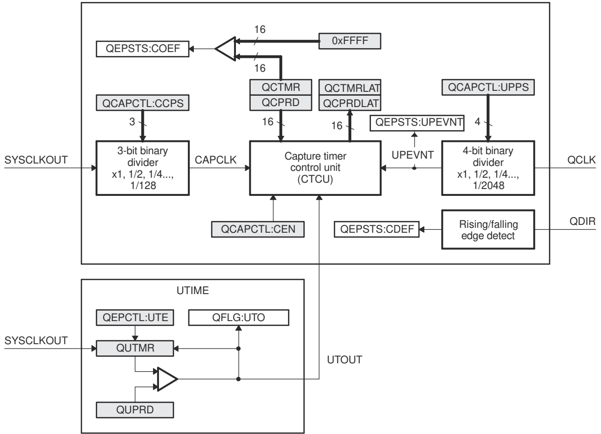
Figure 7-225. eQEP Edge Capture Unit
