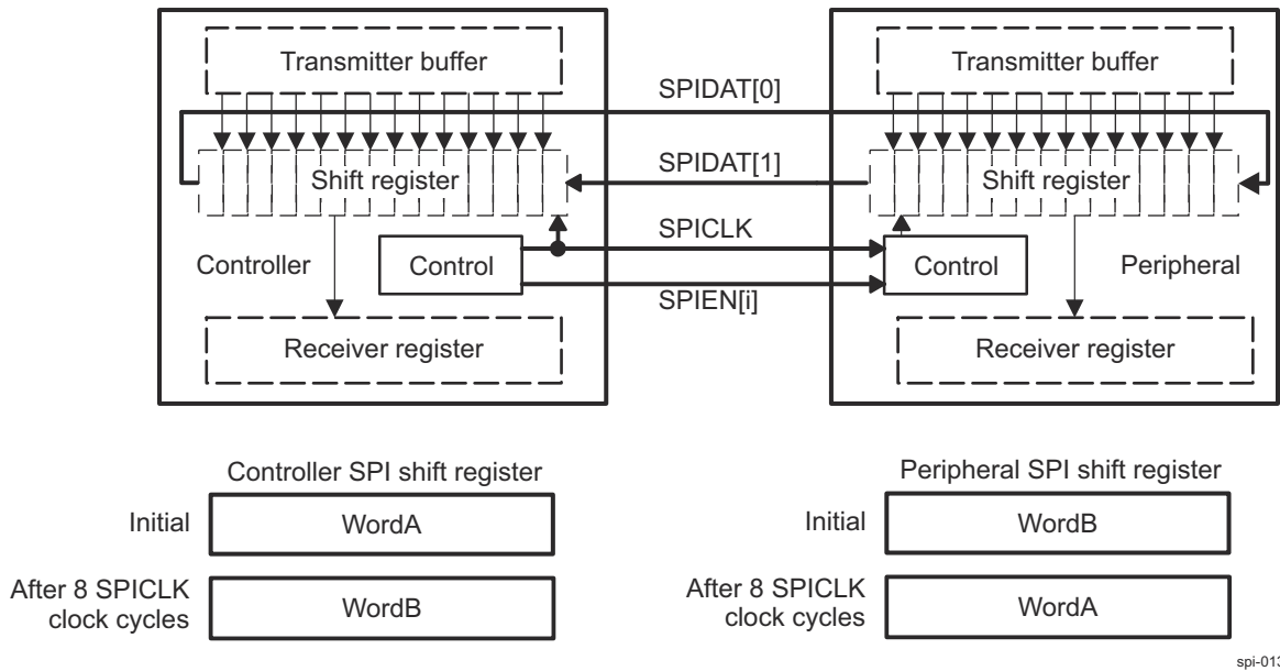
Figure 13-38. MCSPi Full-Duplex Transmission (Example)
