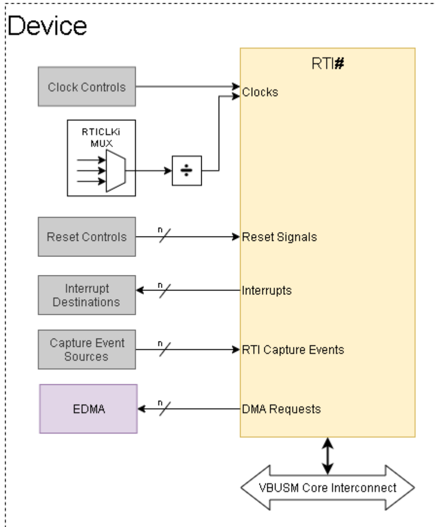
Figure 13-270. WWDT Overview
