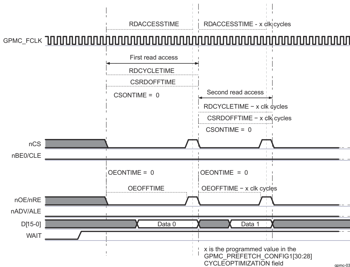
Figure 13-167. NAND Read Cycle Optimization Timing Description
