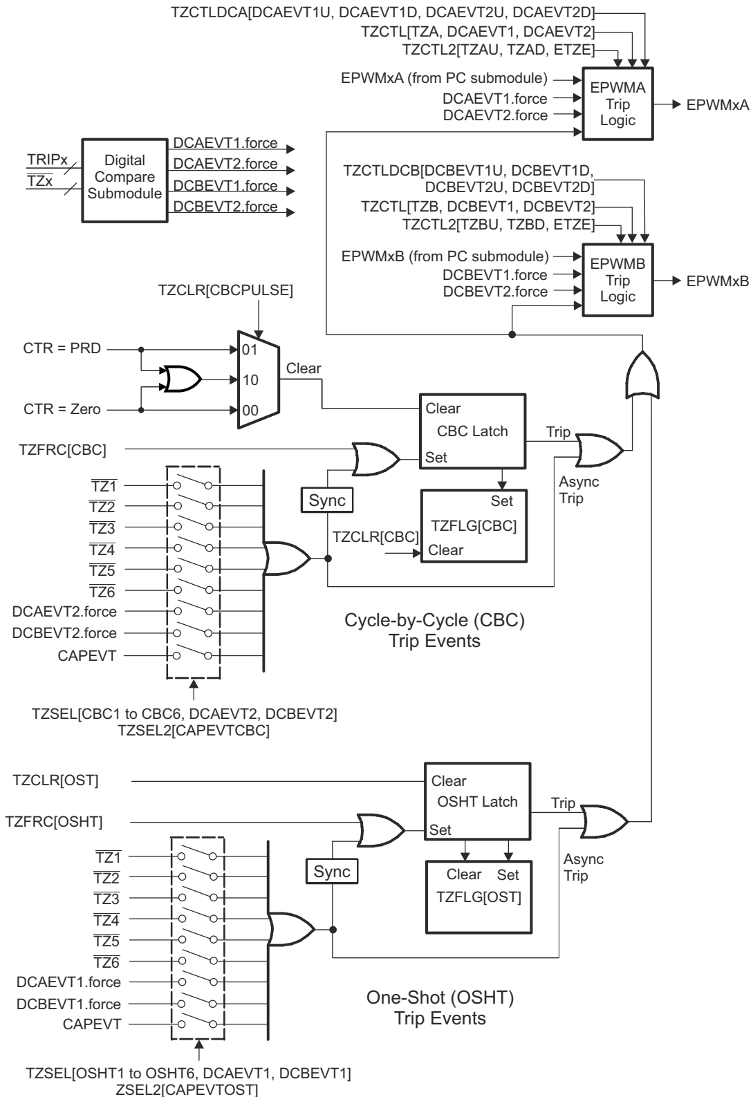
Figure 7-150. Trip-Zone Submodule Mode Control Logic
