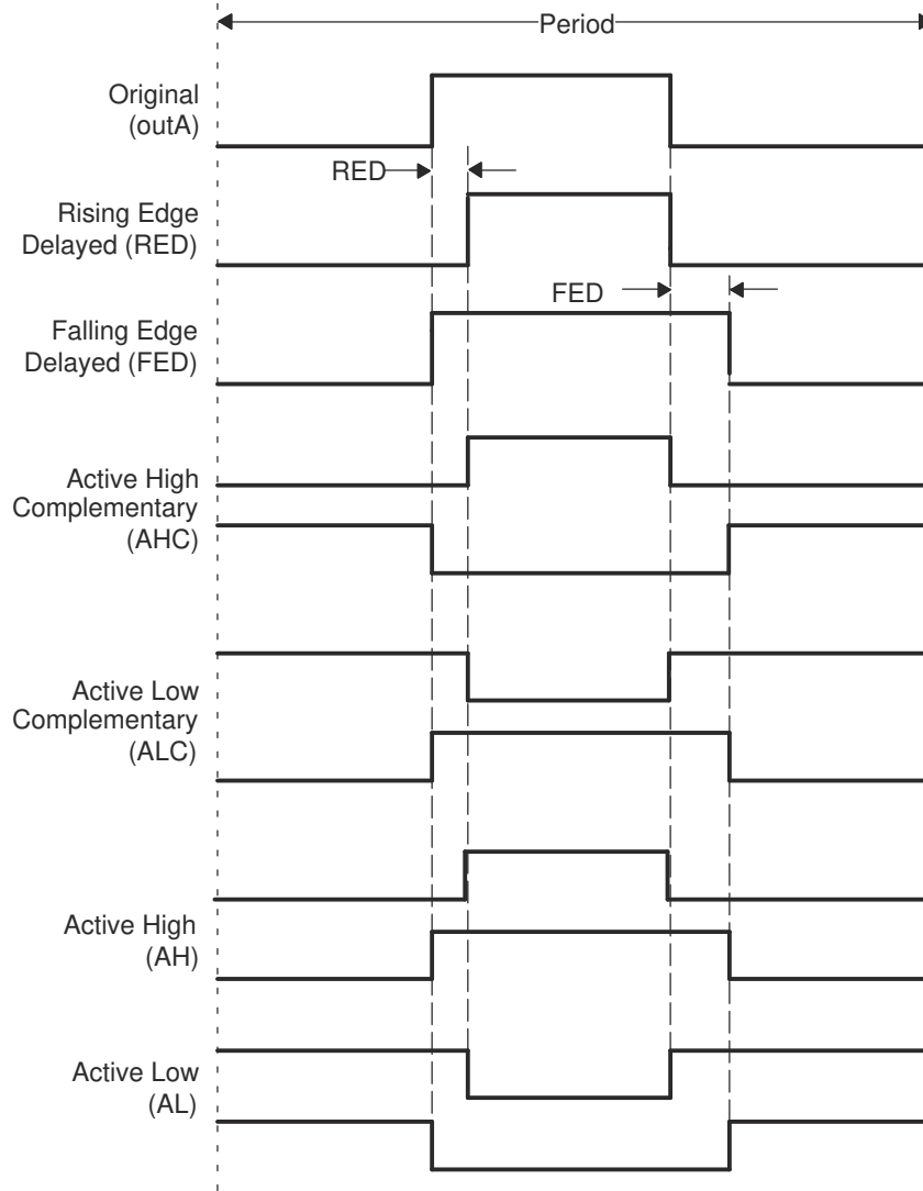
Figure 7-145. Dead-Band Waveforms for Typical Cases (0% < Duty < 100%)
