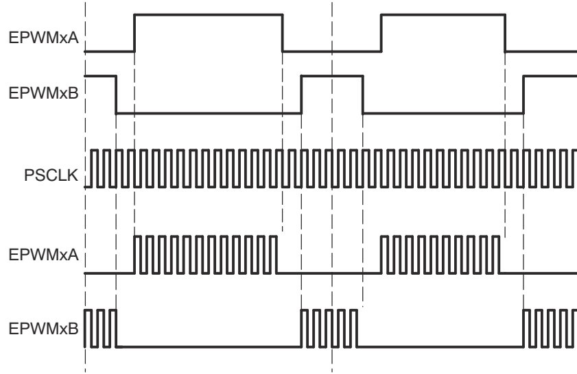
Figure 7-147. Simple PWM Chopper Submodule Waveforms Showing Chopping Action Only
