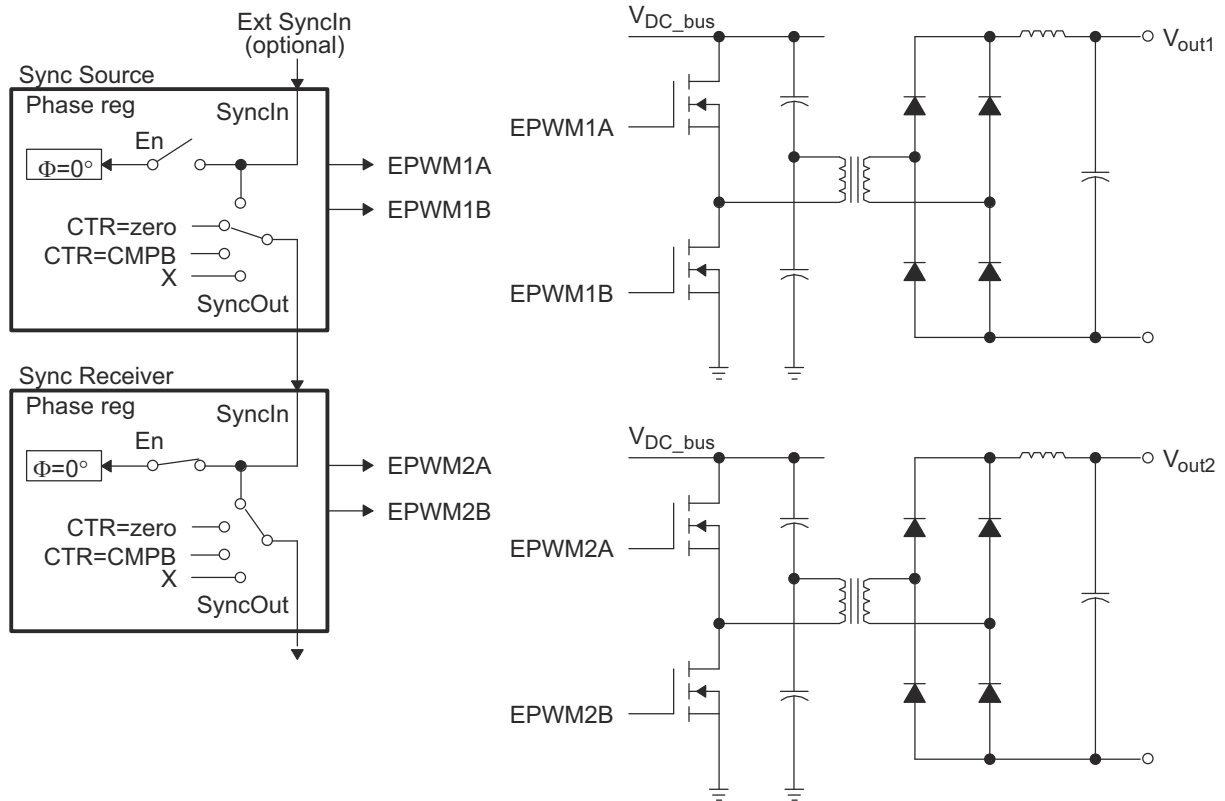
Figure 7-163. Control of Two Half-H Bridge Stages ( F_{PWM2} = N \times F_{PWM1} )
