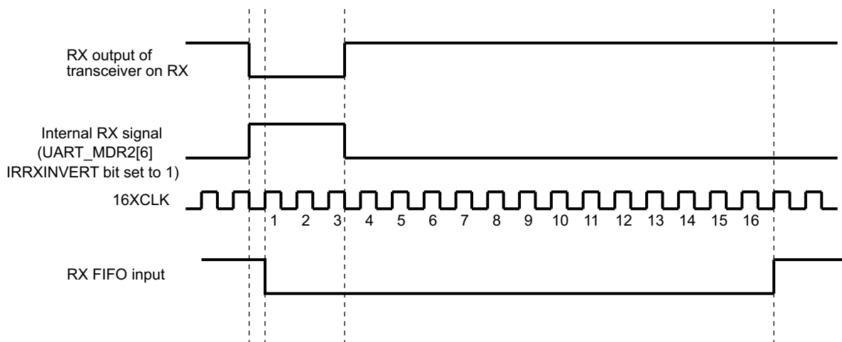
Figure 13-62. IrDA SIR Decoding Mechanism
