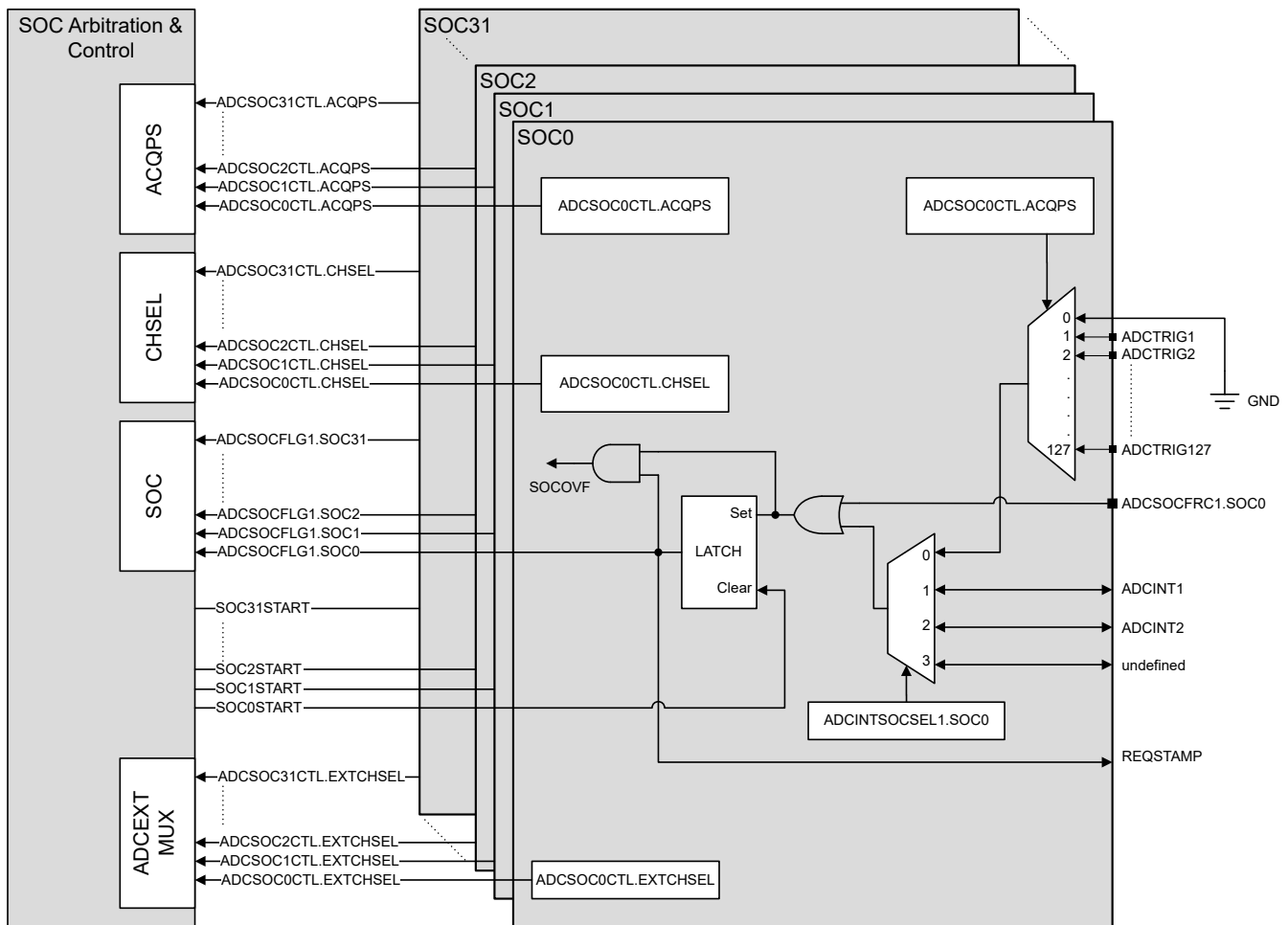
Figure 7-87. SOC Block Diagram
