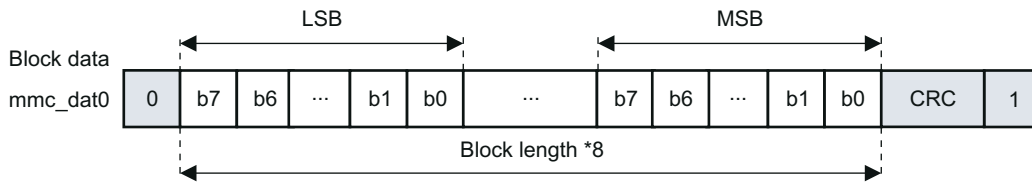
Figure 13-192. Data Packet for Block Transfer (1-Bit)
