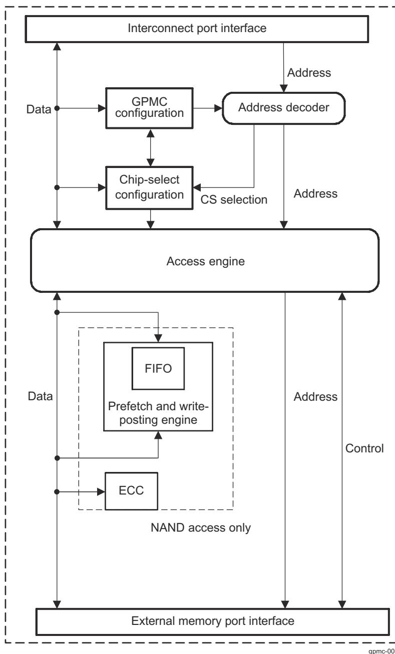
Figure 13-131. GPMC Block Diagram
