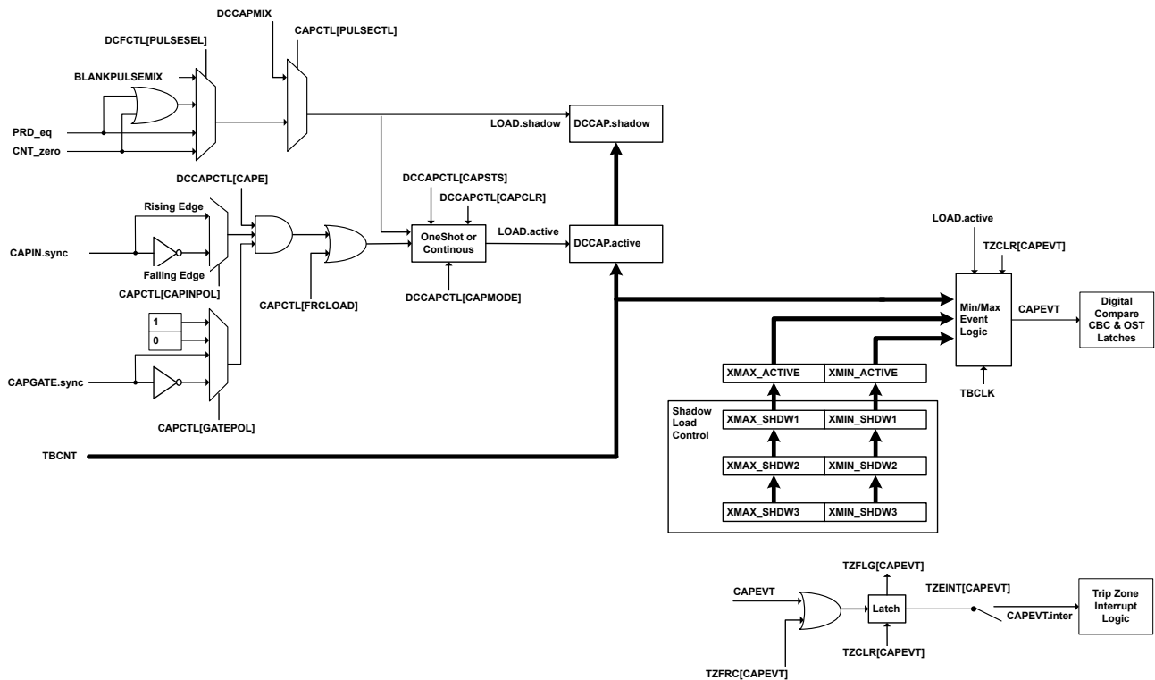
Figure 7-124. CAPEVT Signal Generation
