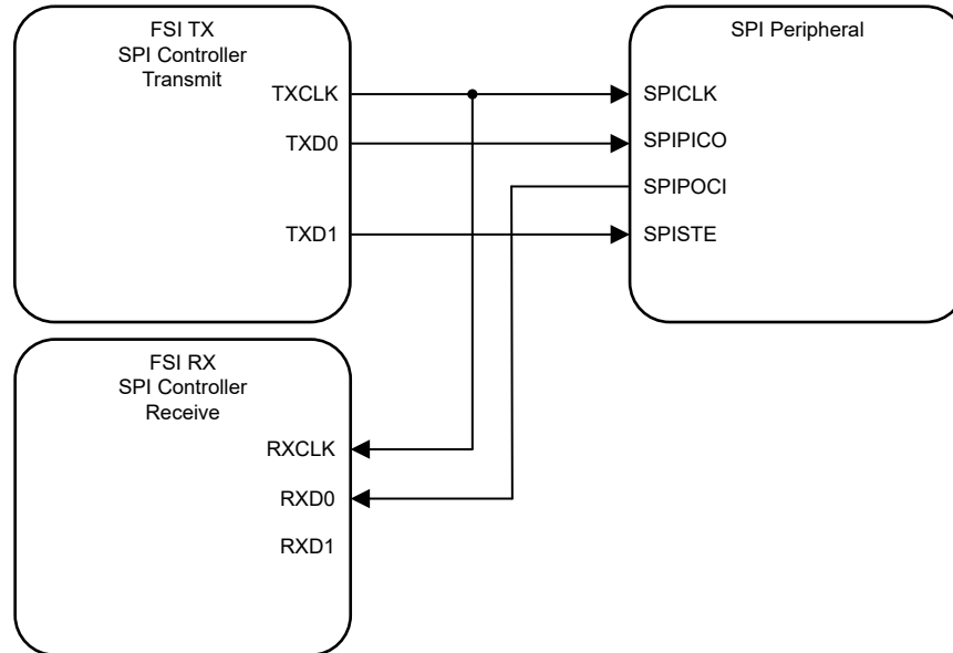
Figure 7-242. FSITX and FSIRX as SPI Controller, Full Duplex
