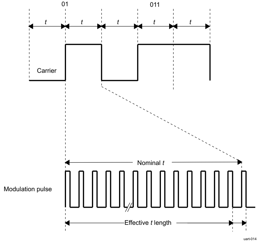
Figure 13-69. CIR Pulse Modulation
