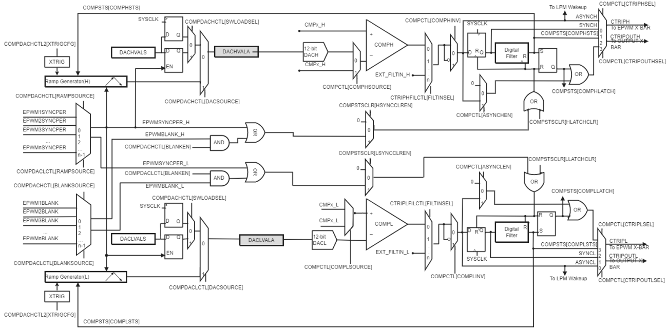
Figure 7-104. CMPSSA Module Block Diagram
