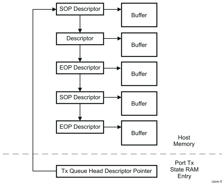
Figure 13-123. TX Queue Head Descriptor
