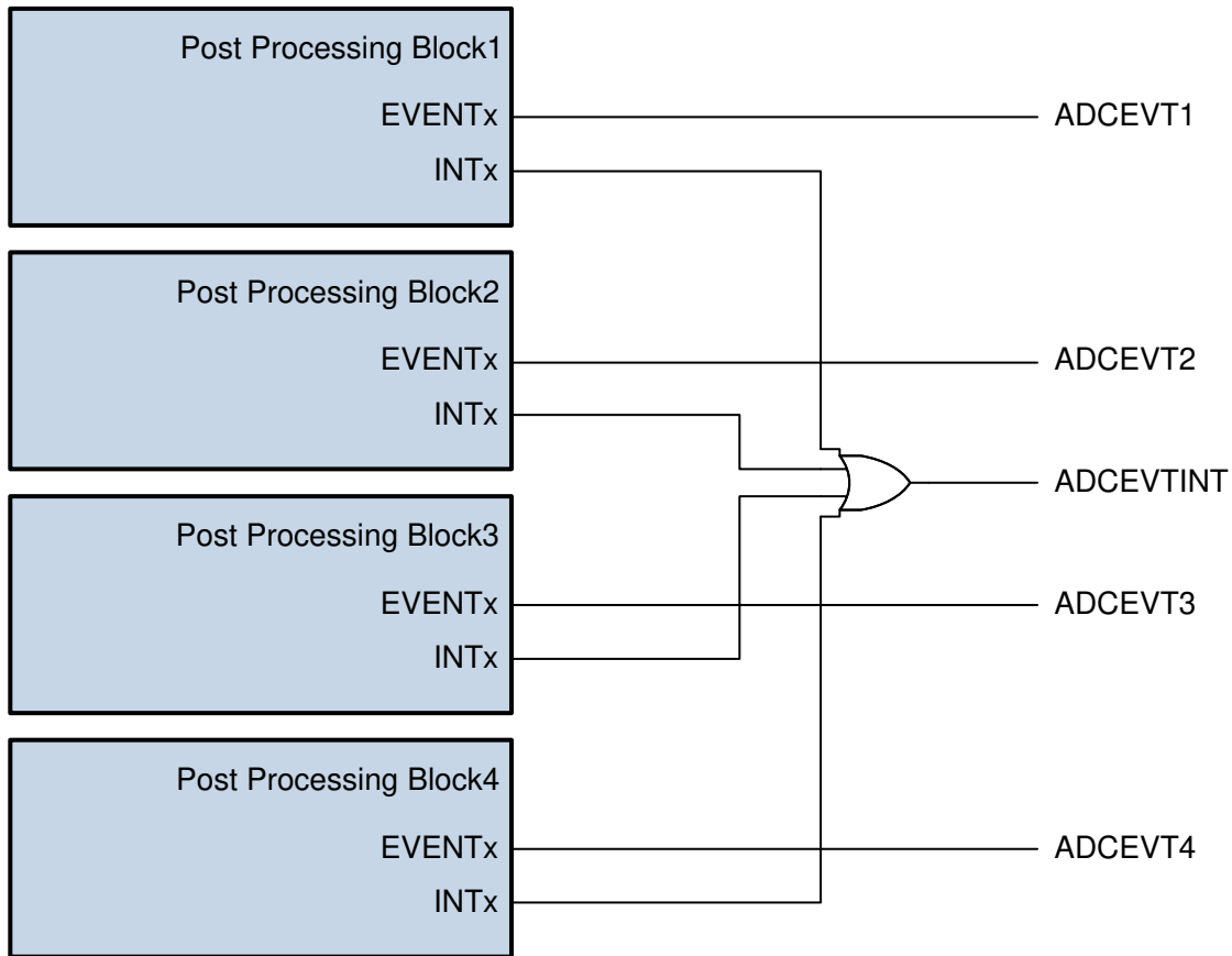
Figure 7-95. ADC PPB Interrupt Event
