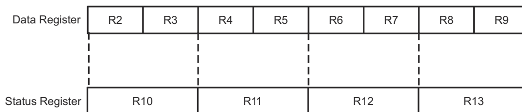
Figure 7-70. Data and Status Register Dependency
