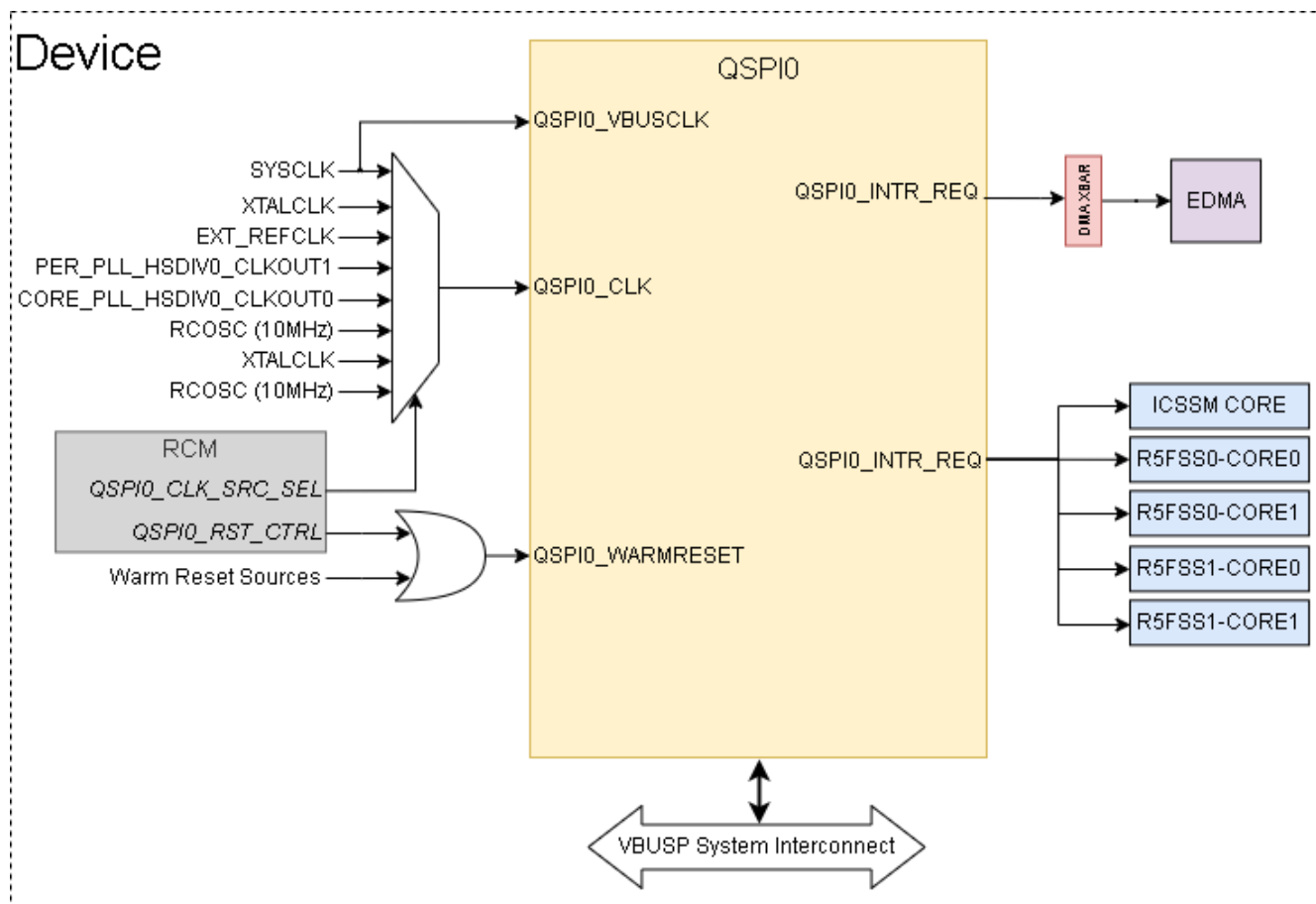
Figure 4-18. QSPI Integration Diagram
