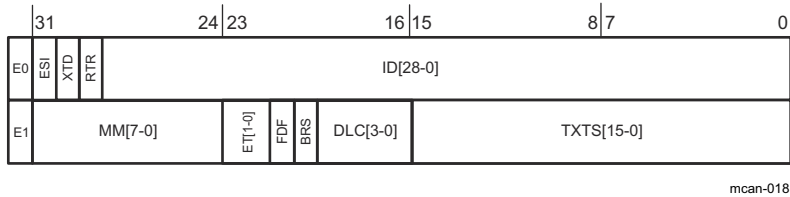
Figure 13-240. Tx Event FIFO Element Structure
