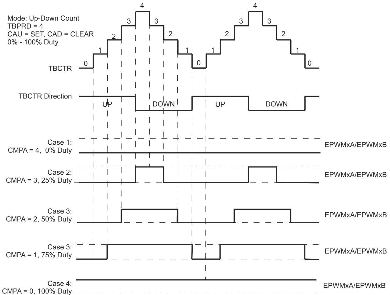
Figure 7-136. Up-Down-Count Mode Symmetrical Waveform
