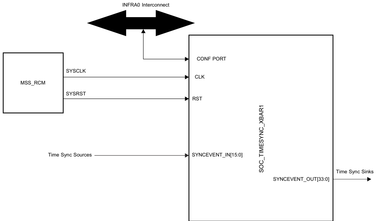
Figure 4-10. SOC_TIMESYNC_XBAR1 Integration
