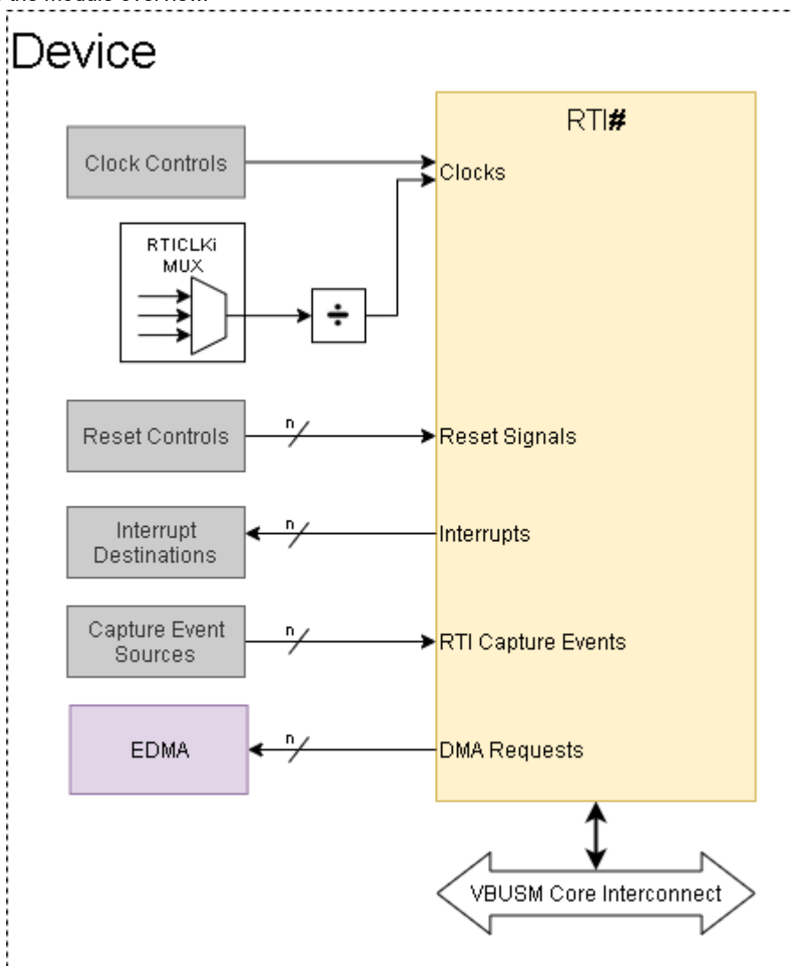
Figure 13-269. RTI Overview
