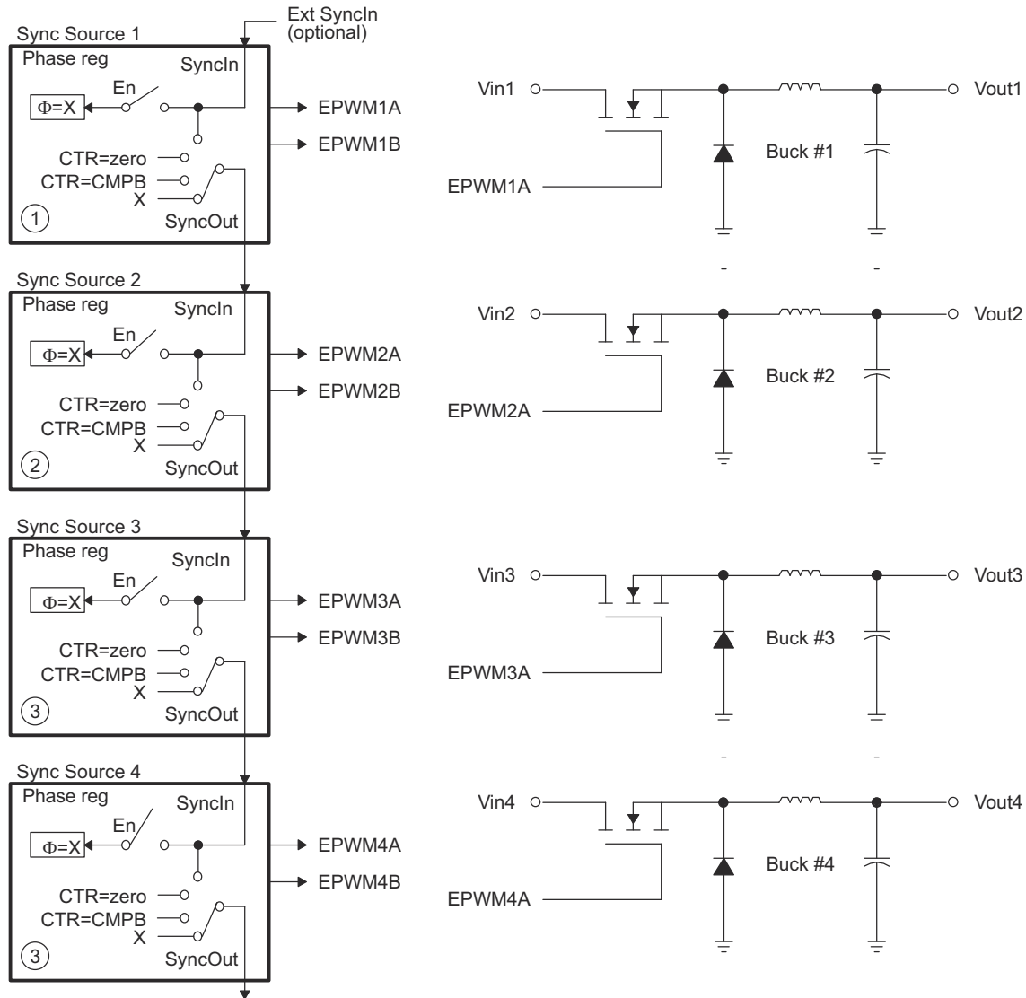
Figure 7-159. Control of Four Buck Stages. Here F_{PWM1} \neq F_{PWM2} \neq F_{PWM3} \neq F_{PWM4}
