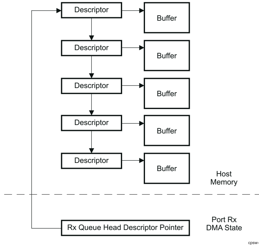
Figure 13-124. RX Queue Head Descriptor
