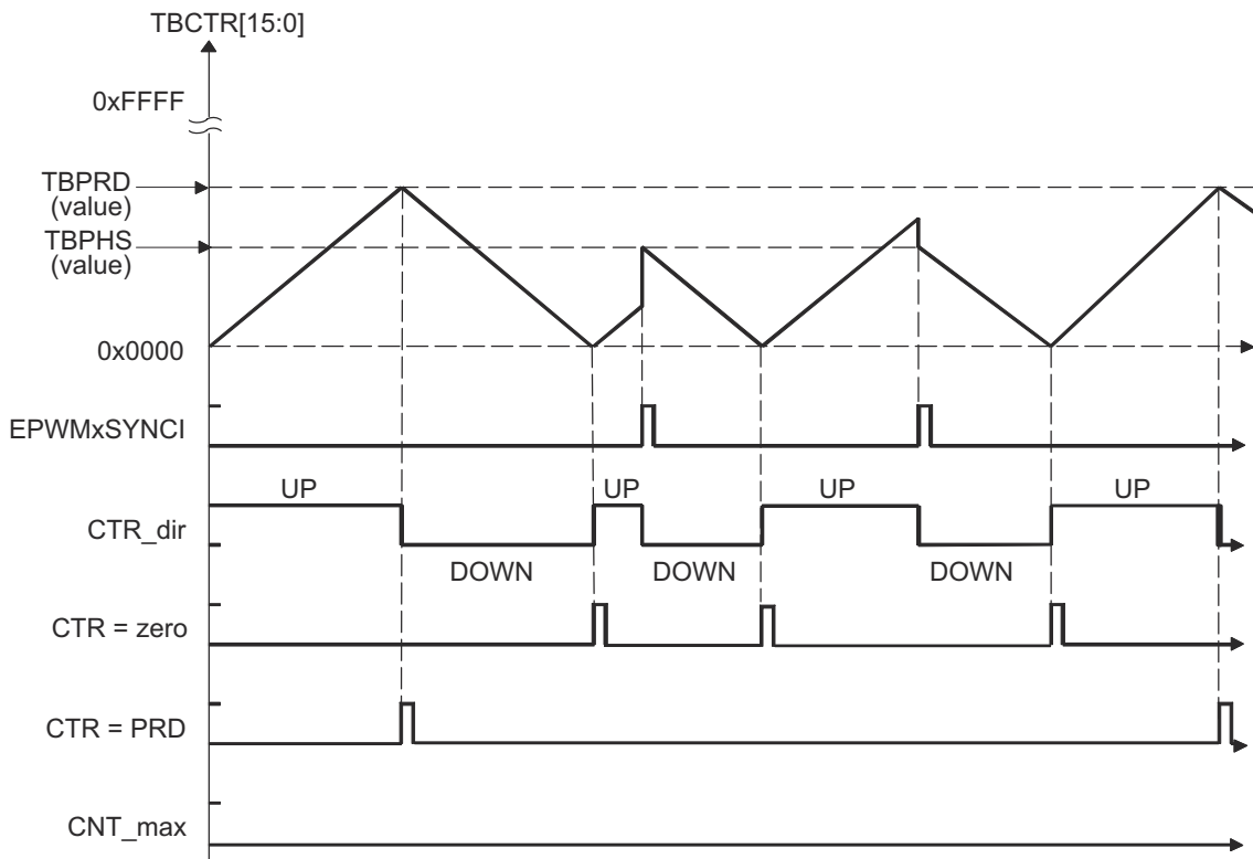
Figure 7-121. Time-Base Up-Down-Count Waveforms, TBCTL[PHSDIR = 0] Count Down On Synchronization Event
