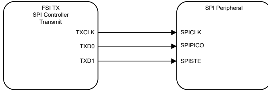
Figure 7-240. FSITX as SPI Controller, Transmit Only
