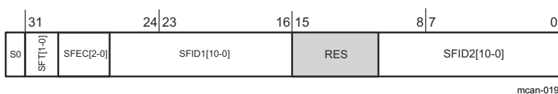
Figure 13-241. Standard Message ID Filter Element Structure
