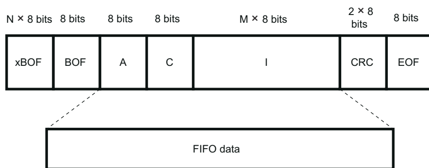
Figure 13-60. IrDA SIR Frame Format
