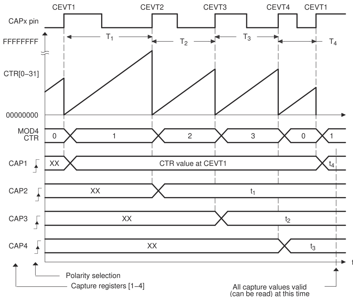
Figure 7-206. Capture Sequence for Delta Mode Time-stamp and Rising Edge Detect
