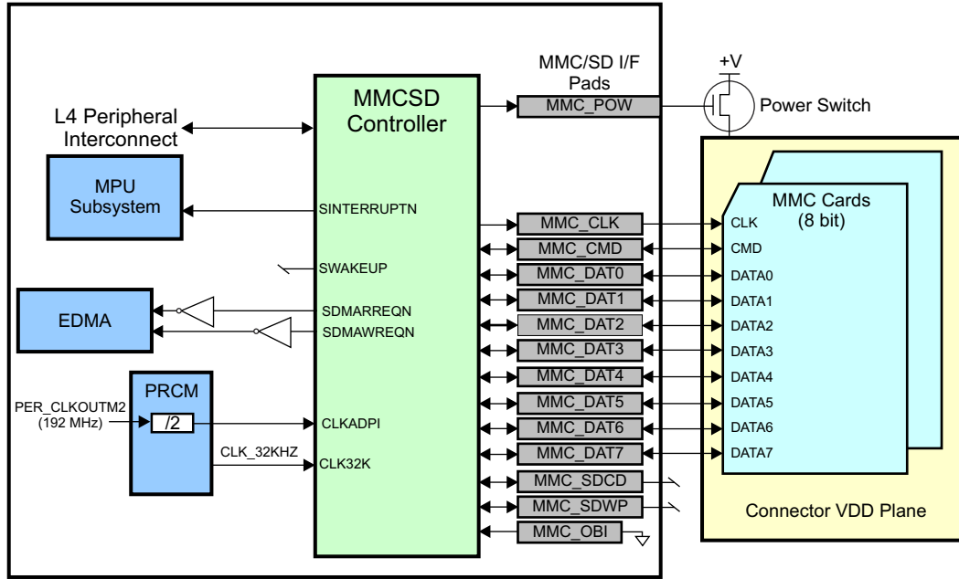
Figure 13-180. MMCS Module MMC Application
