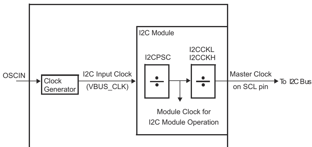
Figure 13-21. Clocking Diagram for the I2C Module
