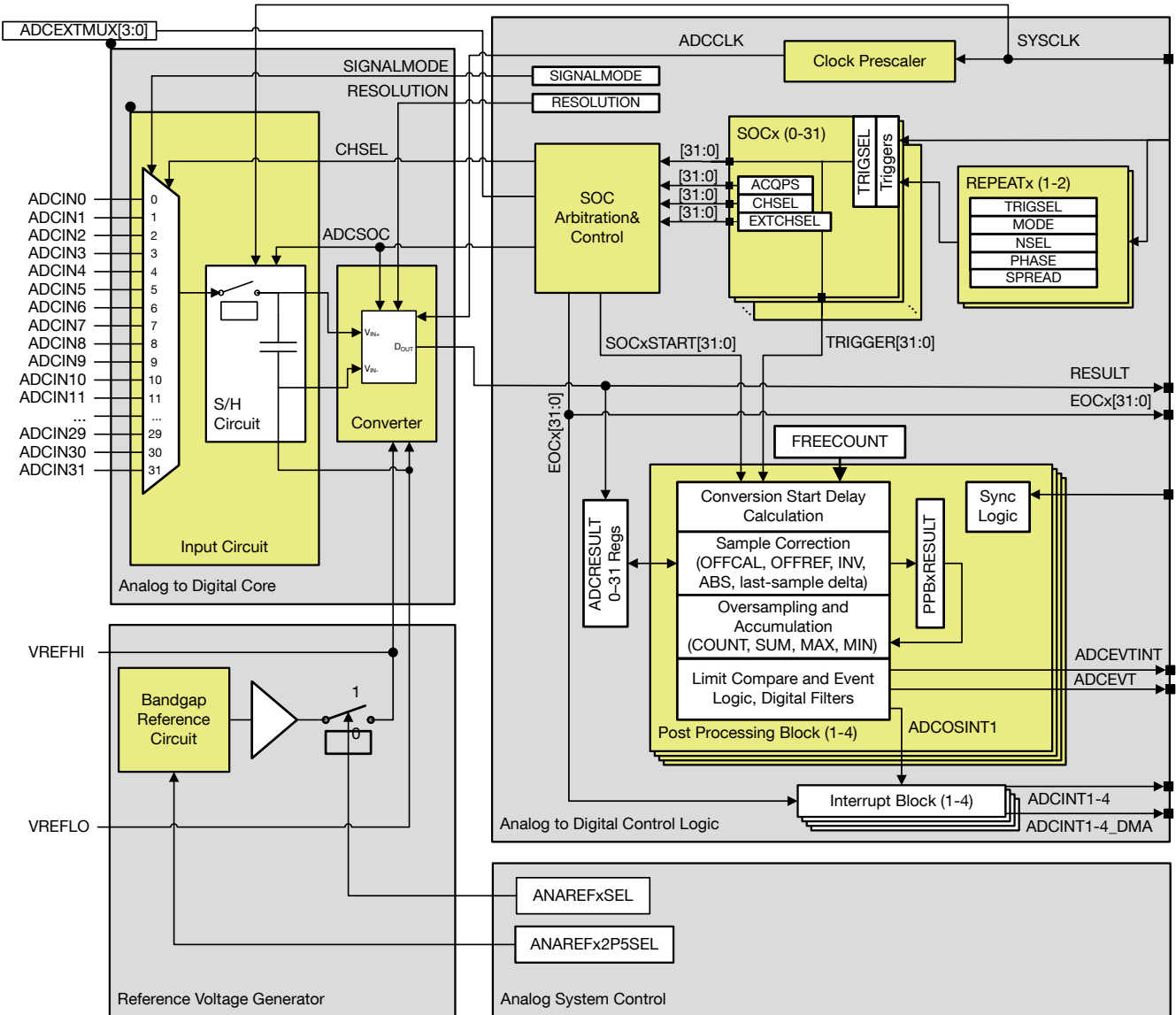
Figure 7-84. ADC Module Block Diagram
