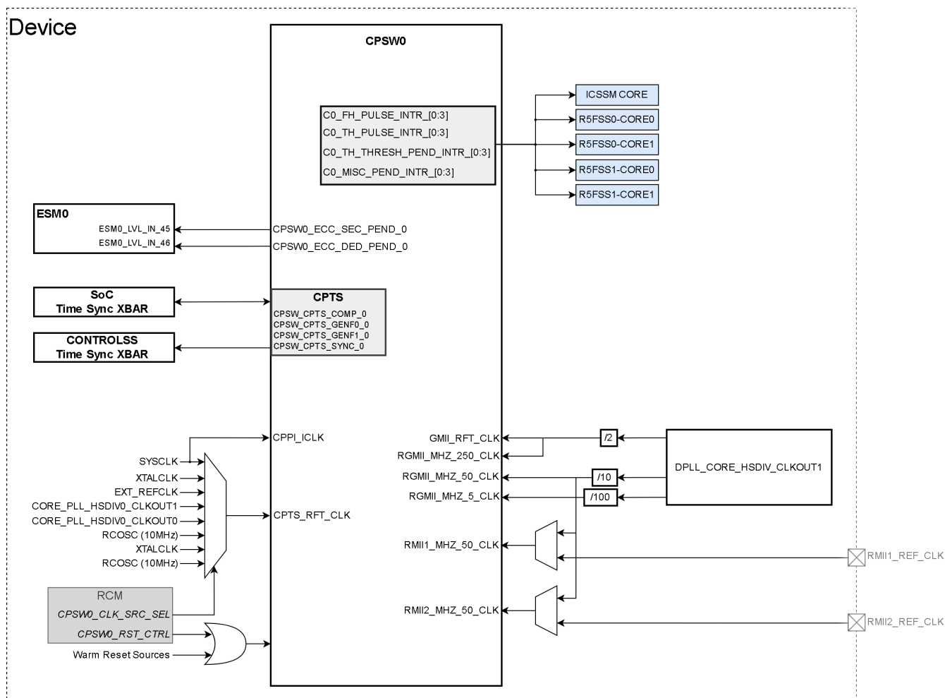
Figure 13-97. CPSW3G Integration Diagram
