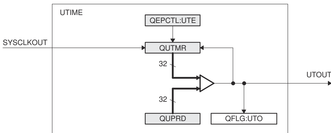
Figure 7-229. eQEP Unit Timer Base
