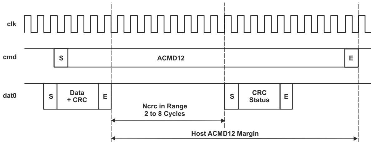
Figure 13-205. Auto CMD12 Timing During Write Transfer
