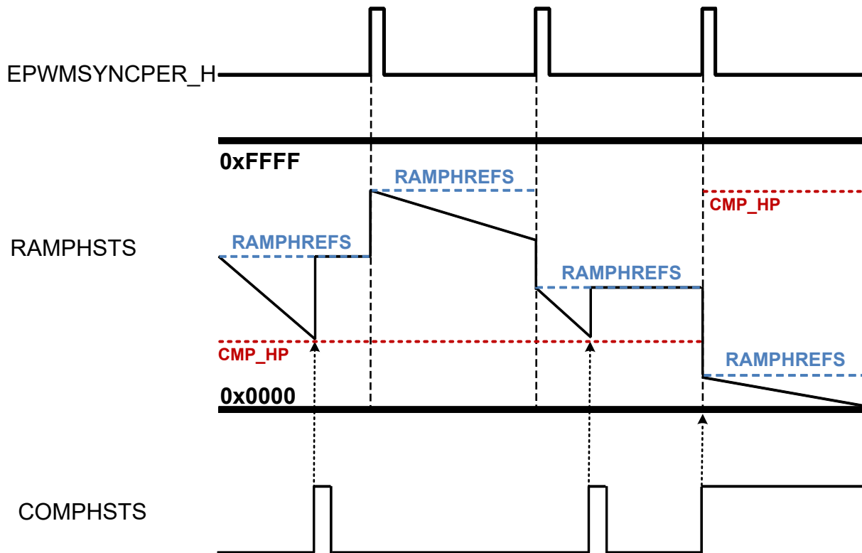
Figure 7-109. Ramp Generator Behavior
