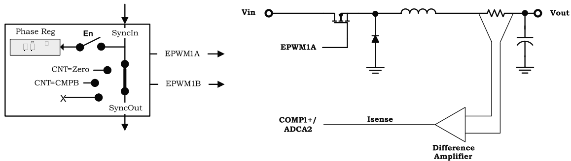
Figure 7-173. Peak Current Mode Control of Buck Converter
