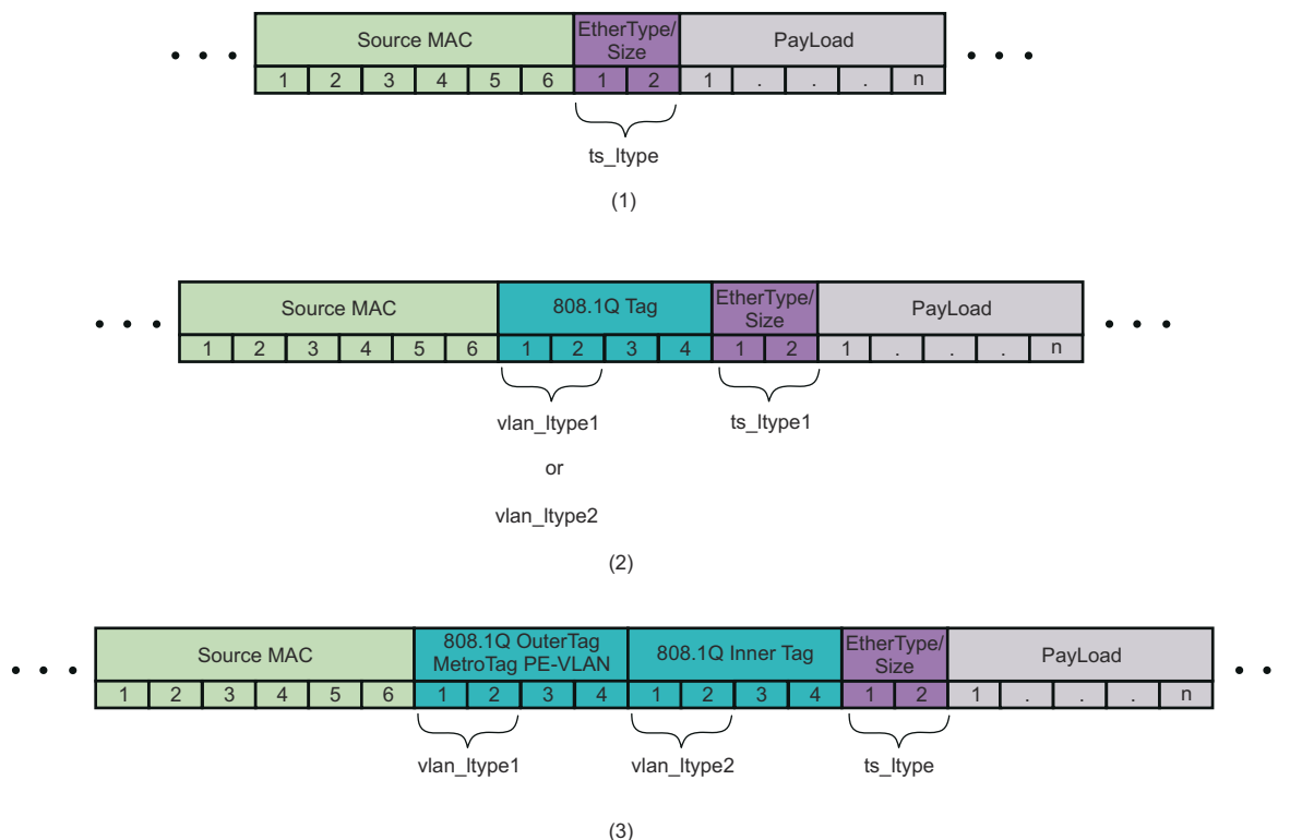
Figure 13-110. Partial Ethernet-II Frames Showing Register Mapping of EtherTypes for a Simple Frame (1), a Single 1Q Tag Added (2), and Two 1Q Tags Added (3)
