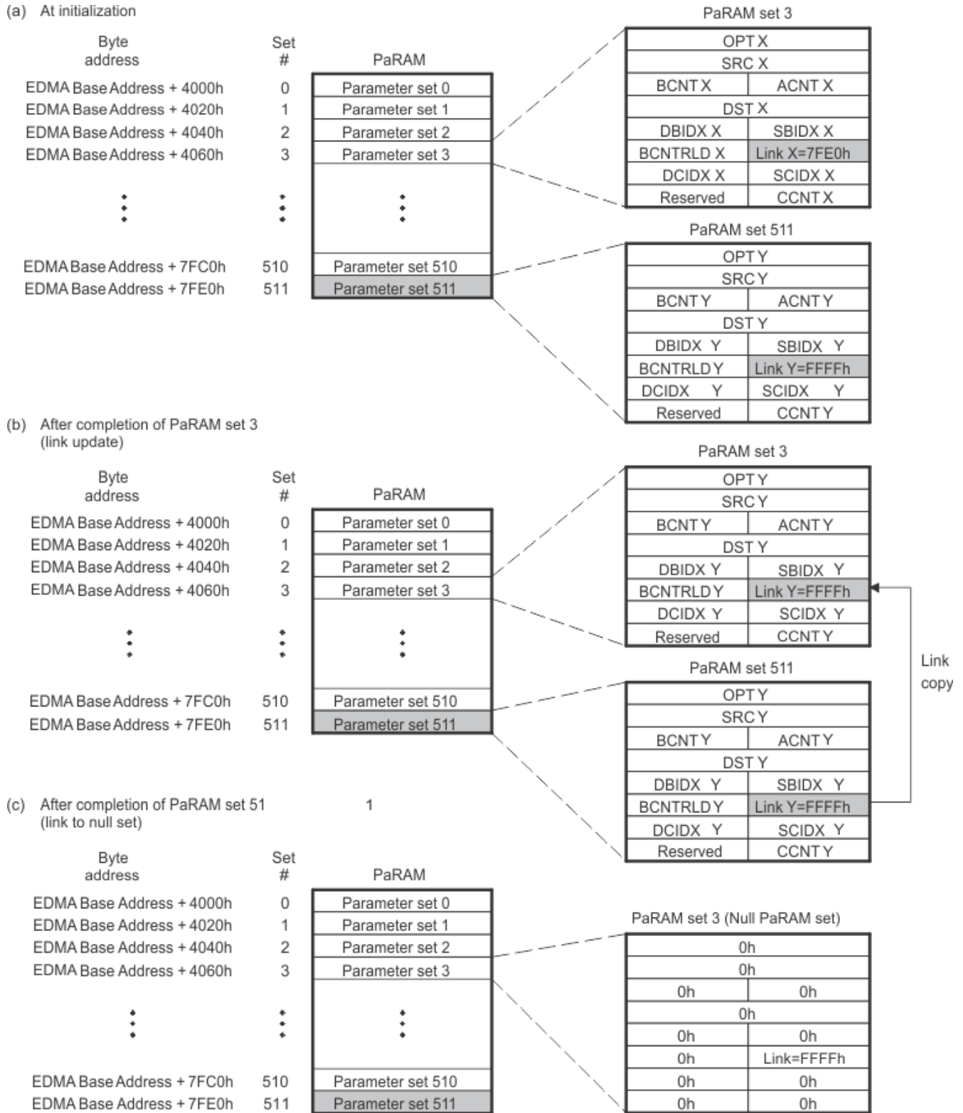
Figure 11-9. Linked Transfer
