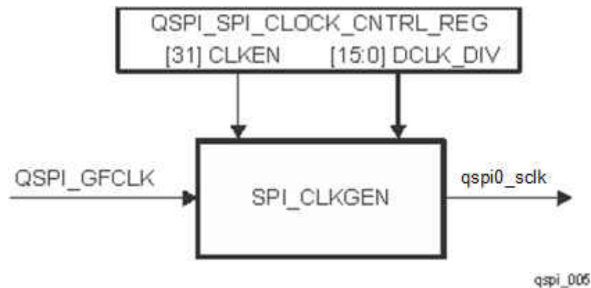
Figure 13-219. SPI_CLKGEN Block
