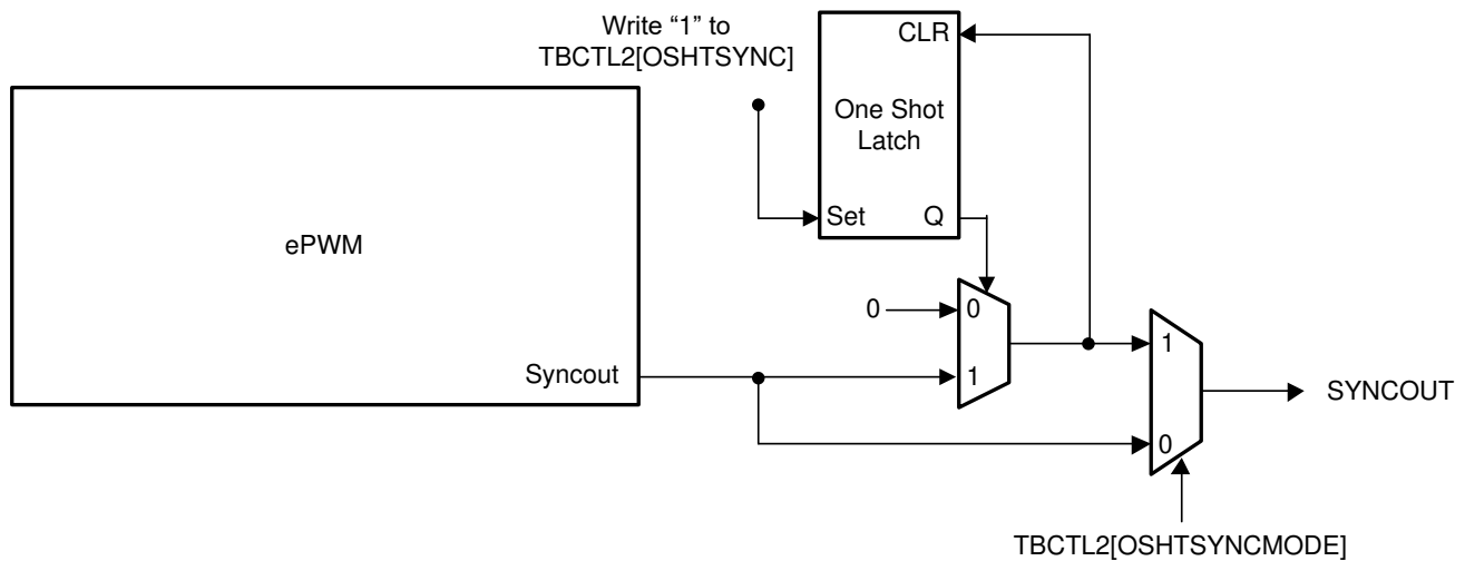
Figure 7-126. One-Shot Sync Mode
