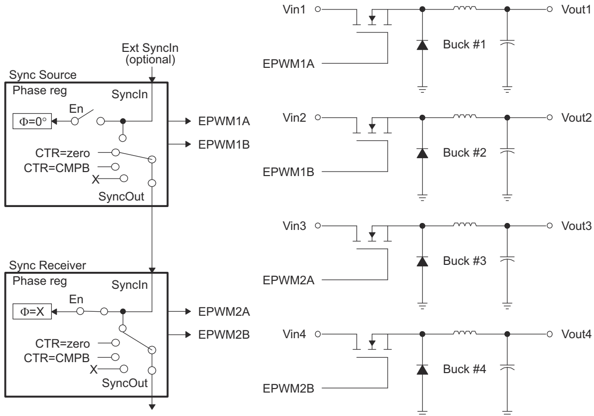
Figure 7-161. Control of Four Buck Stages. (Note: F_{PWM2} = N \times F_{PWM1} )
