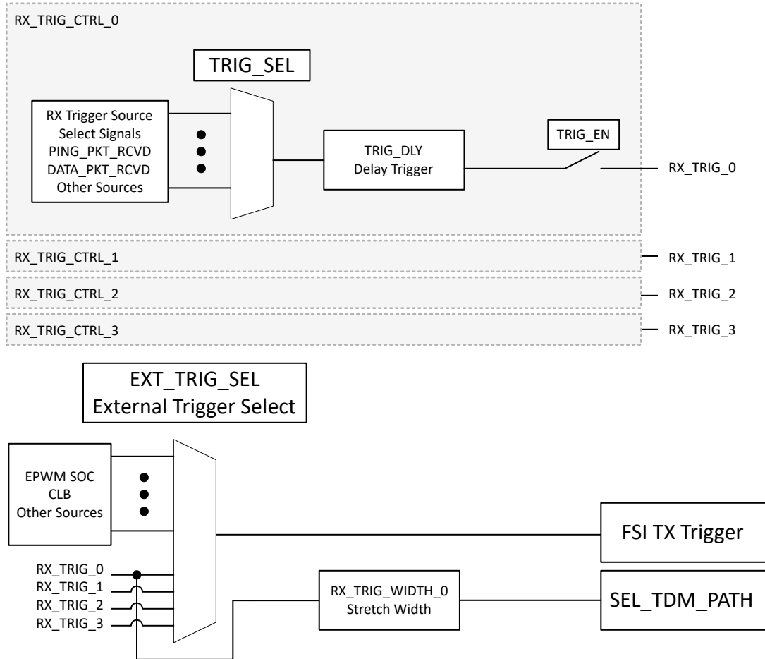
Figure 7-239. RX_TRIGx FSI Trigger
