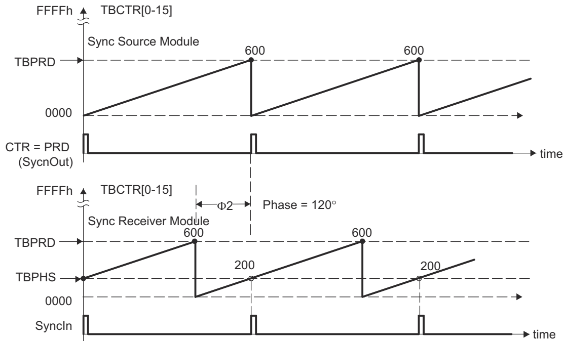
Figure 7-168. Timing Waveforms Associated With Phase Control Between Two Modules
