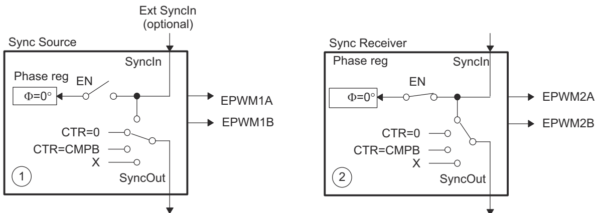
Figure 7-158. EPWM1 Configured as a Typical Sync Source, EPWM2 Configured as a Sync Receiver
