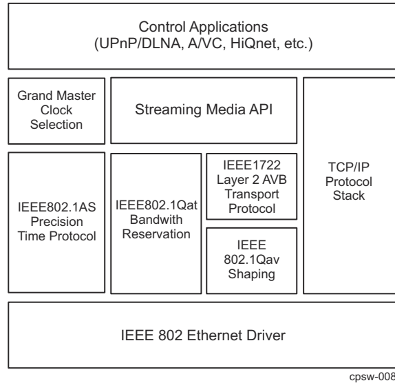
Figure 13-101. The Network Static with AVB
