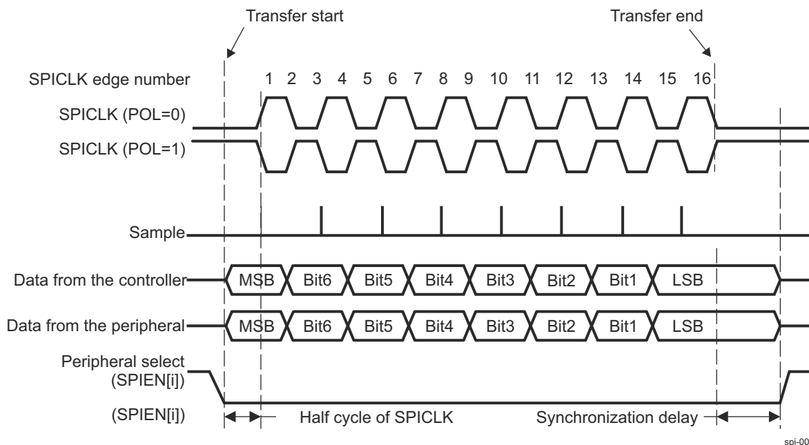
Figure 13-30. Full-Duplex Transfer Format With PHA = 0
