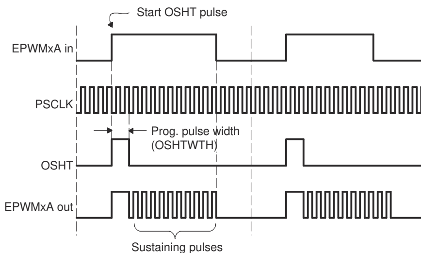
Figure 7-148. PWM Chopper Submodule Waveforms Showing the First Pulse and Subsequent Sustaining Pulses
