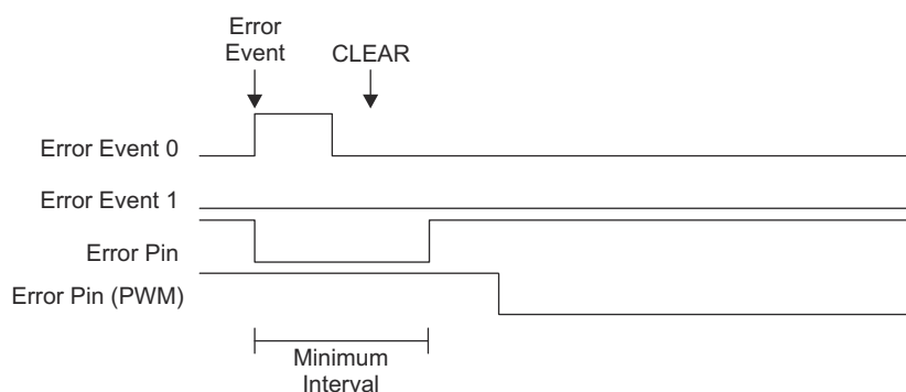
Figure 13-293. ESM Error Pin Assertion with CLEAR during Minimum Interval
