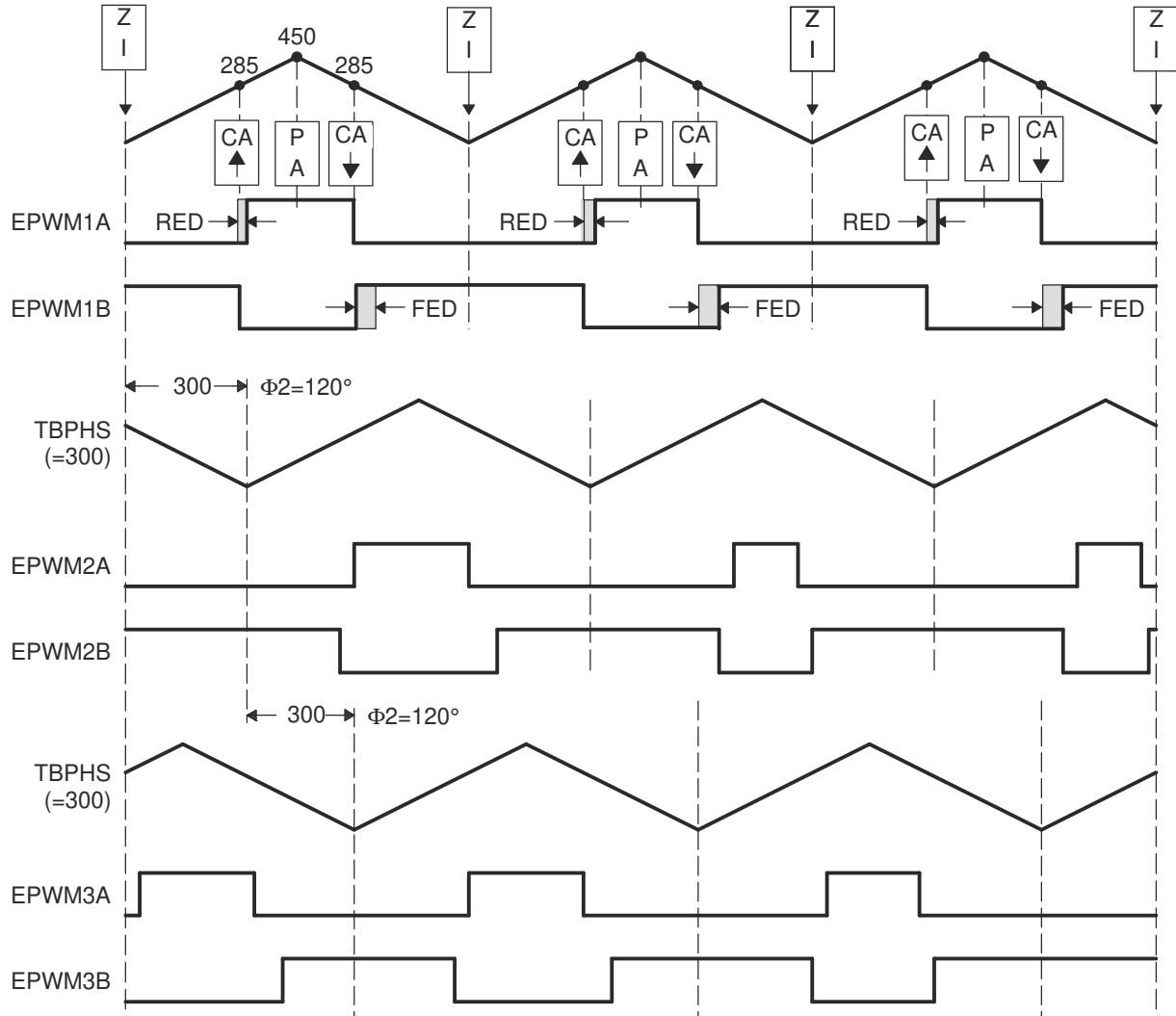
Figure 7-170. 3-Phase Interleaved DC/DC Converter Waveforms for Control of 3-Phase Interleaved DC/DC Converter
