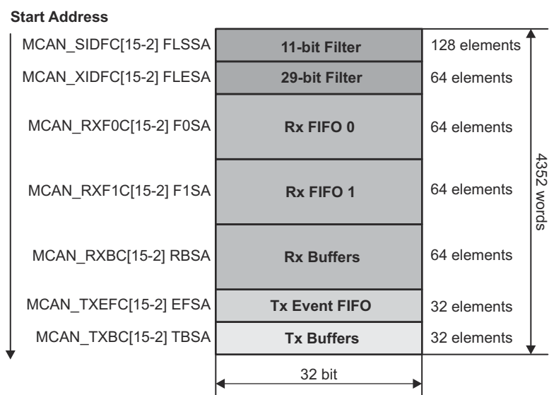
Figure 13-237. Message RAM Configuration
