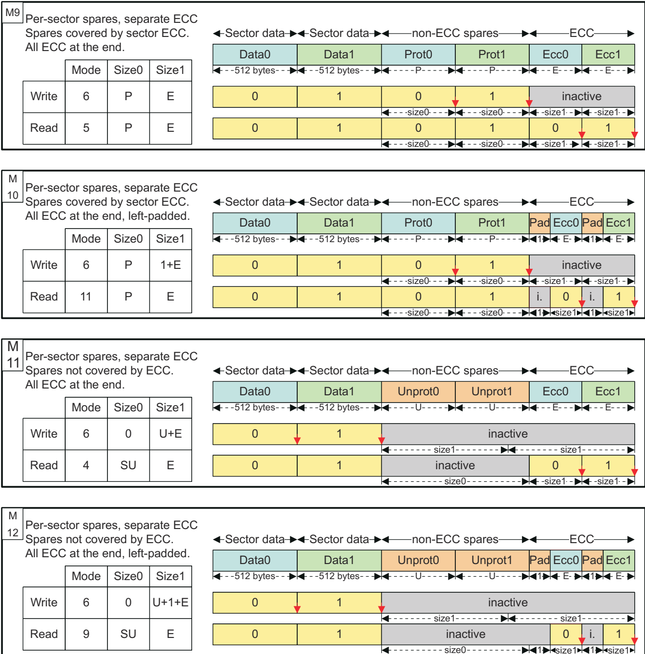
Figure 13-166. NAND Page Mapping and ECC: Per-Sector Schemes, With Separate ECC
