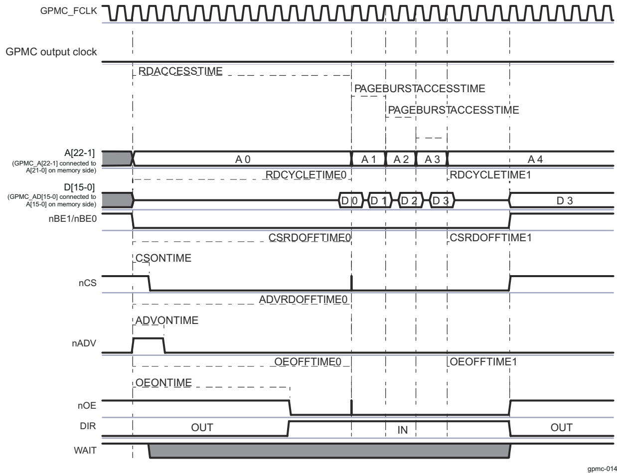
Figure 13-152. Asynchronous Multiple (Page Mode) Read
