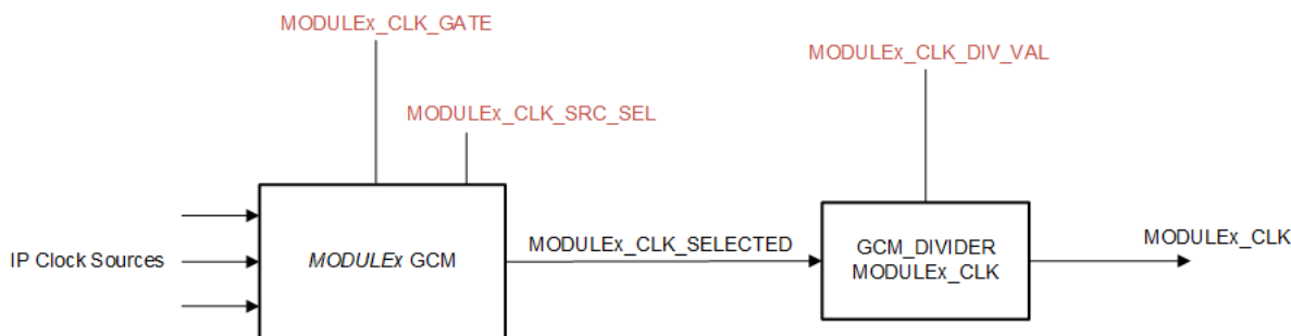
Figure 6-24. Generic IP clocking with GCM and Divider
