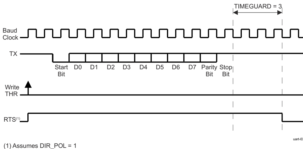
Figure 13-89. RS-485 External Transceiver Direction Control
