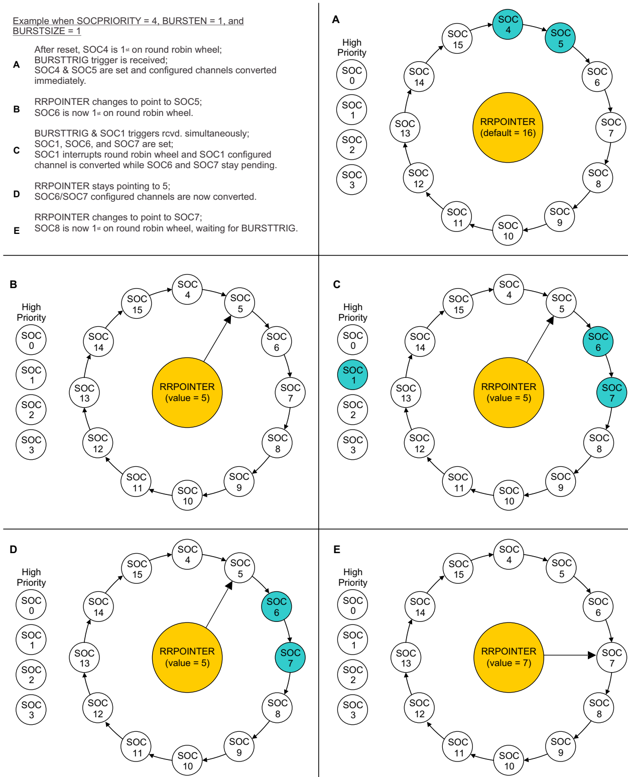
Figure 7-92. Burst Priority Example
