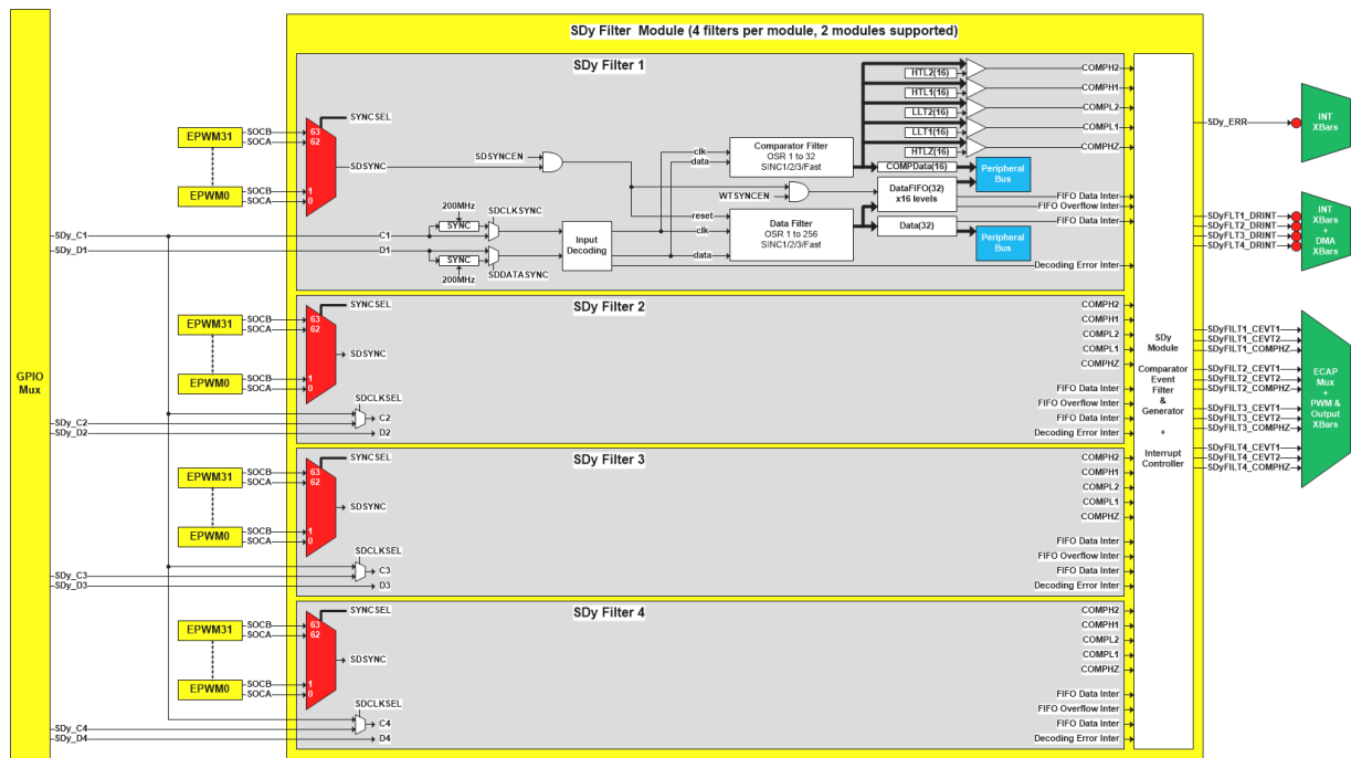
Figure 7-245. Sigma Delta Filter Module (SDFM) Block Diagram
