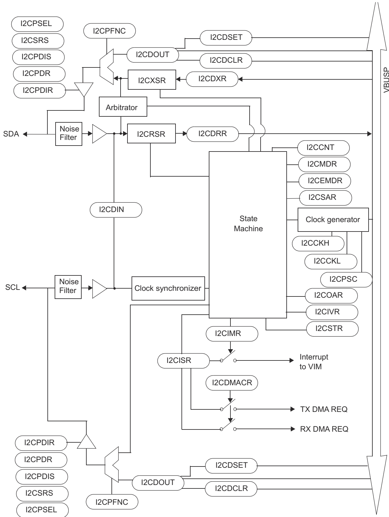
Figure 13-6. Simple I2C Block Diagram
