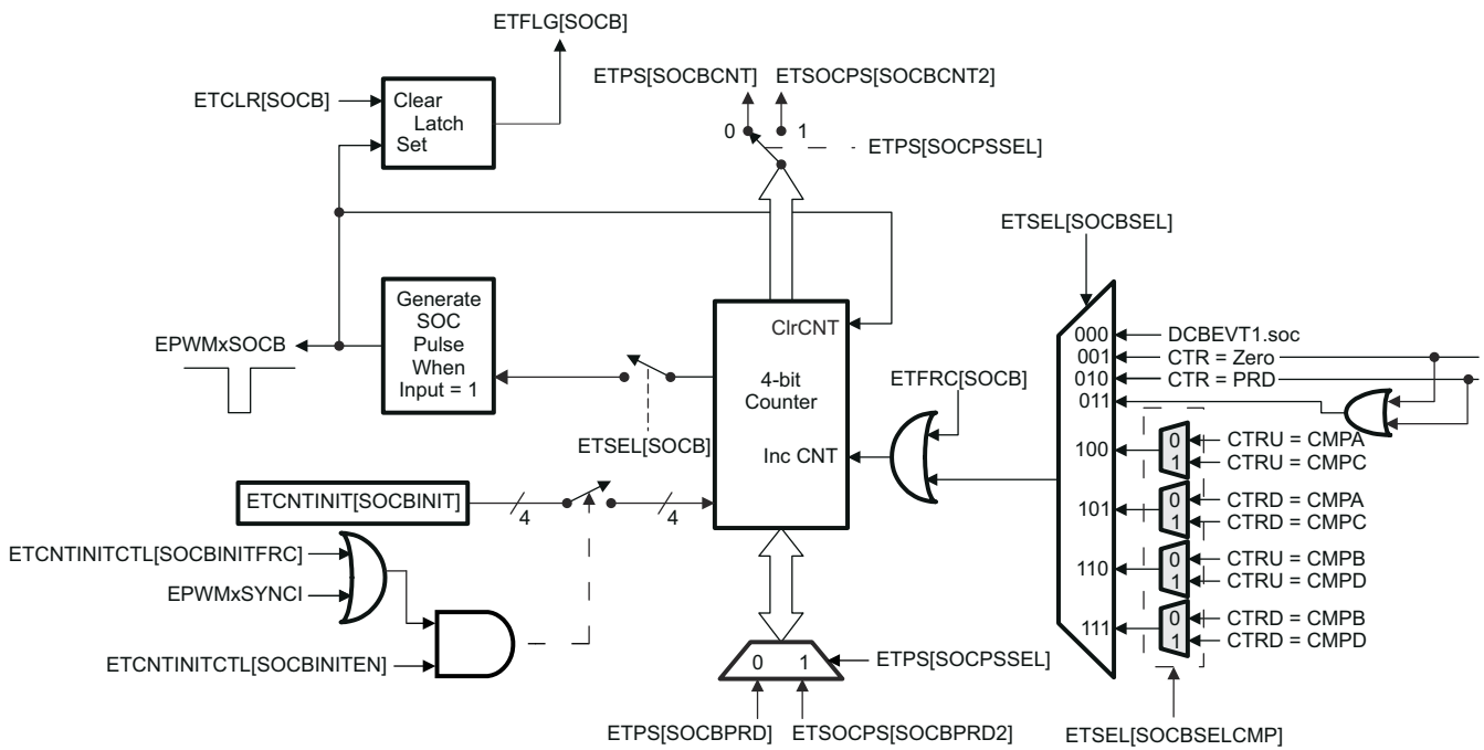
Figure 7-155. Event-Trigger SOCB Pulse Generator
