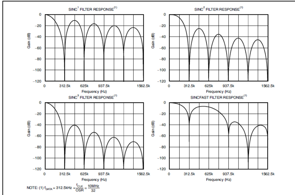
Figure 7-254. Frequency Response of Different Sinc Filters
