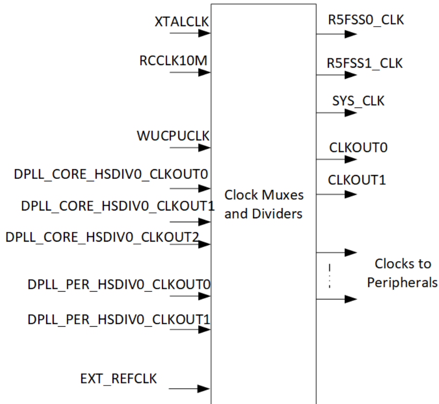
Figure 6-19. Core Clock Tree
