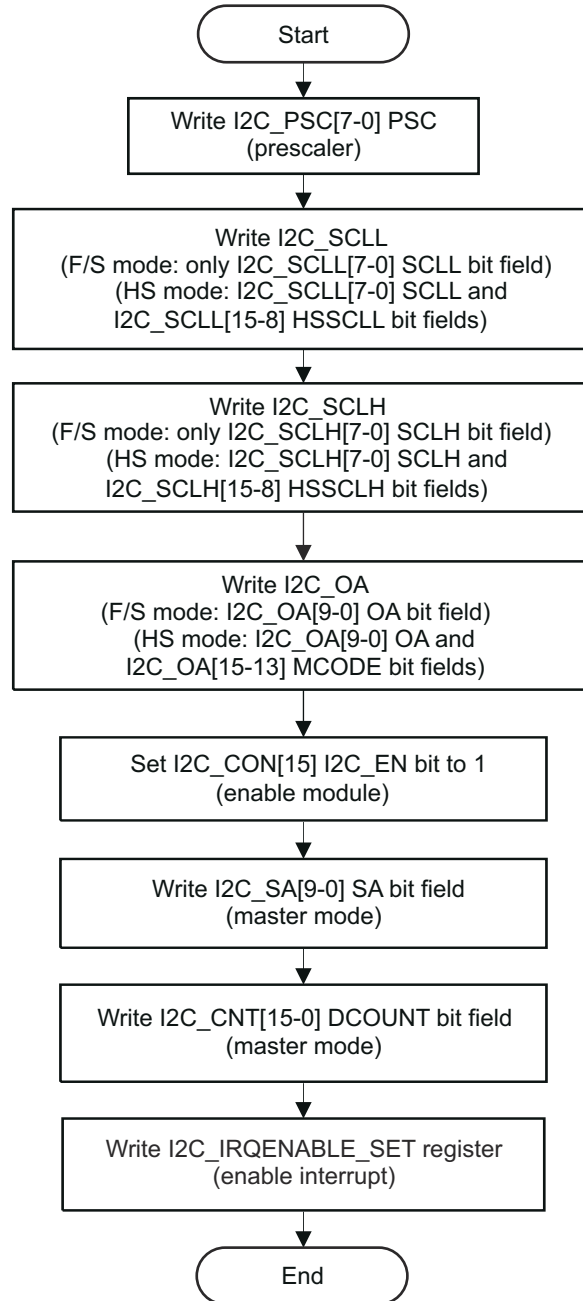
Figure 13-22. I2C Setup Procedure
