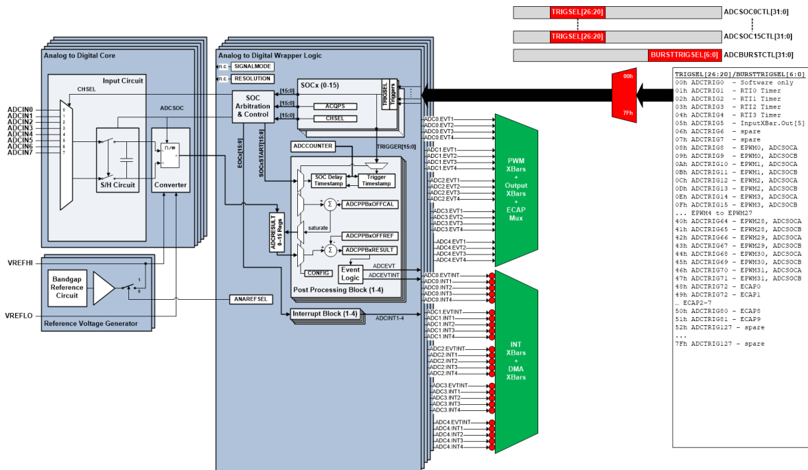
Figure 7-85. ADC Integration Diagram
