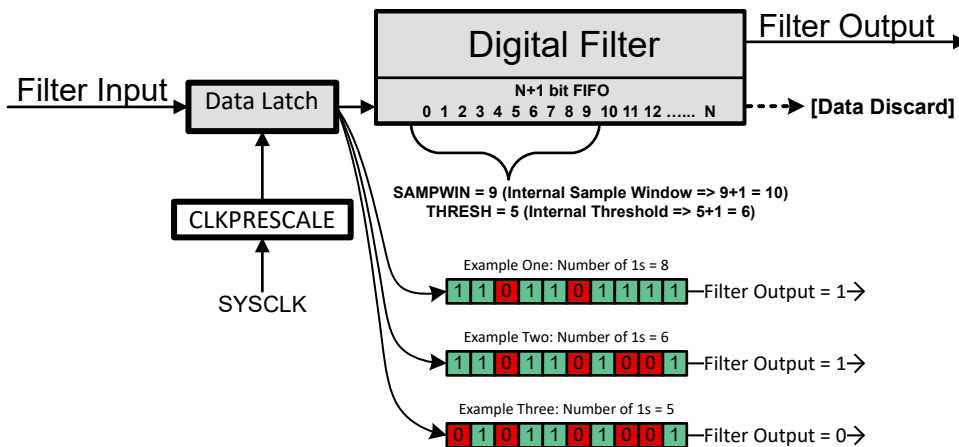
Figure 7-110. Digital Filter Behavior
