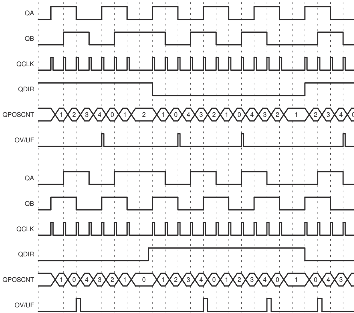
Figure 7-219. Position Counter Underflow/Overflow (QPOSMAX = 4)
