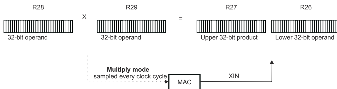
Figure 7-39. MAC Multiply-only Mode- Functional Diagram
