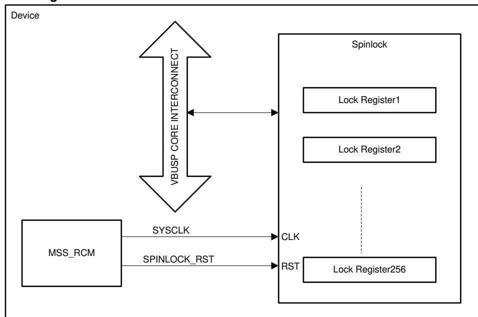
Figure 8-2. SPINLOCK Integration
