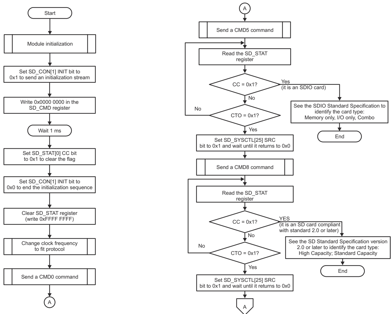
Figure 13-213. MMC/SD/SDIO Controller Card Identification and Selection - Part 1
