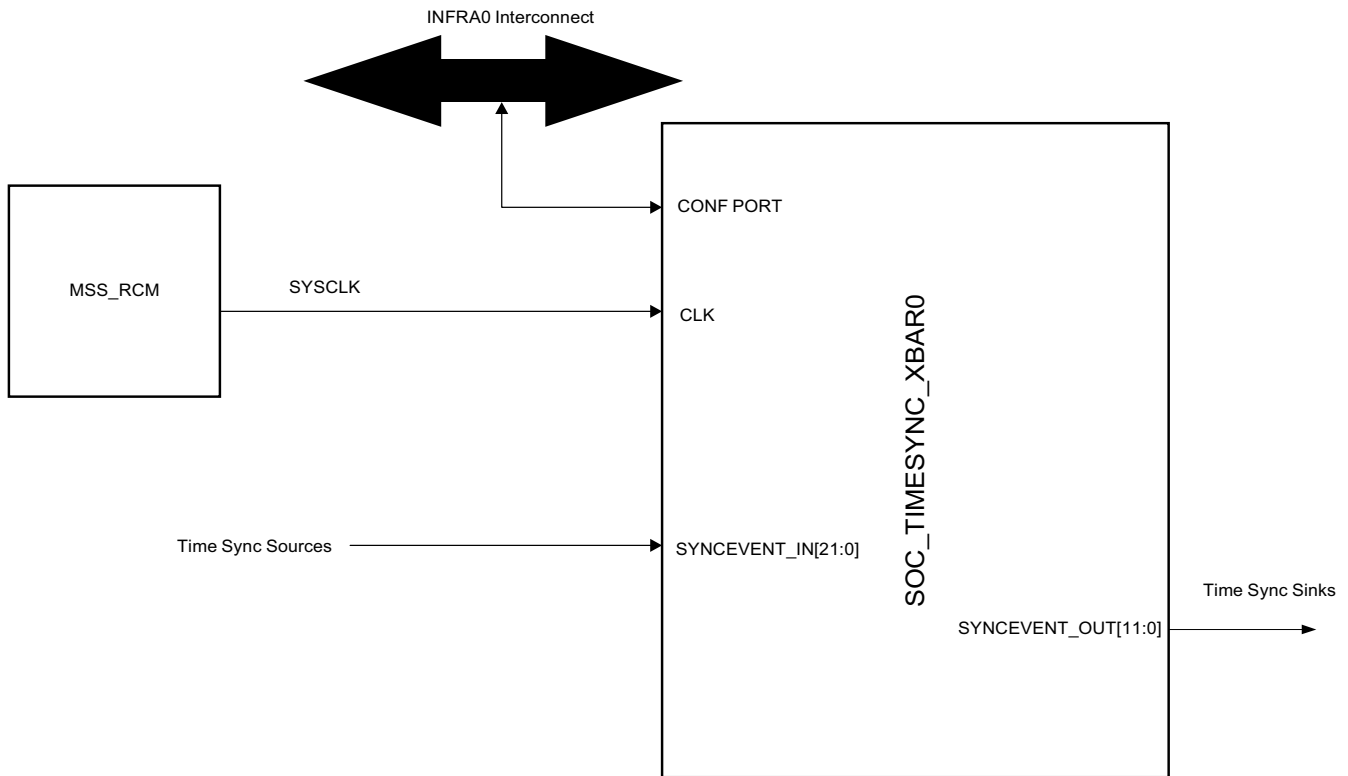
Figure 12-2. SOC_TIMESYNC_XBAR0 Integration
