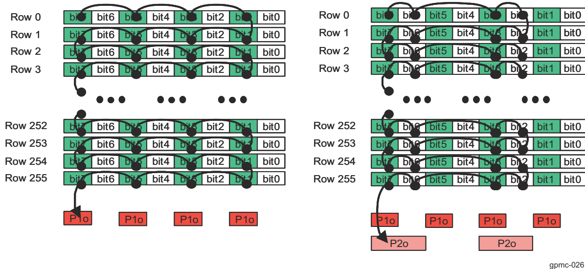
Figure 13-157. Hamming Code Accumulation Algorithm (1/2)
