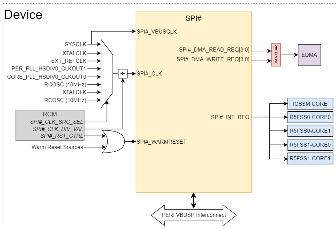
Figure 4-14. SPI Integration
