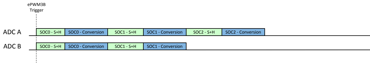
Figure 7-100. Example: Synchronous Operation with Uneven SOC Numbers
