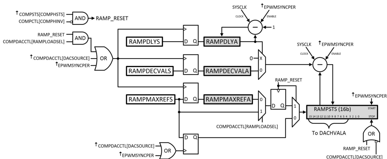
Figure 7-108. Ramp Generator Block Diagram
