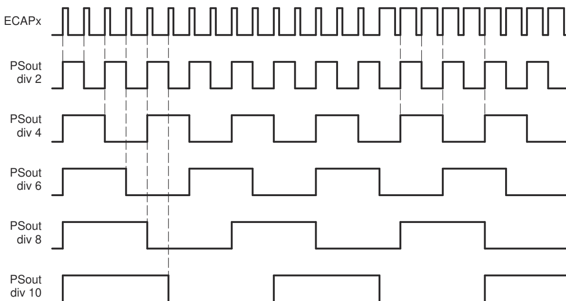
Figure 7-195. Prescale Function Waveforms
