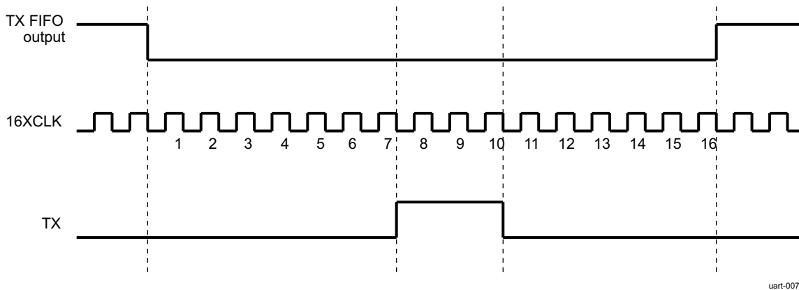
Figure 13-61. IrDA SIR Encoding Mechanism
