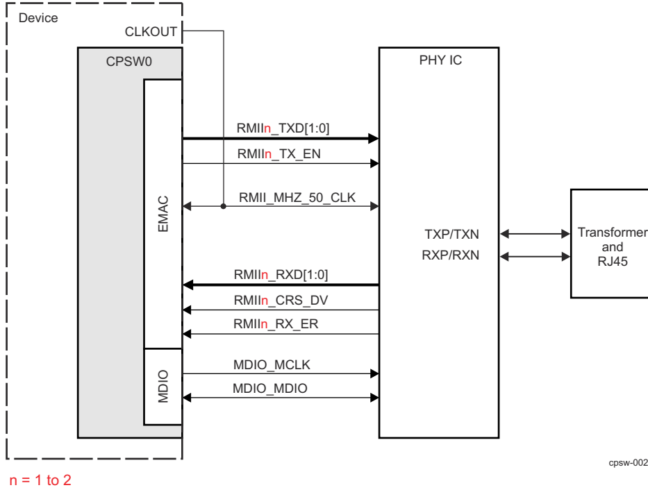
Figure 13-94. RMIi Interface Typical Application (Internal Clock Source)
