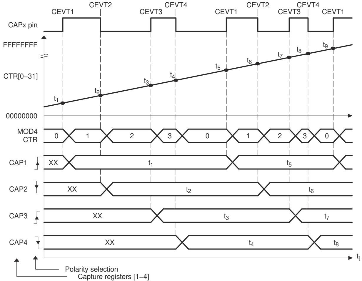
Figure 7-205. Capture Sequence for Absolute Time-stamp With Rising and Falling Edge Detect
