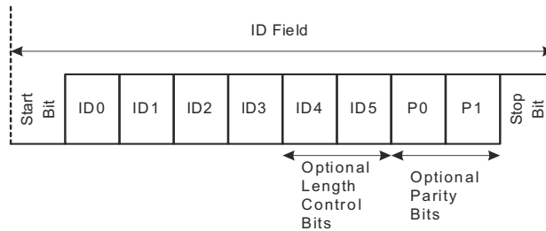
Figure 13-258. ID Field
