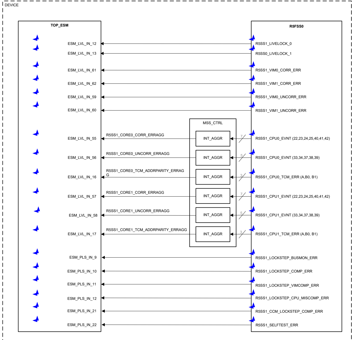
Figure 7-4. R5FSS1 Integration Diagram Continued
