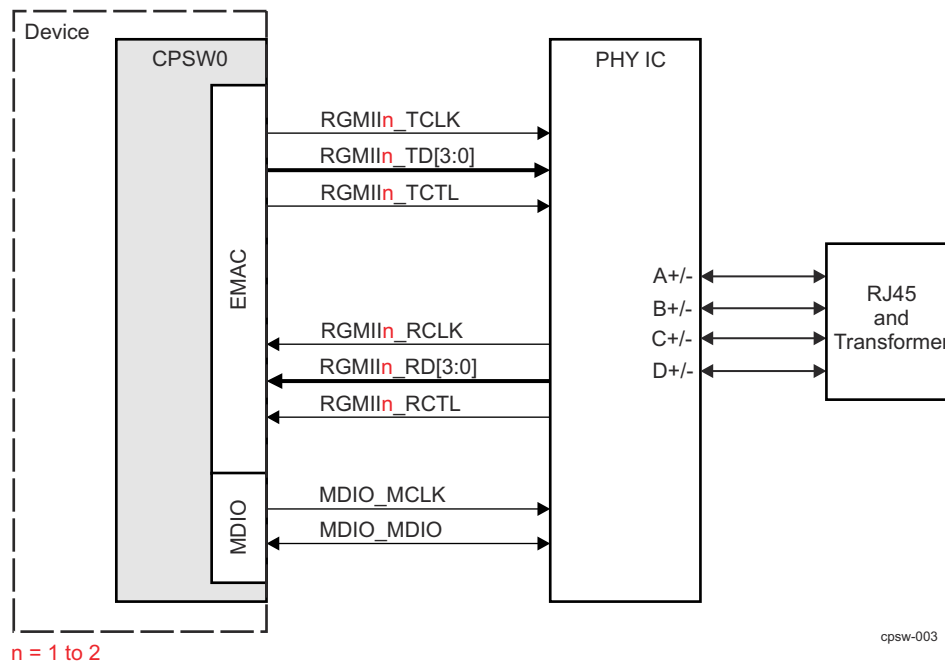
Figure 13-96. RGMII Interface Typical Application
