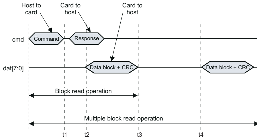
Figure 13-202. Read Data Timeout
