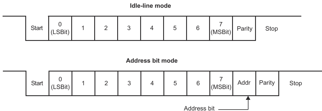
Figure 13-246. Typical SCI Data Frame Formats
