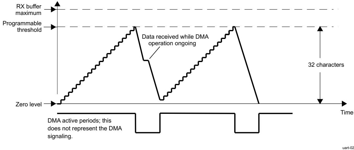
Figure 13-81. UART Receive FIFO DMA Request Generation (32 Characters)
