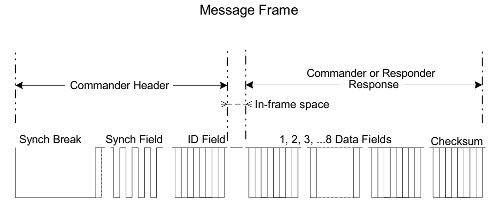
Figure 13-254. LIN Protocol Message Frame Format: Commander Header and Responder Peripheral Response
