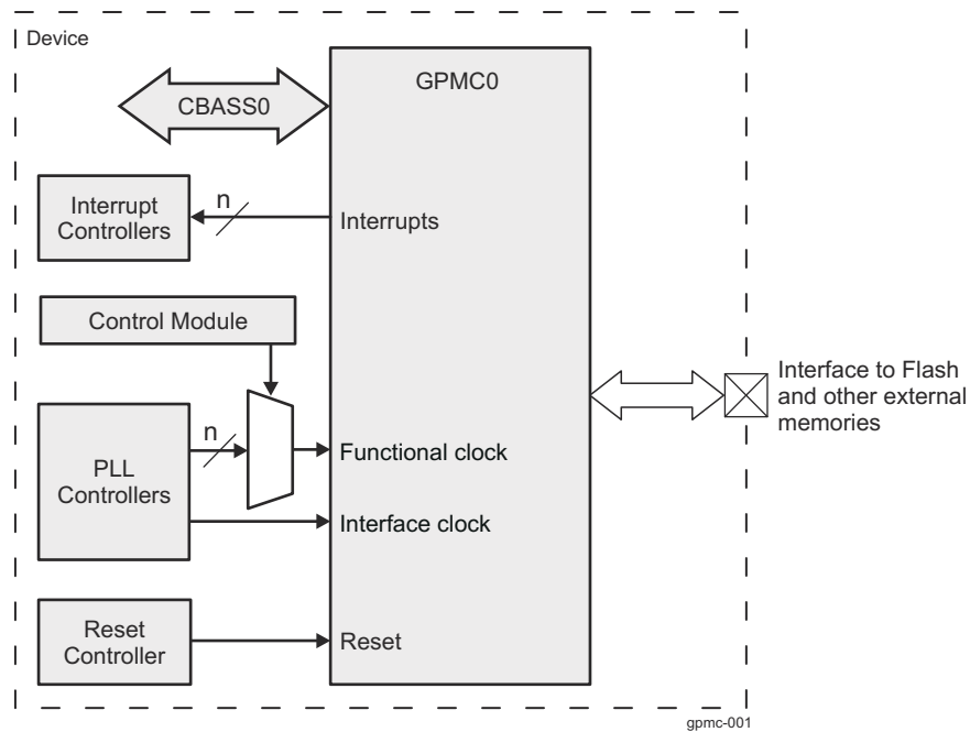
Figure 13-125. GPMC0 Overview
