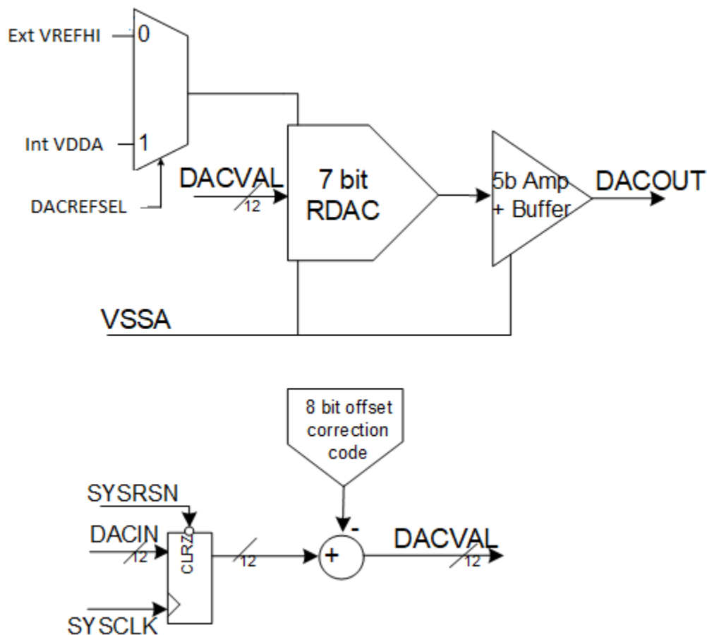
Figure 7-112. DAC Integration Diagram
