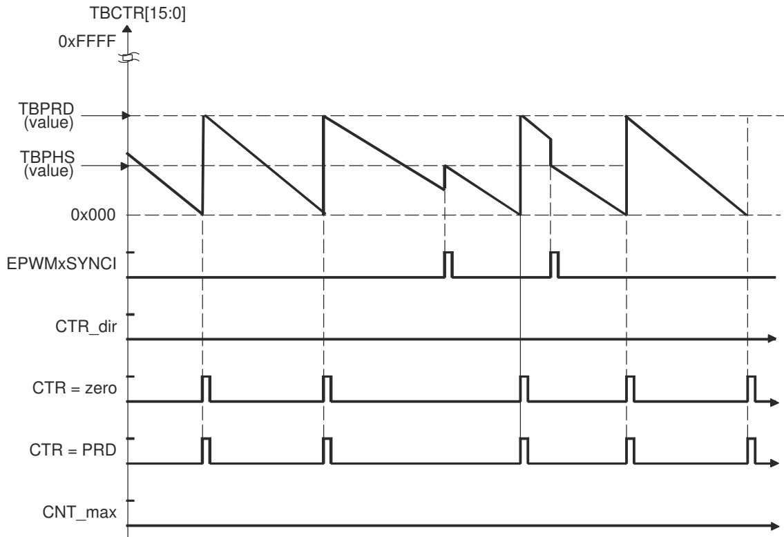
Figure 7-120. Time-Base Down-Count Mode Waveforms
