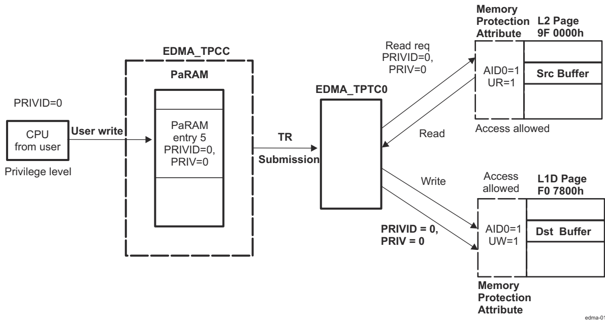
Figure 11-18. Proxy Memory Protection Example
