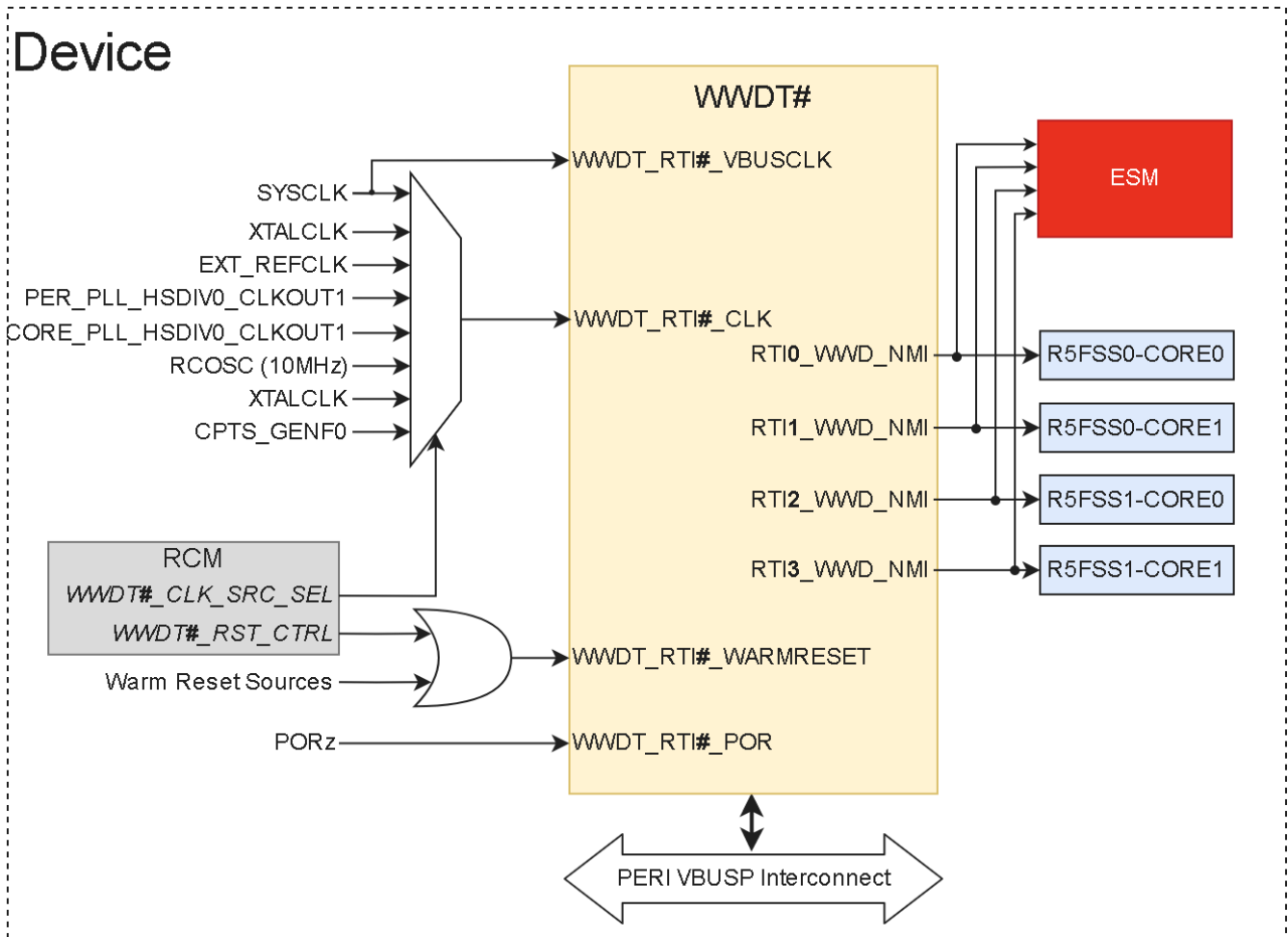
Figure 13-272. WWDT Integration
