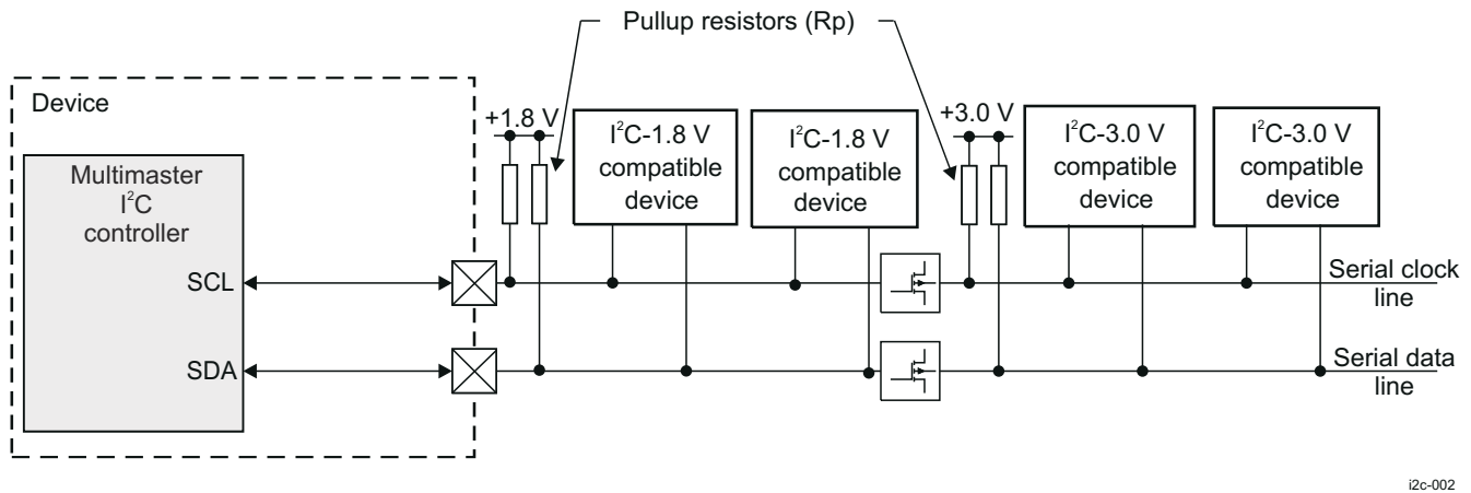
Figure 13-7. I2C and Typical Connections to I2C Devices
