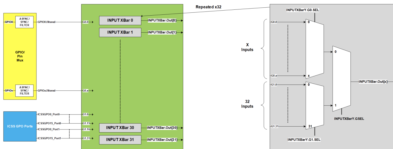
Figure 7-260. INPUTXBAR Functional Block Diagram
