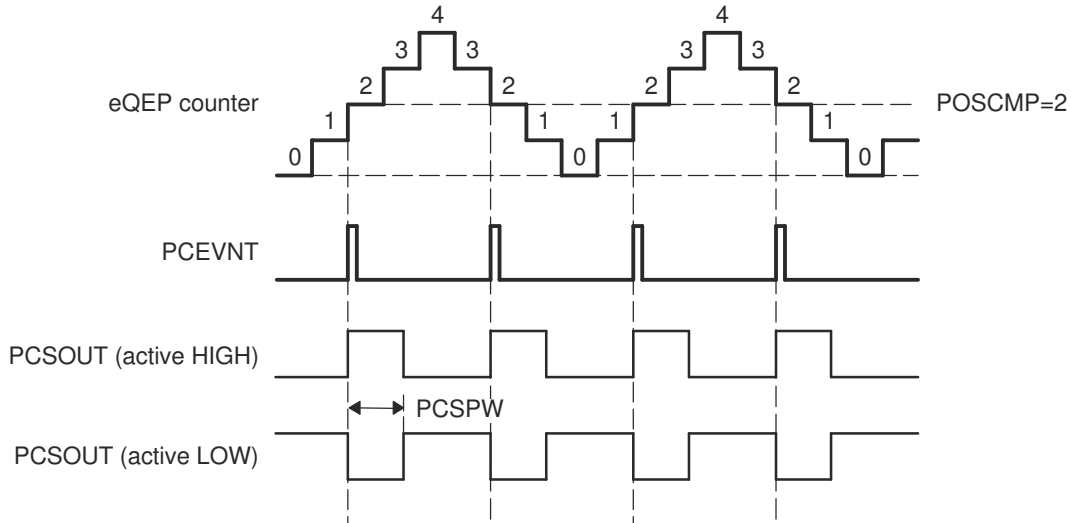
Figure 7-223. eQEP Position-compare Event Generation Points
