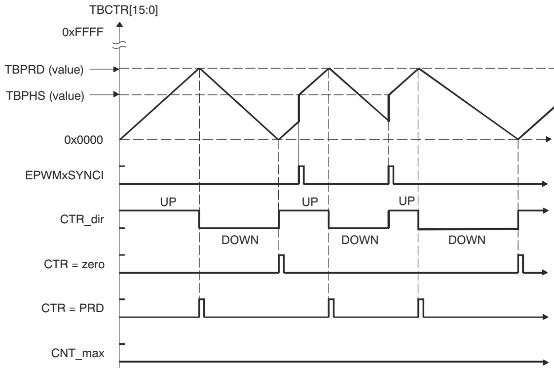
Figure 7-122. Time-Base Up-Down Count Waveforms, TBCTL[PHSDIR = 1] Count Up On Synchronization Event
