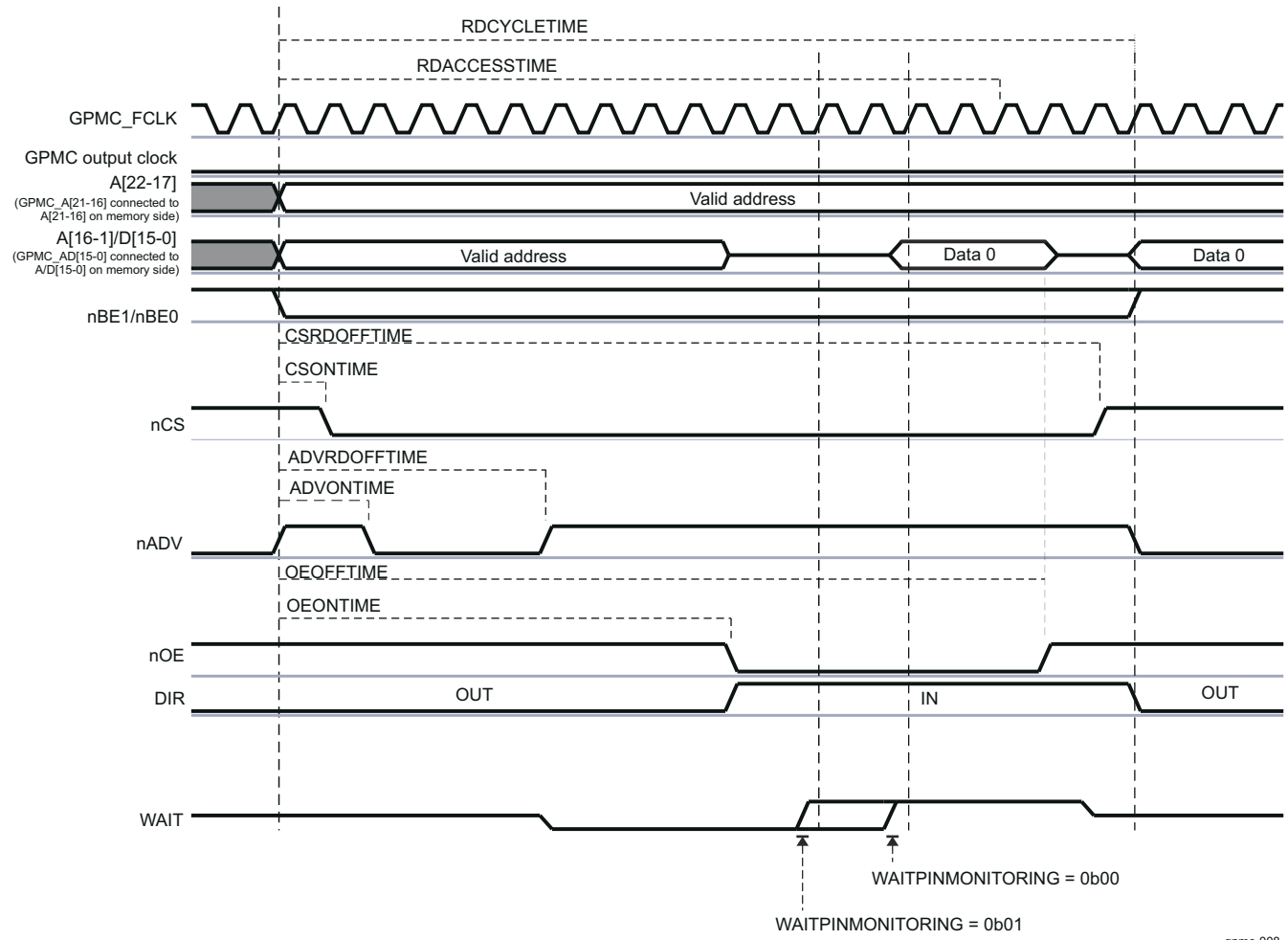
Figure 13-133. Wait Behavior During an Asynchronous Single Read Access (GPMCFCLKDivider = 1)
