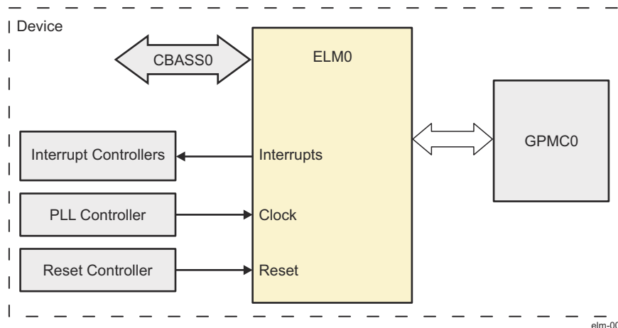
Figure 13-177. ELM0 Overview
