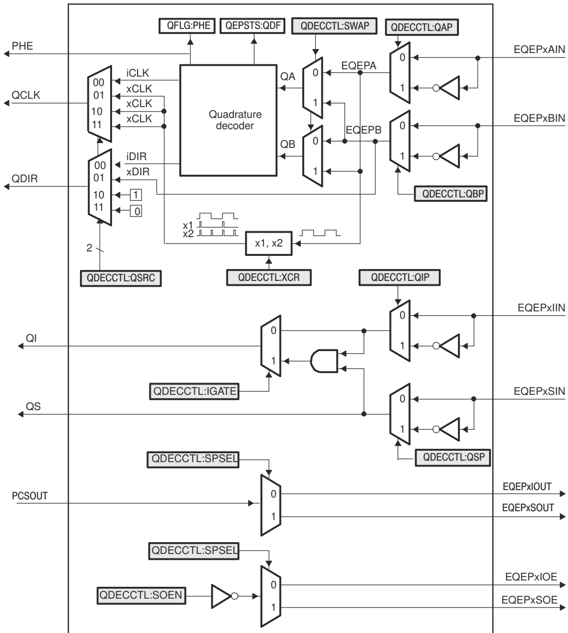
Figure 7-215. Functional Block Diagram of Decoder Unit
