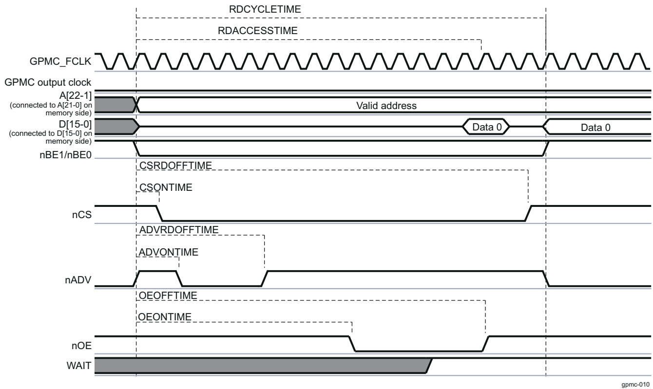
Figure 13-150. Asynchronous Single Read on an Address/Data-non-multiplexed Device
