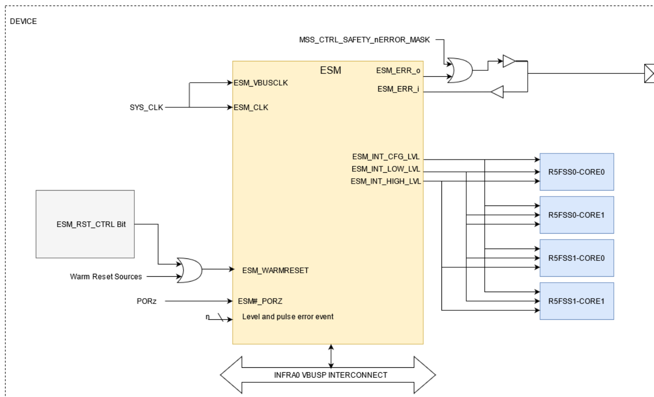
Figure 4-24. ESM Integration Diagram
