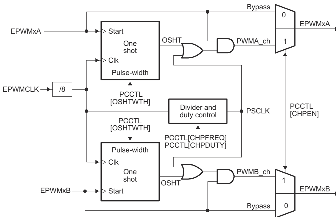
Figure 7-146. PWM Chopper Submodule Operational Details
