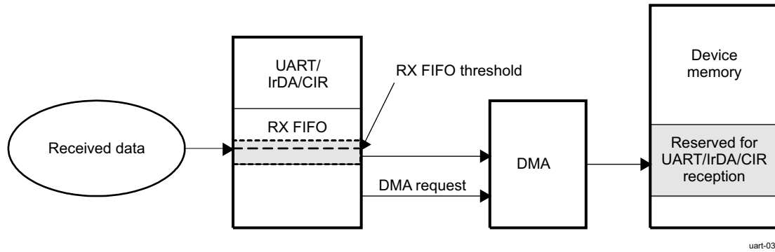
Figure 13-87. DMA Reception
