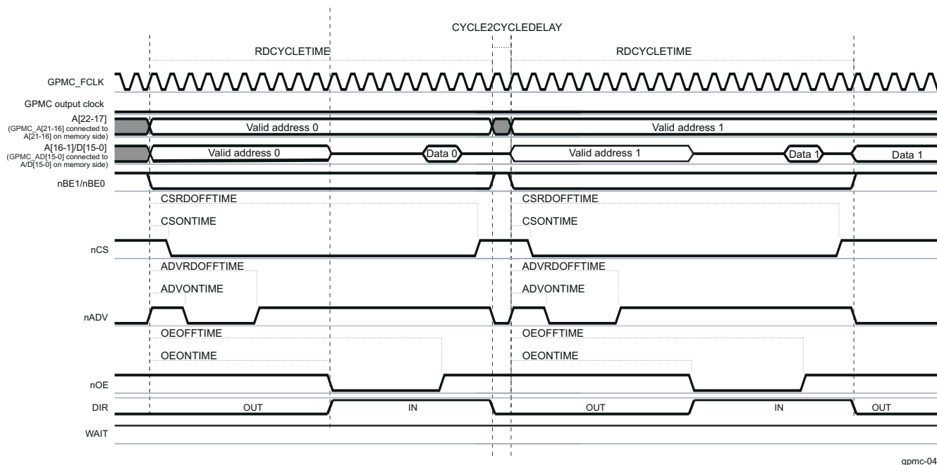
Figure 13-139. Two Asynchronous Single-Read Accesses on an Address/Data-Multiplexed Device (32-Bit Read Split Into 2 x 16-Bit Read)
