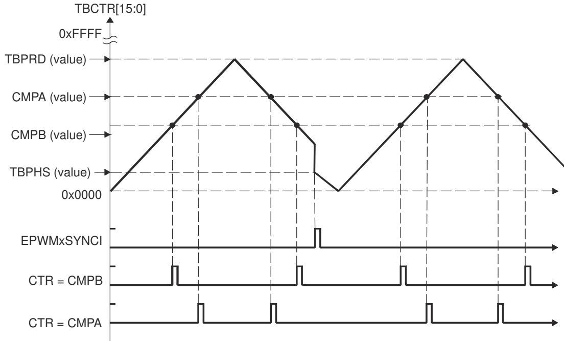
Figure 7-130. Counter-Compare Events In Up-Down-Count Mode, TBCTL[PHSDIR = 0] Count Down On Synchronization Event
