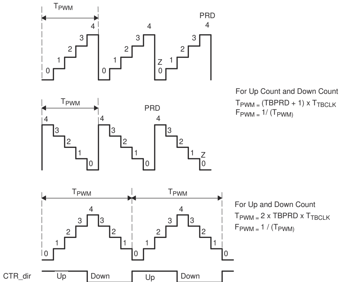
Figure 7-116. Time-Base Frequency and Period
