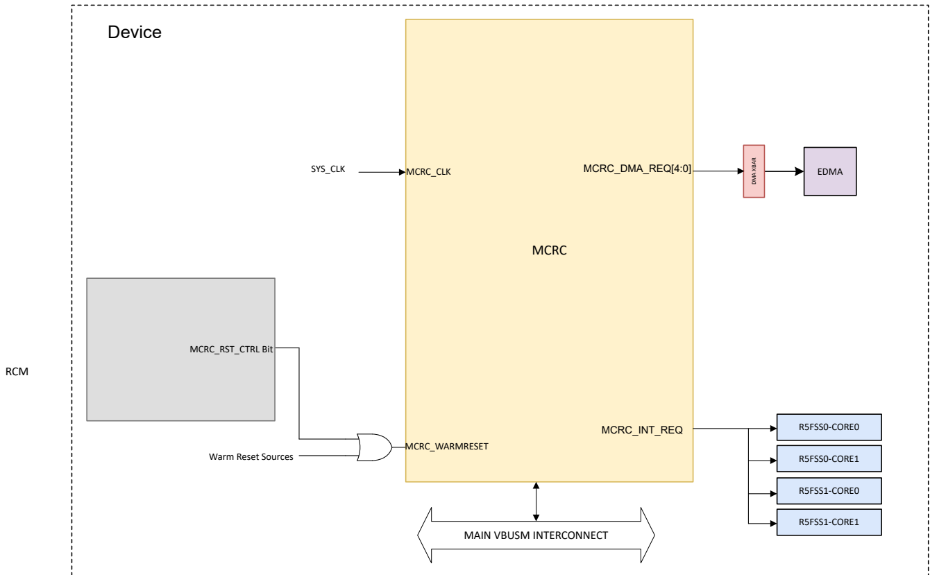
Figure 13-298. MCRC Integration
