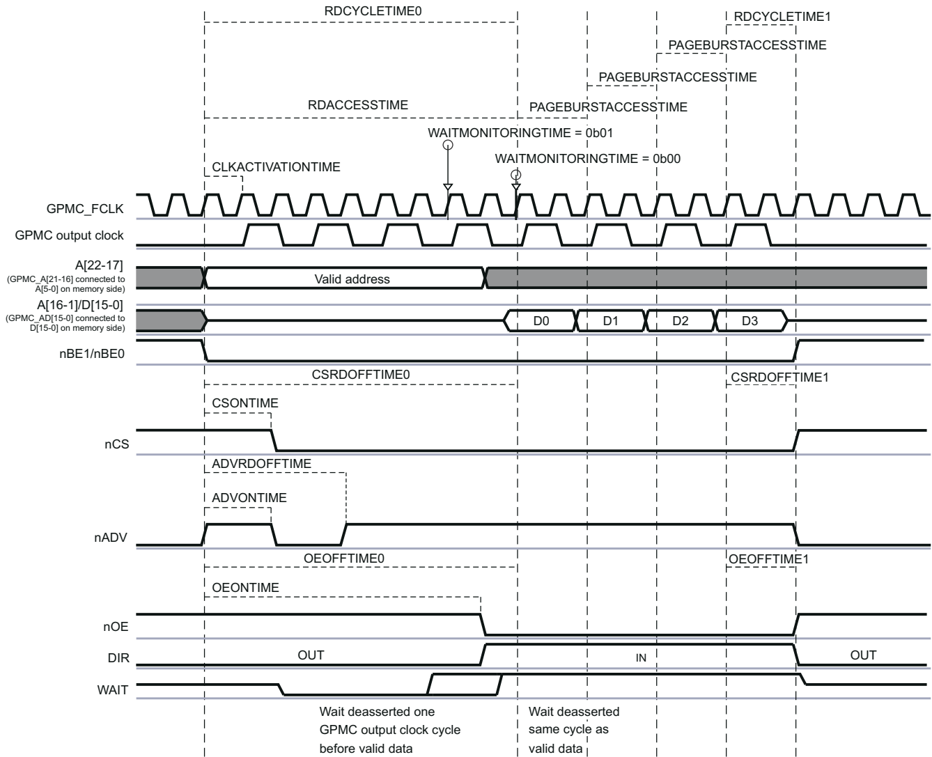
Figure 13-134. Wait Behavior During a Synchronous Read Burst Access
