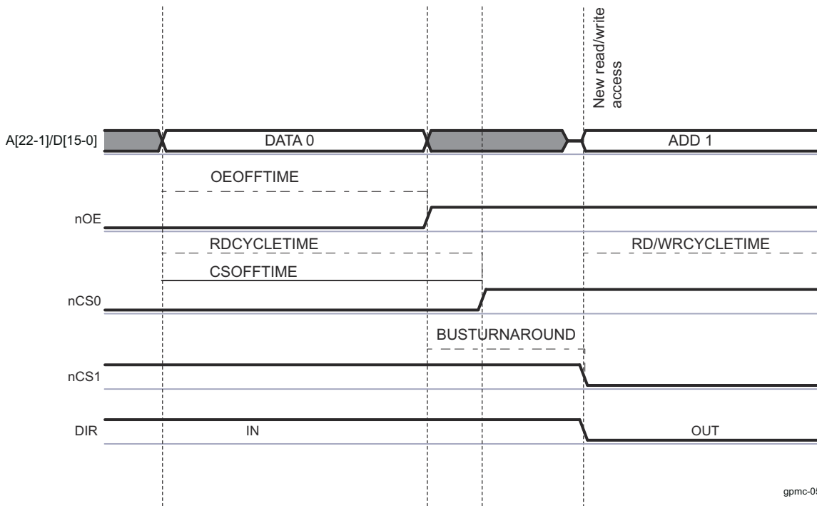
Figure 13-136. Read- to-Read/Write for an Address-Data Multiplexed Device, on Different Chip-Select, With Bus Turnaround
