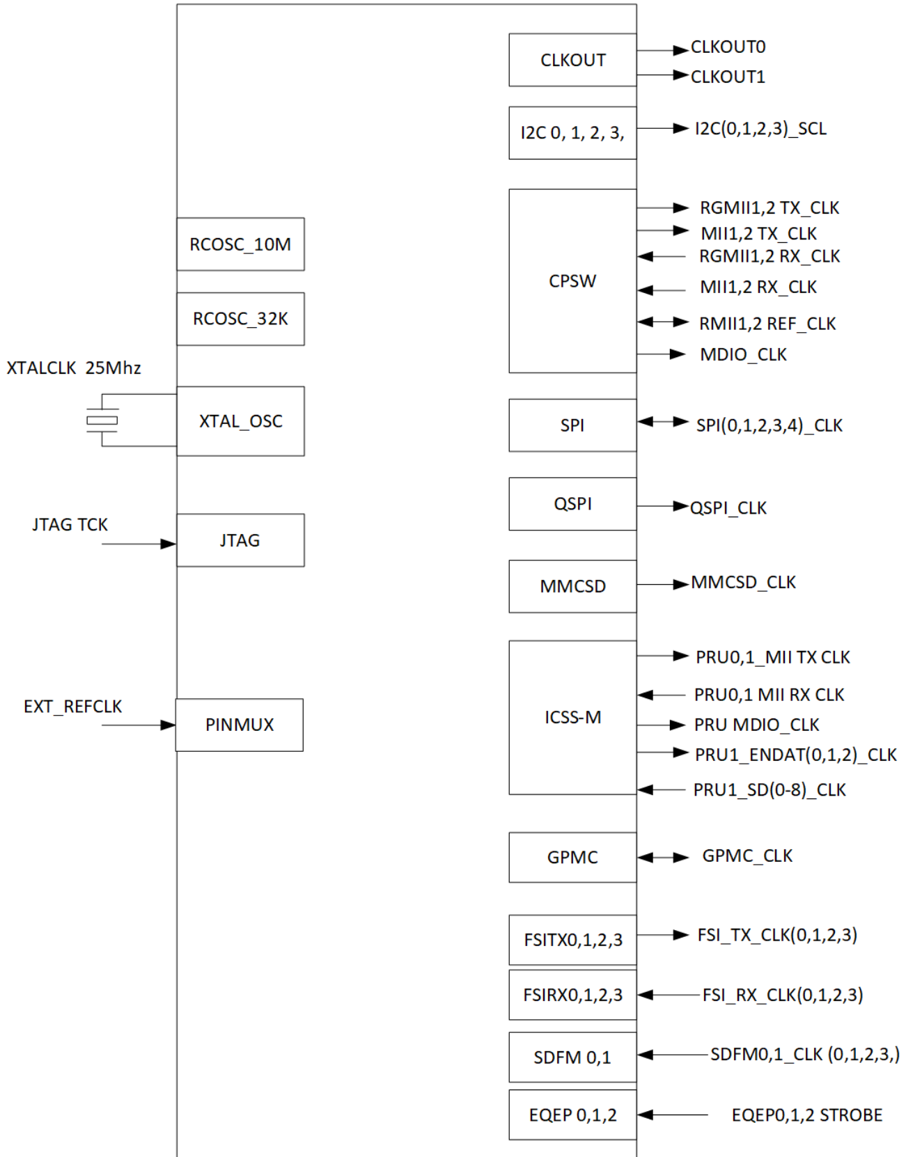
Figure 6-22. External Clocks
