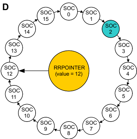
Figure 7-90. Round Robin Priority Example
