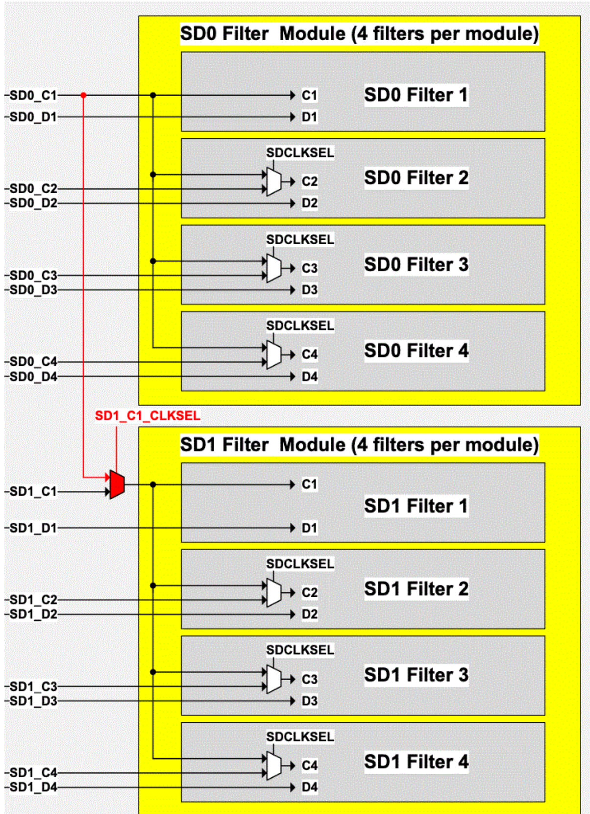
Figure 7-251. SDFM Clock Control
