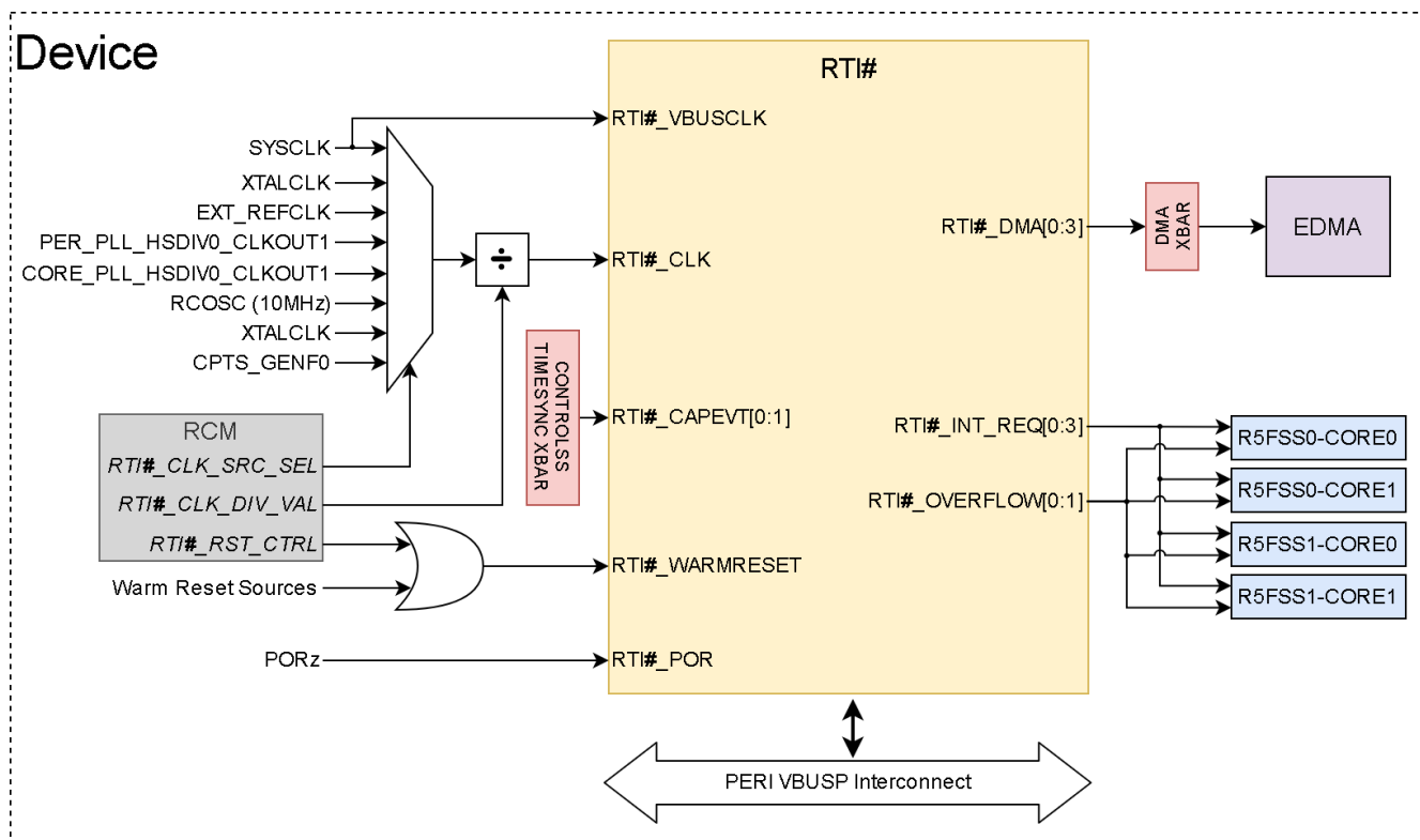
Figure 13-271. RTI Integration
