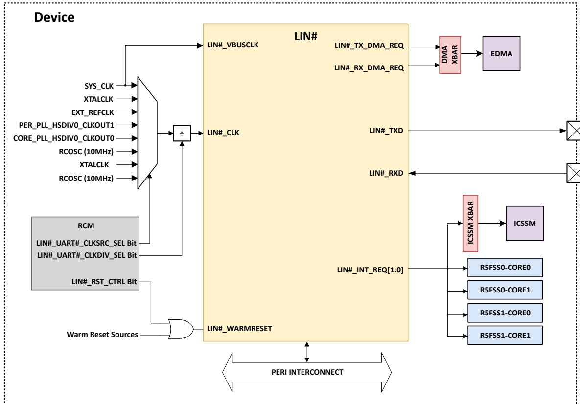
Figure 13-245. LIN Integration
