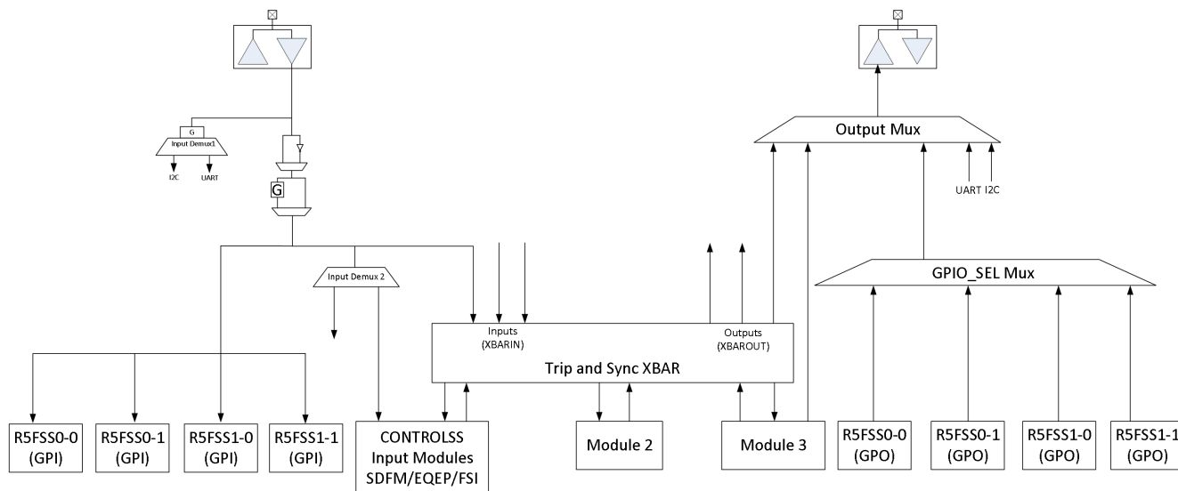
Figure 13-2. GPIO Mux Diagram
