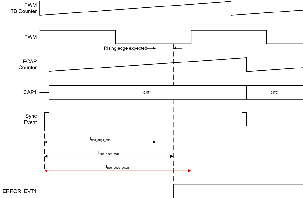
Figure 7-203. ECAP Signal Monitoring Unit Edge Error Example
