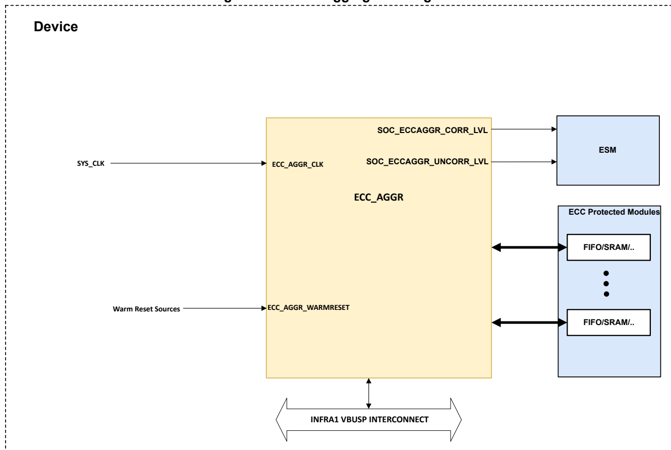
Figure 4-25. ECC Aggregator Integration
