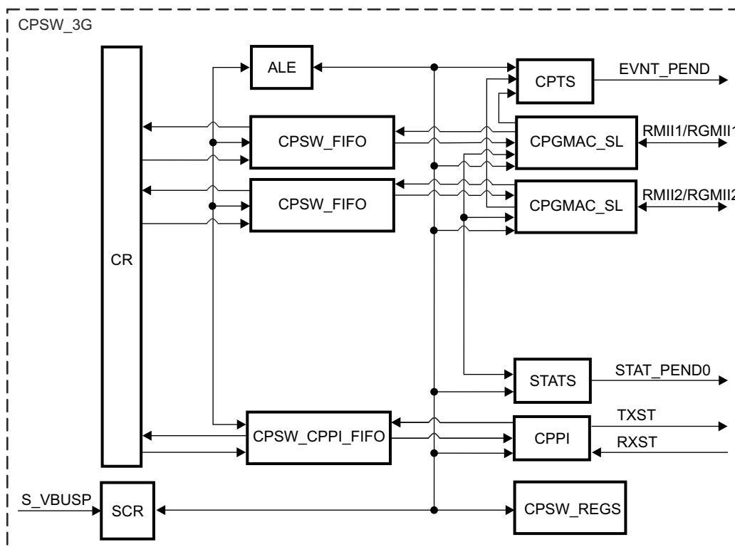
Figure 13-99. CPSW_3G Block Diagram
