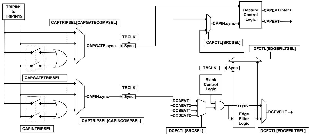
Figure 7-123. CAPIN and CAPGATE Source Selection
