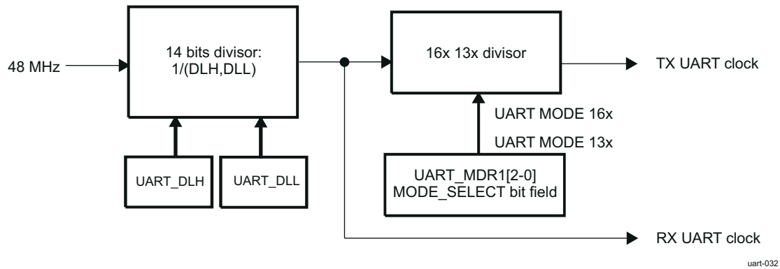
Figure 13-88. UART Baud Rate Generation
