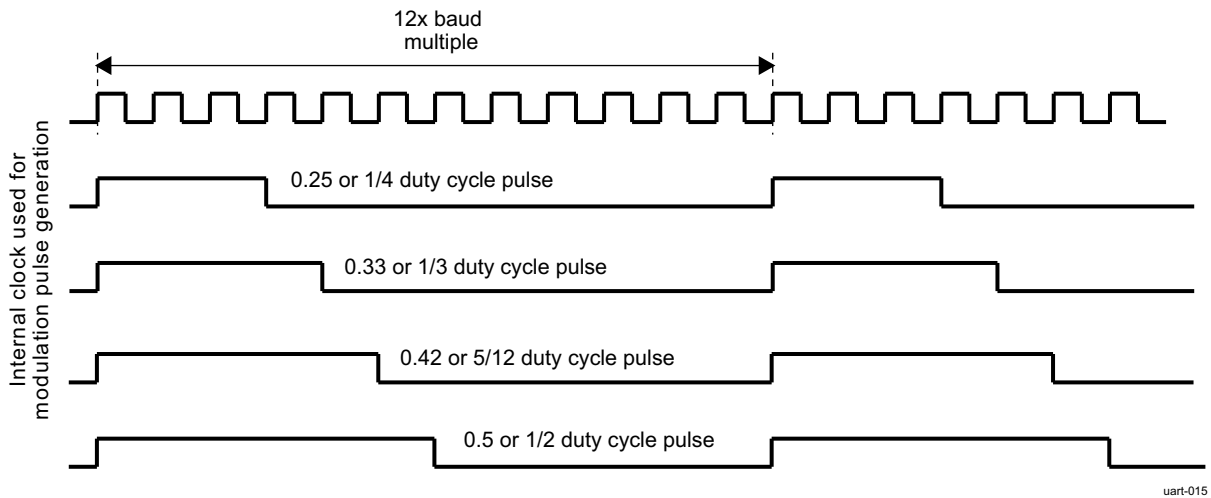
Figure 13-70. CIR Modulation Duty Cycle
