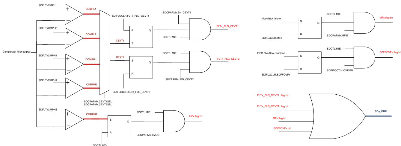
Figure 7-258. SDFM Error (SD_ERR) Interrupt Sources
