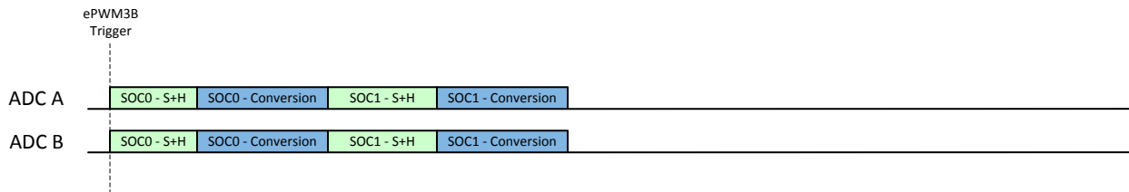
Figure 7-98. Example: Basic Synchronous Operation
