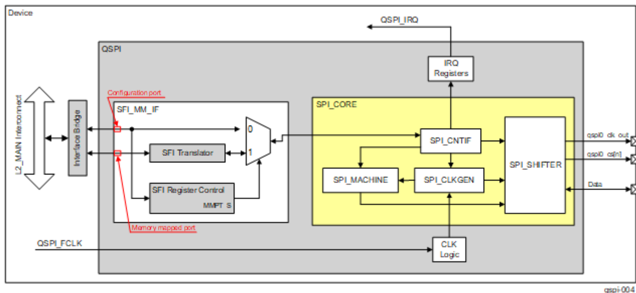
Figure 13-218. QSPI Block Diagram
