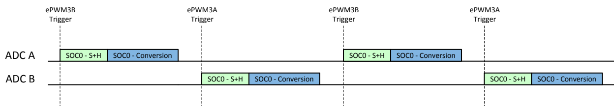
Figure 7-102. Example: Synchronous Equivalent Operation with Non-Overlapping Conversions
