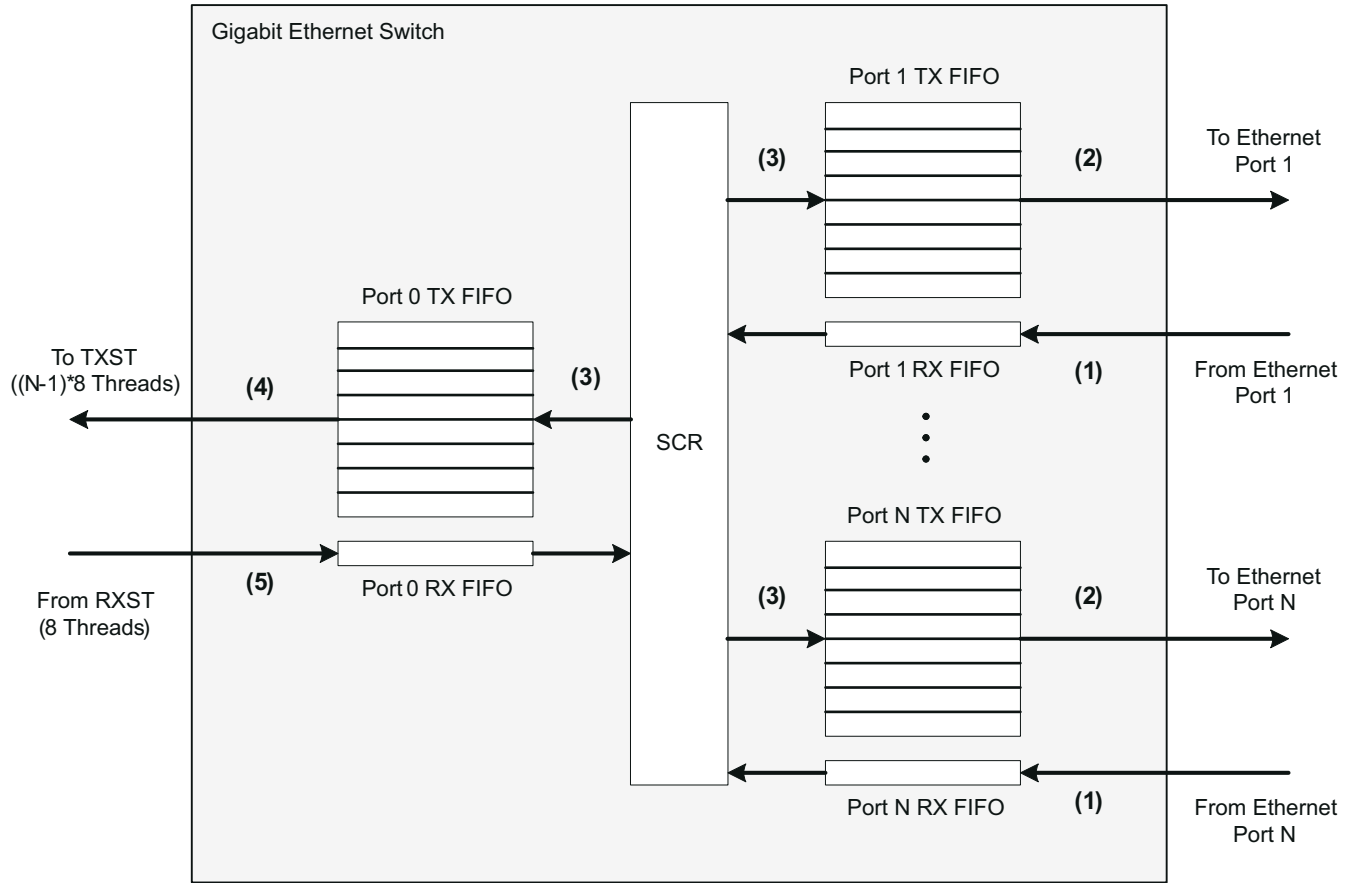
Figure 13-100. Gigabit Ethernet Switch Priority Mapping and Transmit VLAN Processing
