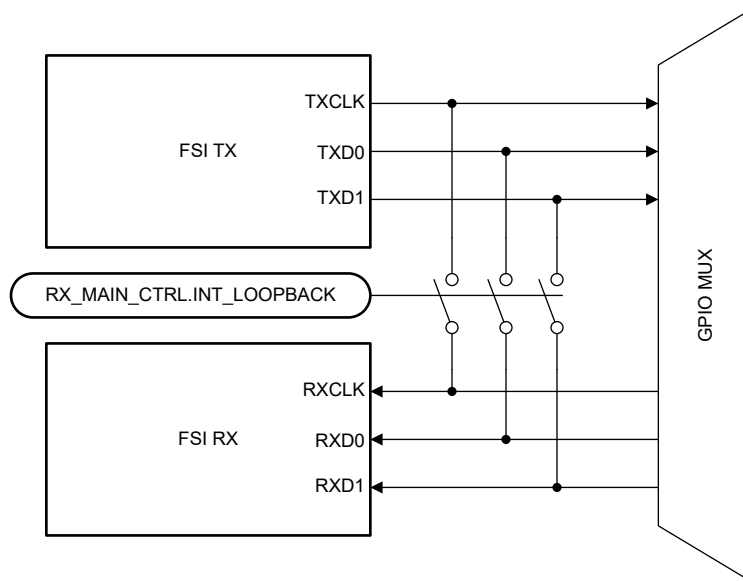
Figure 7-238. FSI with Internal Loopback
