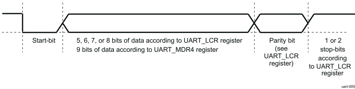
Figure 13-57. UART Frame Data Format
