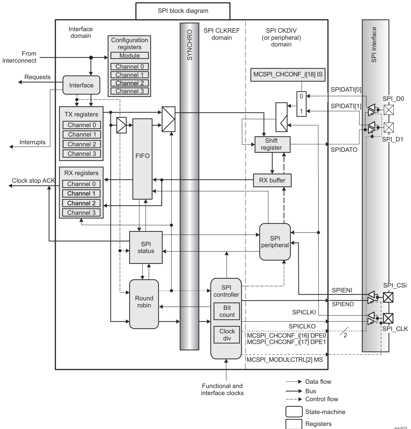
Figure 13-37. MCSPI Block Diagram
