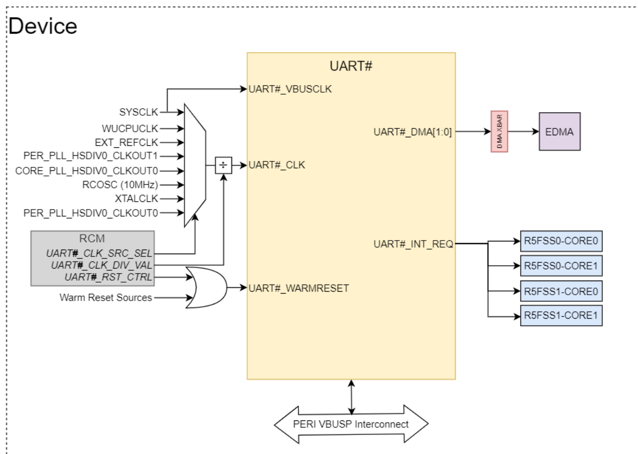
Figure 13-76. UART Integration
