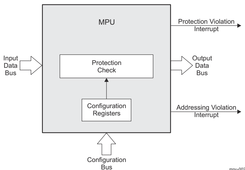
Figure 3-4. MPU Block Diagram
