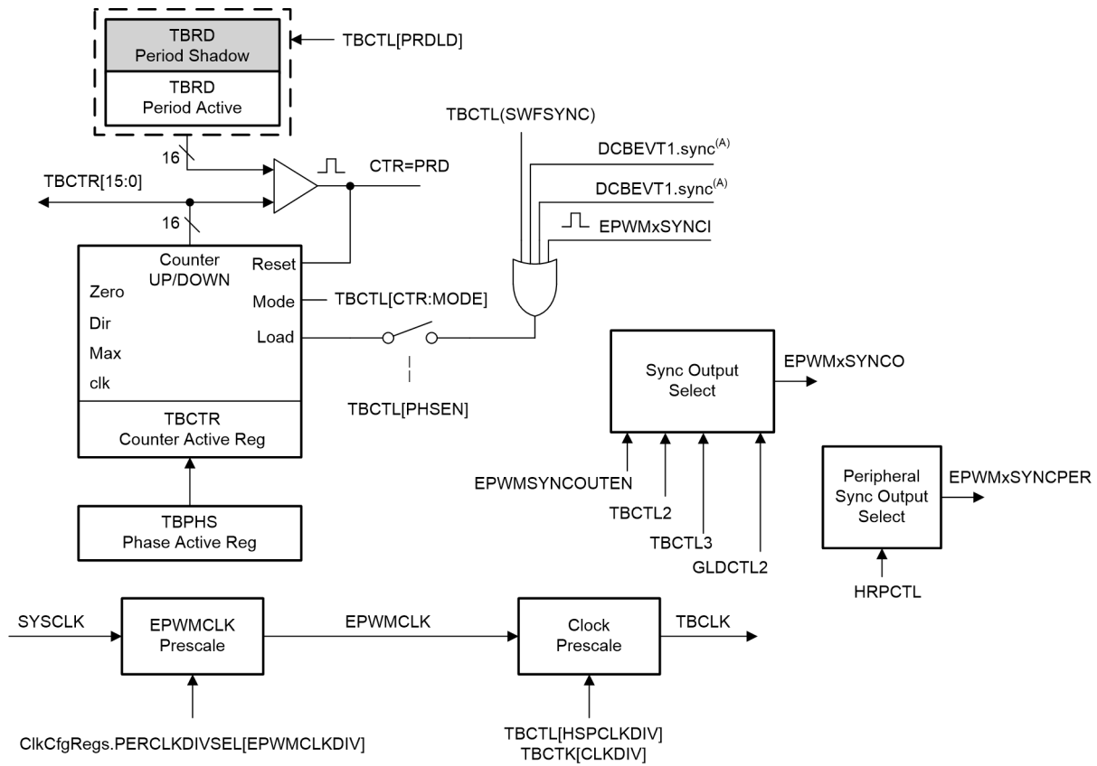
Figure 7-115. Time-Base Submodule Signals and Registers
