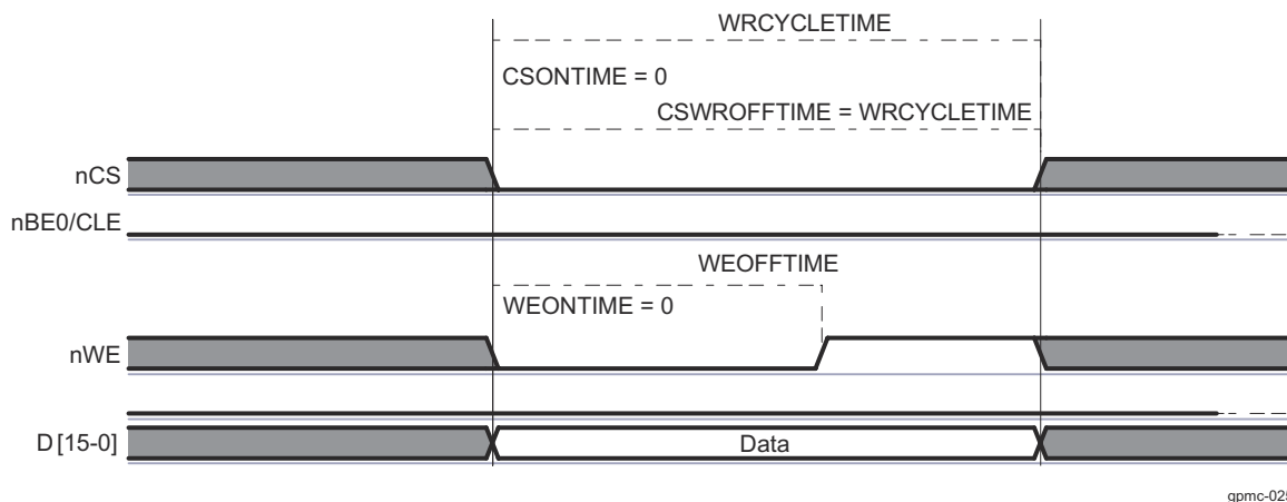
Figure 13-156. NAND Data Write Cycle
