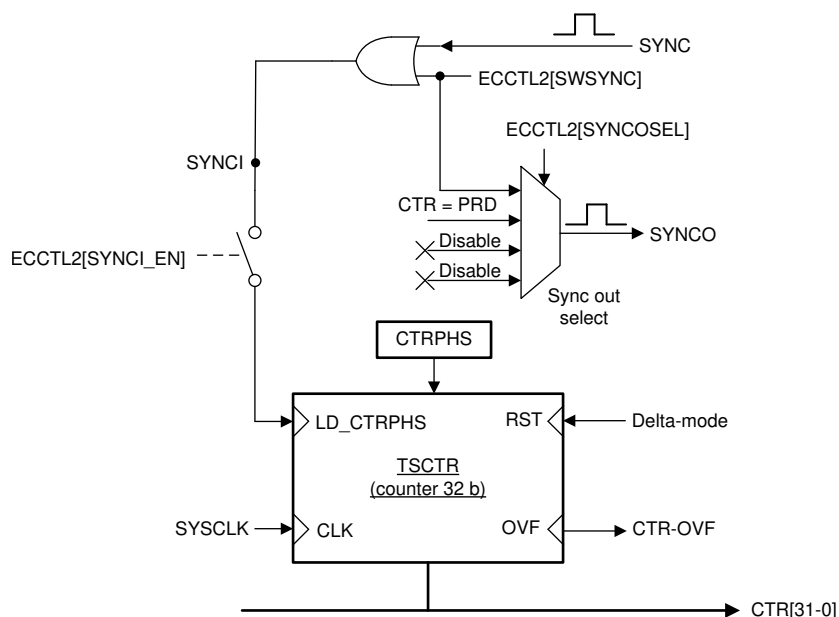
Figure 7-197. Details of the Counter and Synchronization Block
