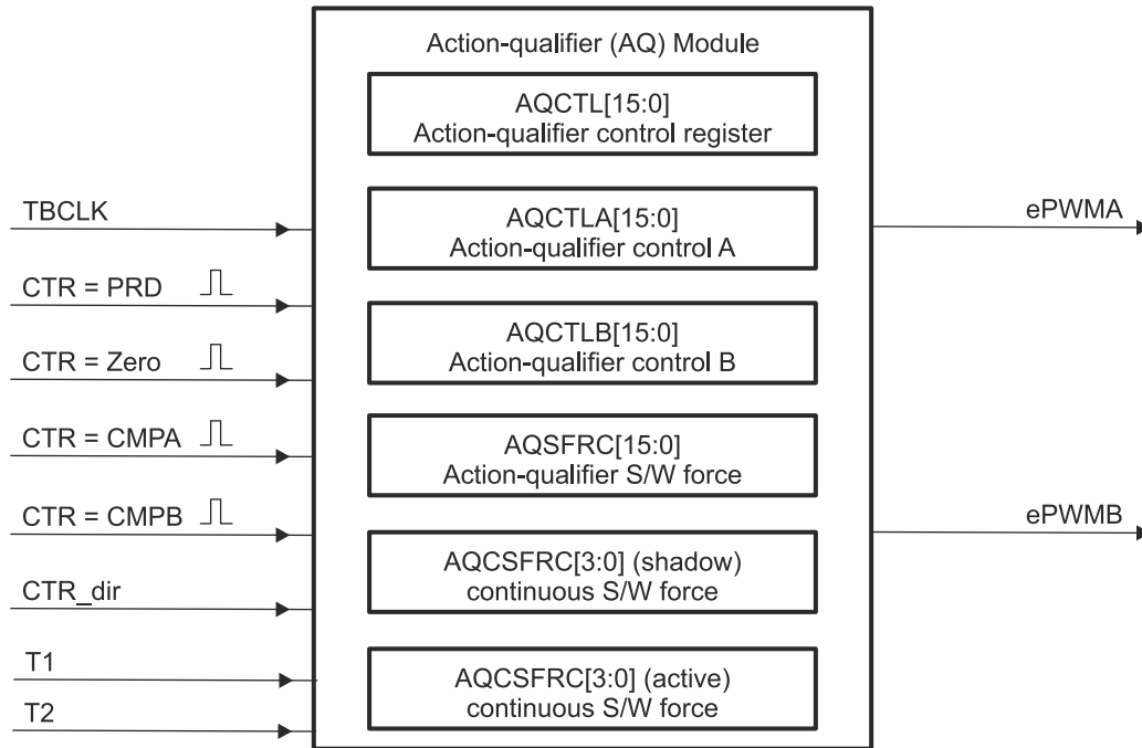
Figure 7-132. Action-Qualifier Submodule Inputs and Outputs
