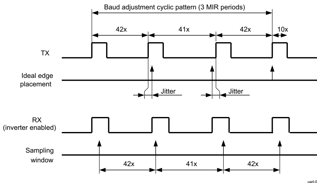
Figure 13-65. MIR Baud Rate Adjustment Mechanism
