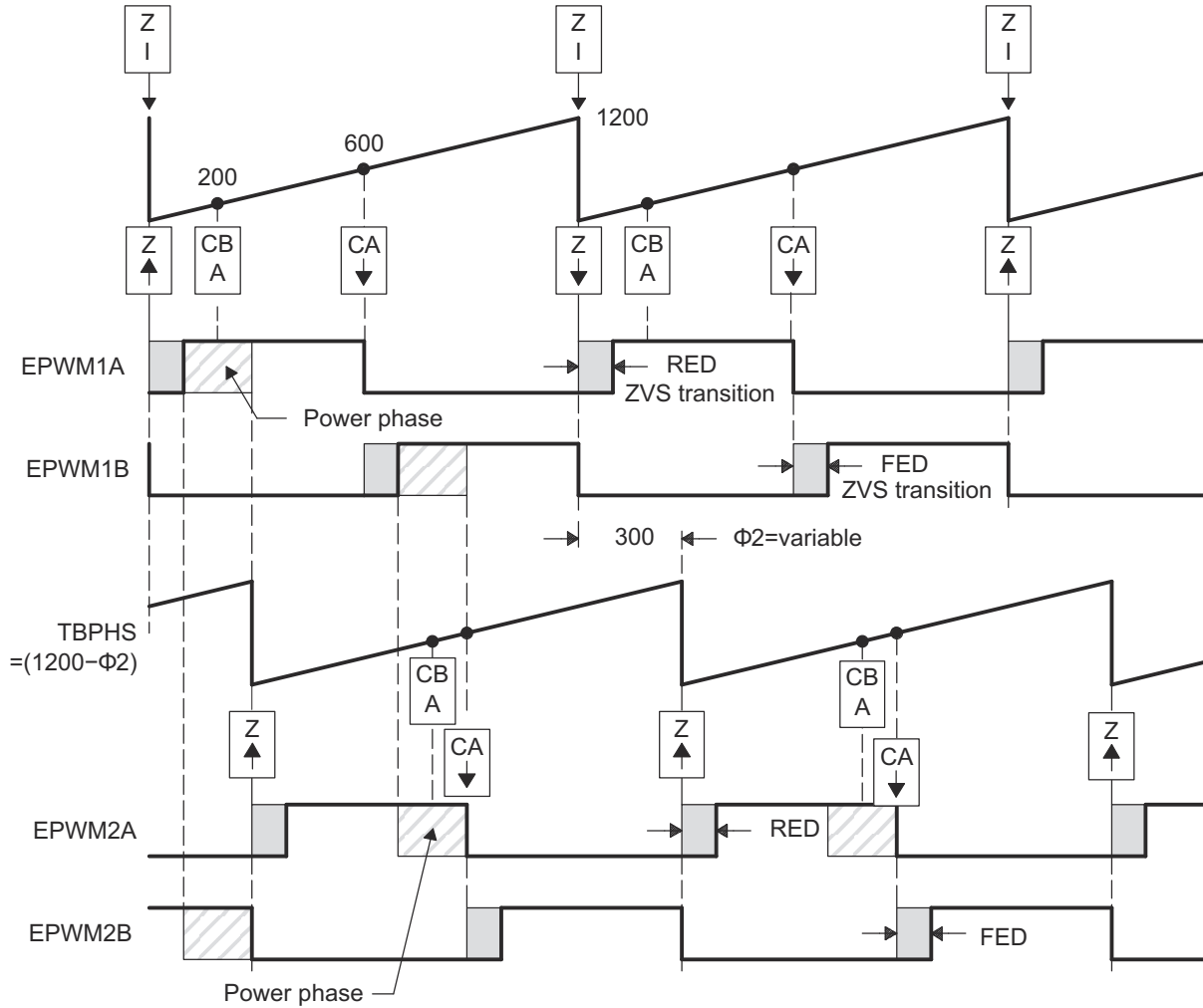
Figure 7-172. ZVS Full-H Bridge Waveforms
