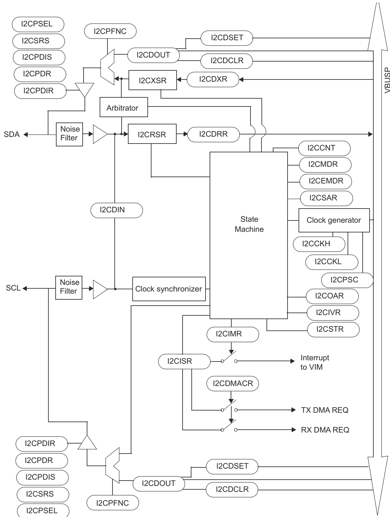
Figure 13-19. I2C Block Diagram
