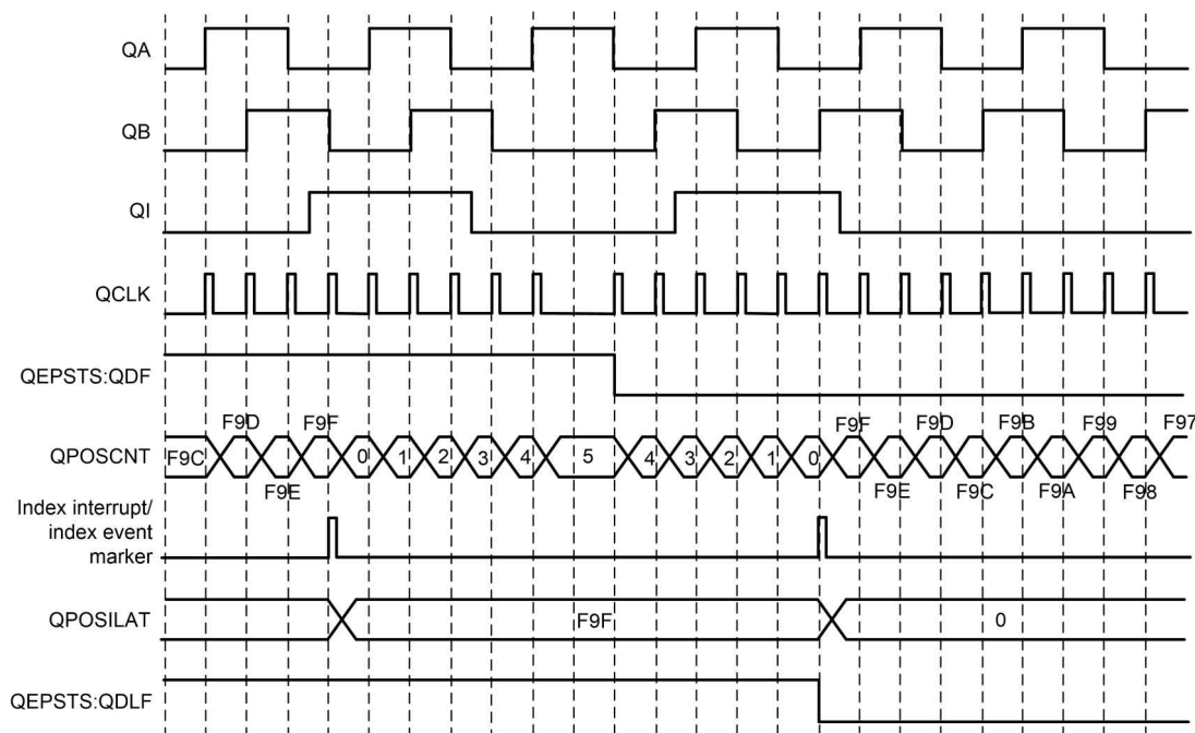
Figure 7-218. Position Counter Reset by Index Pulse for 1000 Line Encoder (QPOS MAX = 3999 or 0xF9F)
