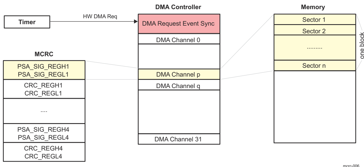
Figure 13-302. Semi-CPU Mode With Hardware Timer Trigger
