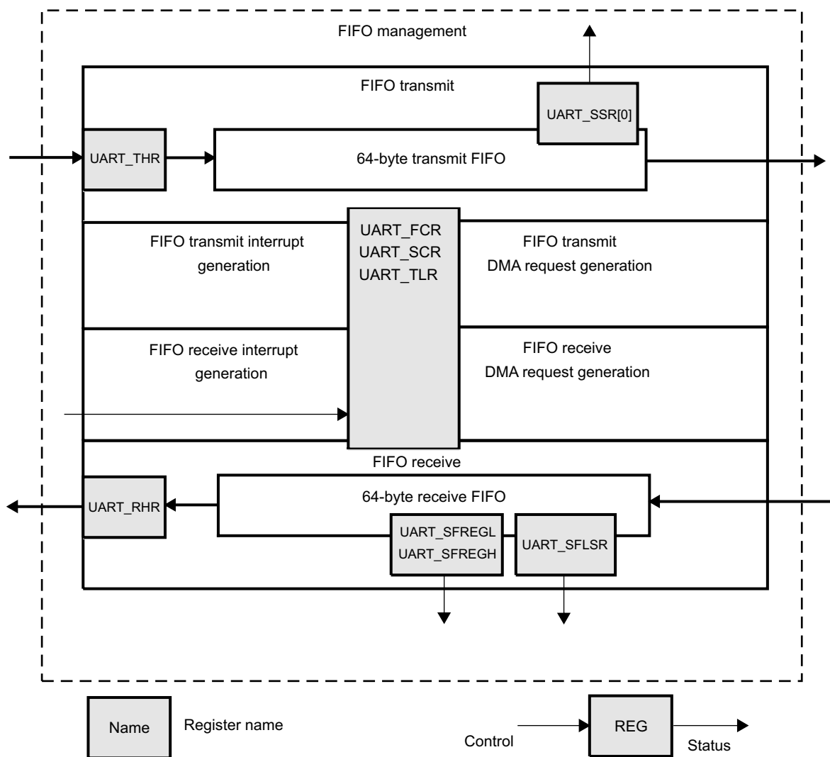
Figure 13-78. UART FIFO Management Registers
