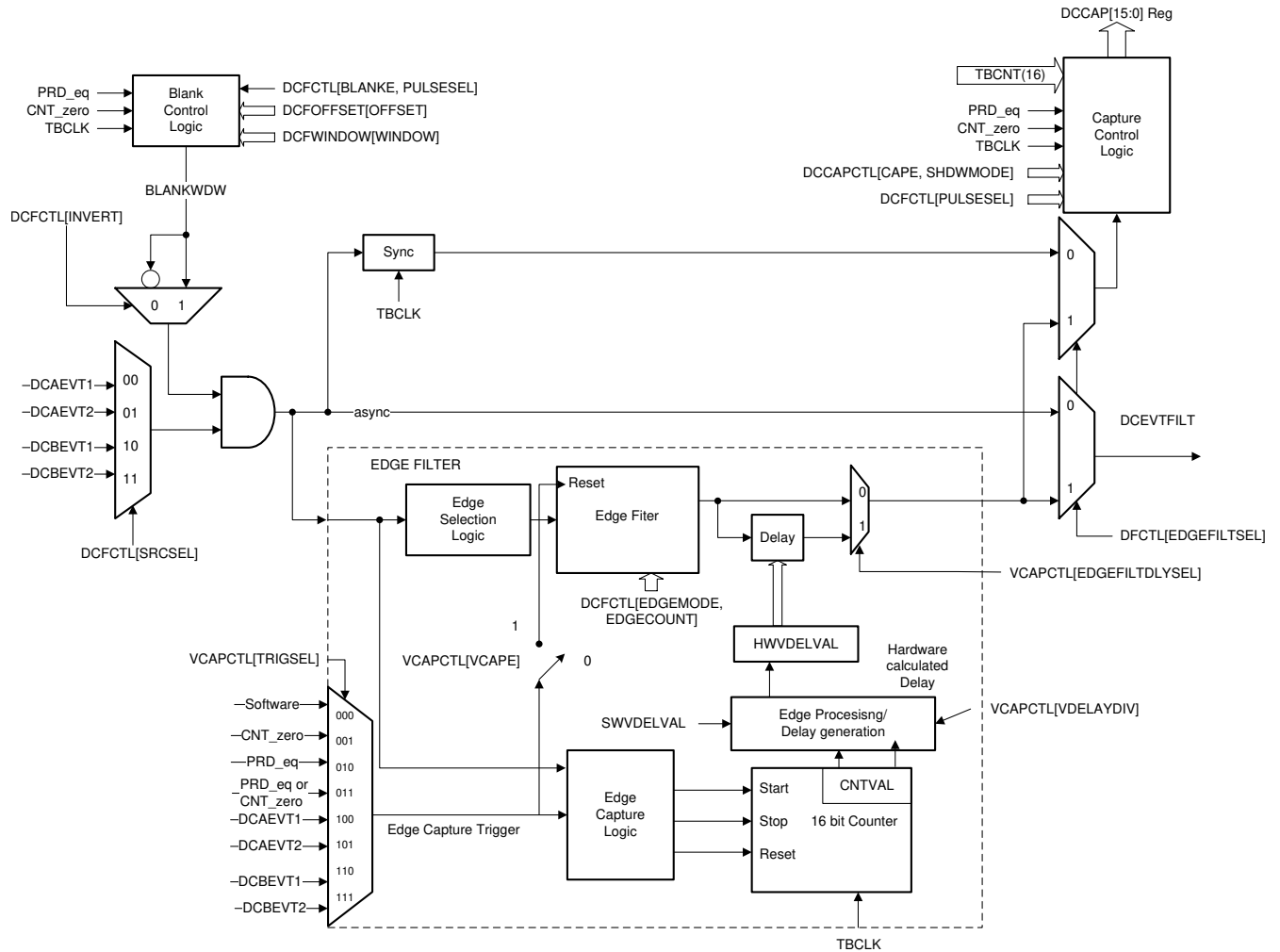
Figure 7-156. Valley Switching
