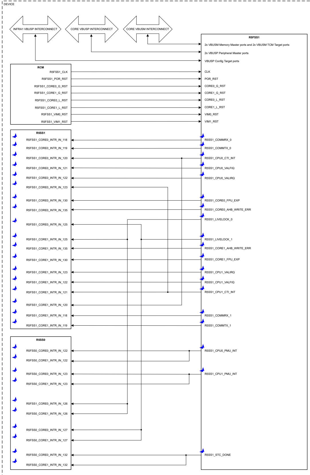
Figure 7-3. R5FSS1 Integration Diagram
