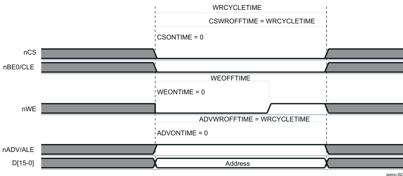
Figure 13-154. NAND Address Latch Cycle
