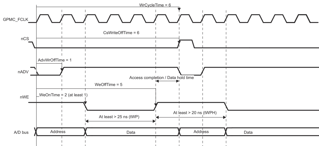
Figure 13-171. Asynchronous Single Write Access (Timing Parameters in Clock Cycles)
