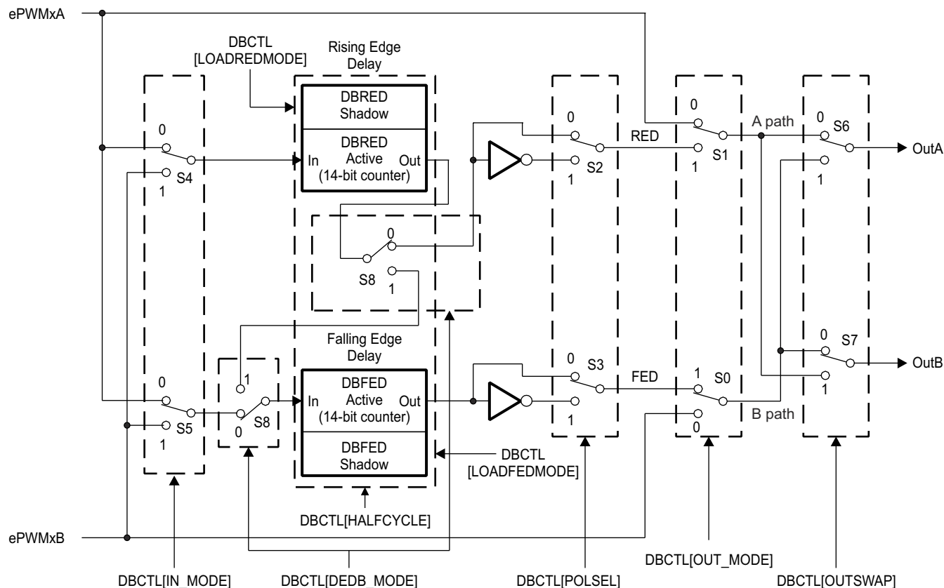
Figure 7-144. Configuration Options for the Dead-Band Submodule
