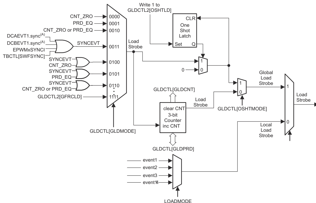
Figure 7-125. Global Load: Signals and Registers
