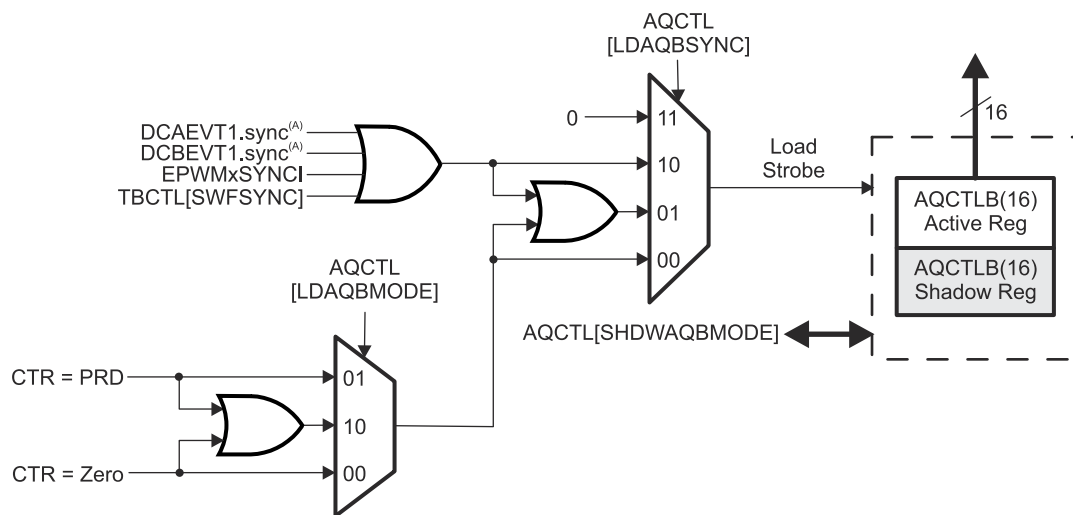
Figure 7-135. AQCTL[SHDWAQBMODE]
