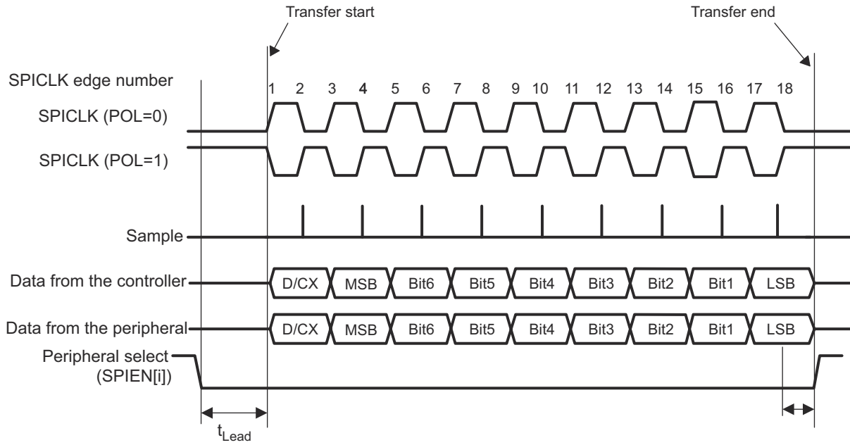
Figure 13-31. Extended MCSPI Transfer With a Start-Bit (SBE = 1)
