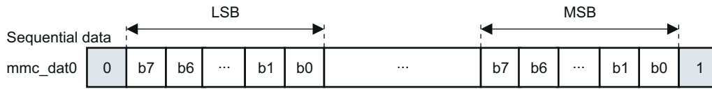
Figure 13-191. Data Packet for Sequential Transfer (1-Bit)
