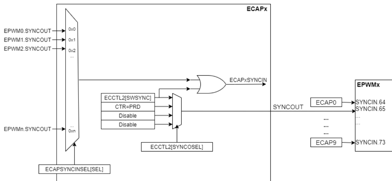
Figure 7-198. eCAP Synchronization Scheme
