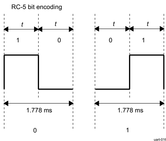
Figure 13-71. UART RC-5 Bit Encoding
