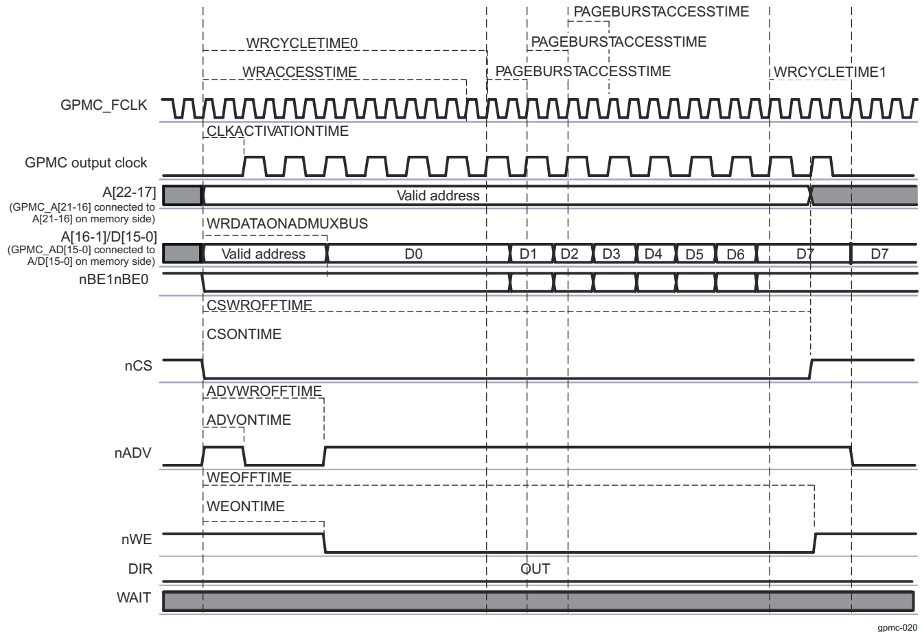
Figure 13-148. Synchronous Multiple Write (Burst Write) in Address/Data-Multiplexed Mode
