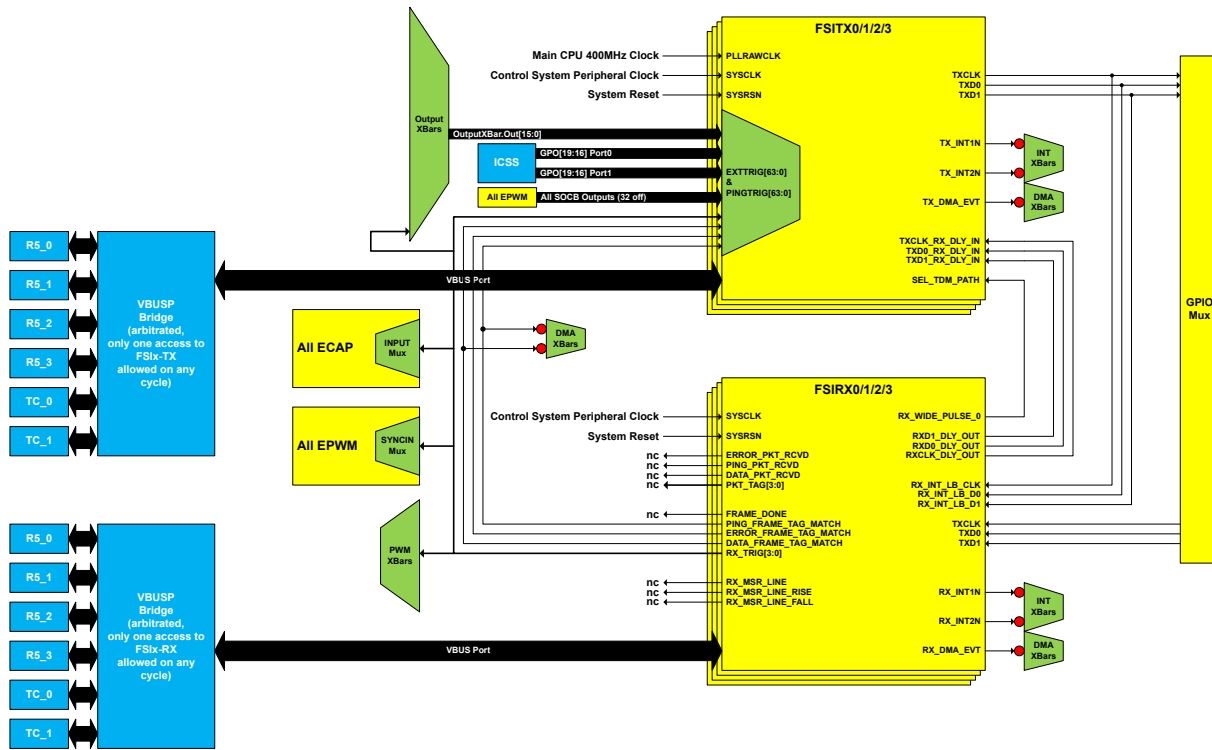
Figure 4-6. FSI Integration Diagram
