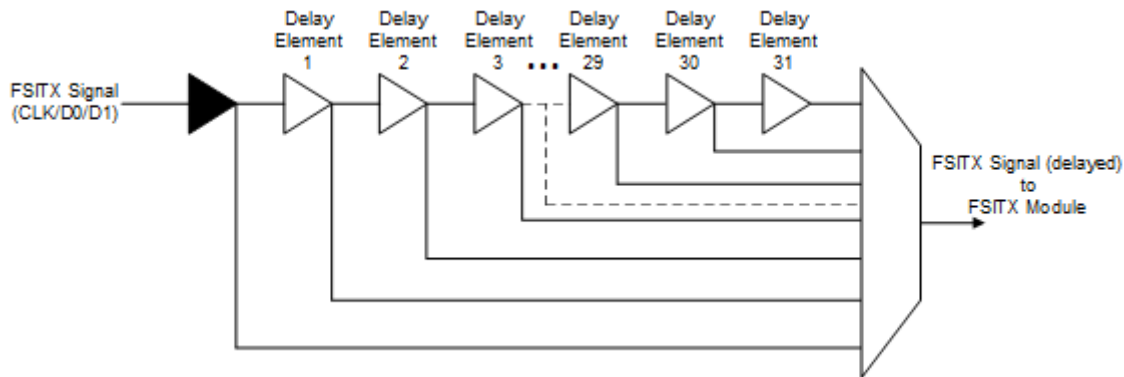
Figure 7-233. Delay Line Control Circuit
