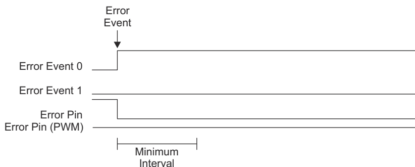
Figure 13-292. ESM Error Pin Assertion
