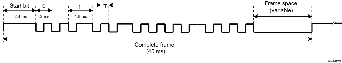
Figure 13-75. UART SIRC Bit Transmission Example
