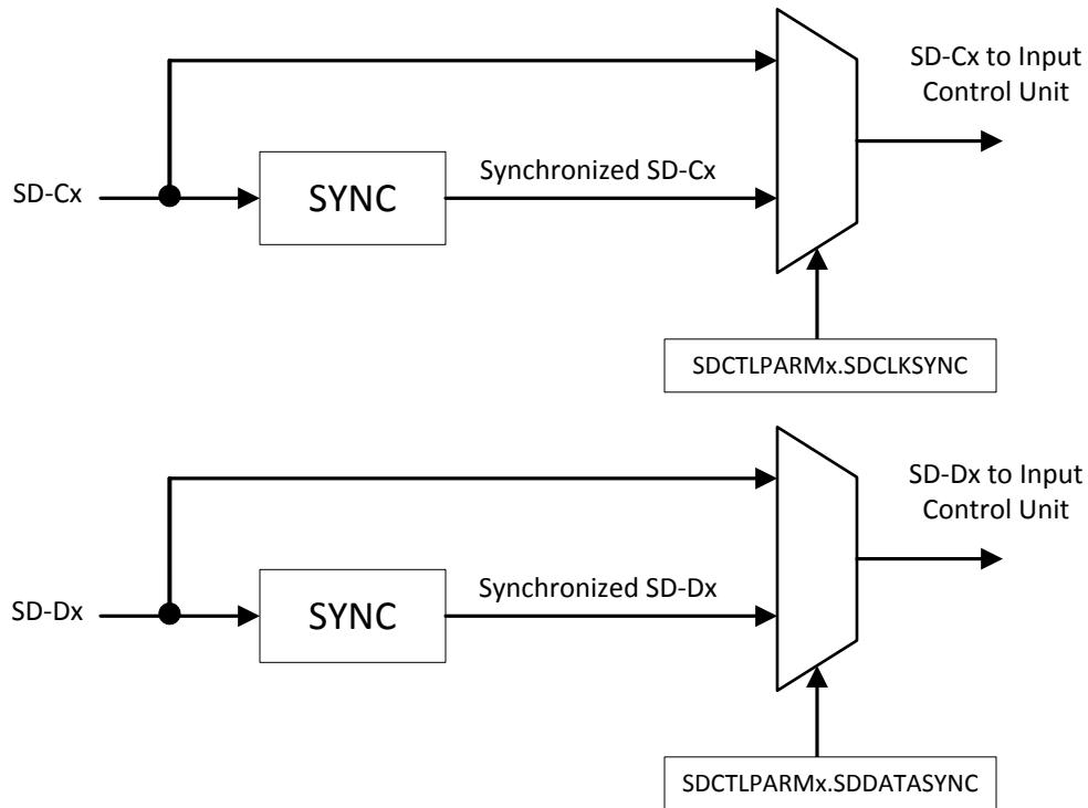
Figure 7-249. Input Qualification on SD-Cx and SD-Dx
