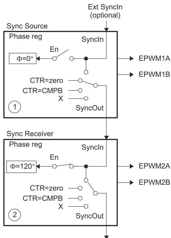
Figure 7-167. Configuring Two PWM Modules for Phase Control
