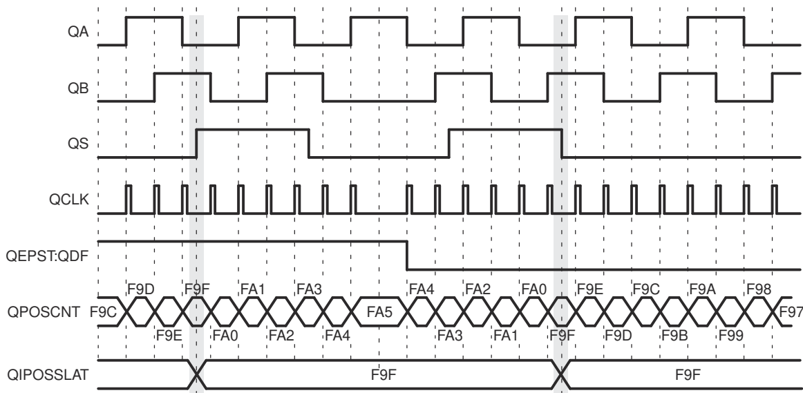
Figure 7-221. Strobe Event Latch (QEPCTL[SEL] = 1)
