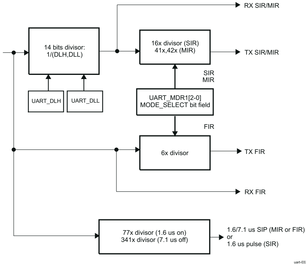
Figure 13-90. IrDA Baud Rate Generator
