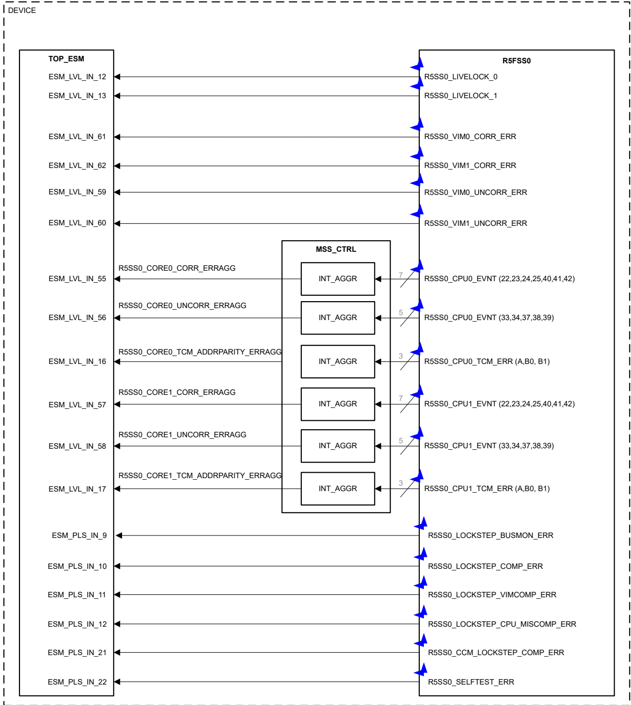
Figure 7-2. R5FSS0 Integration Diagram Continued
