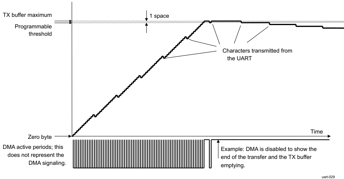
Figure 13-84. UART Transmit FIFO DMA Request Generation (1 Space)
