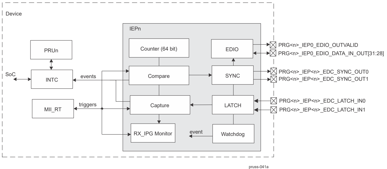
Figure 7-79. IEP Functional Block Diagram
