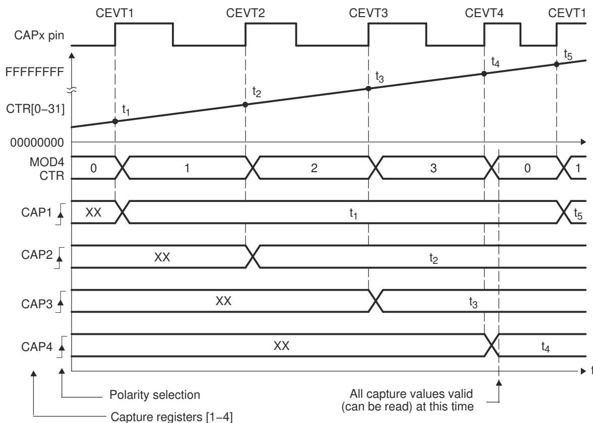
Figure 7-204. Capture Sequence for Absolute Time-stamp and Rising Edge Detect
