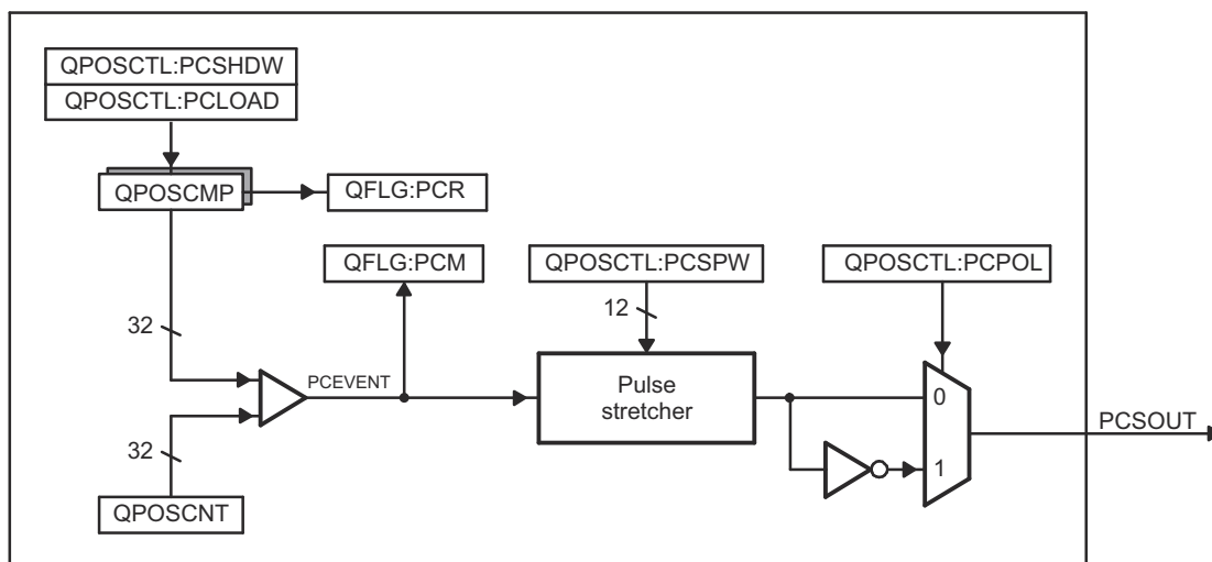
Figure 7-222. eQEP Position-compare Unit
