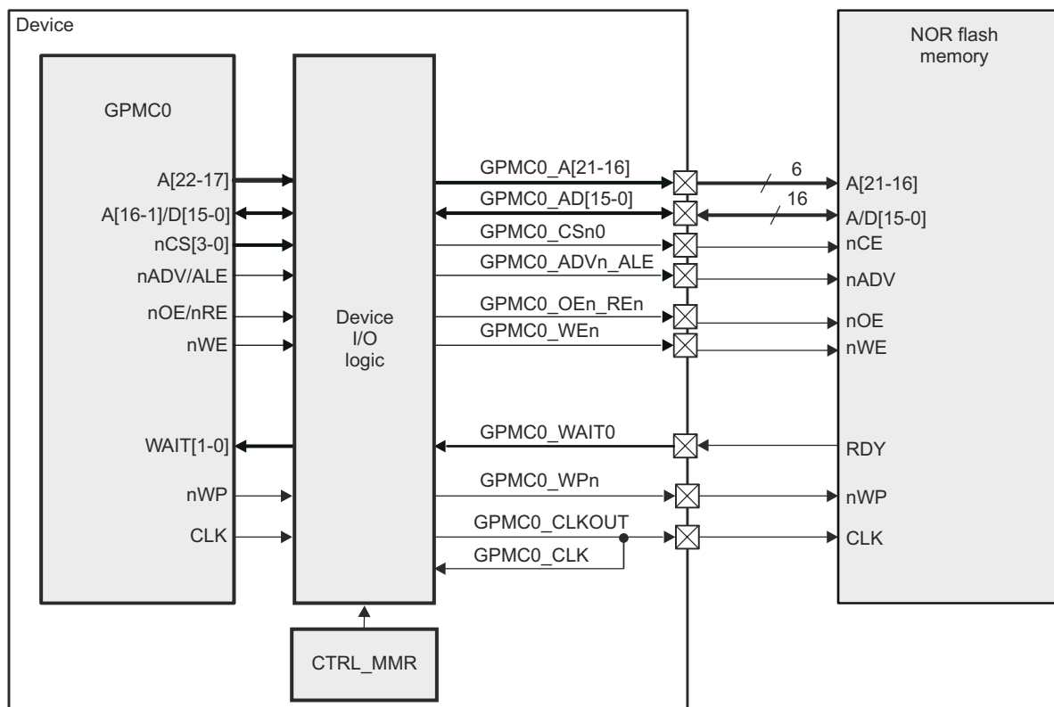
Figure 13-168. GPMC Connection to an External NOR Flash Memory
