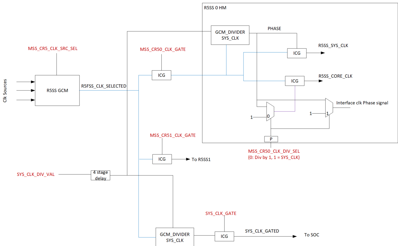
Figure 6-23. R5SS/SYSCLK Clocking
