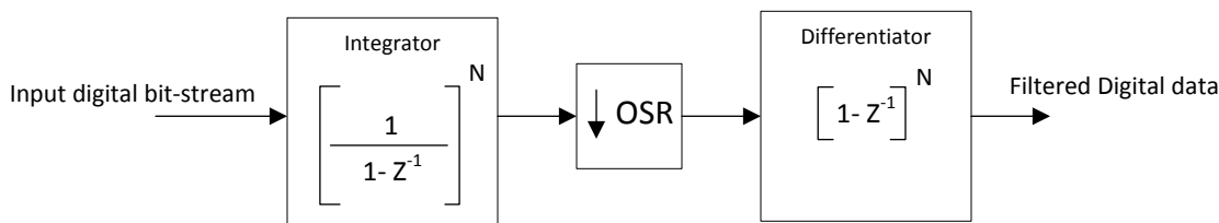
Figure 7-252. Simplified Sinc Filter Architecture
