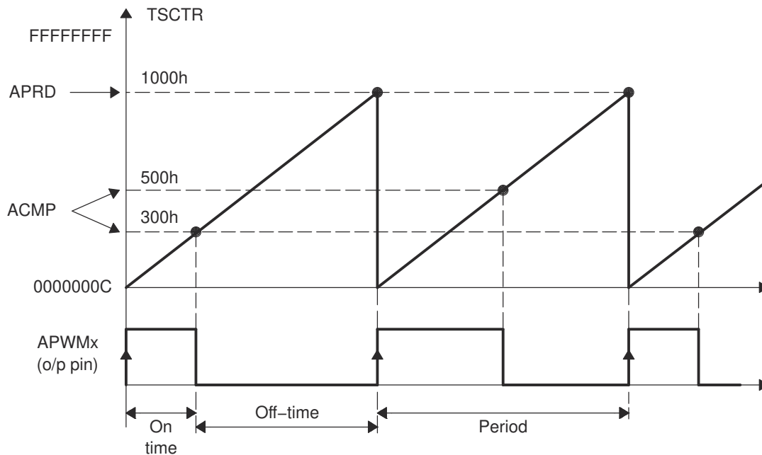
Figure 7-208. PWM Waveform Details of APWM Mode Operation
