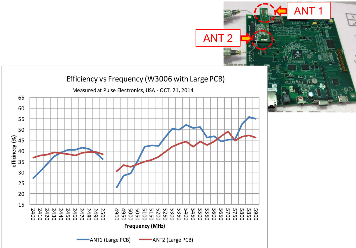
Figure 5-2. Antenna Efficiency
