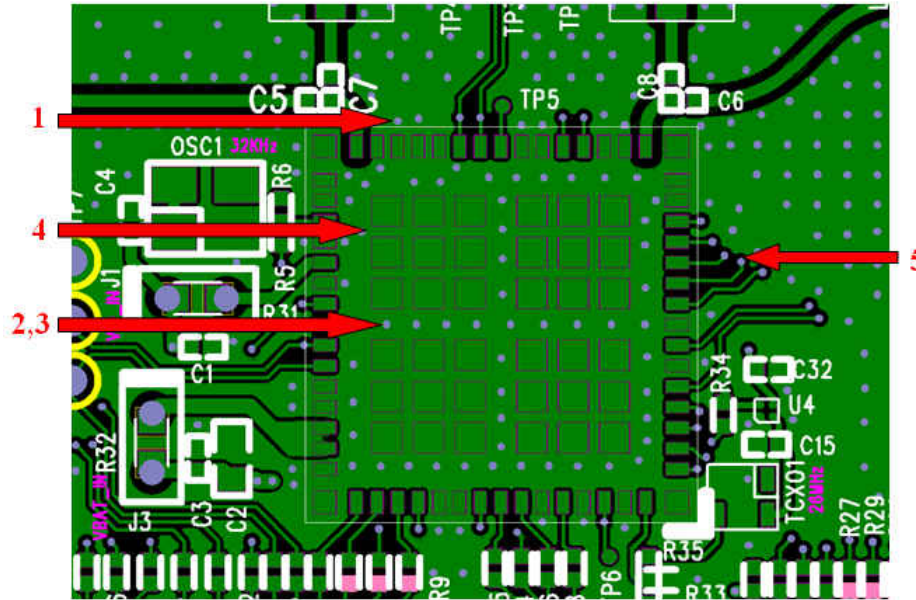
Figure 7-5. Module Layout Guidelines (Top Layer)
