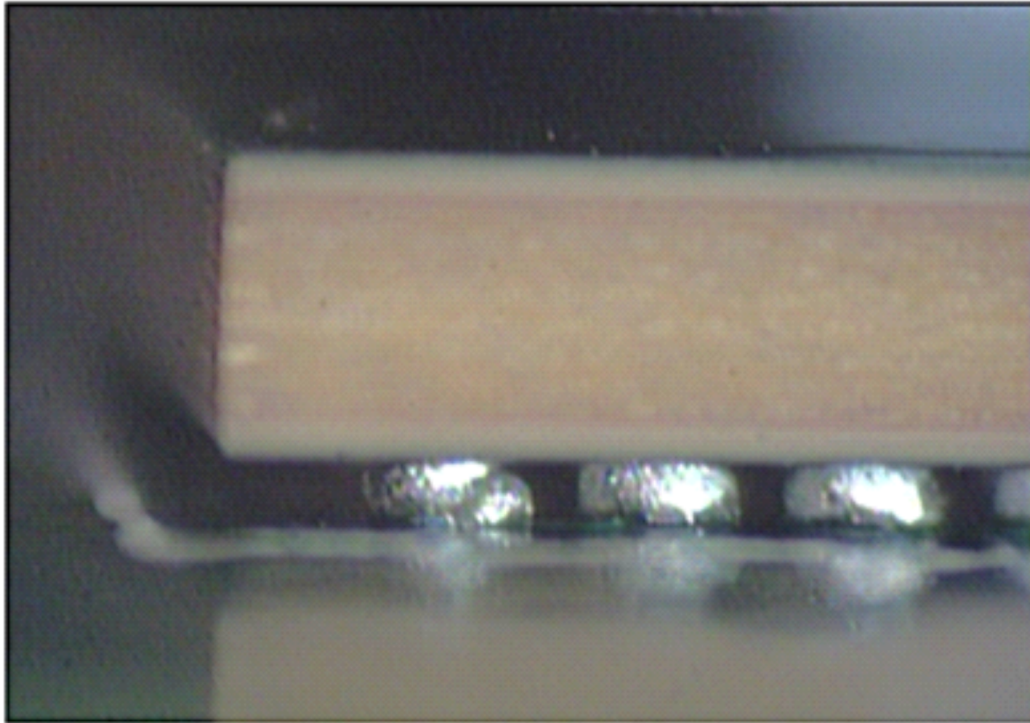
Figure 6. Example of Soldering Defect (Head-In-Pillow) on Perimeter Verified Visually
