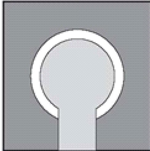
Figure 1. NSMD Pads – Top View
