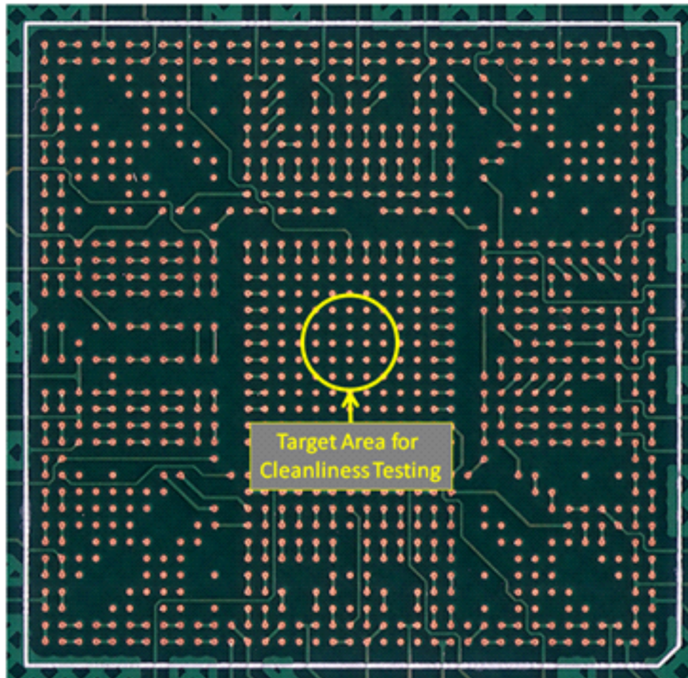
Figure 5. Example of Key Area to Test for Complete Flux Residue Removal
