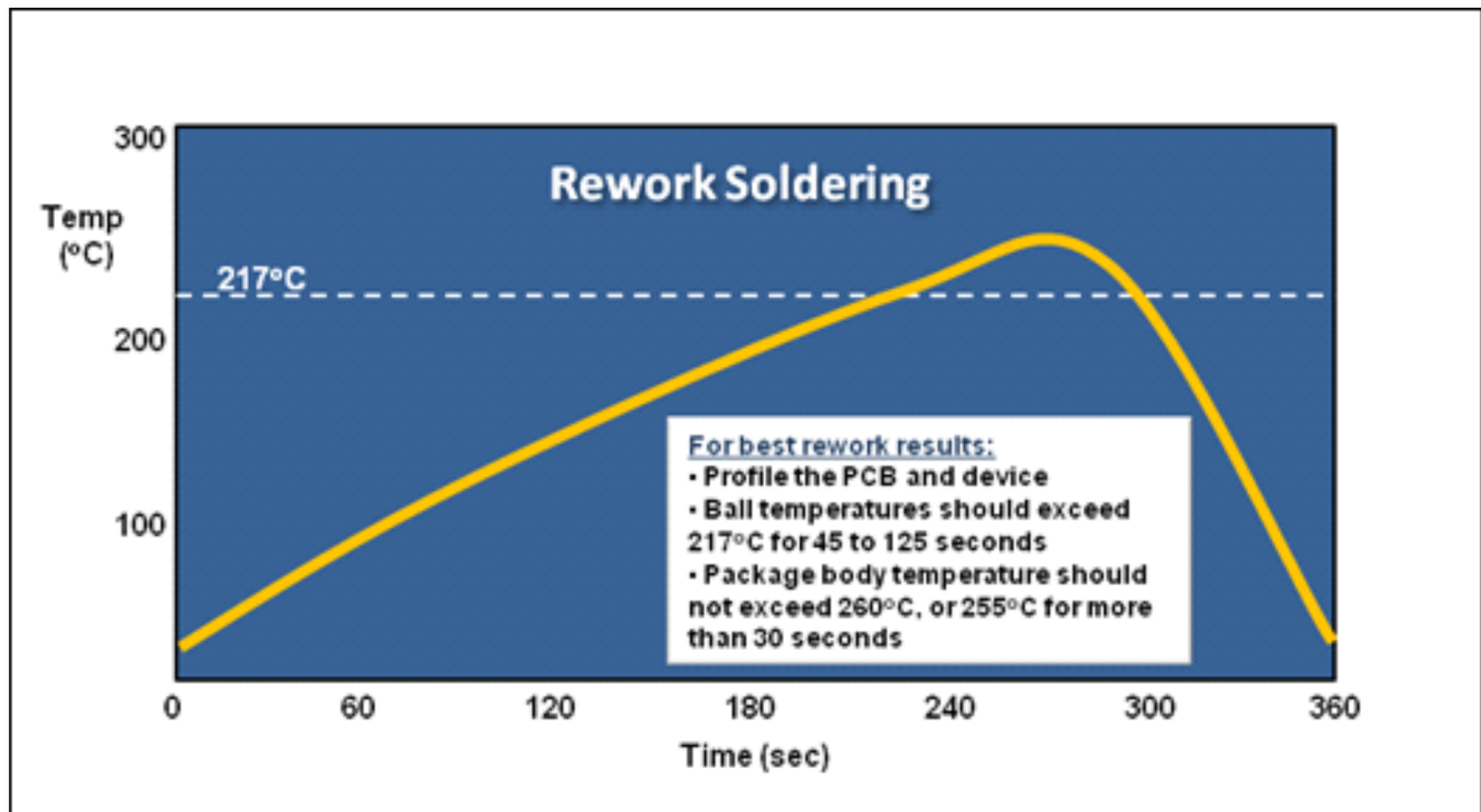
Figure 8. Rework Profile Considerations
