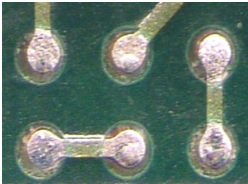
Figure 11. Example of Cleaned PCB Pads Ready to Accept Fresh Solder Paste
