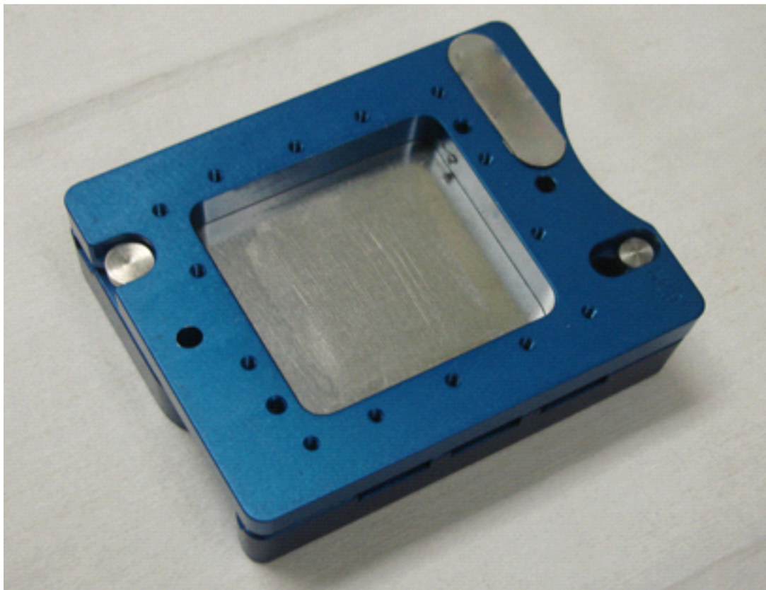
Figure 12. Example of Fixture for Printing Paste on BGA Balls
