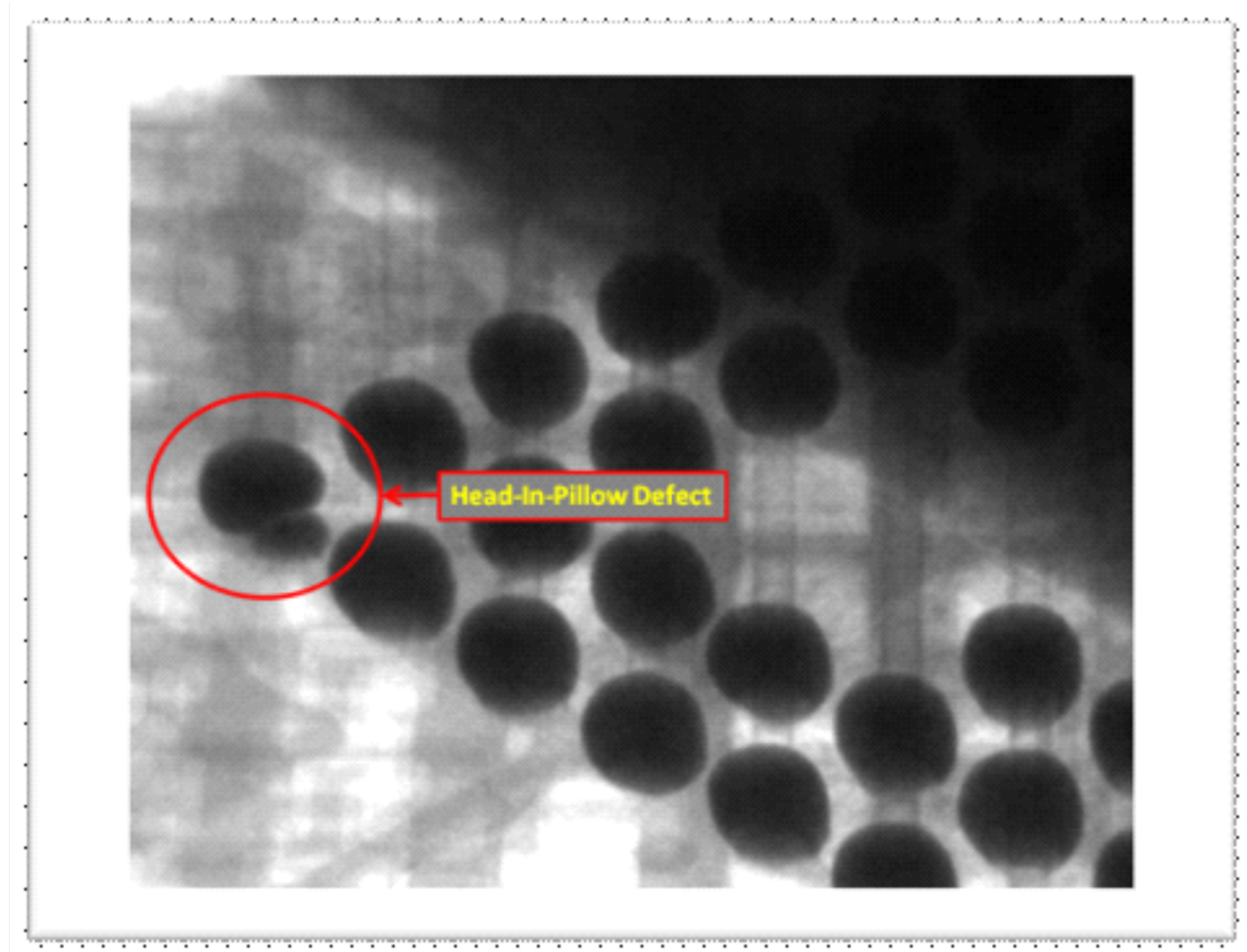
Figure 7. Example of Defect Verified with 2-D X-Ray
