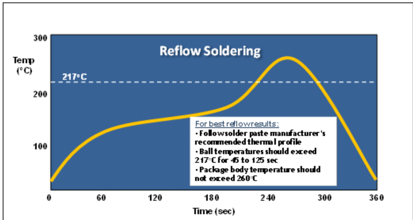
Figure 4. Sample Reflow Profile
