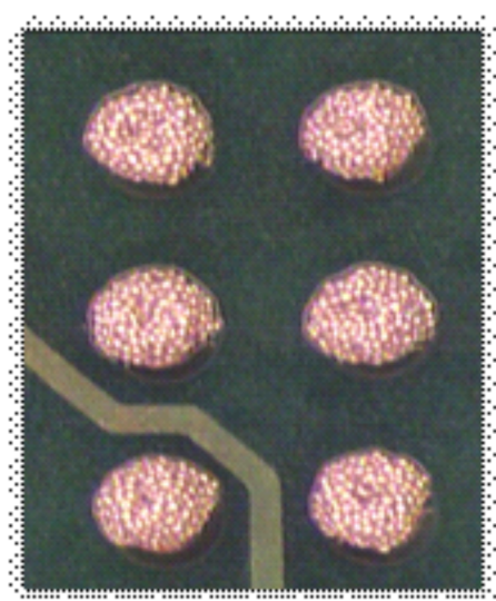
Figure 3. Preferred Solder Paste Alignment
