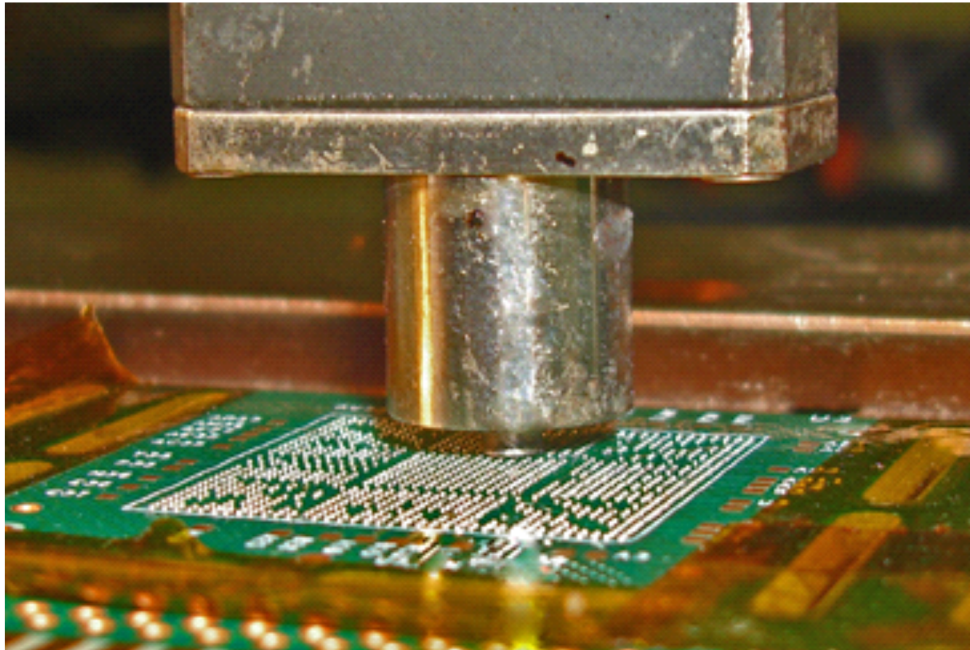
Figure 10. Example of Automated Vacuum Removal of Excess Solder from Pads
