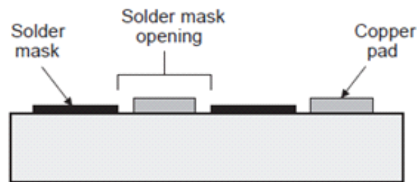
Figure 2. NSMD – Cross-Sectional View
