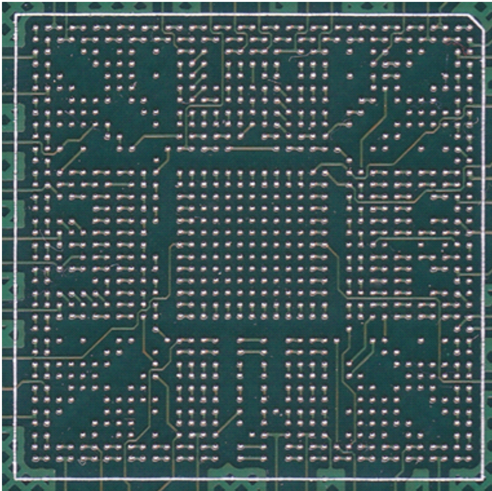
Figure 9. Example of PCB Inspection after Device Removal
