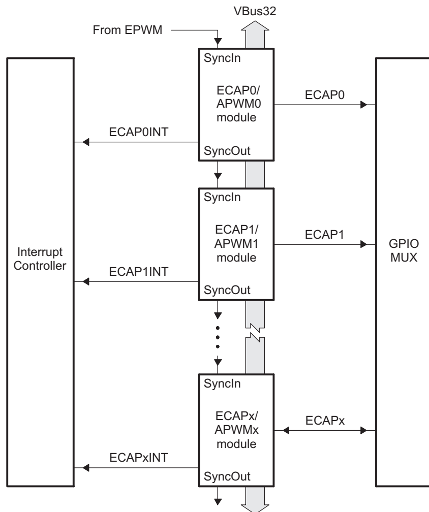
Figure 20-101. Multiple eCAP Modules
