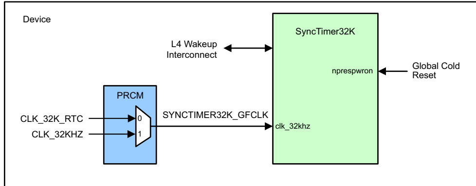
Figure 19-58. SyncTimer32K Integration
