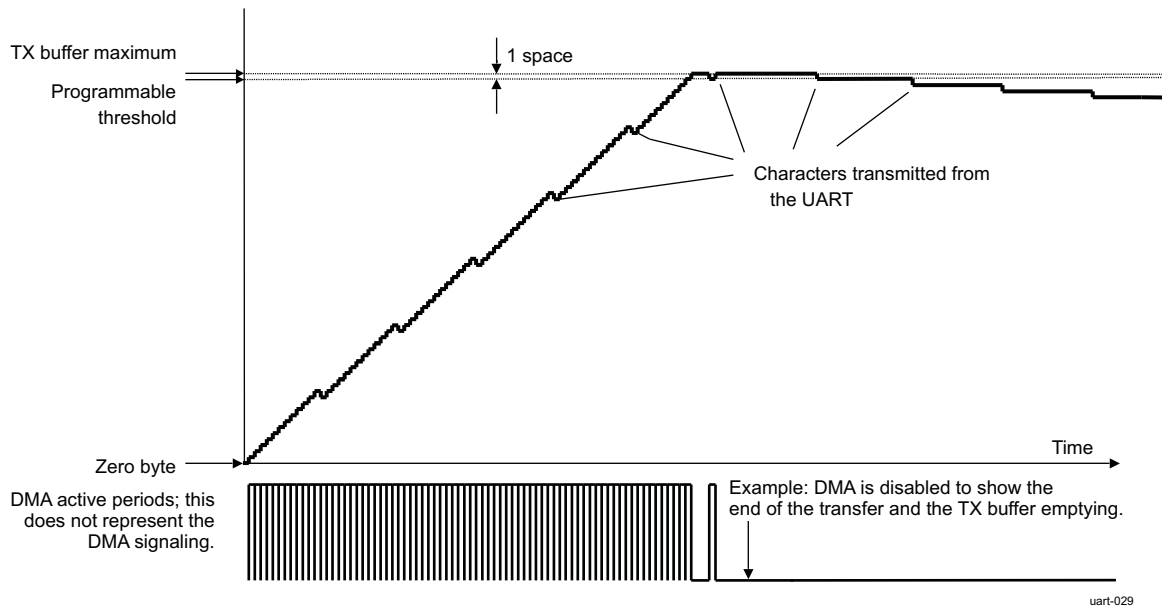
Figure 21-10. Transmit FIFO DMA Request Generation (1 Space)
