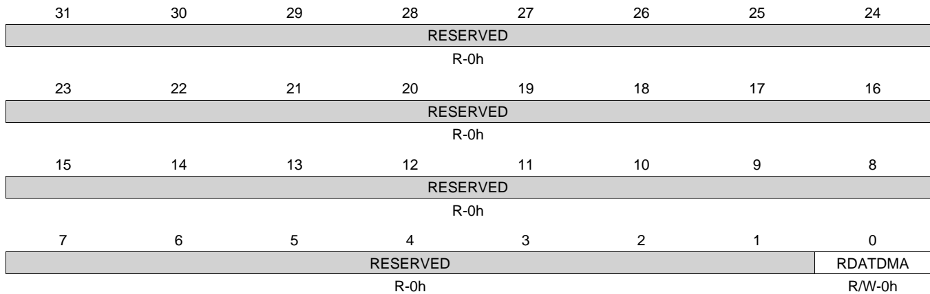
Figure 24-61. MCASP_REVTCTL Register
