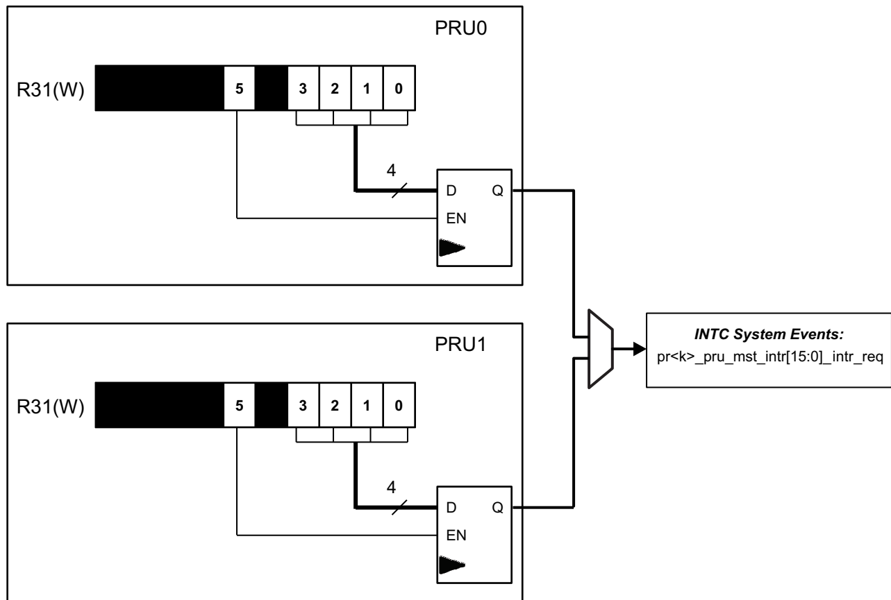
Figure 30-5. Event Interface Mapping (R31)
