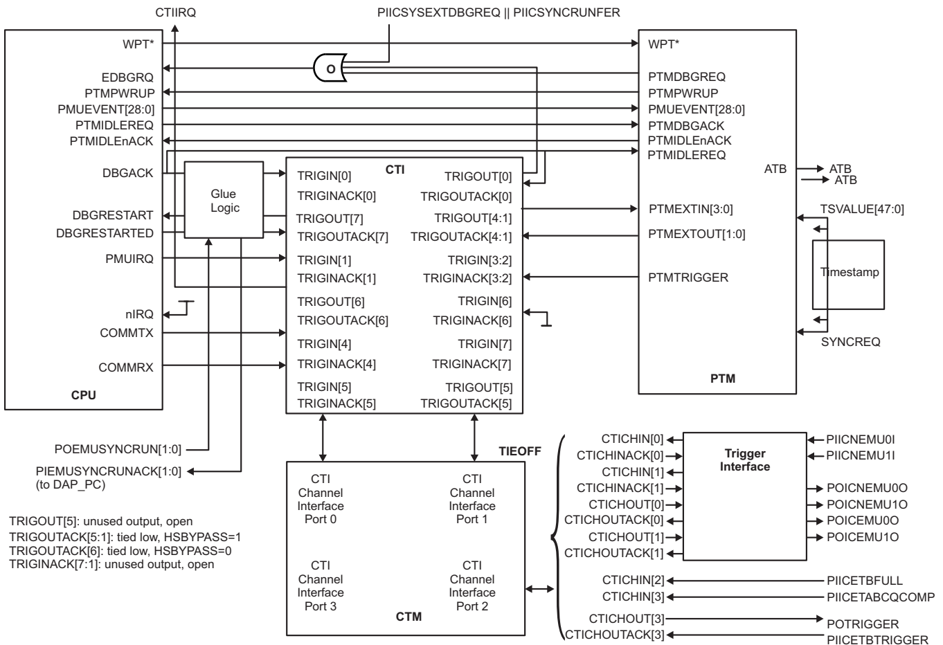
Figure 31-2. MPU Subsystem Cross Trigger Connections
