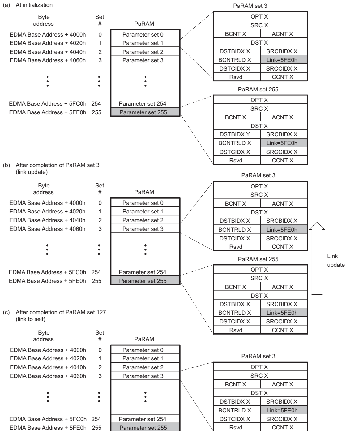
Figure 10-12. Link-to-Self Transfer
