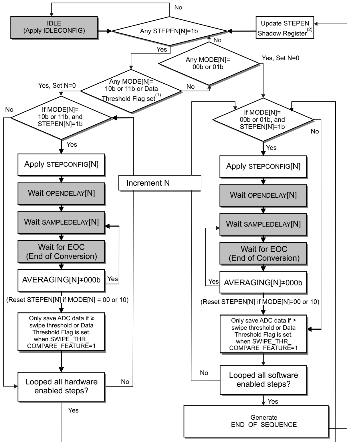
Figure 12-2. FSM Sequencer
