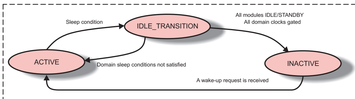
Figure 6-3. Clock Domain State Transitions
