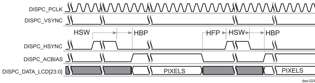
Figure 13-28. Active Matrix Timing Diagram of Configuration 3 (Between Frames)
