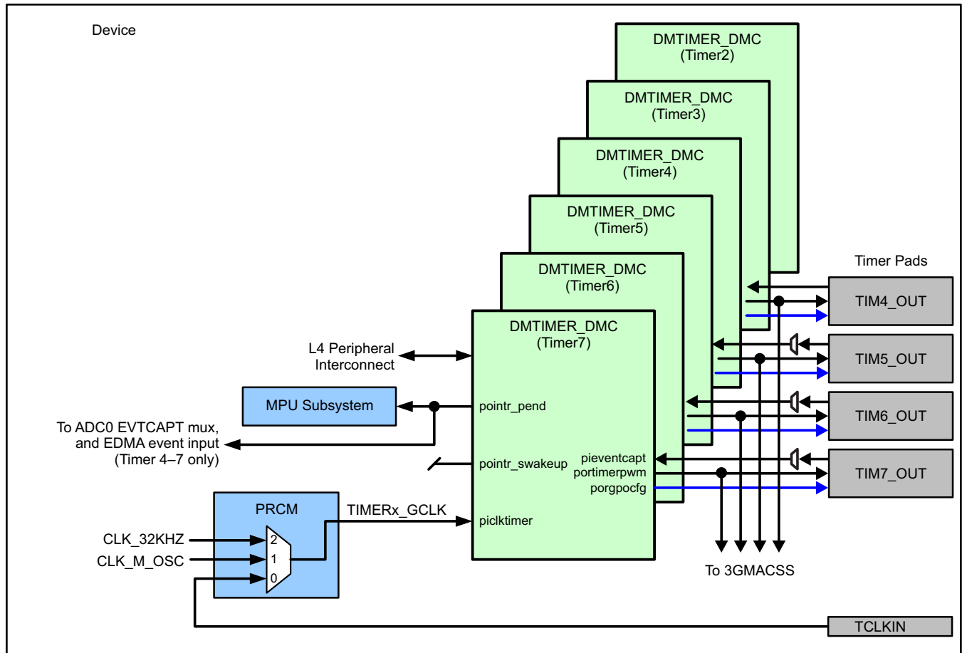
Figure 19-3. Timer2-7 Integration
