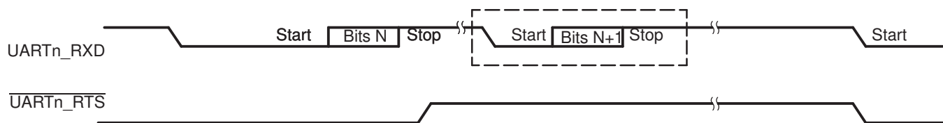
Figure 30-36. Autoflow Functional Timing Waveforms for \overline{\text{UARTn\_RTS}}
