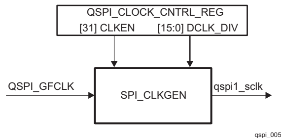
Figure 27-3. SPI_CLKGEN Block
