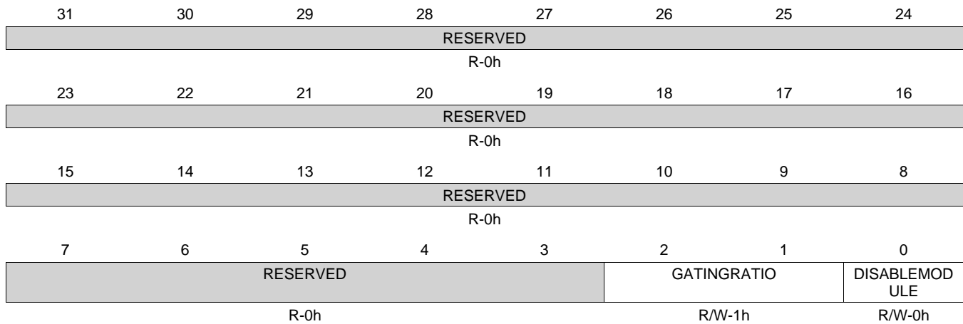
Figure 28-22. GPIO_CTRL Register
