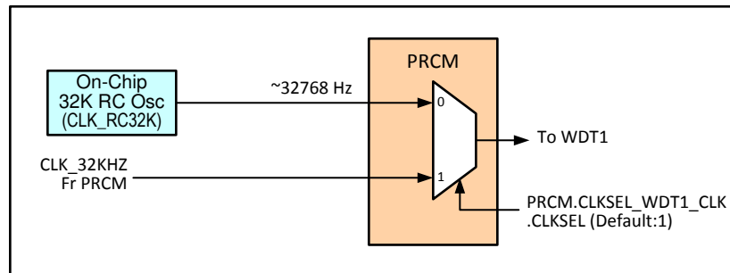
Figure 6-21. Watchdog Timer Clock Selection
