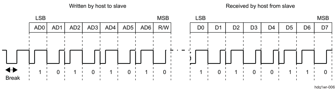
Figure 23-6. HDQ/1-Wire Communication Sequence
