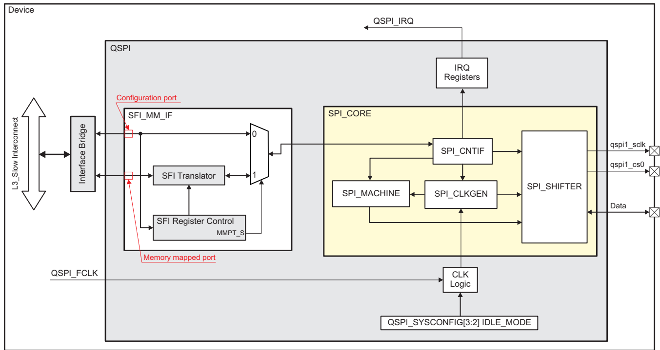
Figure 27-2. QSPI Block Diagram
