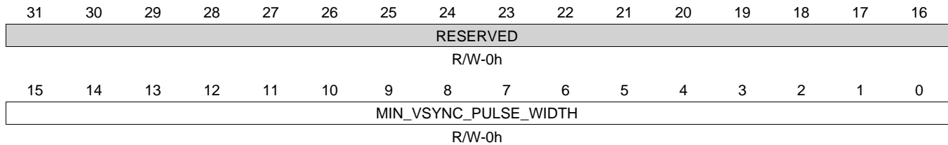
Figure 13-173. RFBI_VSYNC_WIDTH Register
