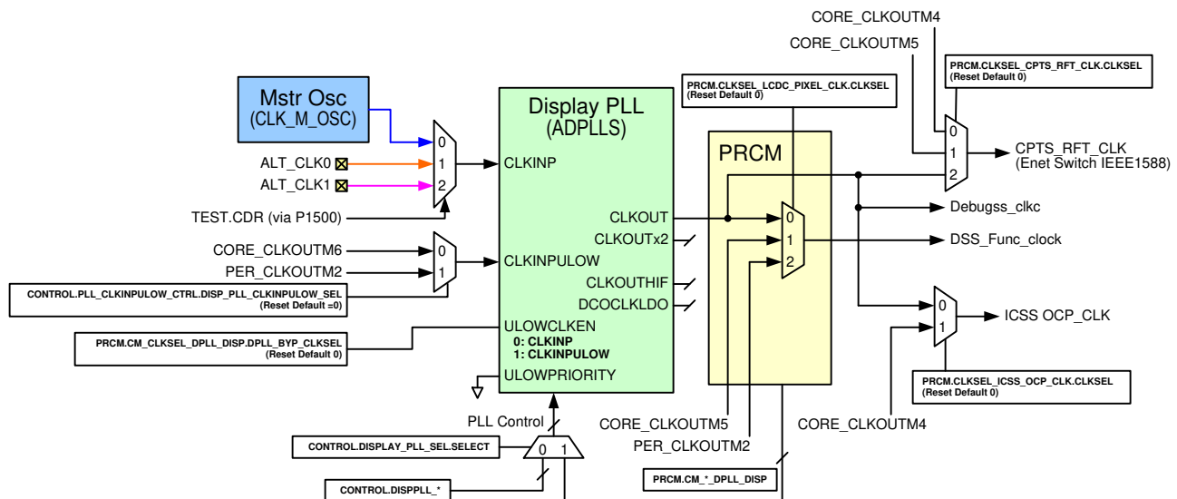
Figure 6-17. Display PLL Structure
