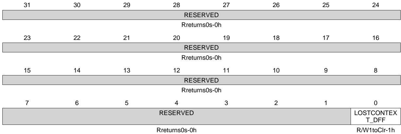
Figure 6-111. PRCM_RM_PER_TIMER8_CONTEXT Register
