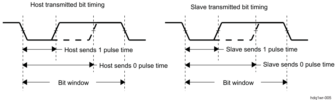
Figure 23-5. HDQ/1-Wire Transmitted Bit Timing
