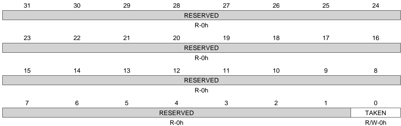
Figure 18-79. SPINLOCK_REG_31 Register
