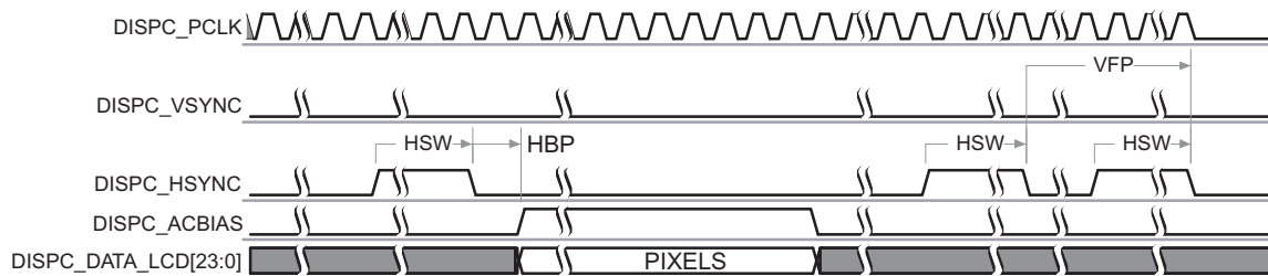
Figure 13-21. Active Matrix Timing Diagram of Configuration 1 (End of Frame)
