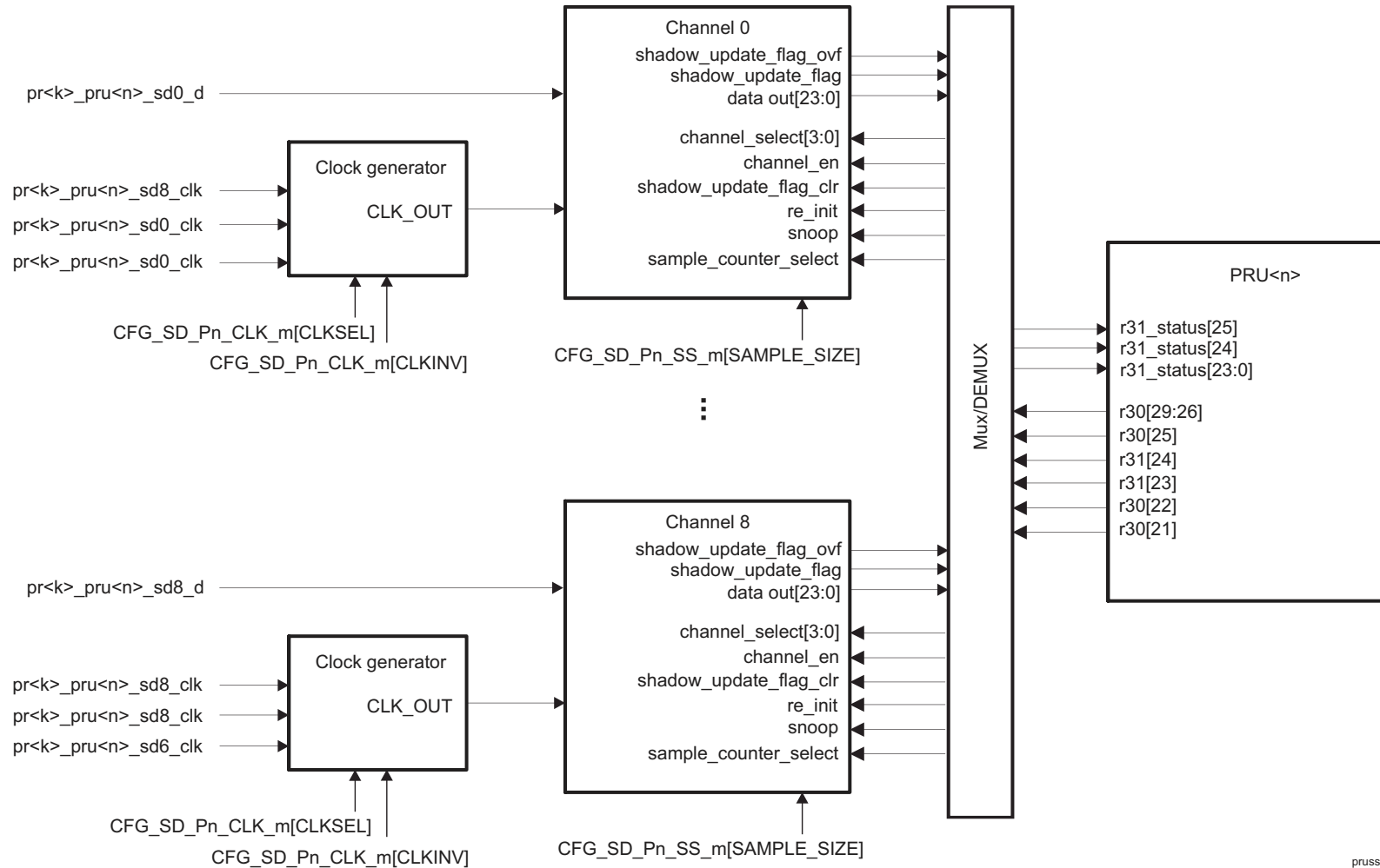
Figure 30-11. Sigma Delta Block Diagram
