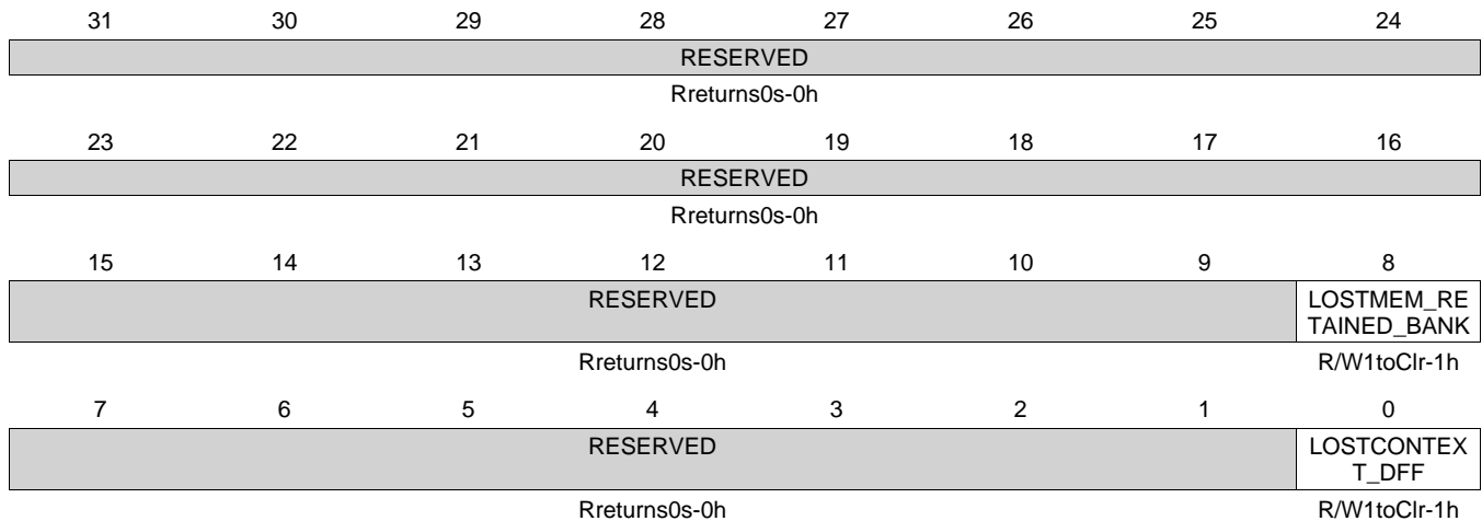
Figure 6-119. PRCM_RM_PER_UART5_CONTEXT Register
