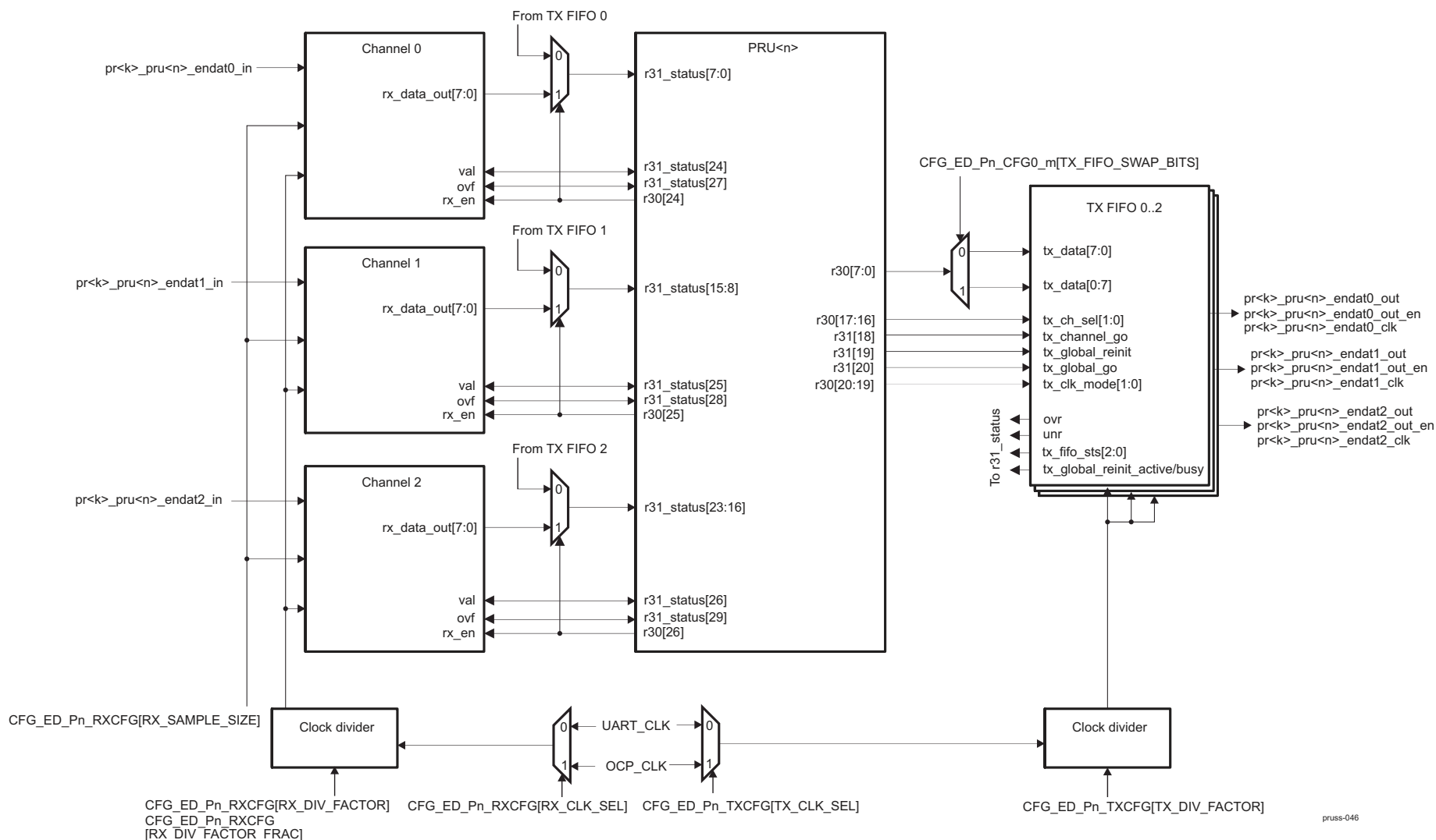
Figure 30-14. Peripheral I/F Block Diagram
