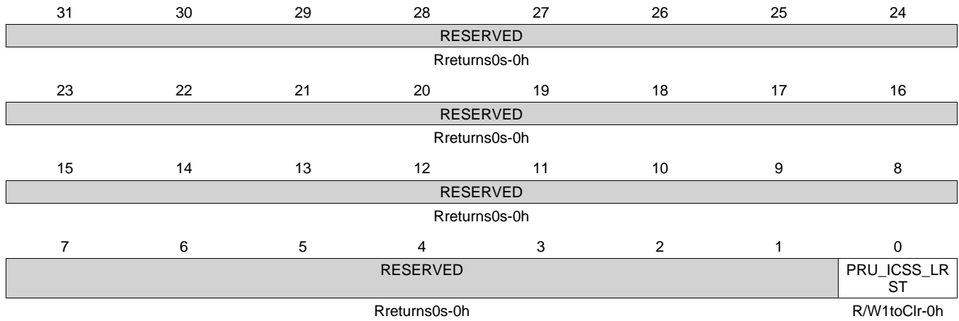
Figure 6-57. PRCM_RM_PER_RSTST Register
