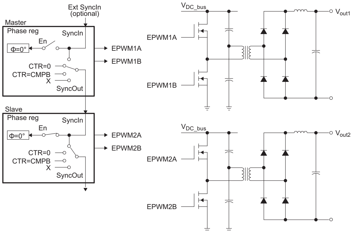
Figure 20-61. Control of Two Half-H Bridge Stages ( F_{P\text{WM}2} = N \times F_{P\text{WM}1} )
