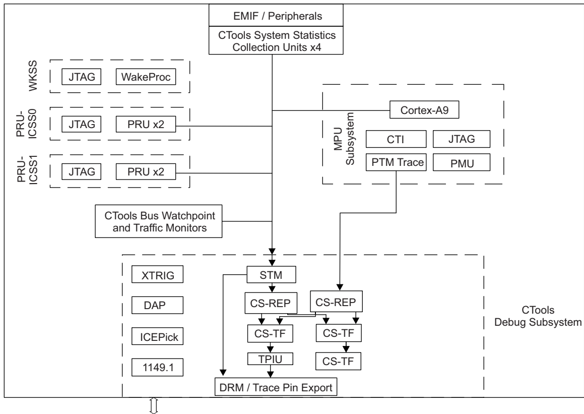
Figure 31-1. Functional Block Diagram Debug View
