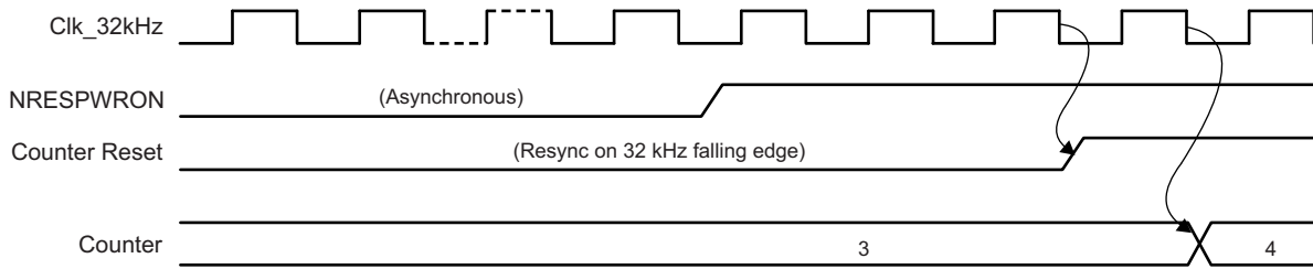
Figure 19-59. Reset Resynchronization Timing
