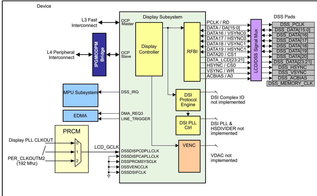
Figure 13-1. DSS Integration
