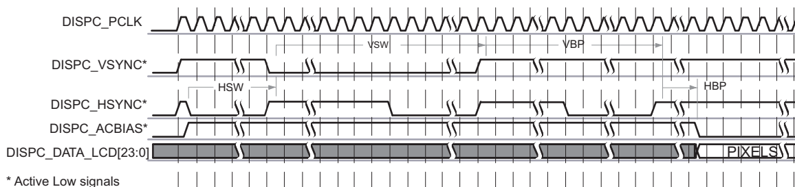
Figure 13-22. Active Matrix Timing Diagram of Configuration 2 (Start of Frame)
