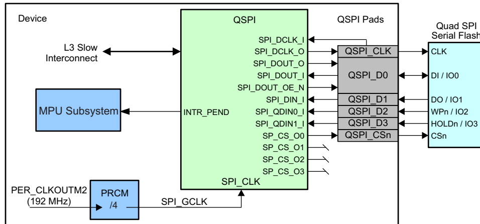
Figure 27-1. QSPI Integration
