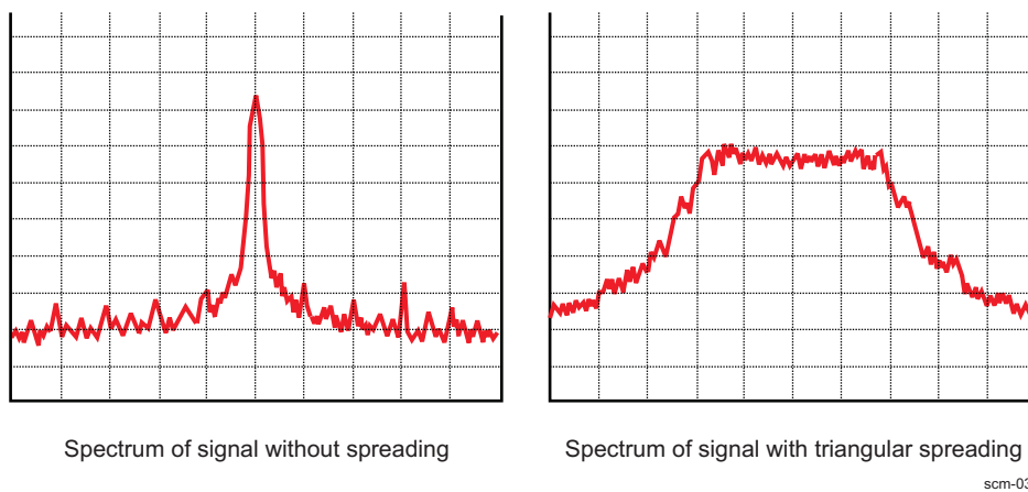
Figure 6-11. Effect of the SSC in Frequency
