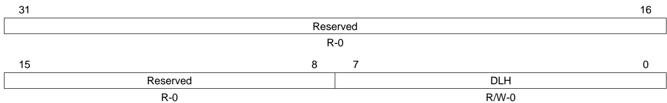
Figure 30-269. Divisor MSB Latch (DLH)
