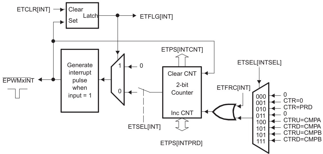
Figure 20-48. Event-Trigger Interrupt Generator
