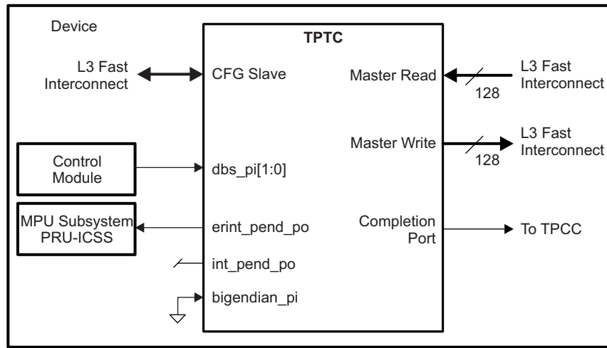
Figure 10-3. TPTC Integration
