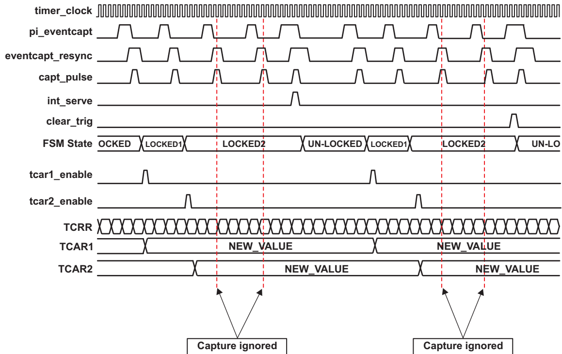
Figure 19-7. Capture Wave Example for CAPT_MODE = 1
