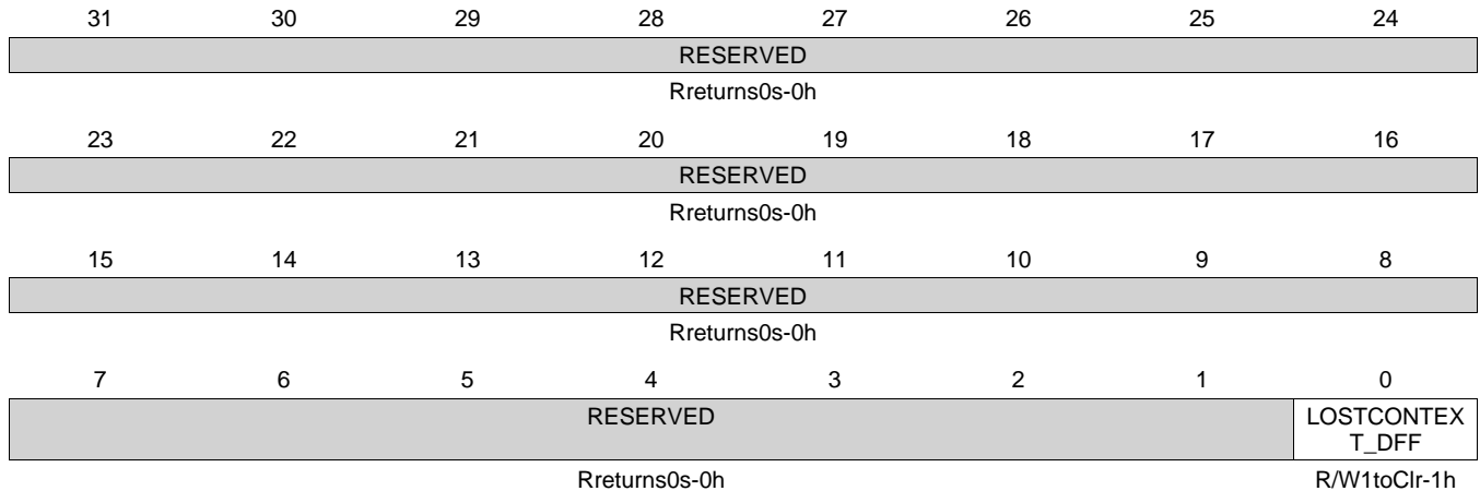
Figure 6-105. PRCM_RM_PER_TIMER2_CONTEXT Register
