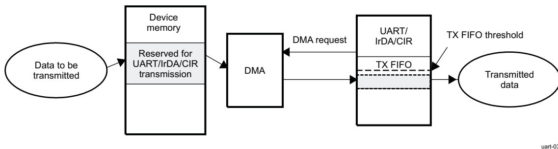
Figure 21-12. DMA Transmission
