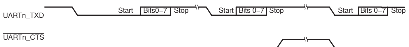
Figure 30-37. Autoflow Functional Timing Waveforms for \overline{\text{UARTn\_CTS}}
