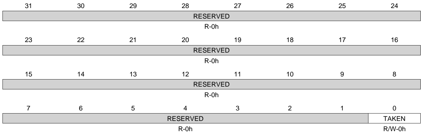
Figure 18-63. SPINLOCK_REG_15 Register
