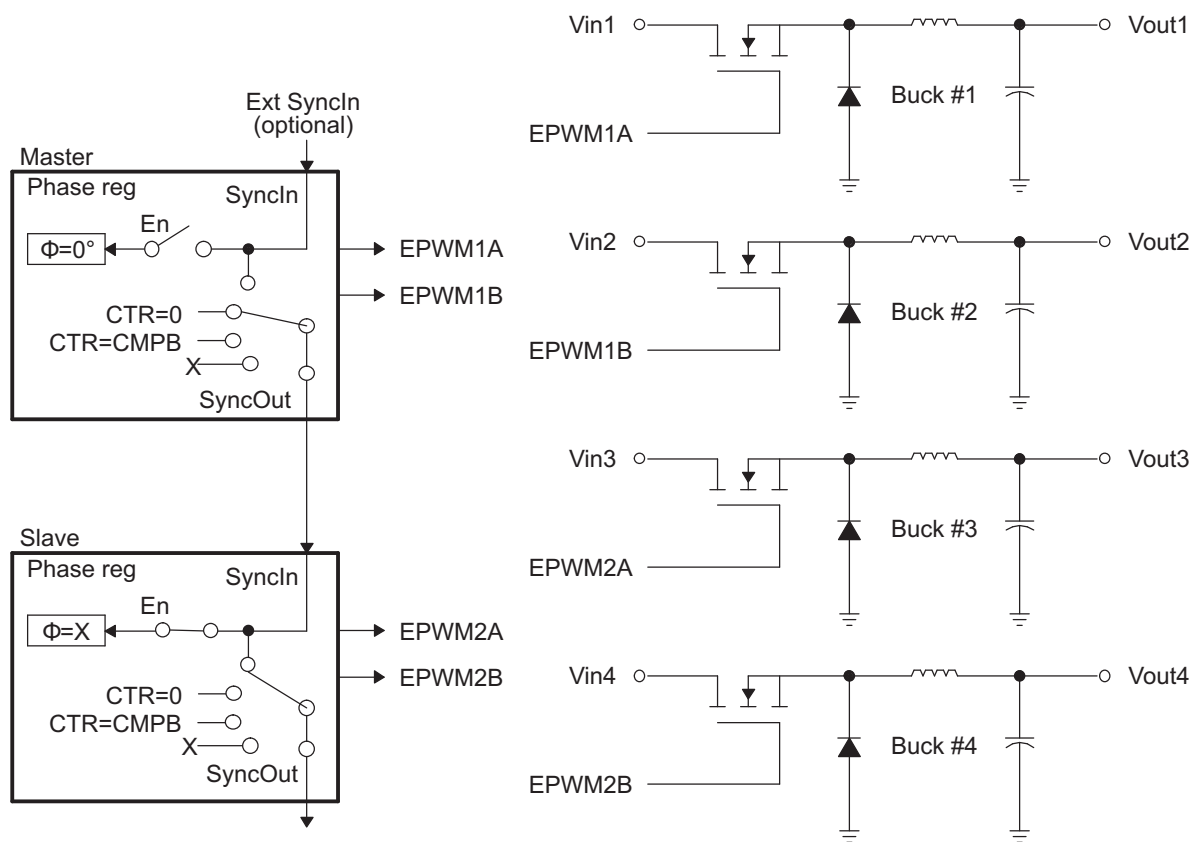
Figure 20-59. Control of Four Buck Stages. (Note: F_{PVM2} = N \times F_{PVM1} )
