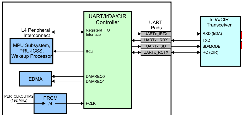
Figure 21-2. UART/IrDA Module — IrDA/CIR Application
