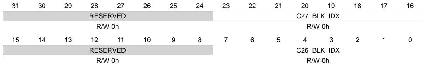
Figure 30-69. PRU_ICSS_CTRL_CTBR1 Register
