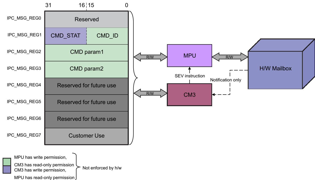
Figure 6-7. IPC Mechanism
