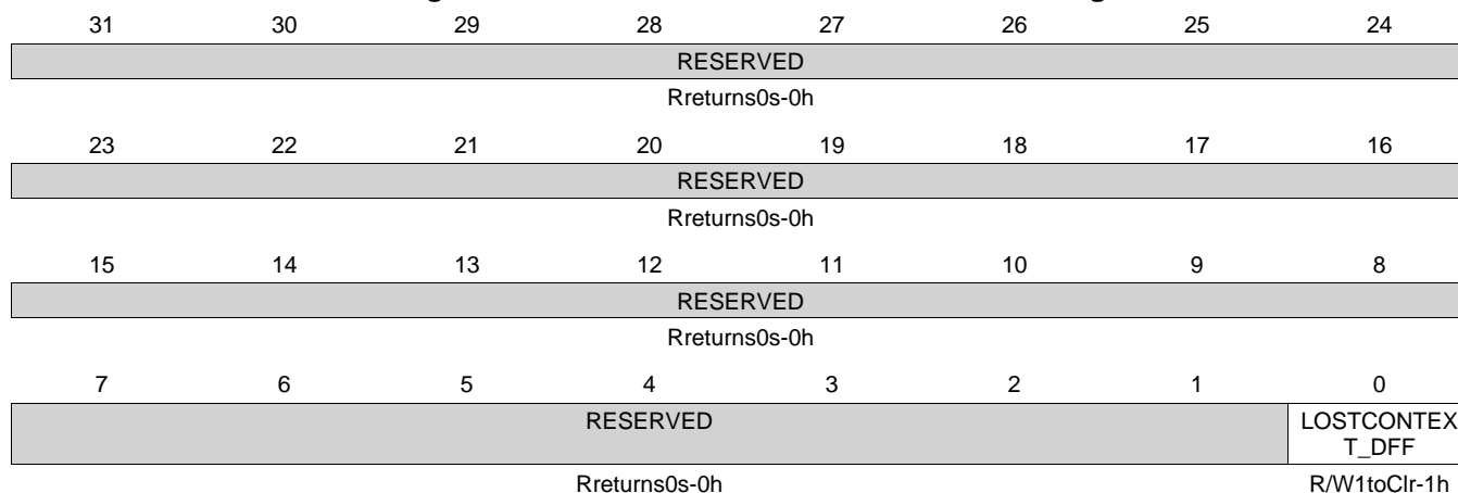
Figure 6-100. PRCM_RM_PER_SPI1_CONTEXT Register
