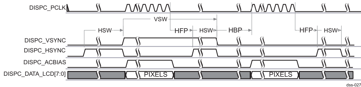
Figure 13-31. Passive Matrix Timing Diagram (Between Lines)
