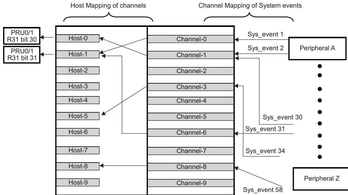
Figure 30-24. Interrupt Controller Block Diagram
