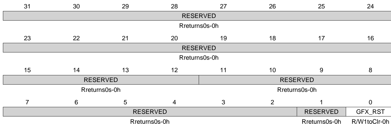
Figure 6-48. PRCM_PRM_RM_GFX_RSTST Register
