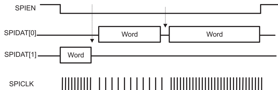
Figure 26-10. Continuous Transfers With SPIEN Maintained Active (Dual-Data-Pin Interface Mode)
