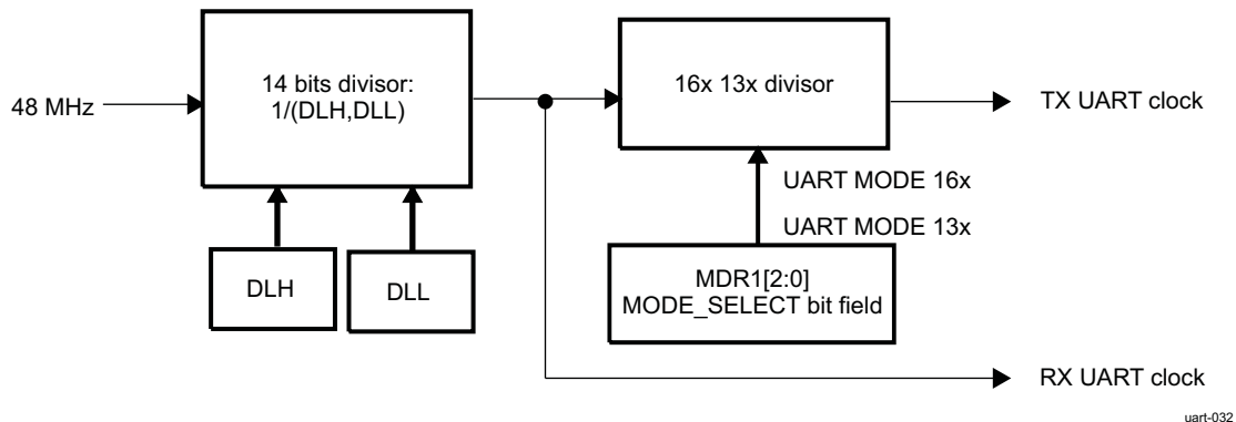
Figure 21-15. Baud Rate Generation
