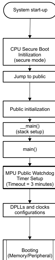
Figure 5-6. ROM Code Startup Sequence
