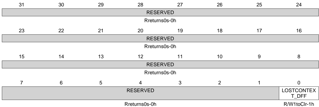
Figure 6-121. PRCM_RM_PER_USBPHYOCP2SCP1_CONTEXT Register
