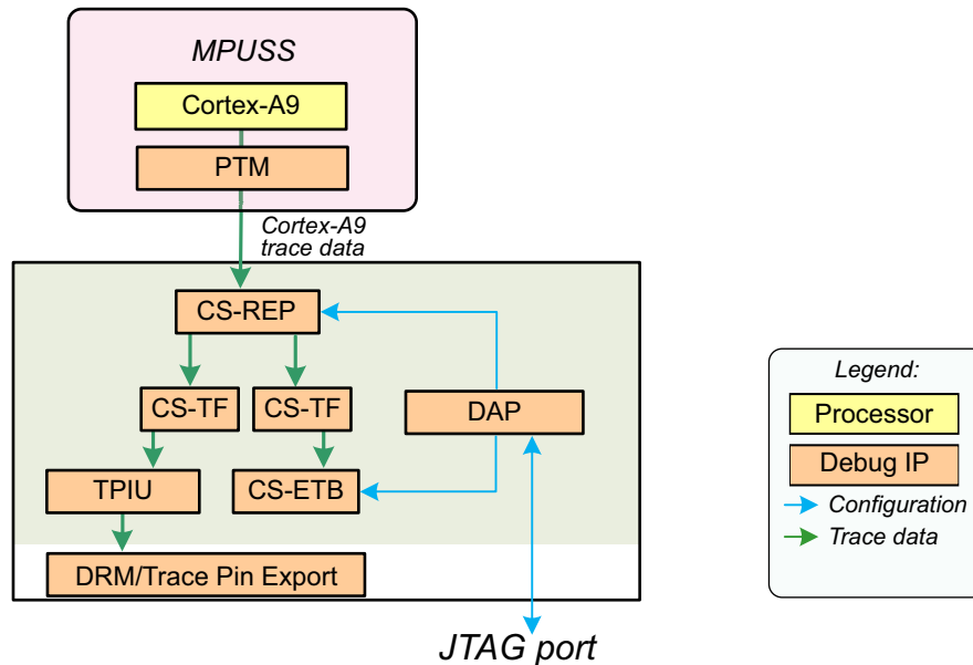
Figure 31-3. SoC Processor Trace Flow
