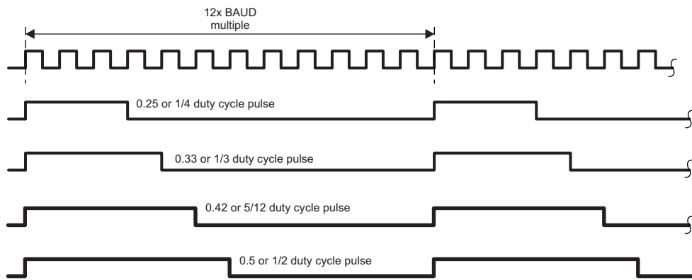
Figure 21-32. CIR Modulation Duty Cycle
