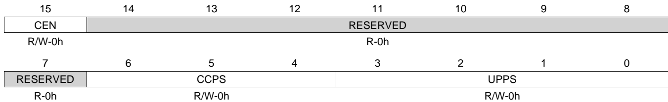
Figure 20-163. QCAPCTL Register
