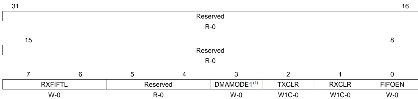
Figure 30-262. FIFO Control Register (FCR)
