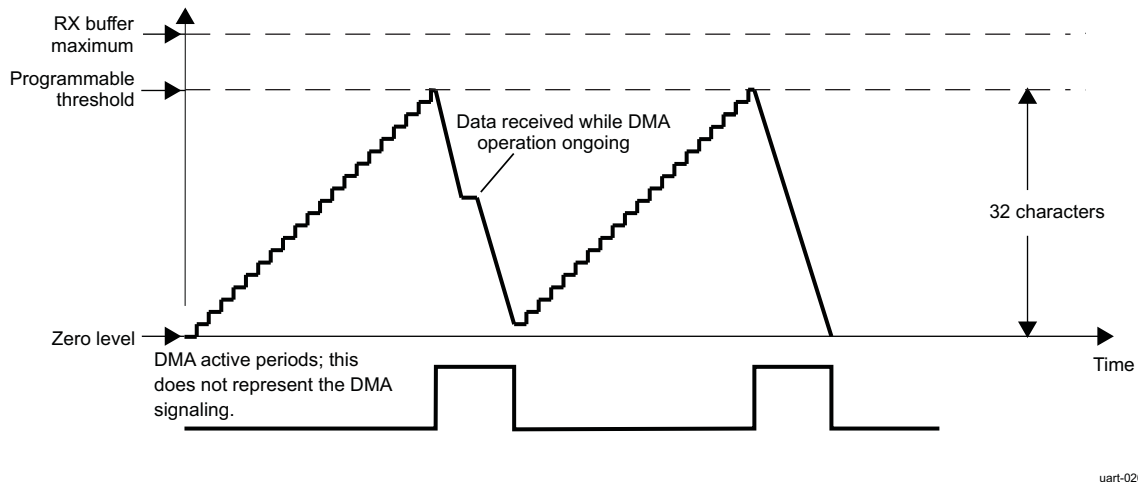
Figure 21-7. Receive FIFO DMA Request Generation (32 Characters)
