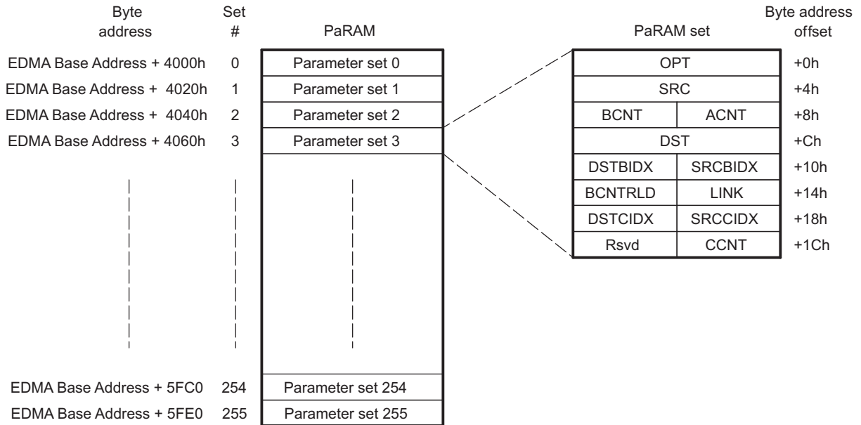
Figure 10-9. PaRAM Set
