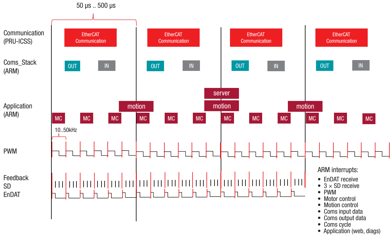
Figure 10: Connected industrial drive control cycle
