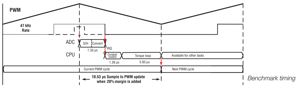
Figure 11: Single-chip drive motor control configuration and benchmark timing on AM437x processors
