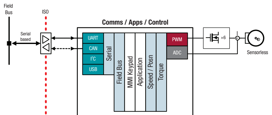
Figure 2: Inverter
