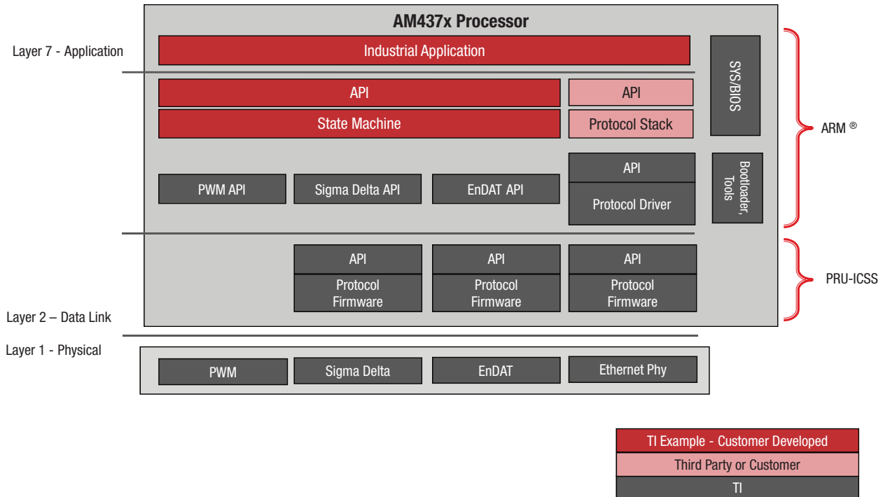
Figure 9: Industrial drive software
