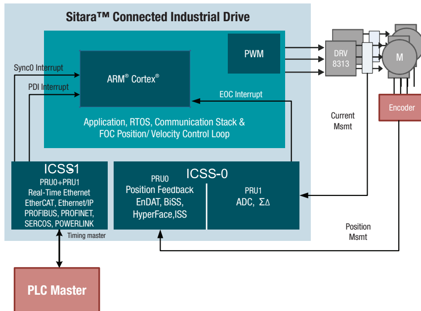
Figure 7: Connected industrial drive processor
