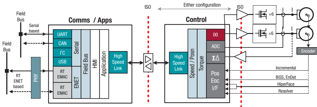
Figure 4: Multi-axis drive with real-time Ethernet
