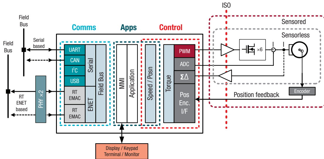
Figure 1: Industrial drive architecture overview
