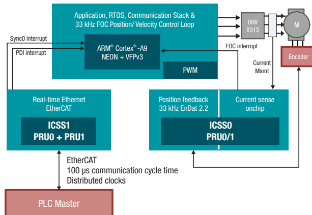
Motor control benchmark configuration
