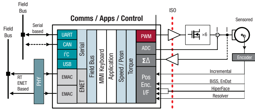
Figure 3: Servo drive with real-time Ethernet
