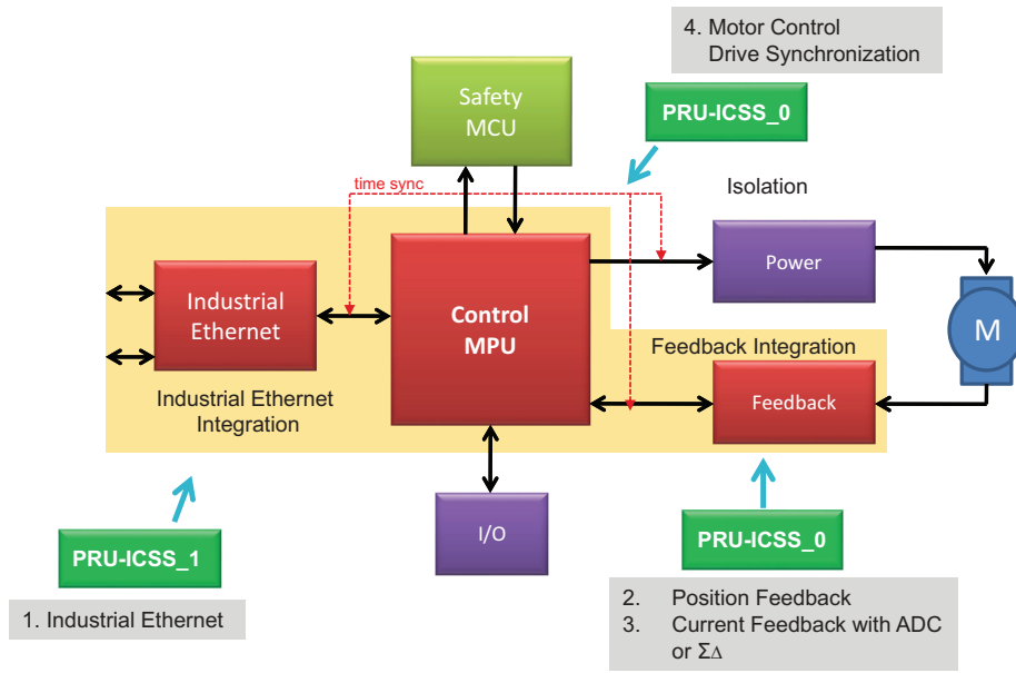
Figure 6: Integrated connected industrial drive building blocks
