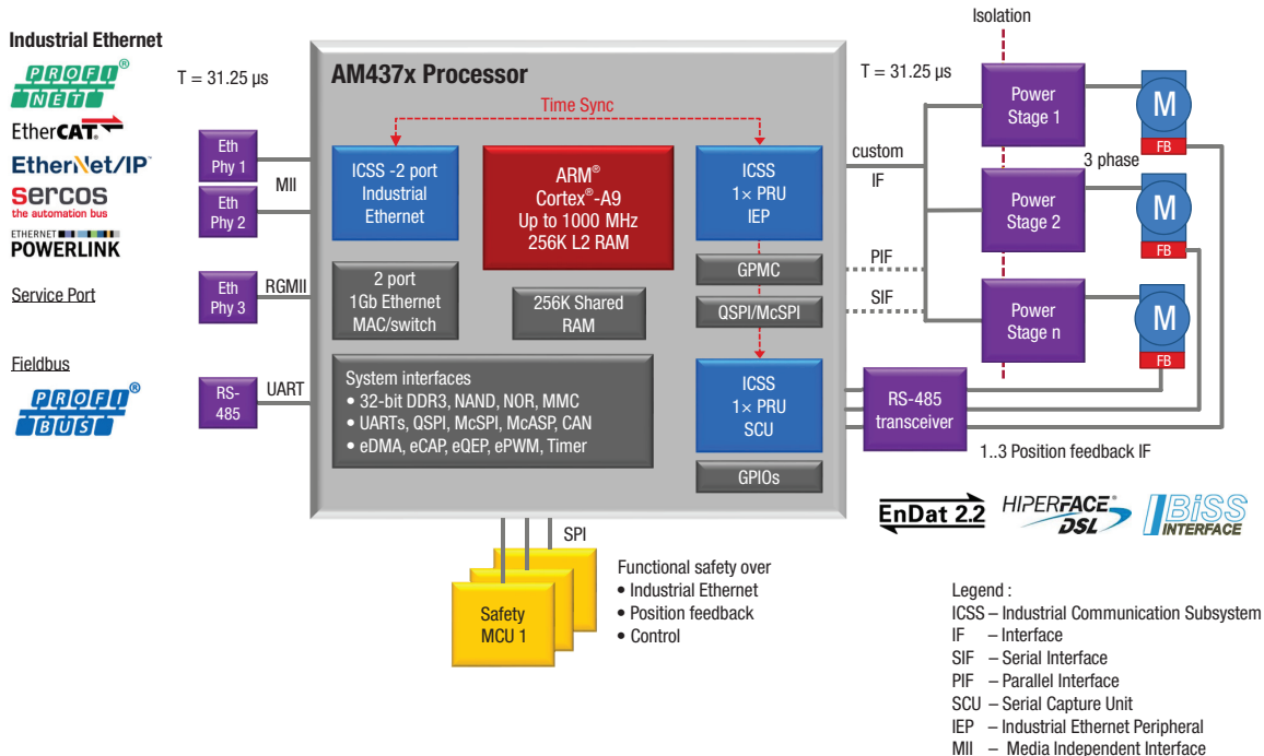
Figure 8: Sitara AM437x processor could also function as a multi-axis drive controller
