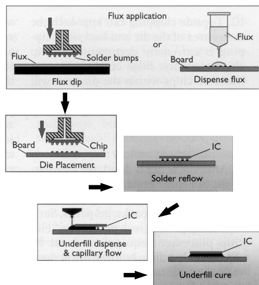
Figure 1. Summary of Flip-chip Assembly Process
