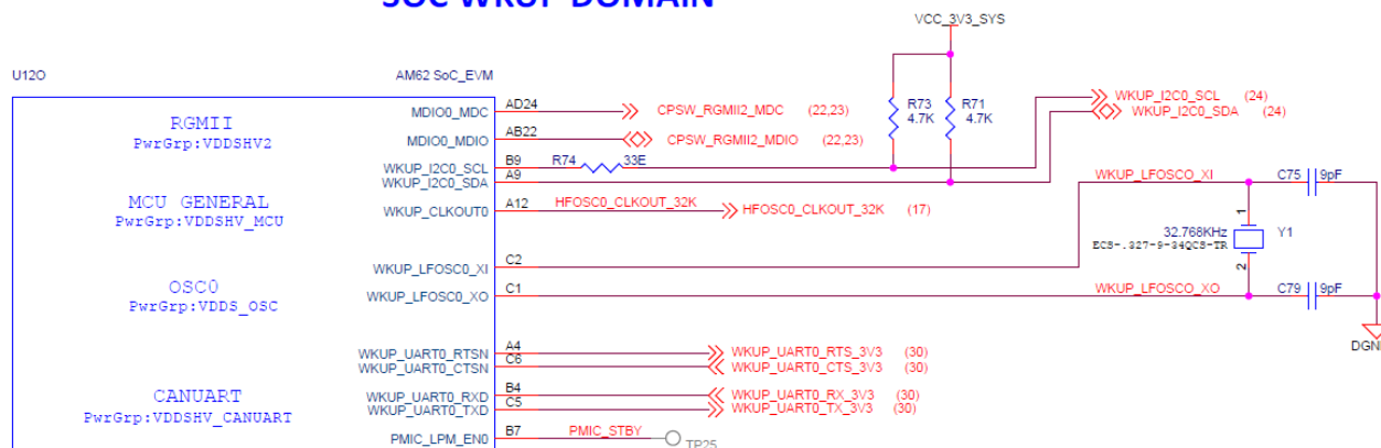
Figure 2-6. SoC WKUP Domain
