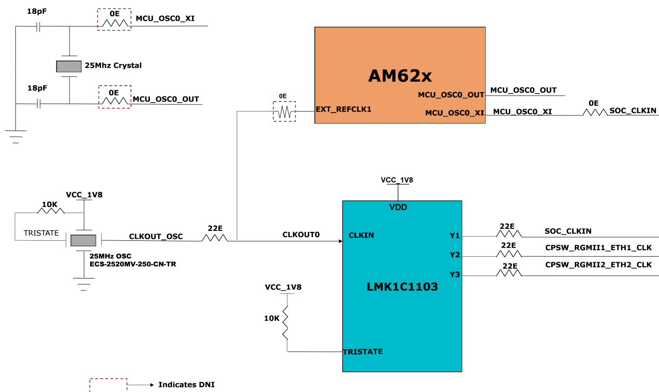
Figure 2-5. Clock Architecture of AM62x SKEVM
