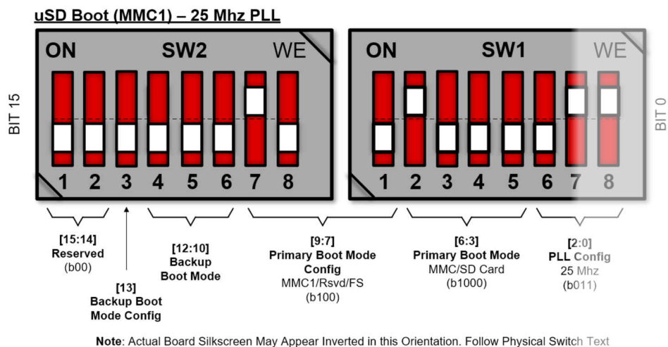
Figure 2-4. SD Bootmode Switch Setting Example
