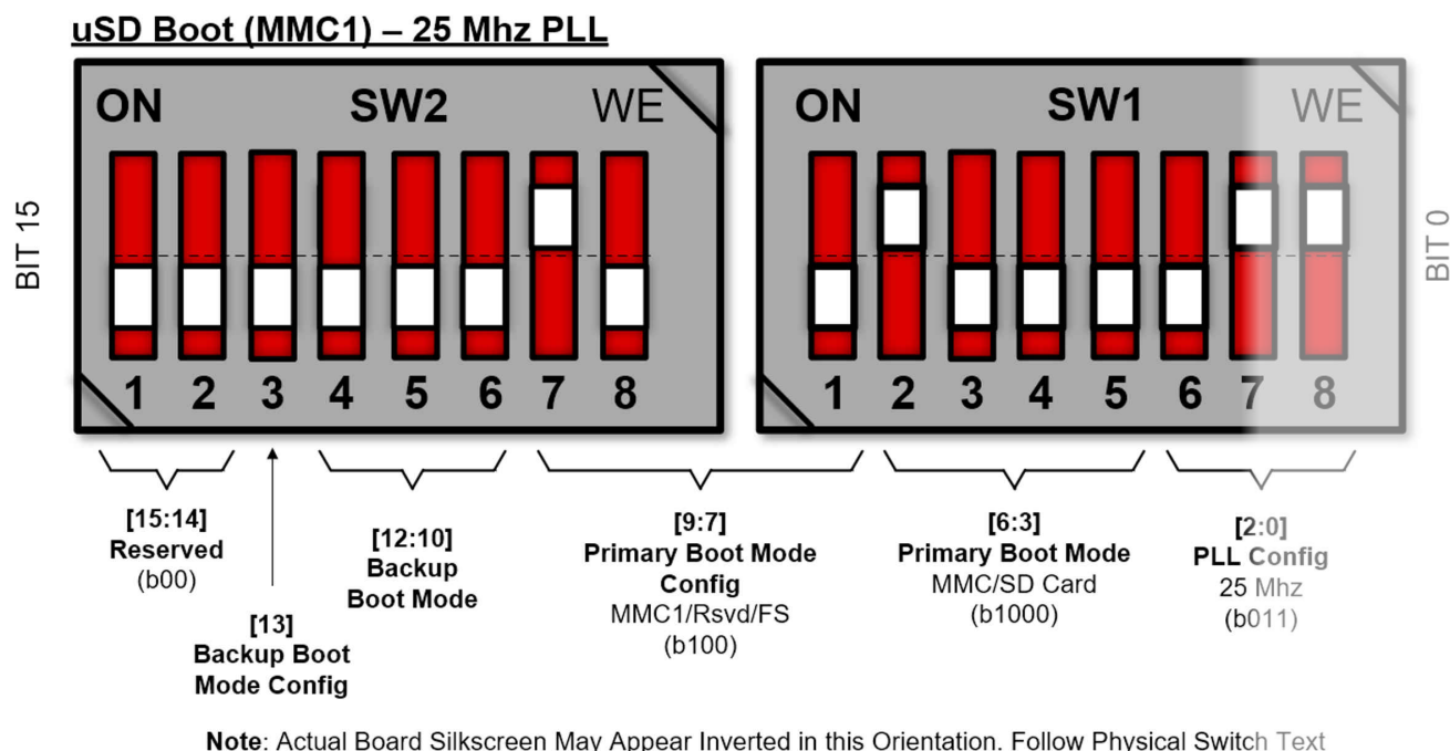
Figure 2-7. Bootmode Switch Configuration for SD Boot (E1)
