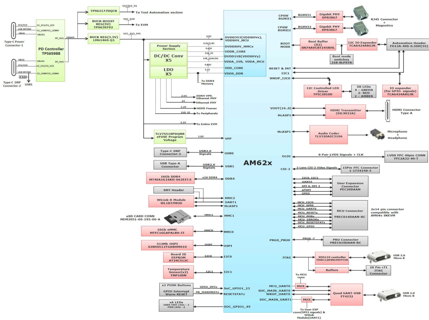
Figure 2-3. Functional Block Diagram of the AM62x SKEVM Board
