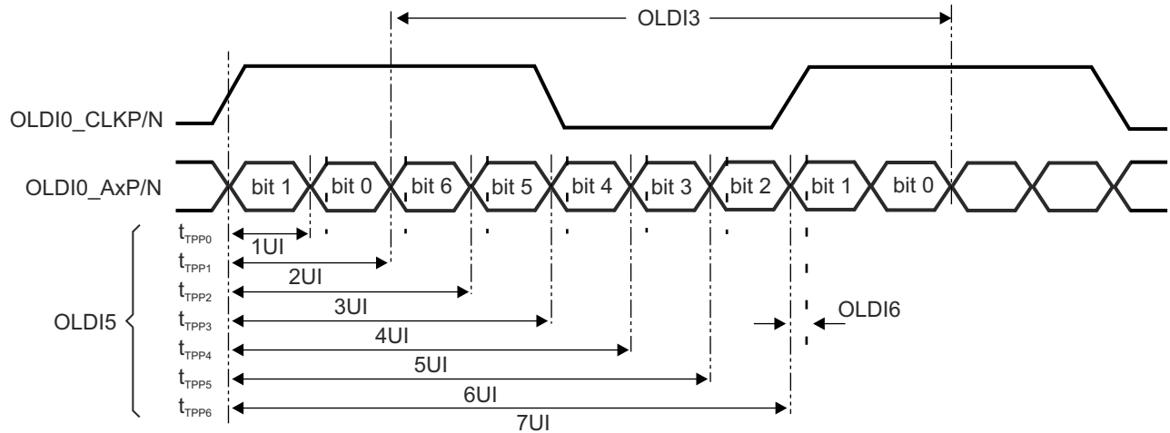
Figure 7-91. OLDI Output Pulse Positions
