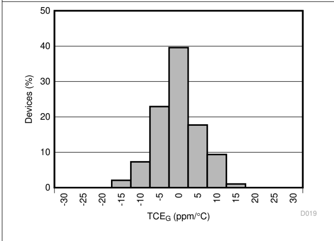
Figure 6-19. Gain Error Drift Histogram
