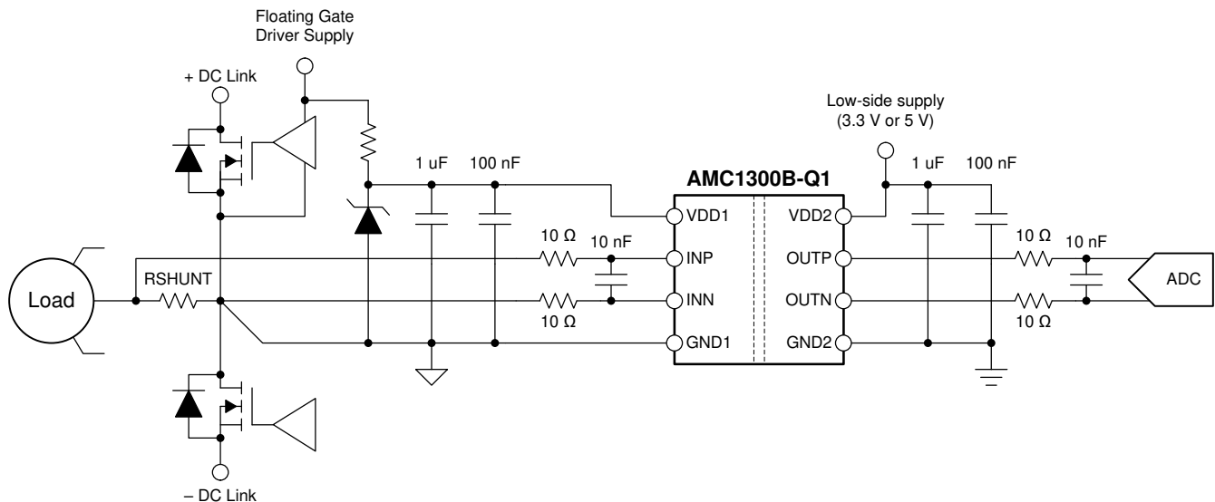
Figure 8-1. Using the AMC1300B-Q1 for Current Sensing in a Typical Application
