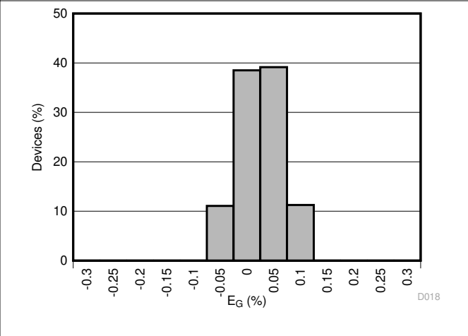
Figure 6-16. Gain Error Histogram
