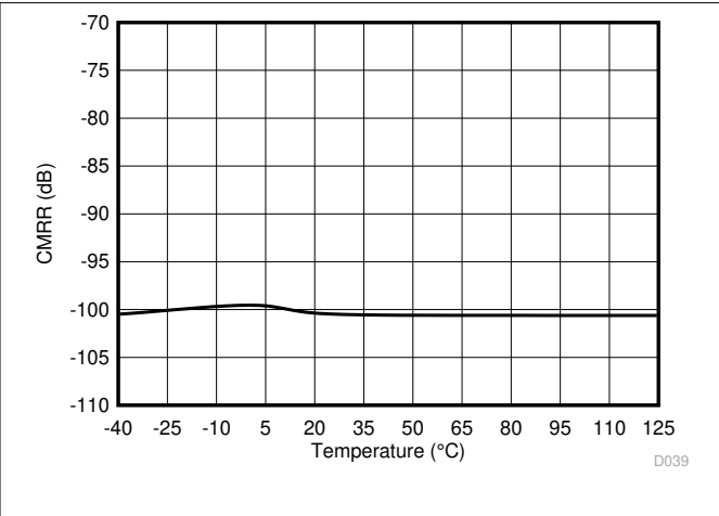
Figure 6-12. Common-Mode Rejection Ratio vs Temperature
