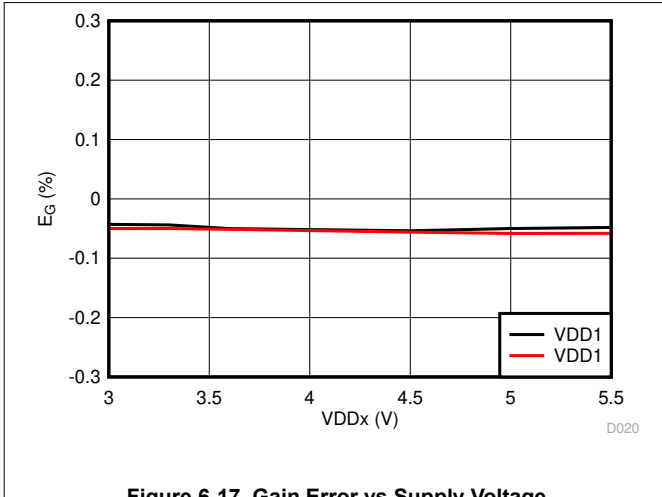
Figure 6-17. Gain Error vs Supply Voltage
