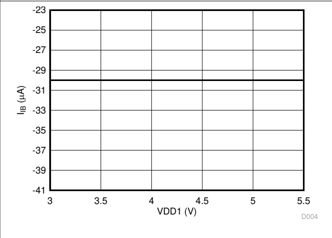
Figure 6-14. Input Bias Current vs High-Side Supply Voltage
