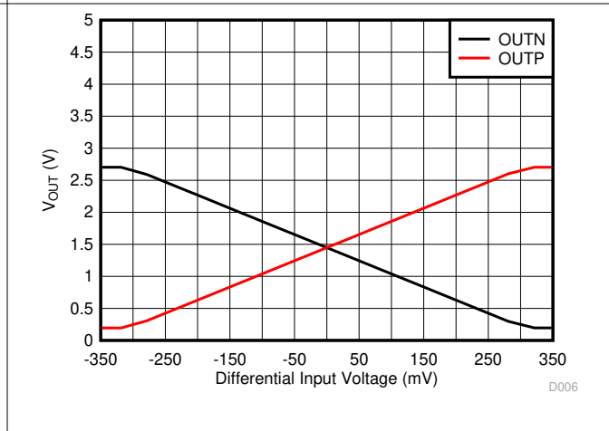
Figure 6-22. Output Voltage vs Input Voltage
