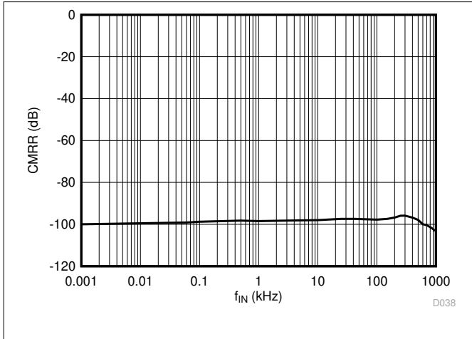
Figure 6-11. Common-Mode Rejection Ratio vs Input Frequency
