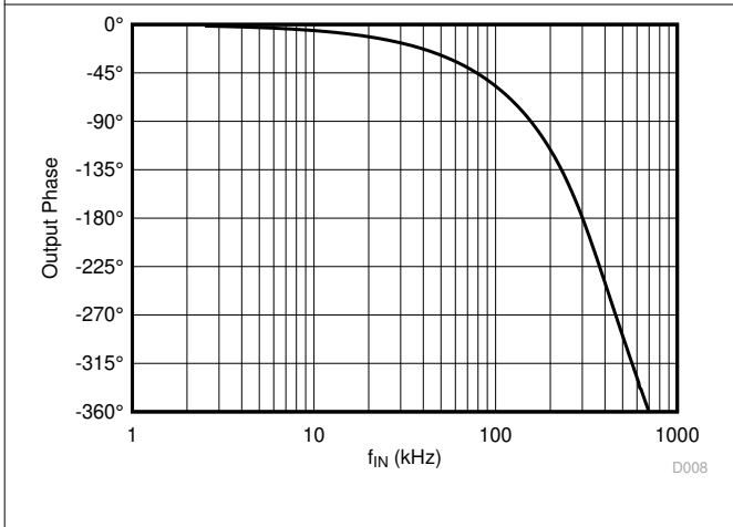
Figure 6-21. Output Phase vs Input Frequency
