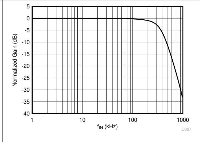
Figure 6-20. Normalized Gain vs Input Frequency
