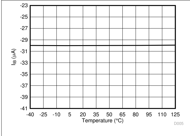
Figure 6-15. Input Bias Current vs Temperature
