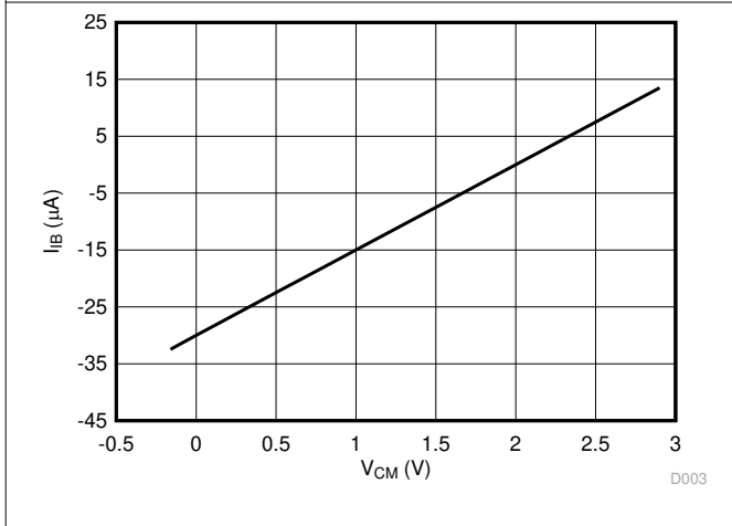
Figure 6-13. Input Bias Current vs Common-Mode Input Voltage
