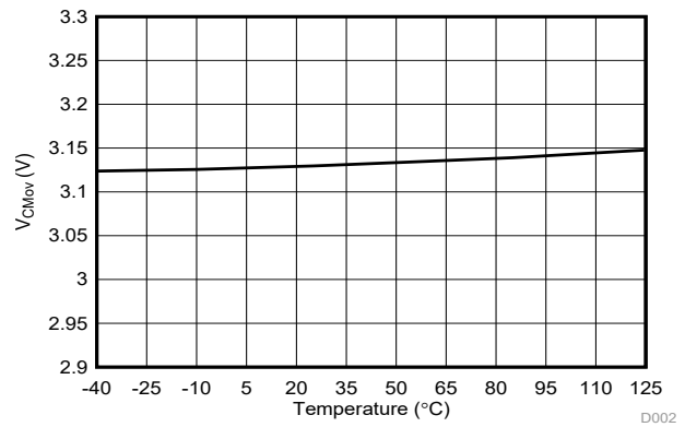
Figure 6-7. Common-Mode Overvoltage Detection Level vs Temperature
