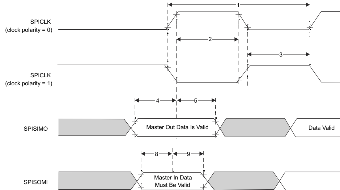
Figure 8-8. SPI Controller Mode External Timing (CLOCK PHASE = 1)
