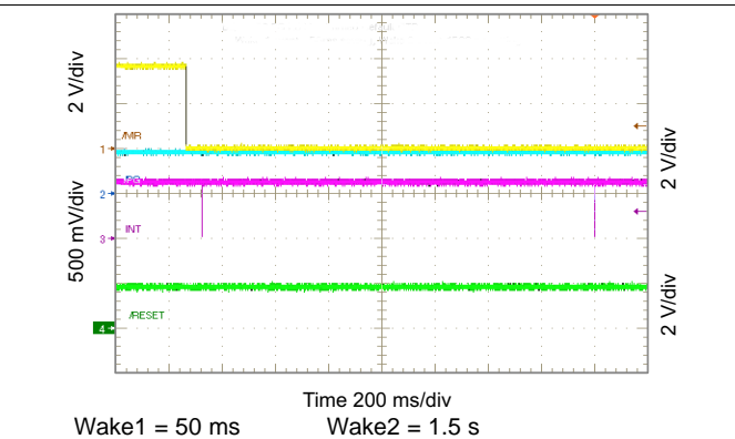
Figure 100. Show \overline{\text{MR}} Timing
