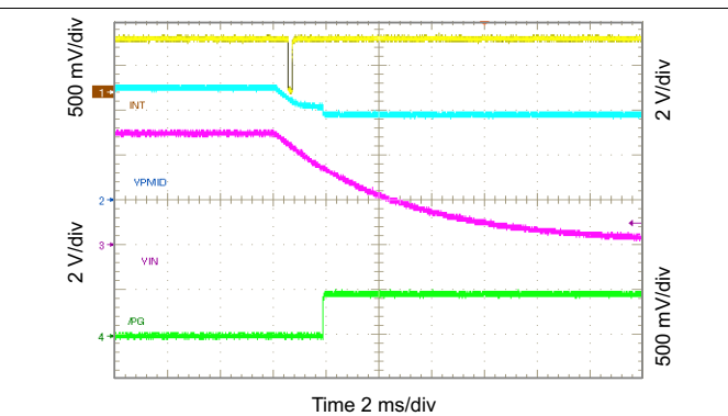
Figure 96. Show \overline{\text{PG}} and \overline{\text{INT}} Timing ( \text{VIN} Removal)
