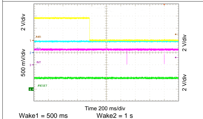
Figure 99. Show \overline{\text{MR}} Timing
