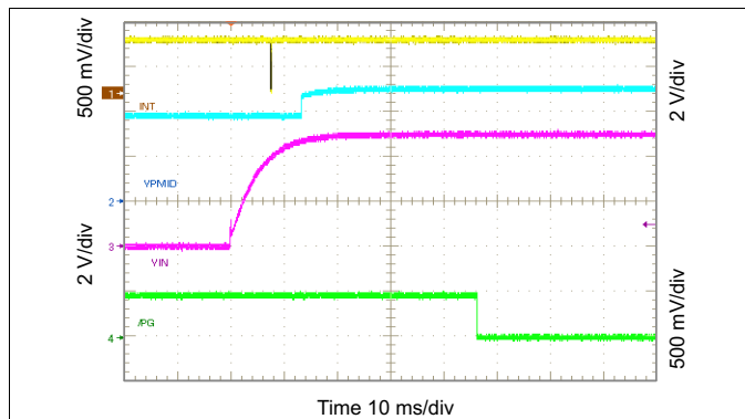
Figure 95. Show \overline{\text{PG}} and \overline{\text{INT}} Timing ( \text{VIN} Insertion)
