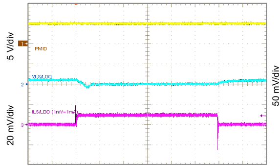
V_{LSLDO} = 0.8\text{ V} Figure 10-47. 0.8 V LSLDO Load Transient, 0 to 10 mA
