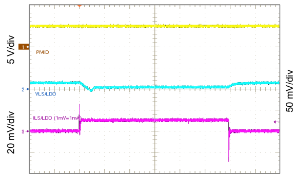
V_{LSLDO} = 1.8\text{ V} Figure 10-49. 1.8 V LSLDO Load Transient, 0 to 10 mA
