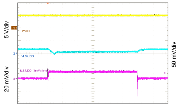
V_{LSLDO} = 2.5\text{ V} Figure 10-50. 2.5 V LSLDO Load Transient, 0 to 10 mA
