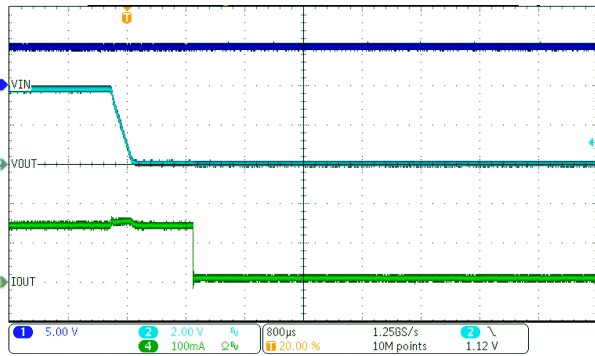
Figure 8-8. IN Transient Response
