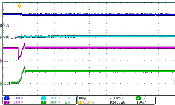
Figure 8-12. ISET Change Response
