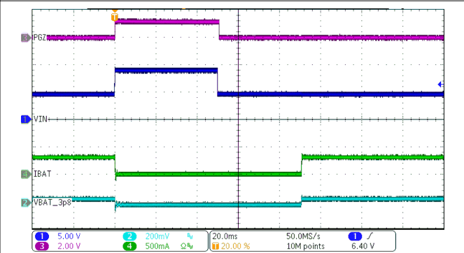
Figure 8-5. Charge Disable
