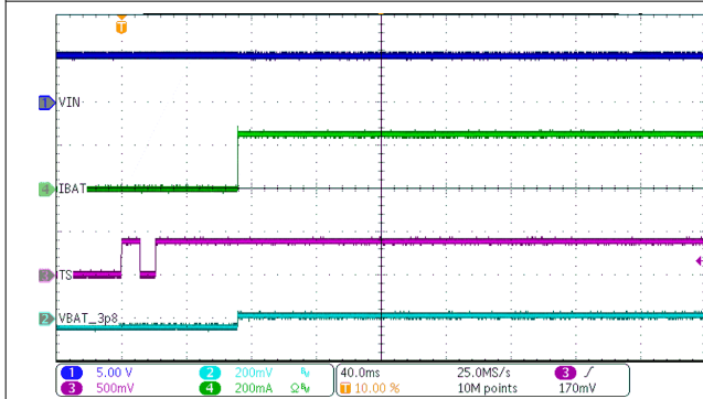
Figure 8-4. Power Down
