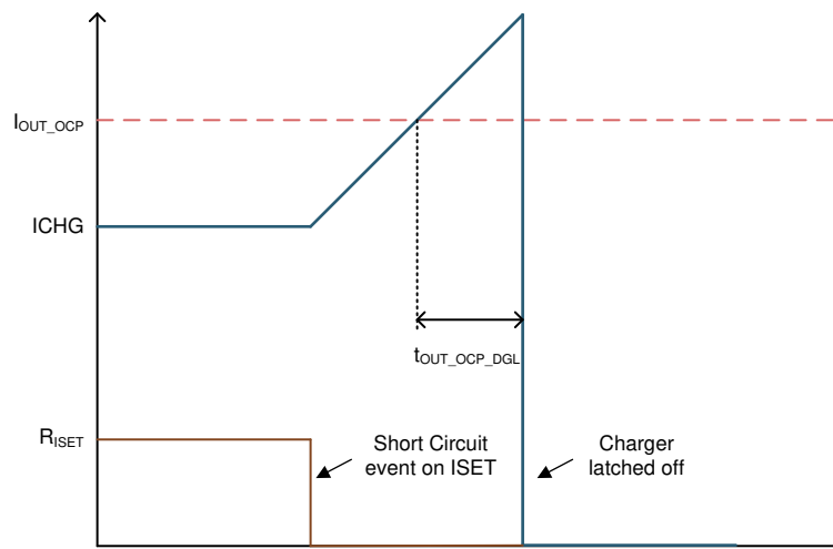
Figure 7-4. Overcurrent Protection
