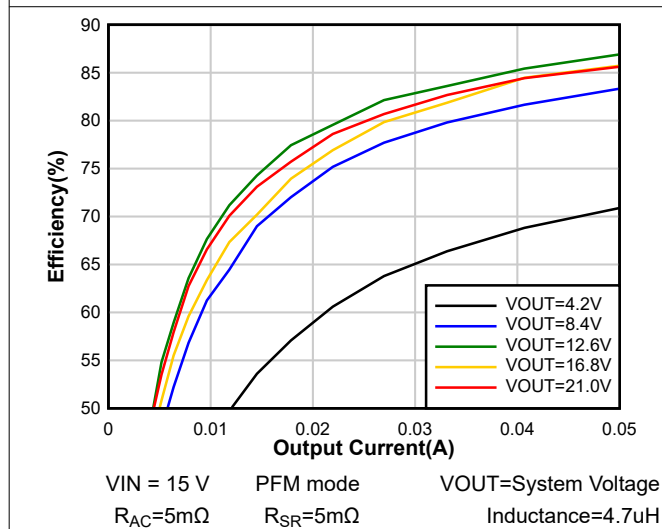
Figure 8-3. Light Load System Efficiency
