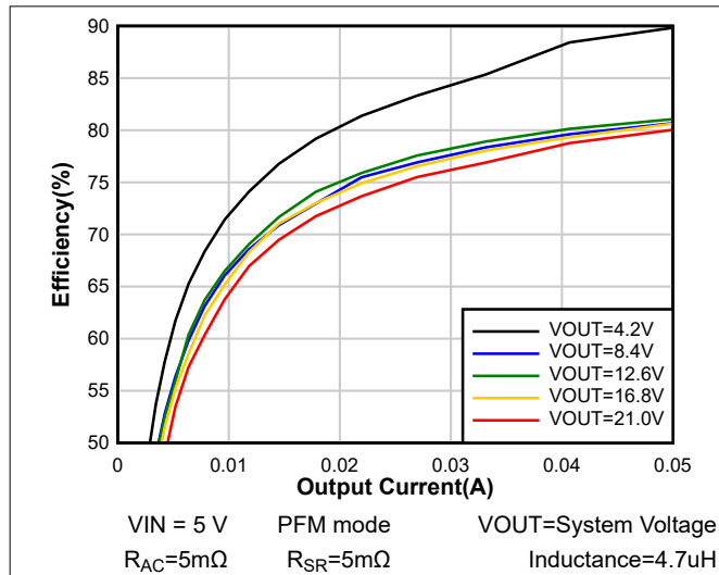
Figure 8-1. Light Load System Efficiency
