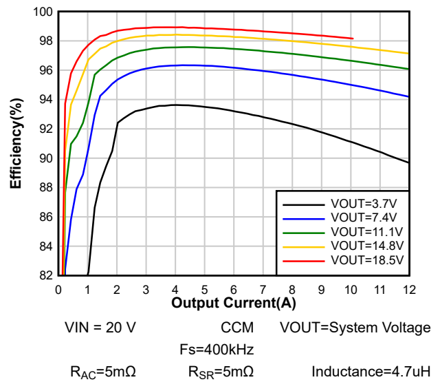
Figure 8-8. System Efficiency
