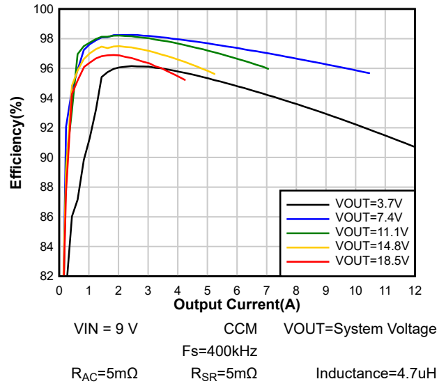
Figure 8-6. System Efficiency
