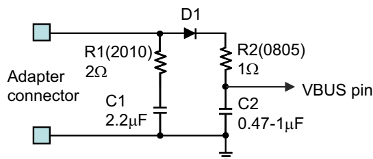
Figure 10-2. Input Filter
