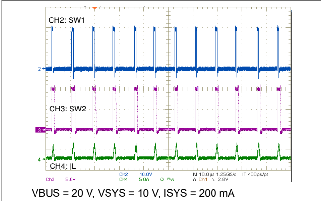
Figure 10-8. PFM Operation
