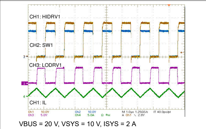
Figure 10-9. PWM Operation
