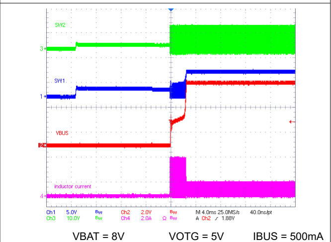
Figure 10-6. OTG Startup at 500-mA Load
