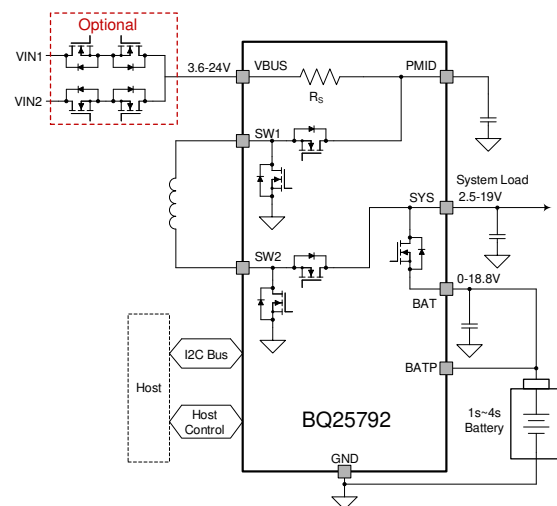
Simplified Schematic
