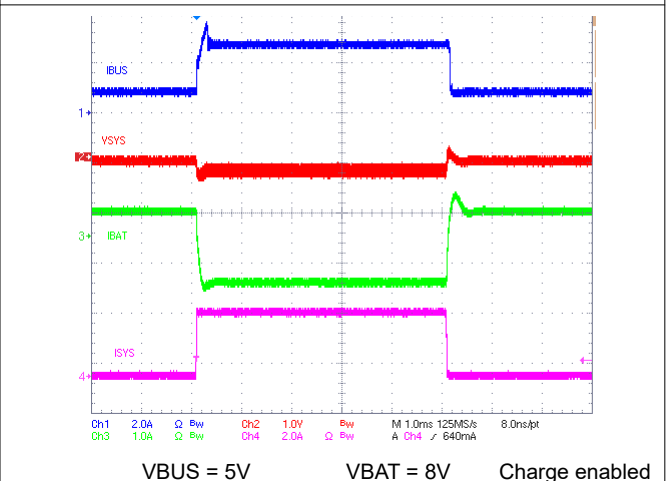
Figure 10-8. IINDPM Transient Response
