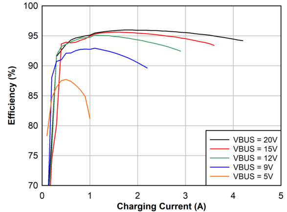
Figure 8-8. 4s Battery Charge Efficiency, 1.5 MHz
