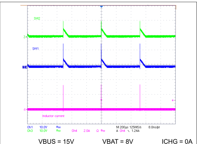
Figure 10-4. Buck Mode PFM without OOA
