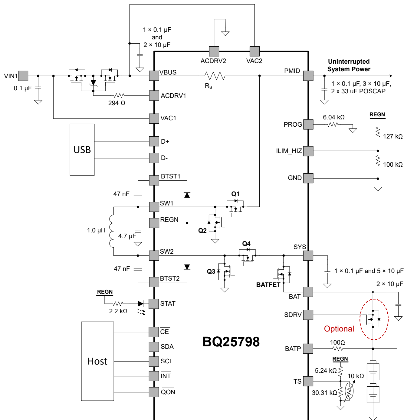
Figure 9-3. BQ25798 Application Diagram with Single Input Source, Back Up Mode and Ship FET
