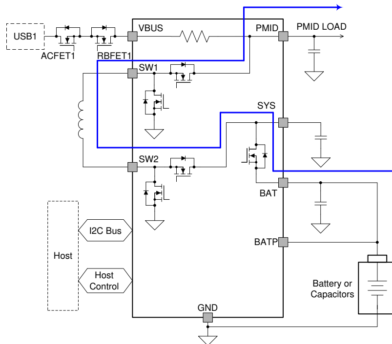
Figure 8-6. The Simplified Application Diagram for the Backup Mode
