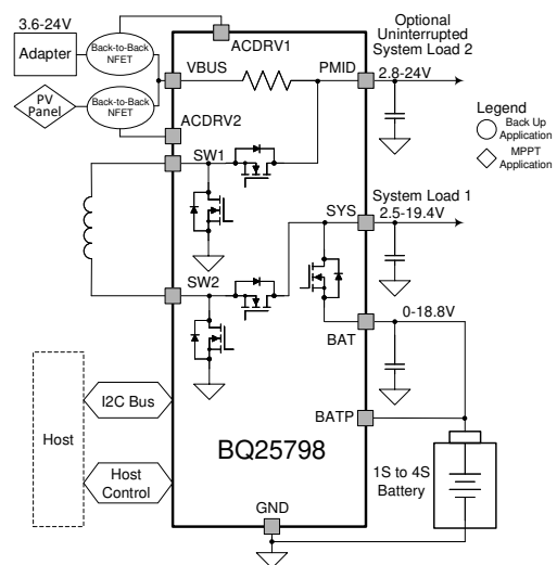
Simplified Schematic
