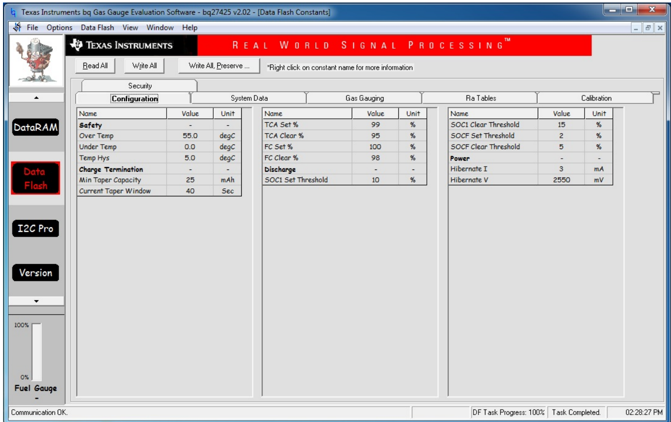
Figure 8. Data Flash Screen on bq27425 EVSW with EEPROM Values
