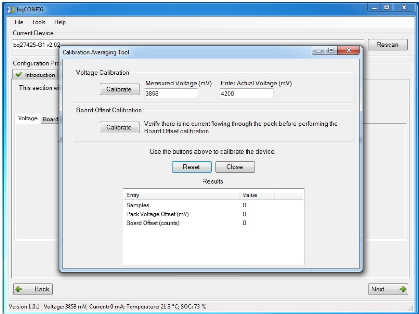
Figure 6. bqCONFIG Calibration Averaging Tool
