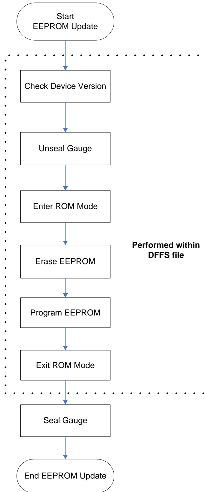
Figure 9. Basic DFFS Programming Flow
