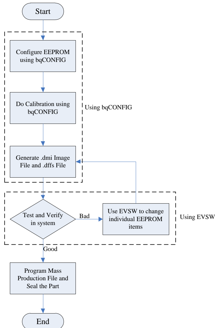
Figure 1. Flowchart for Creating Mass Production Files
