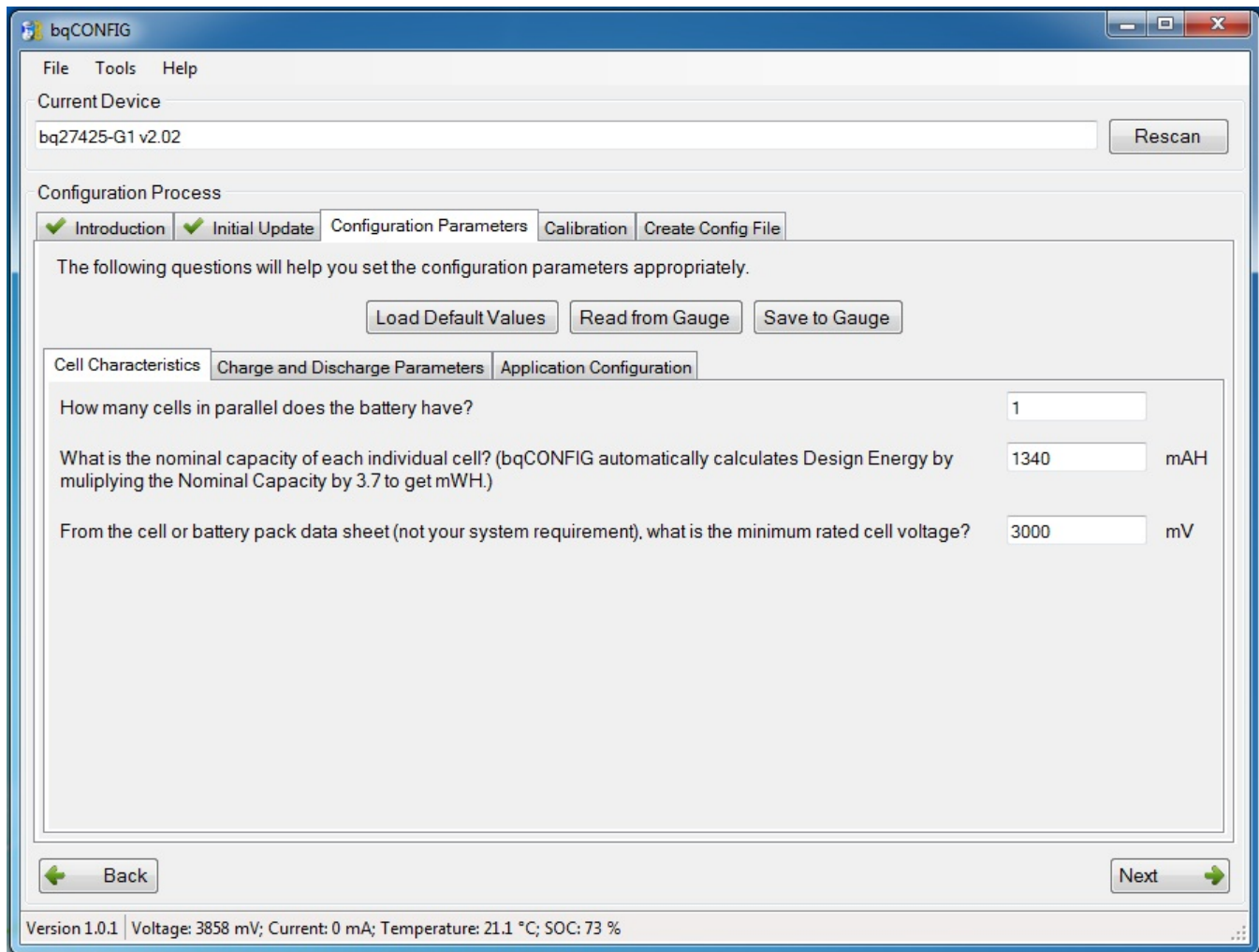
Figure 4. bqCONFIG Configuration Parameters Screen
