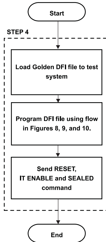
Figure 7. bq275xx Production Flow
