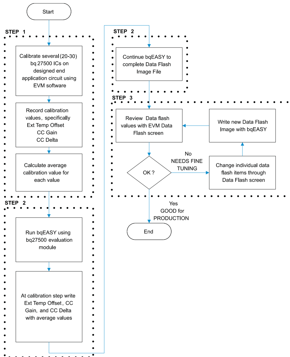
Figure 1. DFI Creation Flow
