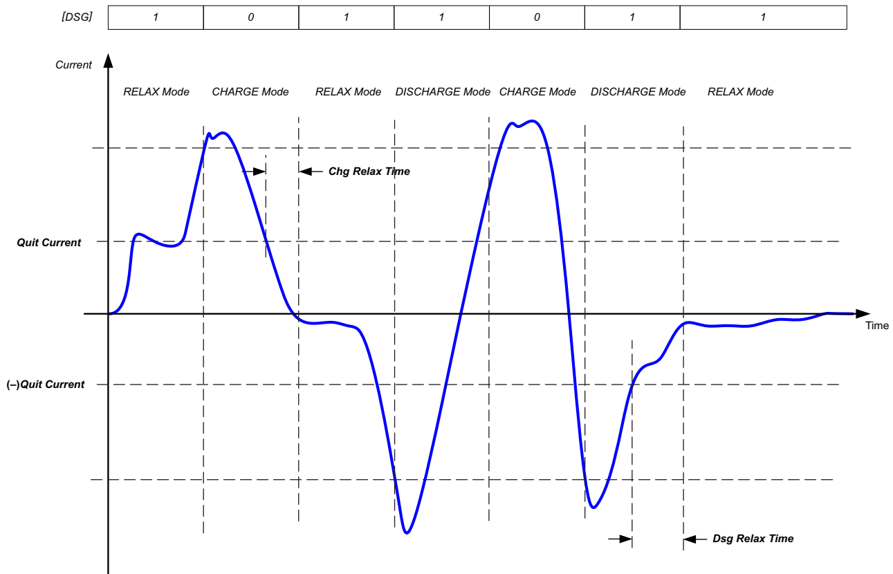
Figure 6-2. Fuel Gauge Operating Mode Example
